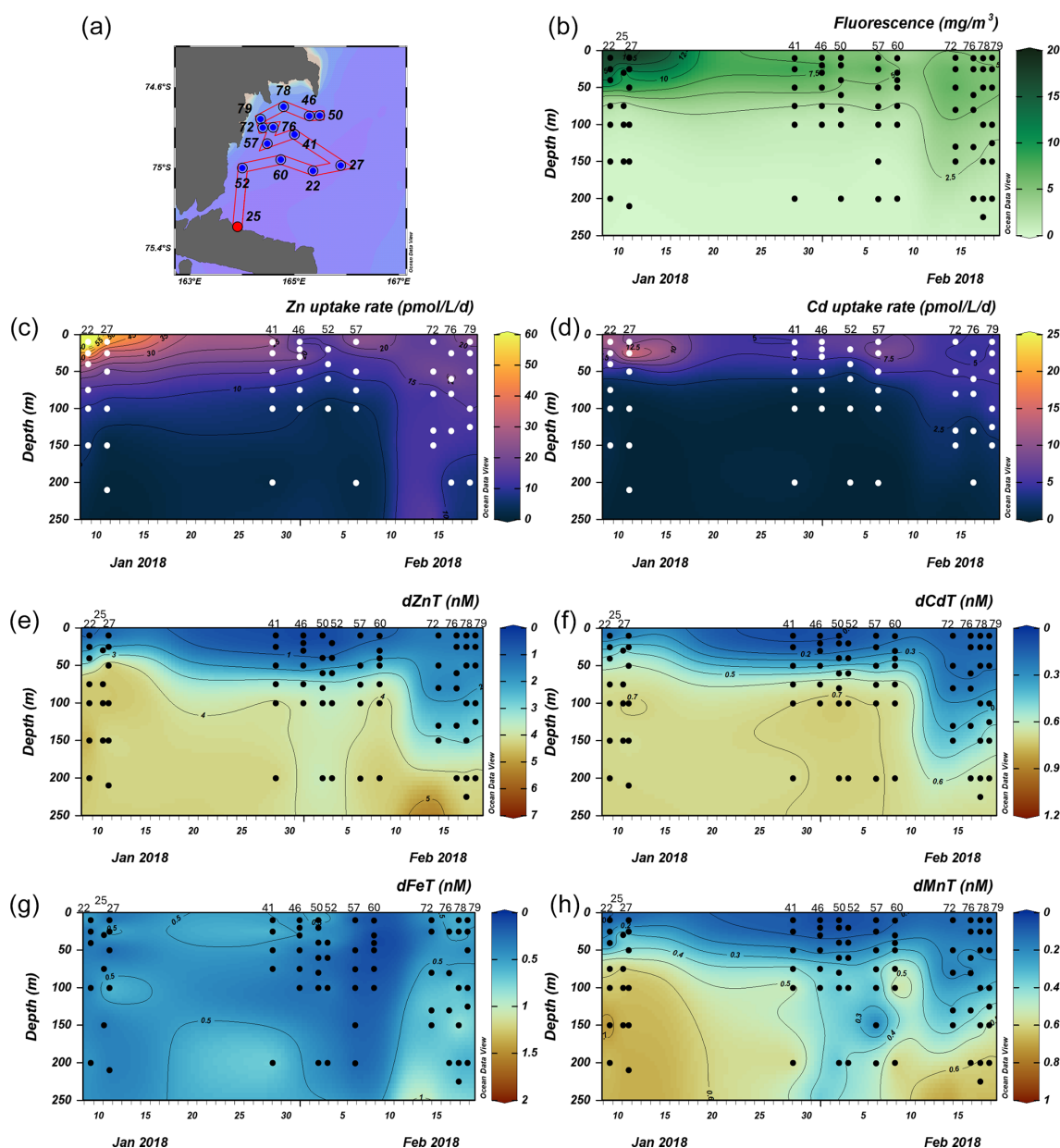
Figure 7. Total fluorescence and trace metal concentrations measured at Terra Nova Bay (TNB) stations shown over time. (a) Map showing station locations, (b) total chlorophyll (Chl) fluorescence, (c) total Zn uptake rates, (d) total Cd uptake rates, (e) total dissolved Zn, (f) total dissolved Cd, (g) total dissolved Fe, and (h) total dissolved Mn measured in the upper 250 m represented on a color scale. Uptake experiments were not performed at stations 70 and 34. Metal concentrations measured to 600 m depth are shown in Fig. S5. The following abbreviations are used: dZnT is total dissolved Zn, dCdT is total dissolved Cd, dFeT is total dissolved Fe, and dMnT is total dissolved Mn.
