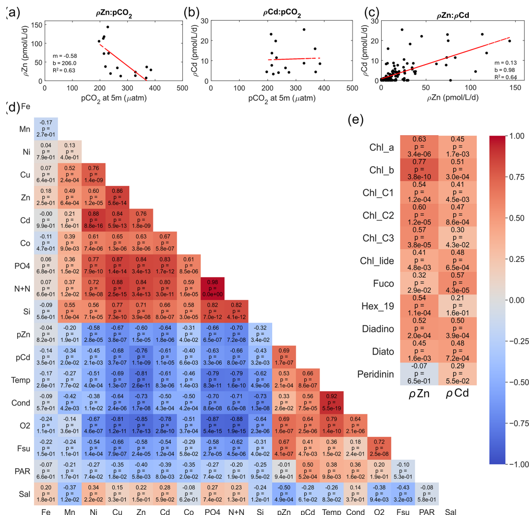
Figure 11. Relationships comparing seawater CO 2 partial pressure (pCO 2 ) at 5 m depth to (a) Zn uptake rates (ρZn; n = 15 , R^2 = 0.63 ) and (b) Cd uptake rates (ρCd; n = 15 ) measured at surface ( \leq 10 m) depths. (c) Relationship between ρZn and ρCd for all depths ( n = 121 , R^2 = 0.64 ). (d) Visual representation of the correlation matrix comparing all water column parameters measured with depth with warm and cool colors indicative of positive and inverse correlations, respectively. Pearson correlation coefficients and p values are shown. (e) Representation of the correlation matrix comparing ρZn and ρCd to various phytoplankton pigments. Fe, Mn, Ni, Cu, Zn, Cd, and Co labels correspond to total dissolved metal concentrations. PO 4 , N+N, and Si correspond to total dissolved concentrations of phosphate, the sum of nitrate+nitrite, and silicate. The following abbreviations are used: Temp is temperature, Cond is conductivity, O 2 is dissolved oxygen, Fsu is total fluorescence, PAR is photosynthetically active radiation, Sal is salinity, Chl_a is chlorophyll a, Chl_b is chlorophyll b, Chl_c1 is chlorophyll c1, Chl_c2 is chlorophyll c2, Chl_c3 is chlorophyll c3, chl_lide is chlorophyllide, Fuco is fucoxanthin, Hex_19 is 19'-hexanoyloxyfucoxanthin, Diadino is diadinoxanthin, and Diato is diatinoxanthin.
