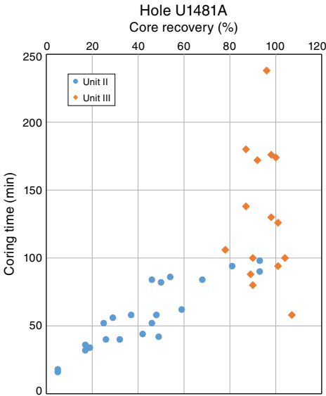
Figure F29. Coring time versus core recovery, Hole U1481A. Core recovery increases as coring time increases, and at high recovery, coring times vary widely.
