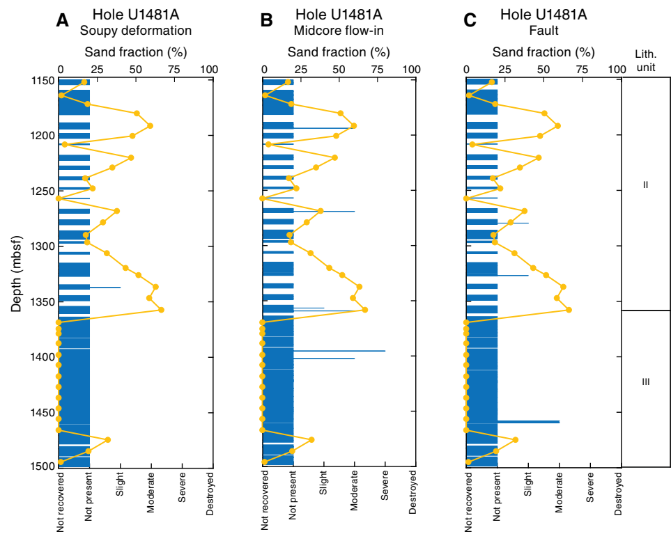
Figure F24. Intensity of (A) soupy deformation, (B) midcore flow-in, and (C) faults, Hole U1481A. Yellow points represent sand fraction for each core. Soupy deformation was observed only once. Midcore flow-in is rare and occurs at ~1350–1400 mbsf. Faults related to drilling occur rarely but are most common at ~1460 mbsf, where fracturing is intensified.
