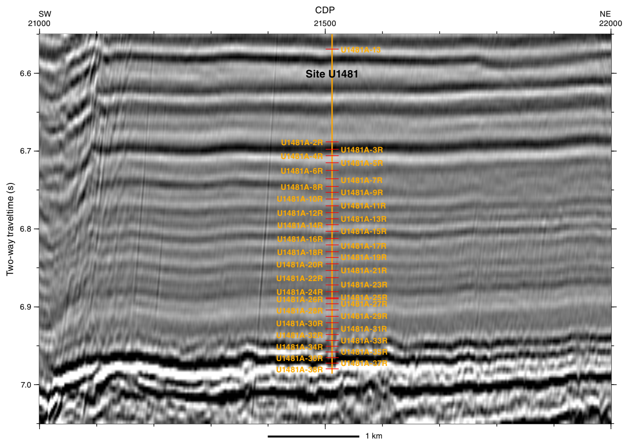
Figure F67. Regional interpretation of seismic Line BGR06-103 around Site U1481. Note that horizons can be traced laterally at all levels in the section even though faulting is pervasive. Seismic Horizon A is the top of the sand body at 30 mbsf close to the top of Unit II. Seismic Horizon B is the downward reduction in reflectivity defined at Site U1480 and correlated to this profile along Line MD116. B* is an equivalent downward reduction in reflectivity defined on this profile. Seismic Horizon C is the positive polarity equivalent to the HANP reflection identified closer to the subduction zone by Dean et al. (2010). This horizon corresponds to the Unit II/III boundary. Seismic Horizon D is the acoustic basement.
