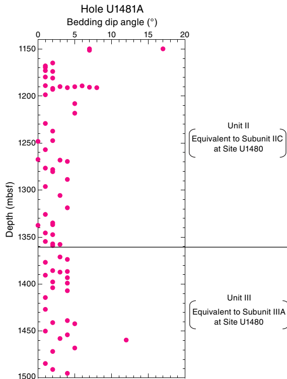
Figure F16. Bedding dip angles, Hole U1481A. Note that most dips are between 0° and 5°. Angles >5° are attributed to synsedimentary slumping processes, and in some cases two measurements at the same depth reflect dips on opposite limbs of a slump fold.
