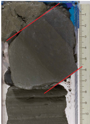
Figure F25. Core segment that was drilled, dropped back into the hole, and recored (U1481A-15R-1, 0–11 cm; 1276.20–1276.31 mbsf). Red lines indicate initial core surfaces perpendicular to bedding. Although this structure is observed at the top of Section 15R-1, the same phenomenon is observed in the middle of a core and is interpreted to form as the drill bit lifts off the coring surface due to ship heave.
