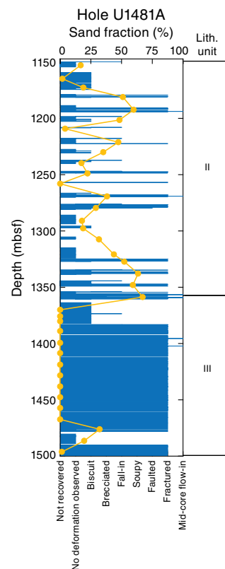
Figure F21. Distribution of drilling disturbance structures, Hole U1481A. Yellow points represent sand fraction for each core. Unit II remains minimally disturbed with fracturing and biscuiting as primary modes of drilling deformation. Fractures increase in abundance below ~1325 mbsf. Biscuits, fracturing, and faulting become more prevalent in Unit III and dominate the deformation style. Breccias, fall-in, soupy sand disturbance, and mid-core flow-in are rare.
