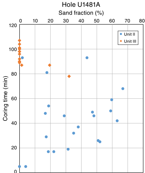
Figure F28. Coring time versus sand fraction, Hole U1481A. These parameters are weakly correlated in Unit II. The longest coring times occurred in Unit III where minimal sand was recovered, and when some sand was present, coring was faster.
