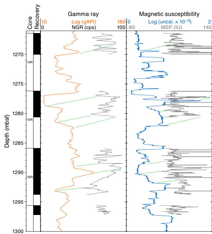
Figure F59. Comparison of gamma ray and magnetic susceptibility logs with core data from an interval with incomplete recovery, Hole U1481A. Horizontal scales are shifted so that overlaps are limited. Magnetic susceptibility core data are from the MSP, and gamma ray logs are from the Enhanced Digital Telemetry Cartridge. Dashed green lines = tentative correlations.
