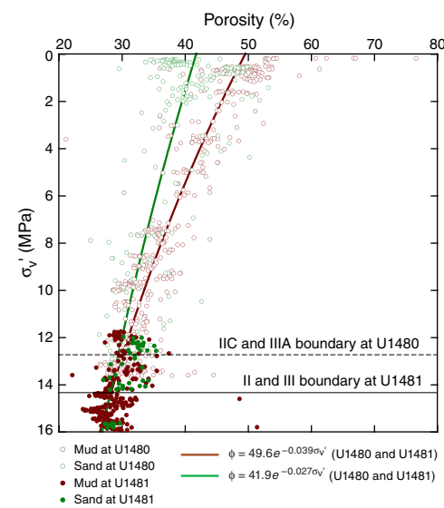
Figure F49. MAD porosity versus effective vertical stress at Sites U1480 and U1481 showing consistency between the two sites.
