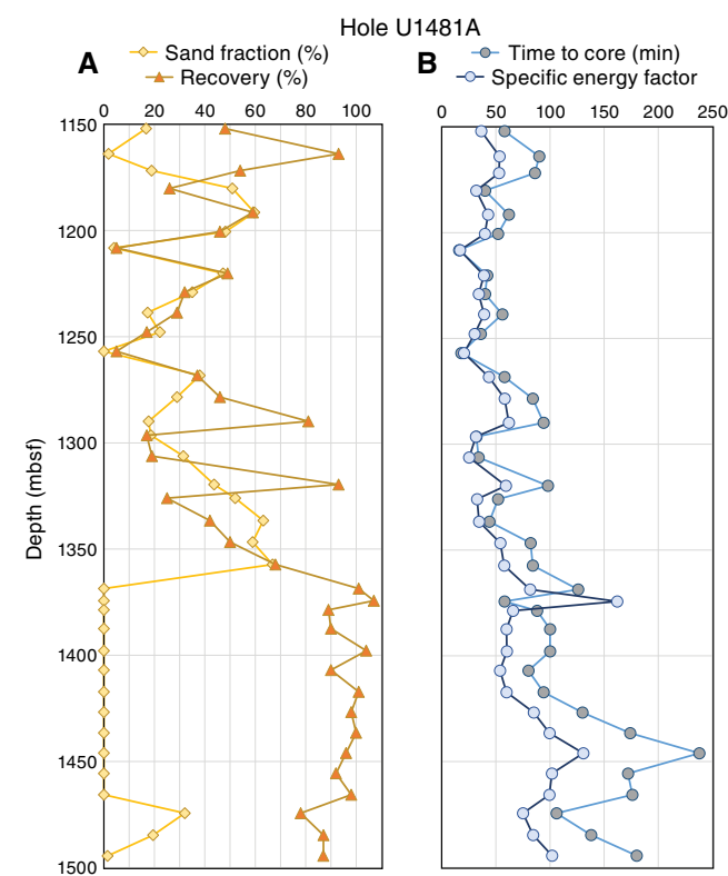
Figure F27. A. Sand fraction and recovery, Hole U1481A. Note divergence in these parameters in the first three cores, but recovery and sand fraction track one another from 1180 mbsf to the base of Unit II (1360 mbsf). In Unit III (below 1360 mbsf) sand is not evident except for the interval at the base of the hole, and recovery is consistently high. B. SEF and time to core. As in Hole U1480G, SEF largely follows time to core, indicating that ROP is the dominant control on SEF. Note how the highest SEF values are in Unit III below 1360 mbsf, and the highest SEF is in Core 33R at 1445 mbsf.
