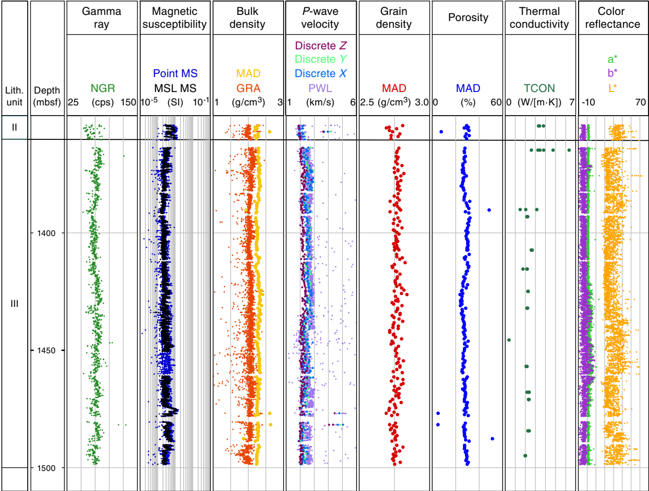
Figure F42. Physical property measurements deeper than 1350 mbsf, Site U1481. MSL data for Core 362-U1481A-34R were removed due to a calibration error that resulted in anomalously low values. Lithostratigraphic Unit II/III boundary is shown for reference. For discrete P -wave velocity measurements, all X , Y , Z measurements are from the P -wave caliper.
