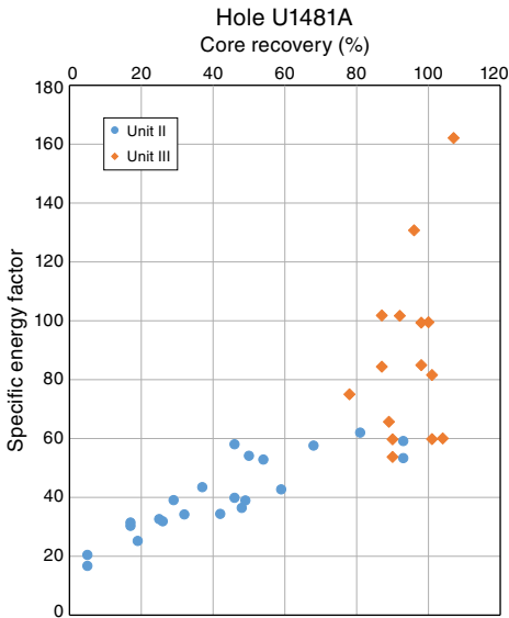
Figure F30. SEF versus core recovery, Hole U1481A. Core recovery increases with increasing SEF in Unit II. More work was required to obtain cores in Unit III than Unit II, and core recovery was consistently high.
