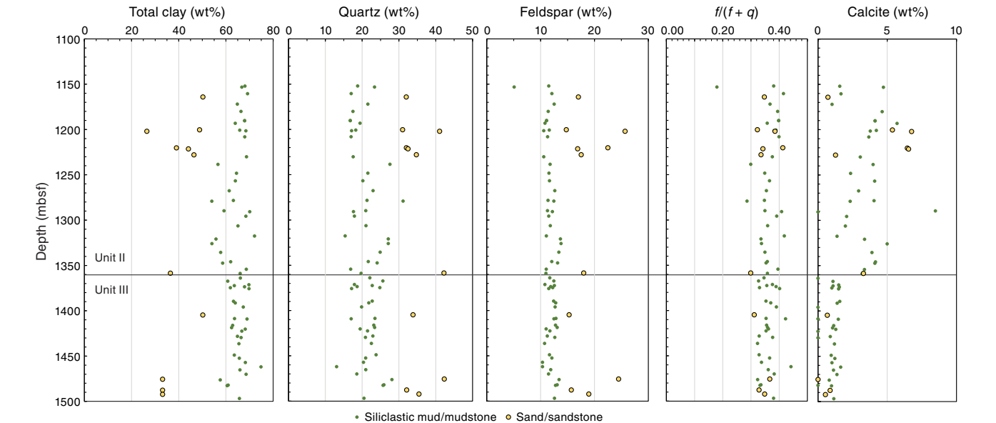
Figure F7. Bulk mineralogy as determined by X-ray diffraction, Site U1481. f = feldspar, q = quartz.
