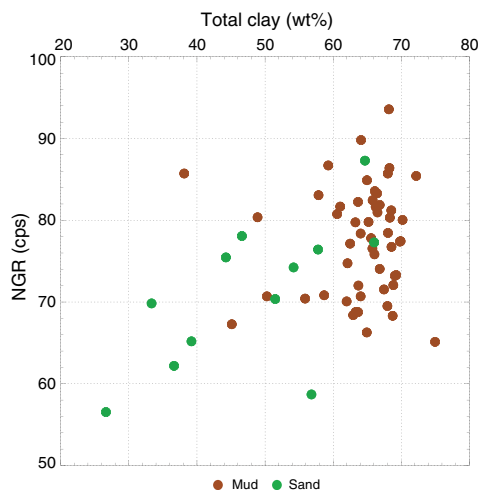
Figure F44. NGR versus total clay content from XRD analyses, Site U1481.
