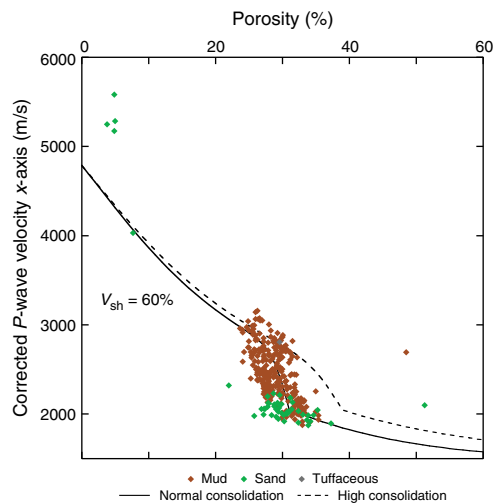
Figure F50. Corrected discrete P -wave velocity in the x -direction versus porosity, Site U1481. Solid and dashed lines are the trends derived from global compilations (Erickson and Jarrard, 1998) for normal and high consolidation, respectively, assuming V_{sh} (volume of clay) = 60%.
