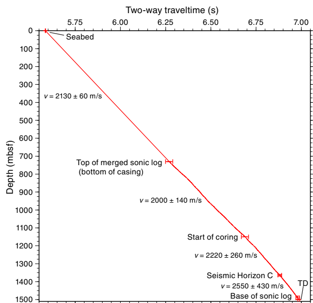
Figure F68. Summary of tie points (key depth points and time-depth point) between time on seismic Line BGR06-103 and depth at Site U1481. In detail, the tie between time and depth is accomplished using the sonic logs, so these represent selected key intervals only. An estimate of the error in time and depth for each tie is included (bars on tie points), along with the resulting interval velocity between each tie and the error in that estimate. TD = total depth.
