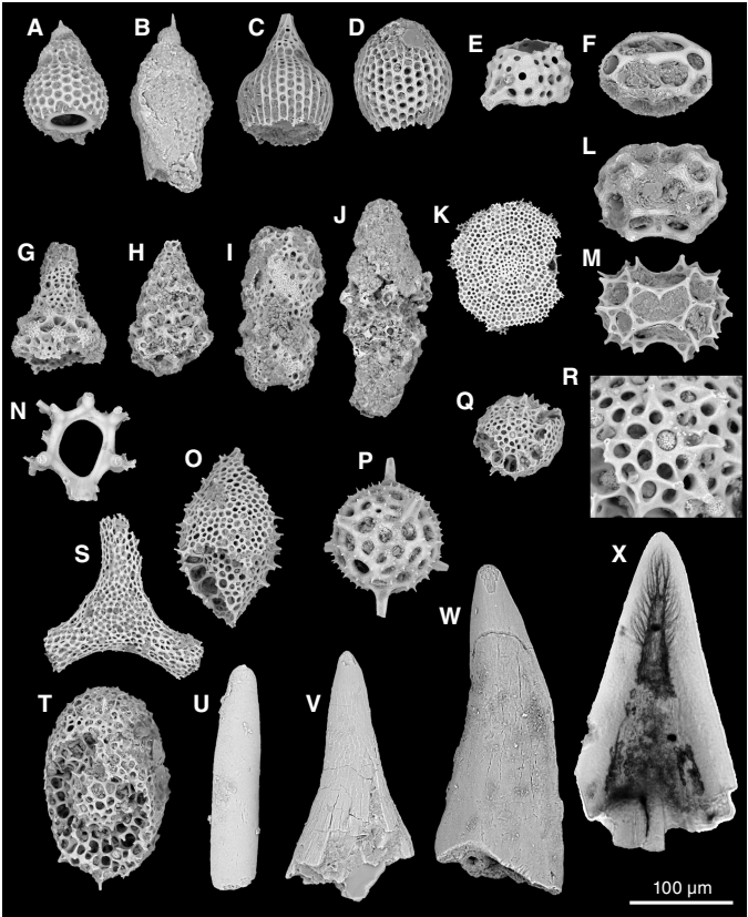
Figure F31. Composite plate of Quaternary radiolarians, Hole U1481A. A, B. Stichocorys wolffii Haeckel. C. Calocyclus virginis Haeckel. D. Carpocanopsis cingulata Riedel and Sanfilippo. E. Dorcadospirys simplex s.s. F. Liriospyris mutuarii Goll. G. Broken specimen of Didymocytis antepenultima (Riedel and Sanfilippo) showing the wide, spongy polar column. H. Broken specimen of Didymocytis laticonus (Riedel) showing the spongy polar column. I. Didymocytis antepenultima (Riedel and Sanfilippo). J. Didymocytis laticonus (Riedel). K. Stylodictya validispina Jørgensen. L, M. Dorcadospirys sp. N. Zygocircus productus (Hertwig). O, Q. Radiolarian indet. P. Actinomma sp. R. Close-up of Q showing numerous pyrite framboids. S. Dictyocoryne sp. T. Larcopyle nebulum Lazarus. U–X. Ichthyoliths. A, B: 362-U1481A-29R-4, 63–65 cm; C, D, F, L, M, W: 38R-5, 32–33 cm; E: 28R-6, 6–8 cm; G, H, J, K, N–Q, S, T: 29R-5, 24–26 cm; I: 24R-5, 84–86 cm; U, V: 26R-4, 32–33 cm; X: 32R-4, 73–75 cm.
