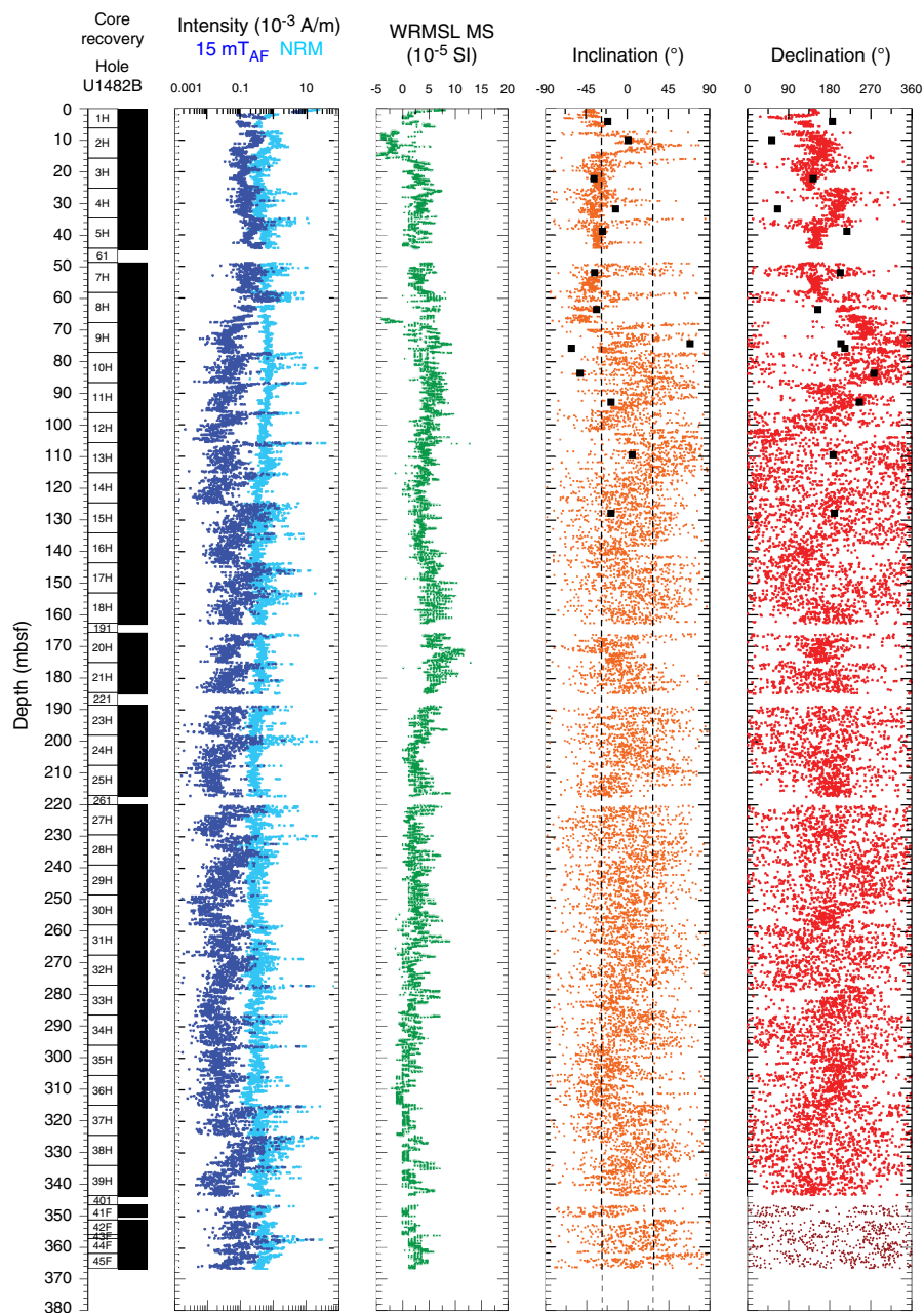
Figure F26. NRM intensities before and after 15 mT AF demagnetization, WRMSL magnetic susceptibility (MS), and inclination (dashed lines = expected values of \pm 28^\circ for the site latitude assuming a GAD) and declination (red = azimuthally corrected values, dark red = unoriented HLAPC core values) after 15 mT AF demagnetization, Hole U1482B. Black squares = discrete sample locations.
