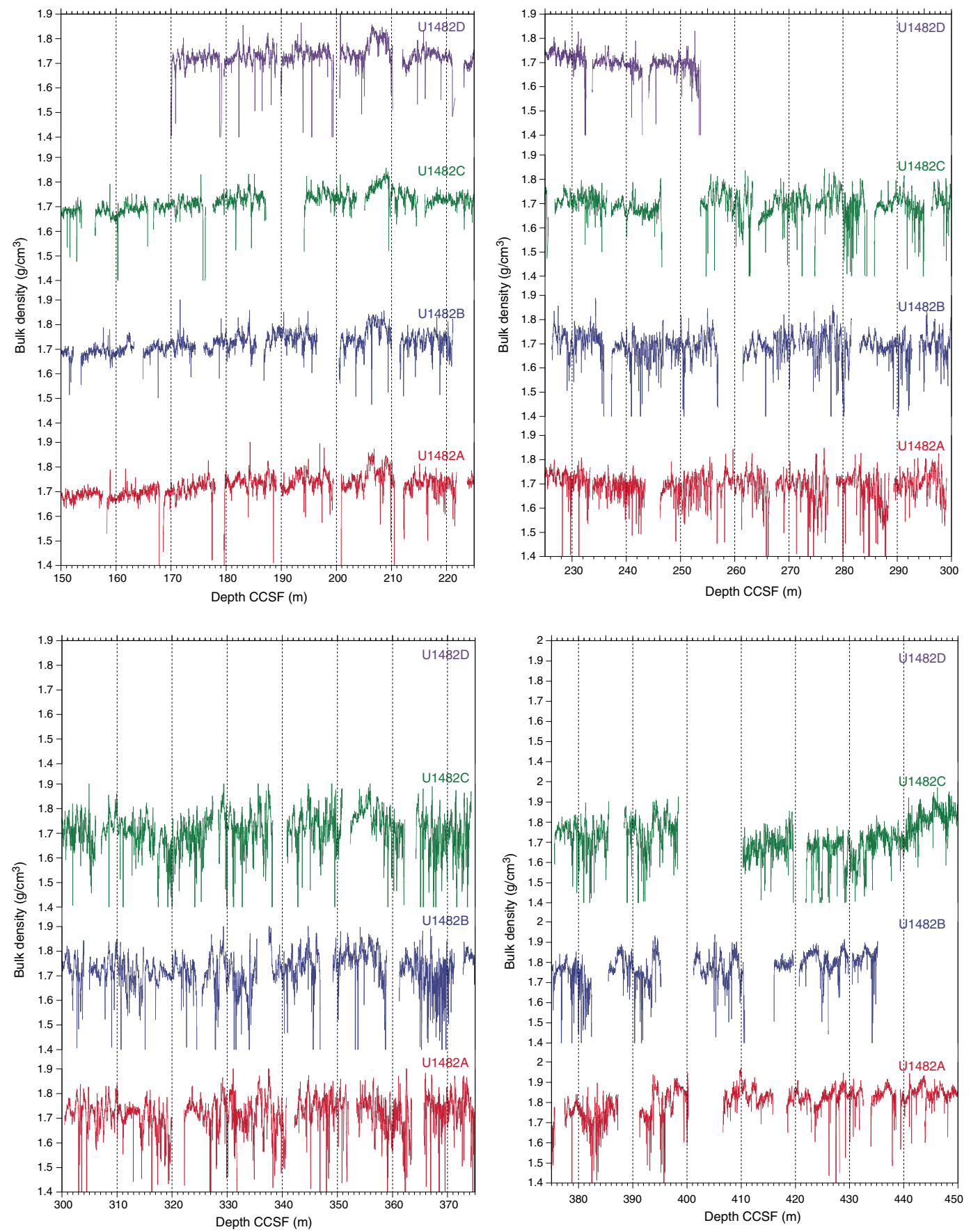
Figure F36 (continued). (Continued on next page.)
