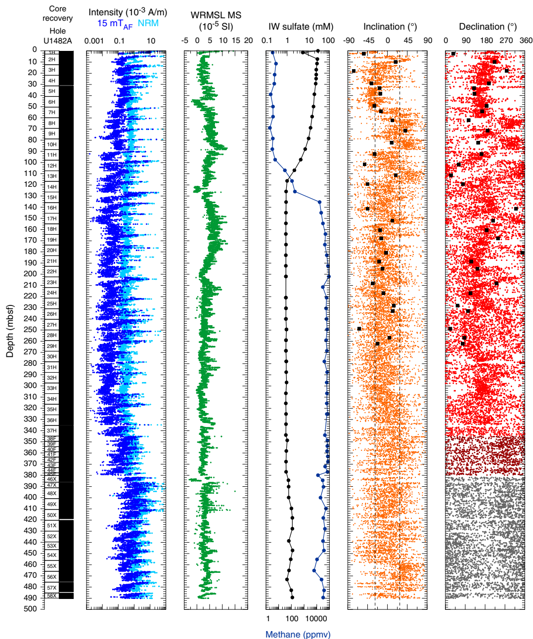
Figure F24. NRM intensities before and after 15 mT AF demagnetization, WRMSL magnetic susceptibility (MS), interstitial water (IW) sulfate and methane concentrations, and inclination (dashed lines = expected values of \pm 28^\circ for the site latitude assuming a geocentric axial dipole [GAD]) and declination (red = azimuthally corrected values, dark red = unoriented HLAPC core values, gray = XCB core values) after 15 mT AF demagnetization, Hole U1482A. Black squares = discrete sample locations.
