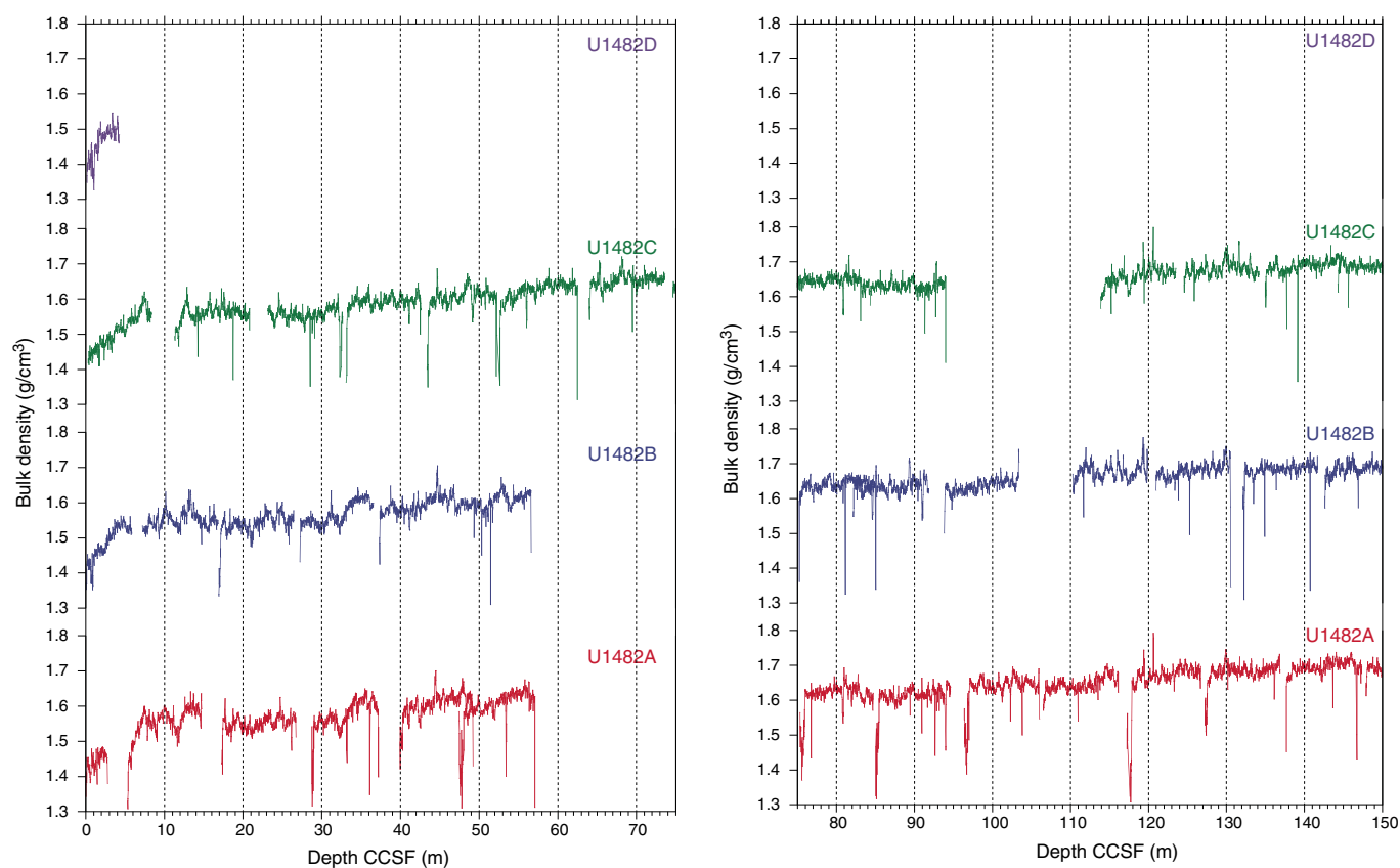
Figure F36. WRMSL GRA bulk density data, Holes U1482A–U1482D. (Continued on next two pages.)
