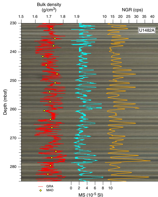
Figure F30. WRMSL GRA bulk density and magnetic susceptibility and NGR overlaid on core photos (generated using Code for Ocean Drilling Data [CODD] [Wilkins et al., 2017]) from Hole U1482A, 230–285 mbsf. cps = counts per second. cps = counts per second.
