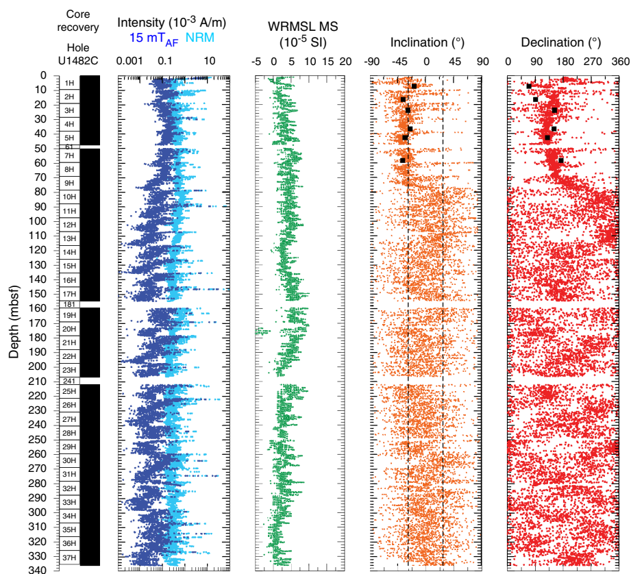
Figure F27. NRM intensities before and after 15 mT AF demagnetization, WRMSL magnetic susceptibility (MS), and inclination (dashed lines = expected values of \pm 28^\circ for the site latitude assuming a GAD) and declination (red = azimuthally corrected values) after 15 mT AF demagnetization, Hole U1482C. Black squares = discrete sample locations.
