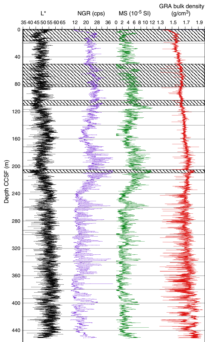
Figure F40. Spliced WRMSL GRA bulk density, MS, NGR, and L* data, Site U1482. Cross-hatched bars = intervals with differences in WRMSL data variations between cores from different holes. These sections have soft-sediment deformation and stratigraphic discontinuity between holes and may contain missing intervals or repeated intervals. cps = counts per second.
