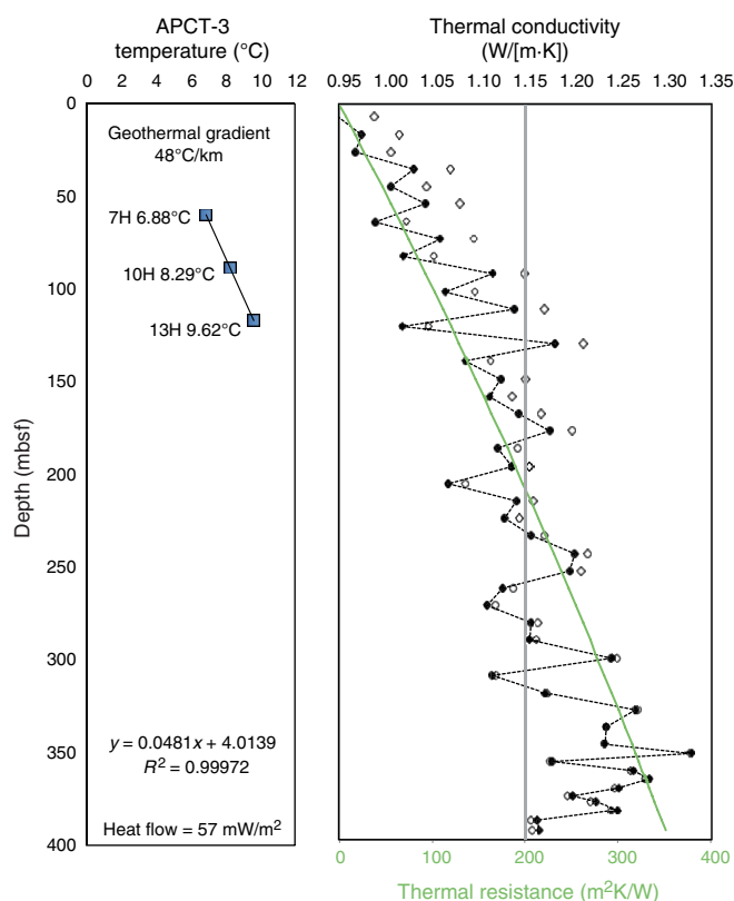
Figure F35. Heat flow calculations, Hole U1482A. Green line = calculated thermal resistance, gray vertical line = average thermal conductivity value used for calculation of thermal resistance, solid diamonds and dashed line = corrected thermal conductivity, open diamonds = uncorrected thermal conductivity.
