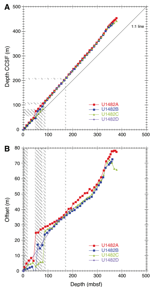
Figure F41. A. Comparison of mbsf and composite depth scales in the Site U1482 splice (0–451.26 m CCSF). B. Comparison of the growth of cumulative depth offset and the mbsf depth scale. Shaded bars show intervals with soft-sediment deformation and uncertain correlation.
