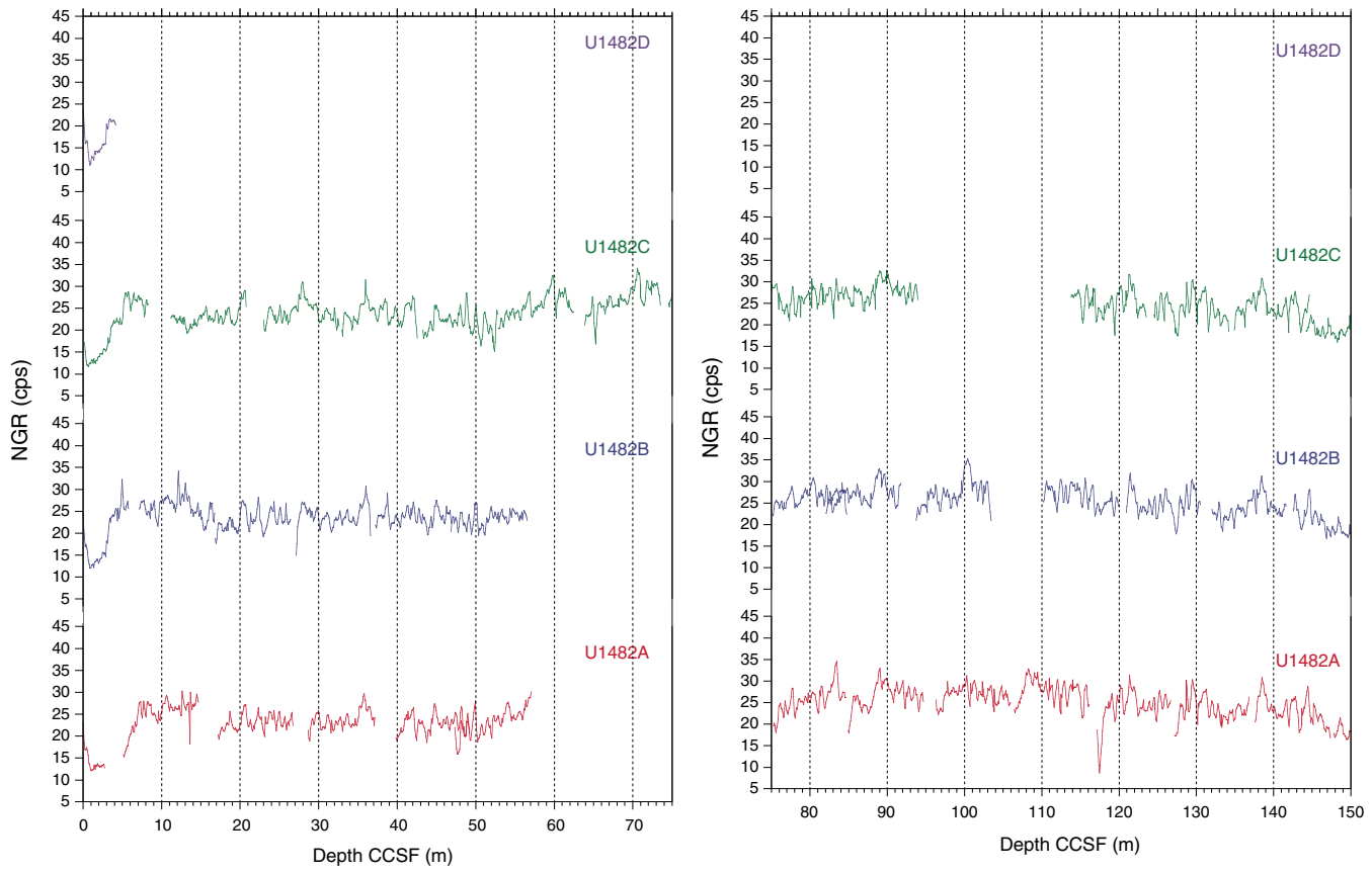
Figure F38. WRMSL NGR data, Holes U1482A–U1482D. cps = counts per second. (Continued on next two pages.)
