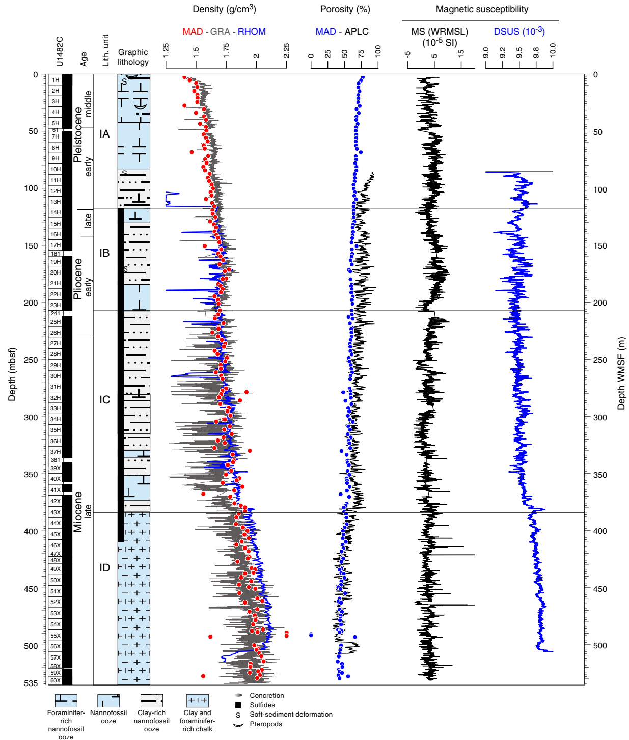
Figure F48. Wireline log measurements compared to sediment core measurements, Hole U1482C. Small depth discrepancies may exist between the mbsf and WMSF depth scales (usually <2 m).
