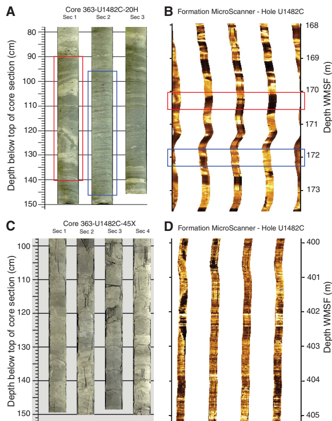
Figure F49. A–D. Processed FMS images and core photographs of sections from corresponding depths, Hole U1482C. Additional image enhancement of the FMS image may prove helpful in defining bedding characteristics and primary sedimentary structures. See text for detailed explanation.
