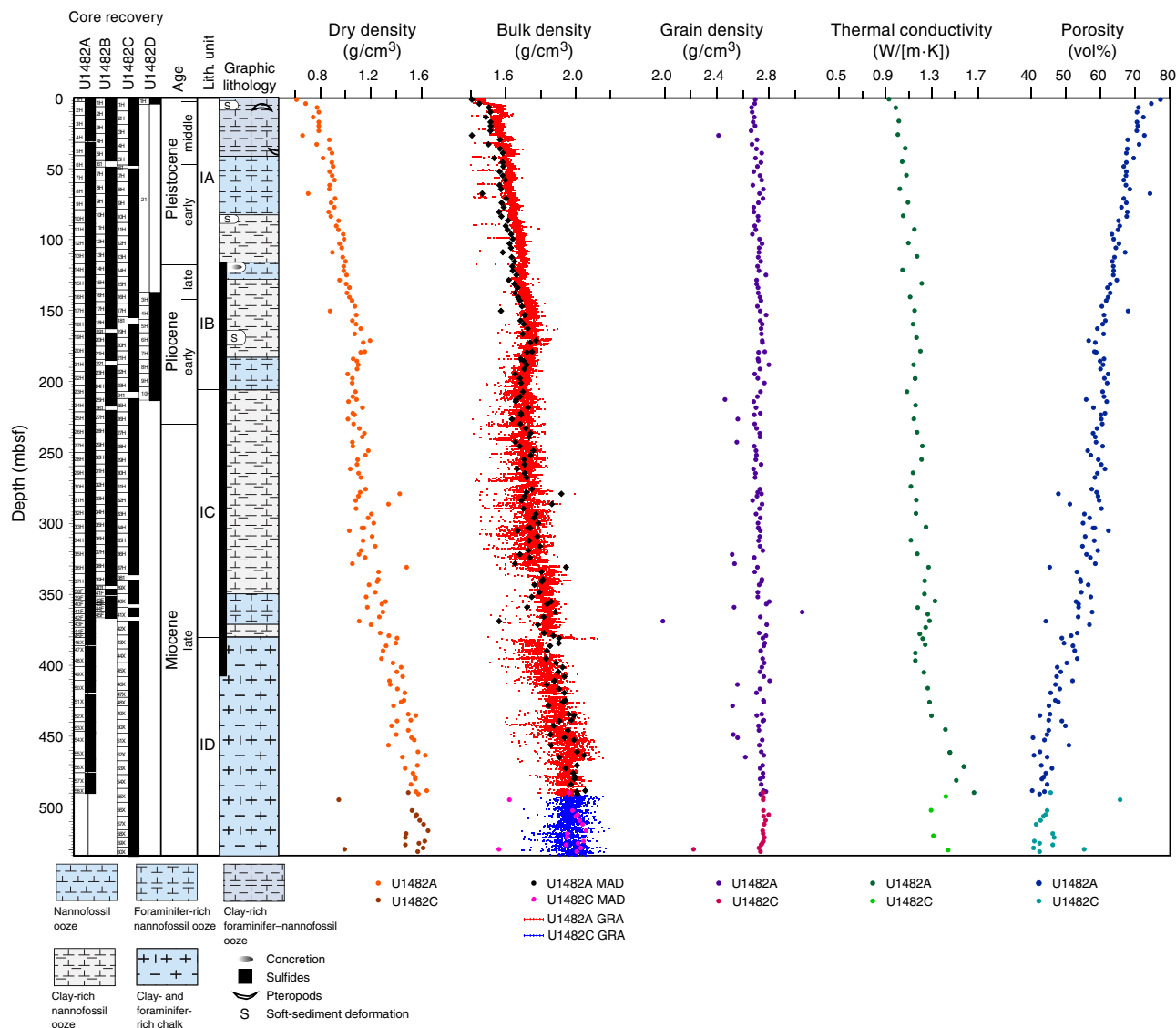
Figure F33. MAD discrete sample dry, bulk, and grain densities and porosity, WRMSL GRA bulk density, and thermal conductivity, Holes U1482A and U1482C.
