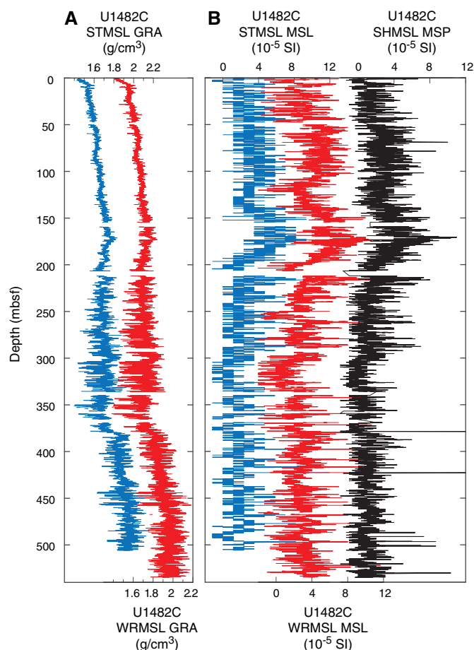
Figure F29. Comparison of cleaned (A) GRA bulk density and (B) magnetic susceptibility data obtained using different measurement tracks, Hole U1482C.
