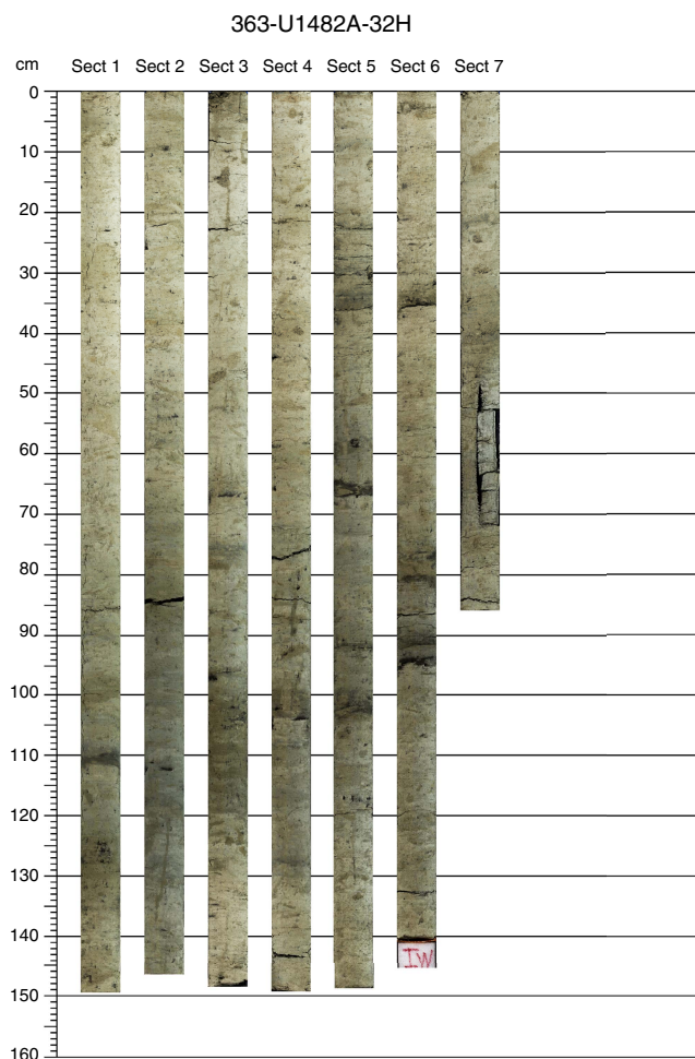
Figure F8. Characteristic lithology and strong color alternations in Subunit IC, Hole U1482A.
