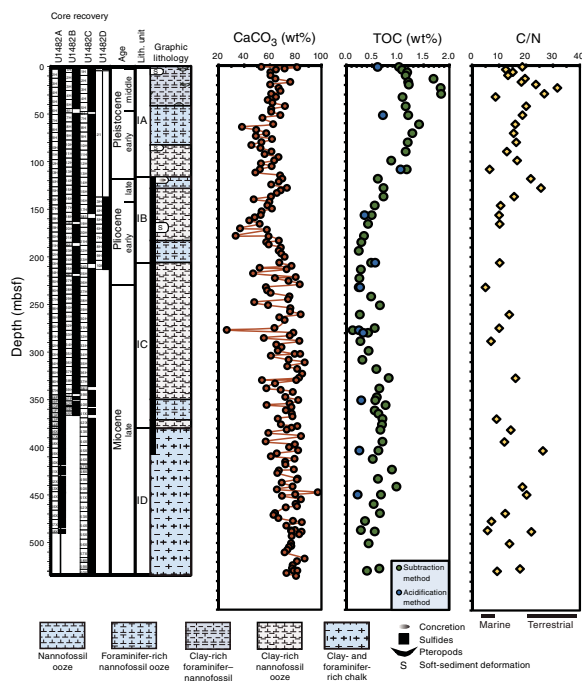
Figure F43. Calcium carbonate, TOC, and C/N profiles, Site U1482. Ranges of marine and terrestrial organic matter based on C/N are indicated by annotated bars at the base of the C/N profile.
