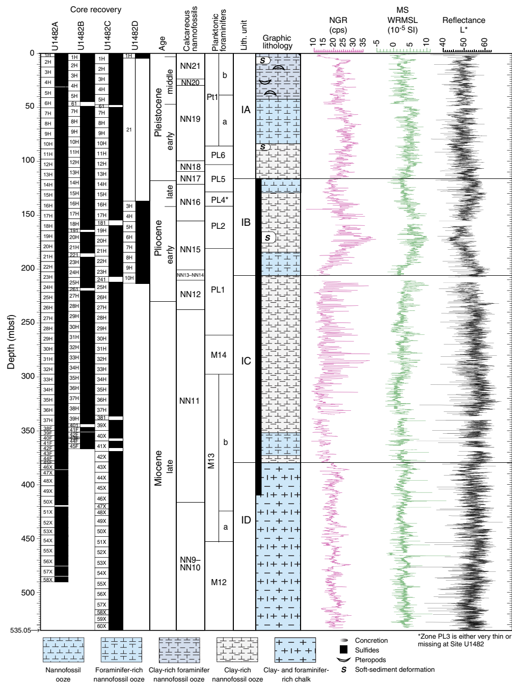
Figure F5. Lithologic summary, Site U1482. cps = counts per second. Magnetic stratigraphy is not shown because early sediment diagenesis compromised the paleomagnetic record deeper than ~50–70 mbsf.
