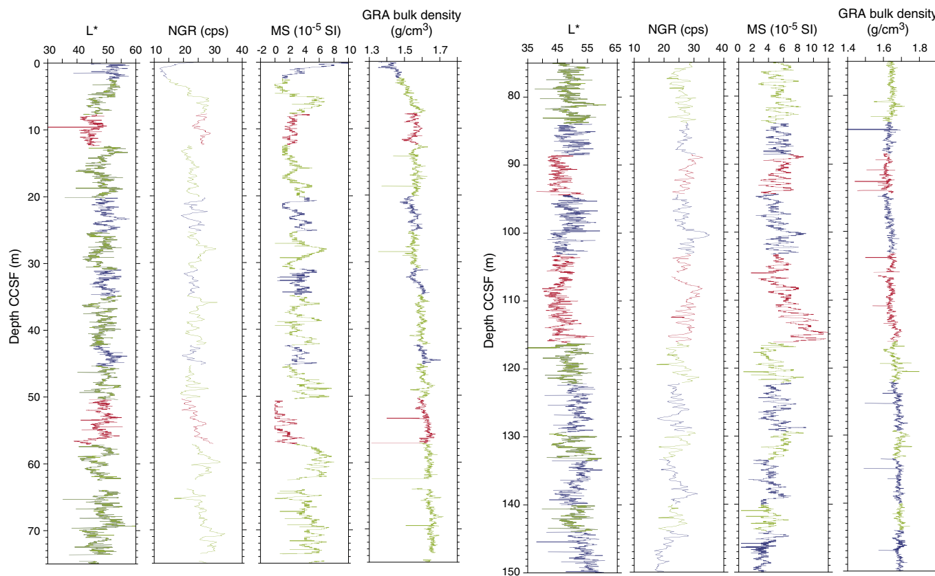
Figure F39. Spliced composite L*, NGR, and WRMSL MS and GRA bulk density data for Holes U1482A (red), U1482B (blue), U1482C (green), and U1482D (lavender). cps = counts per second. (Continued on next page.)
