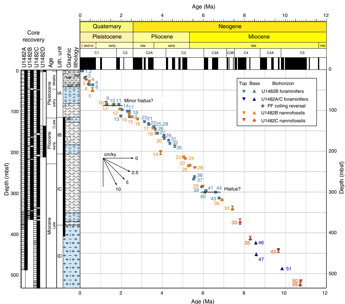
Figure F22. Age-depth plot for calcareous nannofossil and planktonic foraminifer (PF) biohorizons, Site U1482. Average sedimentation rates are ~5.9 cm/ky during the late Miocene, ~3.3 cm/ky in the early Pliocene, and ~7 cm/ky in the Pleistocene. Vertical error bars represent the interval between the two samples that defines the biohorizon (often obscured by the biohorizon symbol). Biohorizon numbers correspond to those in Tables T2 and T3.
