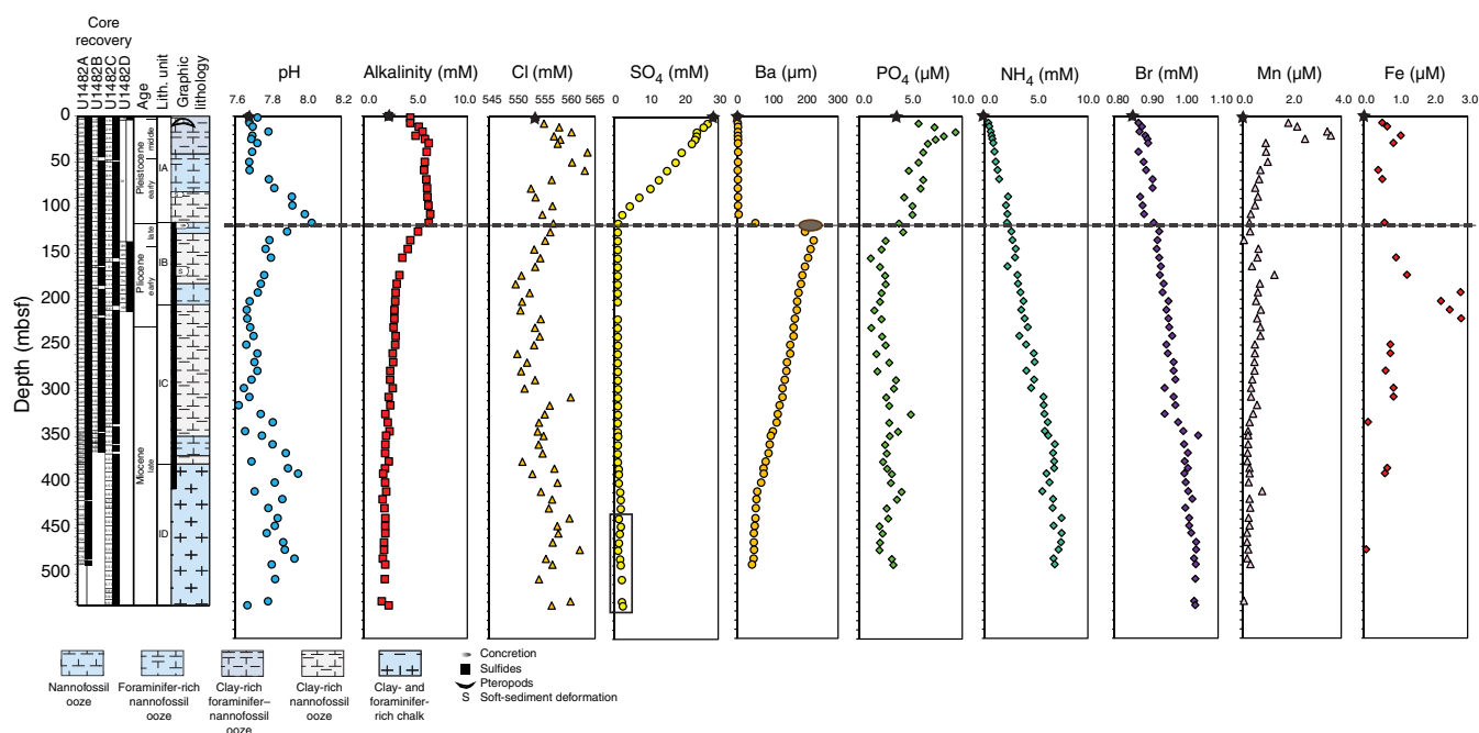
Figure F44. Interstitial water concentration profiles, Holes U1482A and U1482C. Mudline Fe and Mn concentrations were below detection limit and are not plotted. \text{SO}_4 concentration above the background deeper than 344 mbsf (rectangle) correlates with the onset of HLAPC and XCB coring and may reflect small amounts of seawater contamination. Black stars = mudline samples, dashed line = SMTZ, brown ellipse = calcite-barite concretion.
