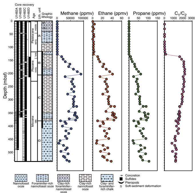
Figure F42. Methane, ethane, propane, and C_1/C_2 profiles, Holes U1482A and U1482C.
