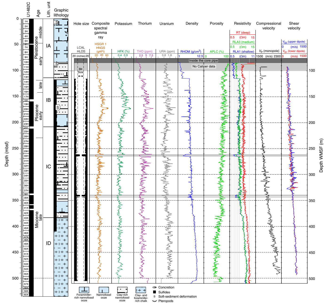
Figure F46. Logging summary, Hole U1482C. Small depth discrepancies may exist between the mbsf and WMSF depth scales (usually <2 m).
