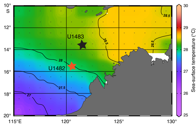
Figure F4. Mean annual SST off Northwest Australia illustrating the steep north-south SST gradient in the region (ODV World Ocean Atlas, 2013; https://odv.awi.de/de/data/ocean/world_ocean_atlas_2013/ ).
