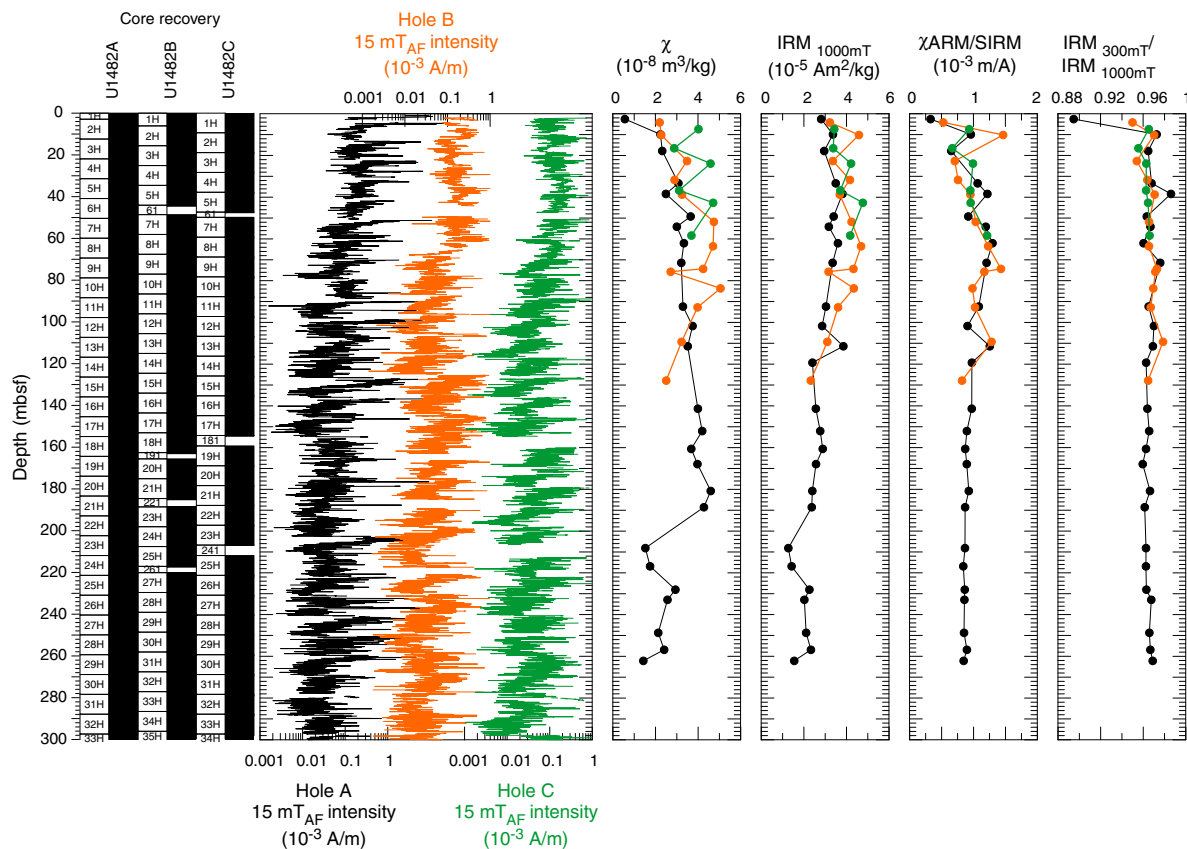
Figure F23. Archive-half section NRM intensity after 15 mT AF demagnetization, discrete sample \chi and SIRM, and discrete sample \chi_{\text{ARM}}/\text{SIRM} and \text{IRM}_{300\text{mT}}/\text{IRM}_{1000\text{mT}} ratios, Holes U1482A–U1482C. Black = Hole U1482A, orange = Hole U1482B, green = Hole U1482C.
