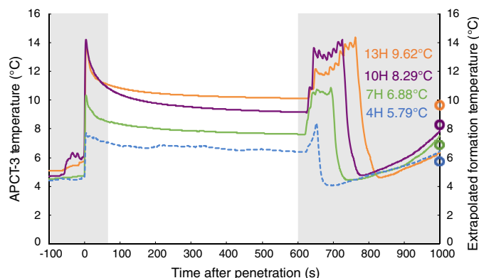
Figure F34. APCT-3 temperature-time series, Hole U1482A. Unshaded area = time interval with exponential decrease in temperature. Dashed blue line = measurement taken during coring of Core 4H, not used for the heat flow calculation.
