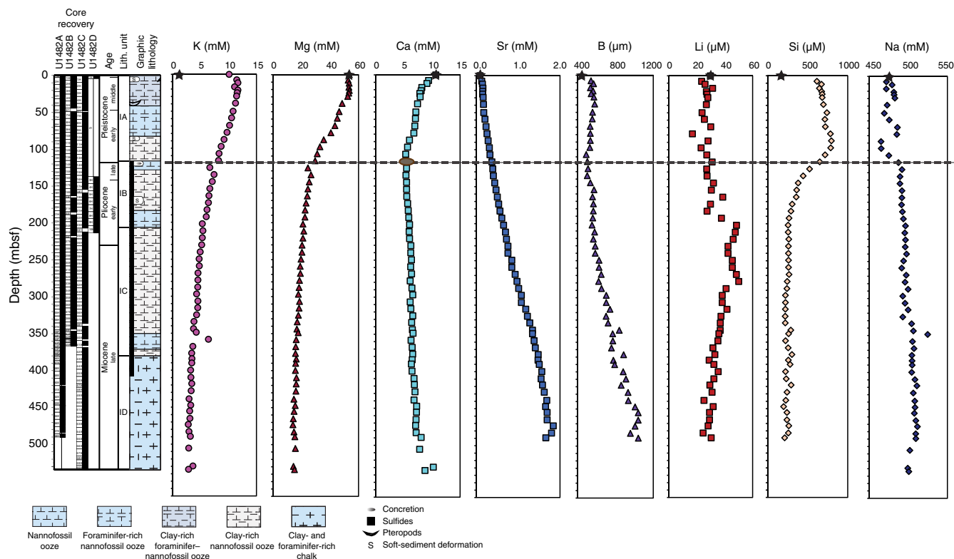
Figure F45. Interstitial water concentration profiles, Holes U1482A and U1482C. Black stars = mudline samples, dashed line = SMTZ, brown ellipse = calcite-barite concretion.
