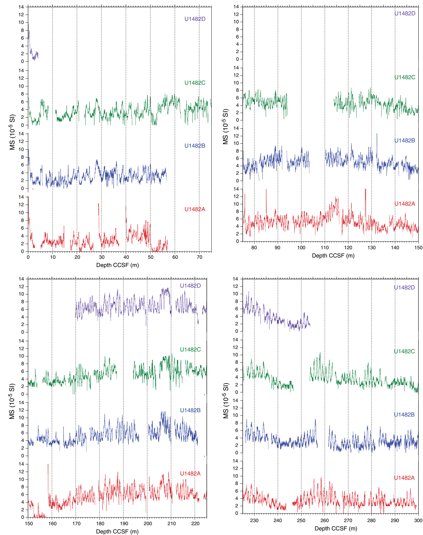
Figure F37. WRMSL magnetic susceptibility (MS) data, Holes U1482A–U1482D. (Continued on next two pages.)
