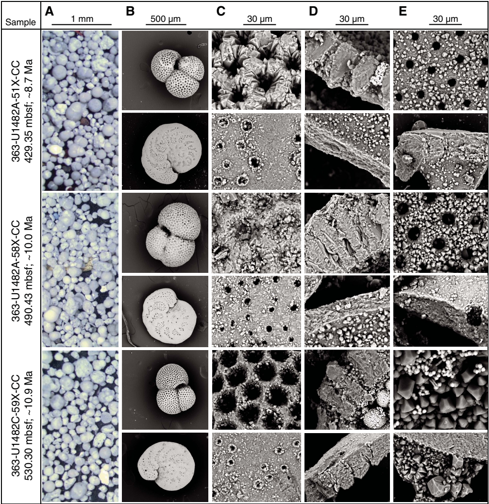
Figure F21 (continued). Images of foraminifer test preservation states, Site U1482. A. Light microscope: extent of fragmentation and staining and whether the tests are glassy or opaque. B. SEM: T. trilobus and P. wuellerstorfi as whole tests, umbilical side upward. C–E. High-magnification; (C) outer wall surfaces showing features such as spine holes, pustules, etc.; (D) wall cross sections to find original microgranules or diagenetic crystallites; (E) inner wall surfaces, focusing on evidence for internal overgrowth and cementation.
