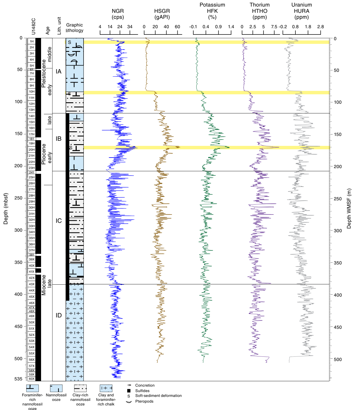
Figure F47. Natural gamma radiation, Hole U1482C. Small depth discrepancies may exist between the mbsf and WMSF depth scales (usually <2 m). Yellow shading = deformed sediment intervals (see Core description), cps = counts per second.
