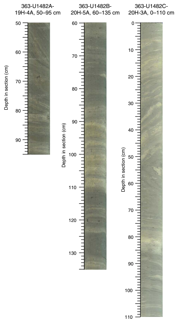
Figure F12. Soft-sediment deformation in Subunit IB, Site U1482.
