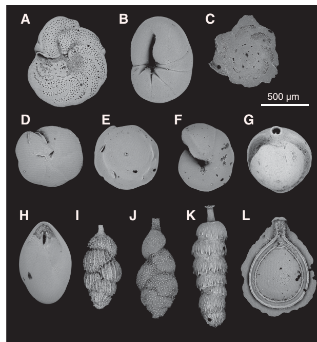
Figure F20. Benthic foraminifers, Hole U1482A. A. Planulina wuellerstorfi (1H-CC). B. Ceratobulimina jonesiana (1H-CC). C. Osangularia bengalensis (11H-CC). D. Oridorsalis umbonatus , ventral (6H-CC). E. Oridorsalis umbonatus , dorsal (6H-CC). F. Gyroidinoides soldanii (7H-CC). G. Pyrgo lucernula (15H-CC). H. Pleurostomella brevis (7H-CC). I. Uvigerina peregrina (7H-CC). J. Uvigerina auberiana (7H-CC). K. Rectuvigerina multicostata (15H-CC). L. Fissurina lacunata (13H-CC).
