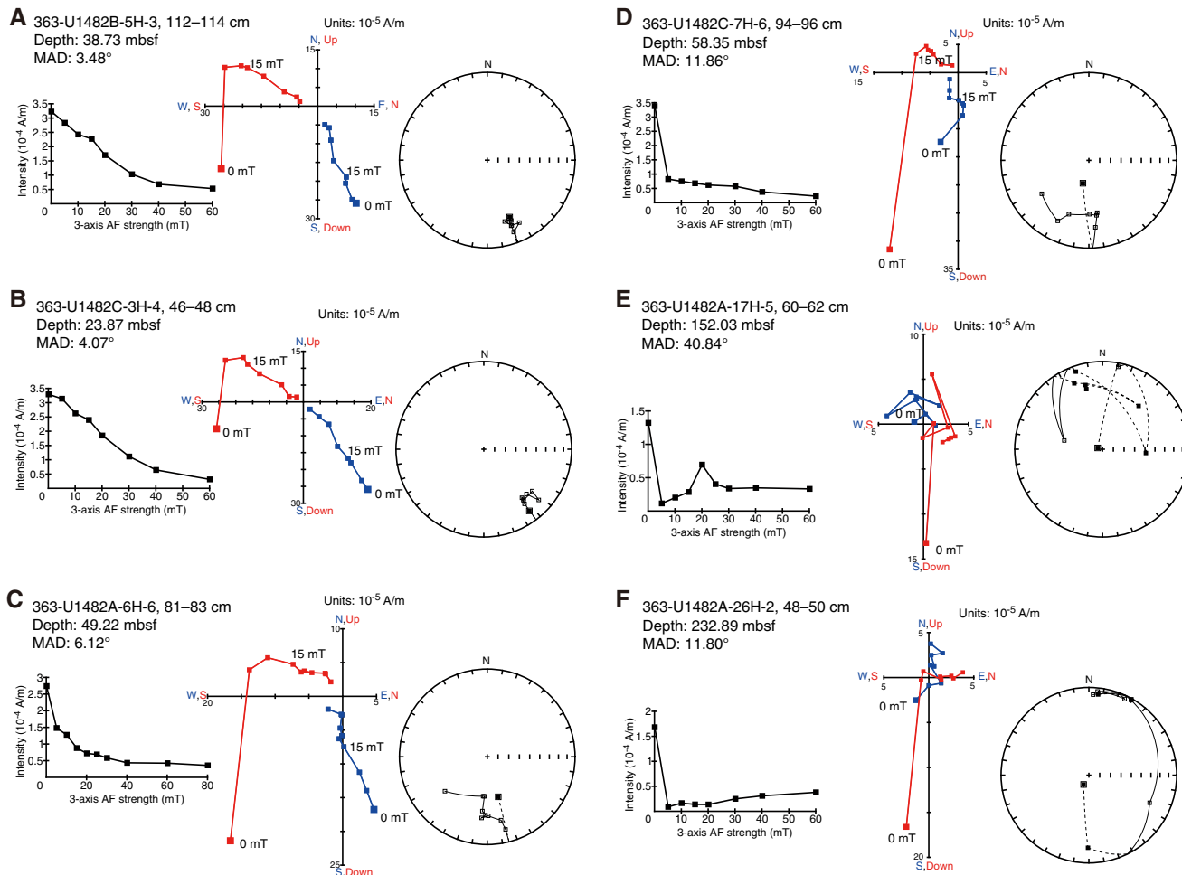
Figure F25. A–F. Discrete sample AF demagnetization results, Site U1482. Left plots: intensity variation through progressive AF demagnetization steps. Middle and right plots: NRM vector measurements after each AF demagnetization treatment on orthogonal (Zijderveld; blue = horizontal projections, red = vertical projections) and stereographic (solid squares = positive inclination, open squares negative inclination) projections, respectively. MAD = maximum angular deviation.
