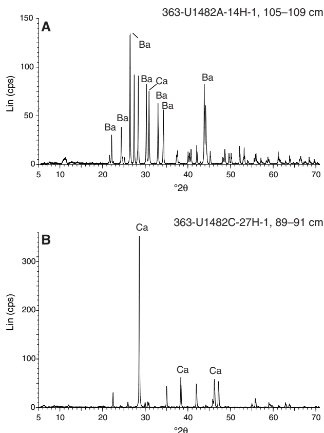
Figure F14. XRD results, Site U1482. A. Concretion composed of barite and calcite. B. Light layer with dominant calcite. Ba = barite, Ca = calcite.
