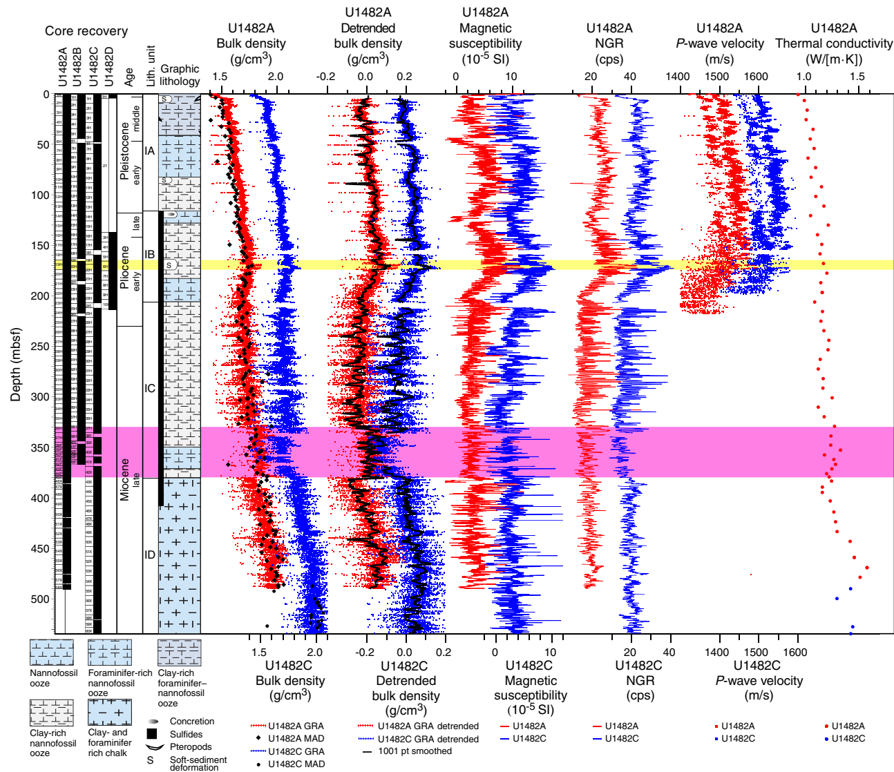
Figure F28. Representative physical property measurements, Holes U1482A and U1482C (WRMSL GRA, MS, and PWL). cps = counts per second. Yellow shading = interval of soft-sediment deformation observed in all holes, pink shading = interval where data are affected by the coring process.
