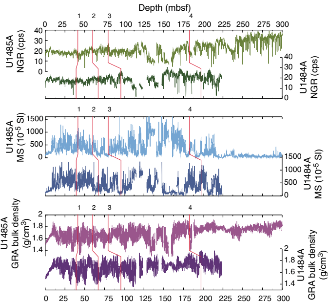
Figure F22. Comparison of major physical property parameters (WRMSL and NGRL), Sites U1484 and U1485. Calcareous nannofossil and planktonic foraminifer biohorizons identified at both sites (red lines): 1 = top Globorotalia flexuosa (0.07 Ma), 2 = base common Emiliania huxleyi (0.09 Ma), 3 = top Globigerinoides ruber (pink) (0.12 Ma), 4 = base Emiliania huxleyi (0.29 Ma).
