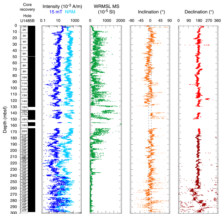
Figure F18. NRM intensities before and after 15 mT AF demagnetization, WRMSL MS, and inclination (dashed lines = predicted values assuming a GAD field for normal ( -5.7^\circ ) and reversed ( 5.7^\circ ) polarity for the site latitude), and declination (red = azimuthally corrected values for APC cores, dark red = manually rotated values for HLAPC cores) after 15 mT AF demagnetization, Hole U1485B.
