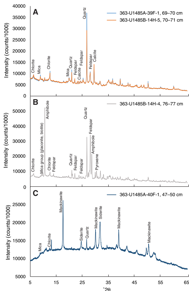
Figure F9. XRD results, Site U1485. A. Nannofossil-rich clay. B. Pumice. C. Iron carbonate concretion.
