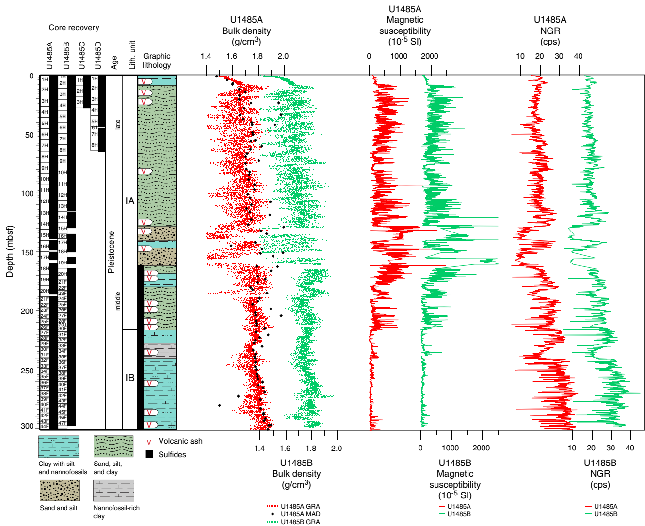
Figure F20. Physical property measurements, Holes U1485A and U1485B. GRA bulk density and magnetic susceptibility data were measured on the WRSMSL. Detrended GRA bulk density data are not included because they show comparable trends. WRSMSL P -wave data are shown in Figures F21 and F23. cps = counts per second.
