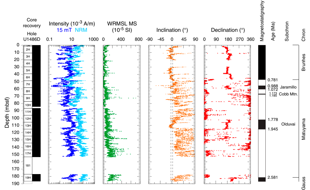
Figure F23. NRM intensities before and after 15 mT AF demagnetization, WRMSL MS, and inclination (dashed lines = predicted values assuming a GAD field for normal (−3°) and reversed (3°) polarity for the site latitude) and azimuthally corrected declination after 15 mT AF demagnetization, Hole U1486D. Magnetostratigraphy and GPTS shown at right. Black = normal polarity, white = reversed polarity.
