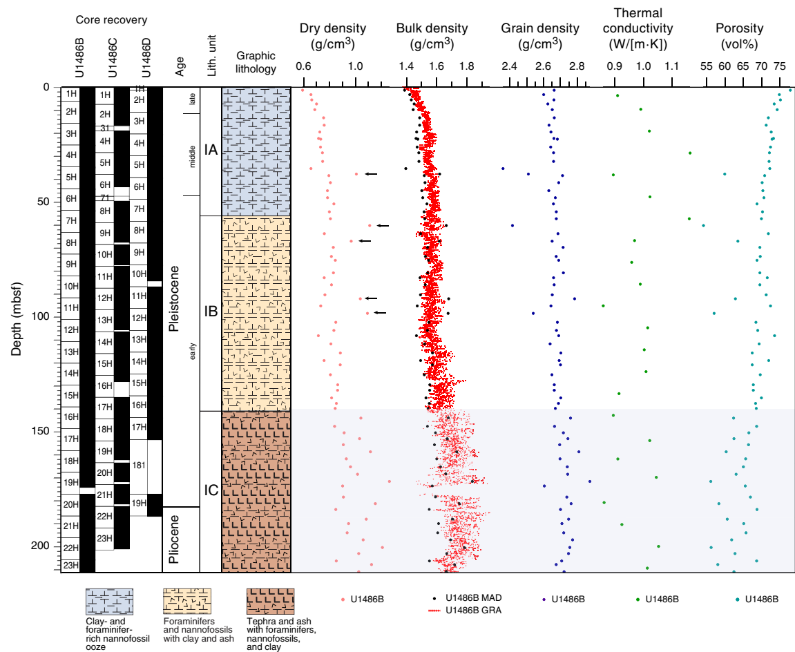
Figure F28. MAD discrete sample dry, bulk, and grain densities and porosity, WRMSL GRA bulk density, and thermal conductivity, Hole U1486B. Arrows = outliers in dry density measured on samples from volcanogenic-rich layers. Outliers are propagated through MAD calculations and are evident in other MAD properties, although they are not explicitly marked. Shading highlights Subunit IC, which shows increased variability in density and porosity measurements.
