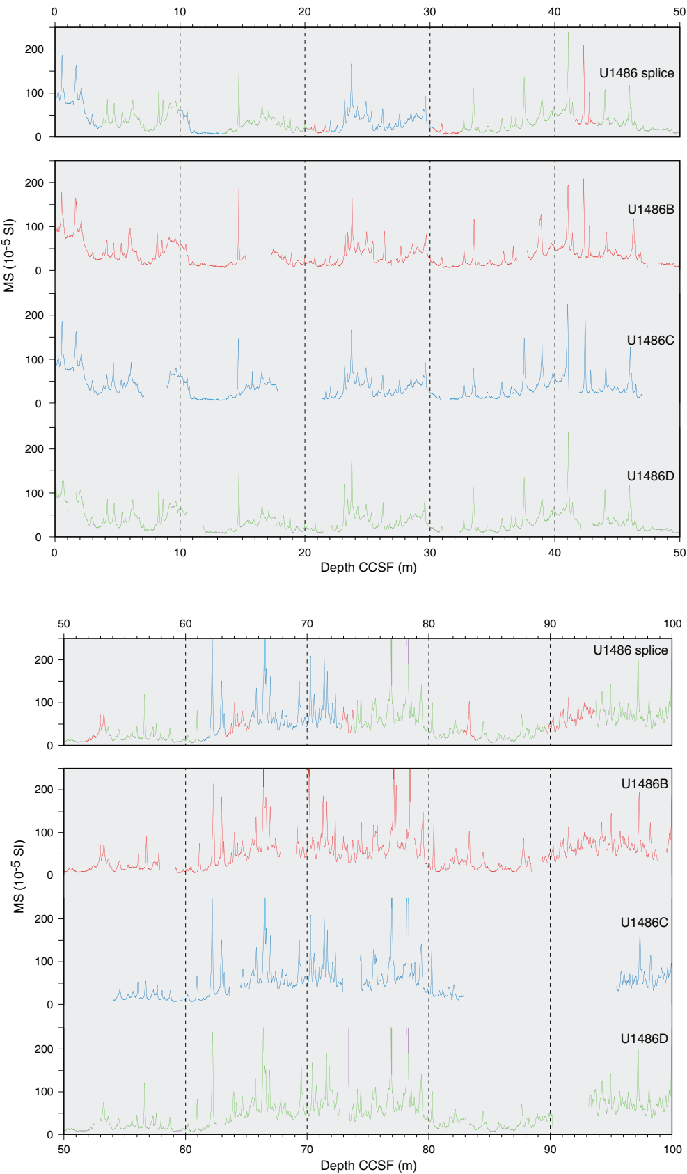
Figure F31. WRMSL MS data for Holes U1486B–U1486D divided into 50 m intervals. Upper panel shows the MS splice constructed by combining data from all holes. (Continued on next two pages.)
