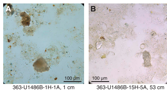
Figure F8. Main lithologies, Site U1486. A. Mainly biogenic sediment (Subunit 1A). B. Alternating dark–light biogenic and volcanogenic sediment (Subunit 1B). C. Dominantly volcanogenic sediment (Subunit 1C).
