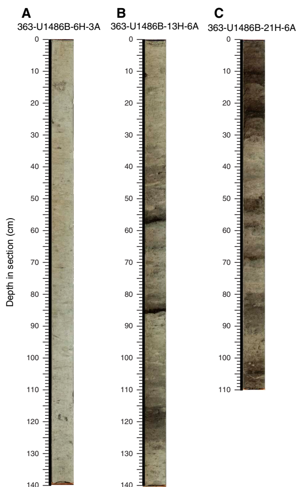
Figure F8. Main lithologies, Site U1486. A. Mainly biogenic sediment (Subunit 1A). B. Alternating dark–light biogenic and volcanogenic sediment (Subunit 1B). C. Dominantly volcanogenic sediment (Subunit 1C).
