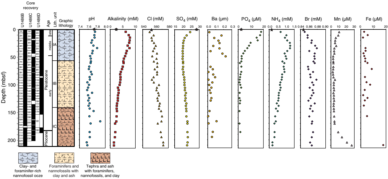
Figure F36. Interstitial water concentration profiles, Hole U1486B. Black stars = mudline samples. Fe, Mn, and Ba mudline concentrations were below detection limit and are not plotted.
