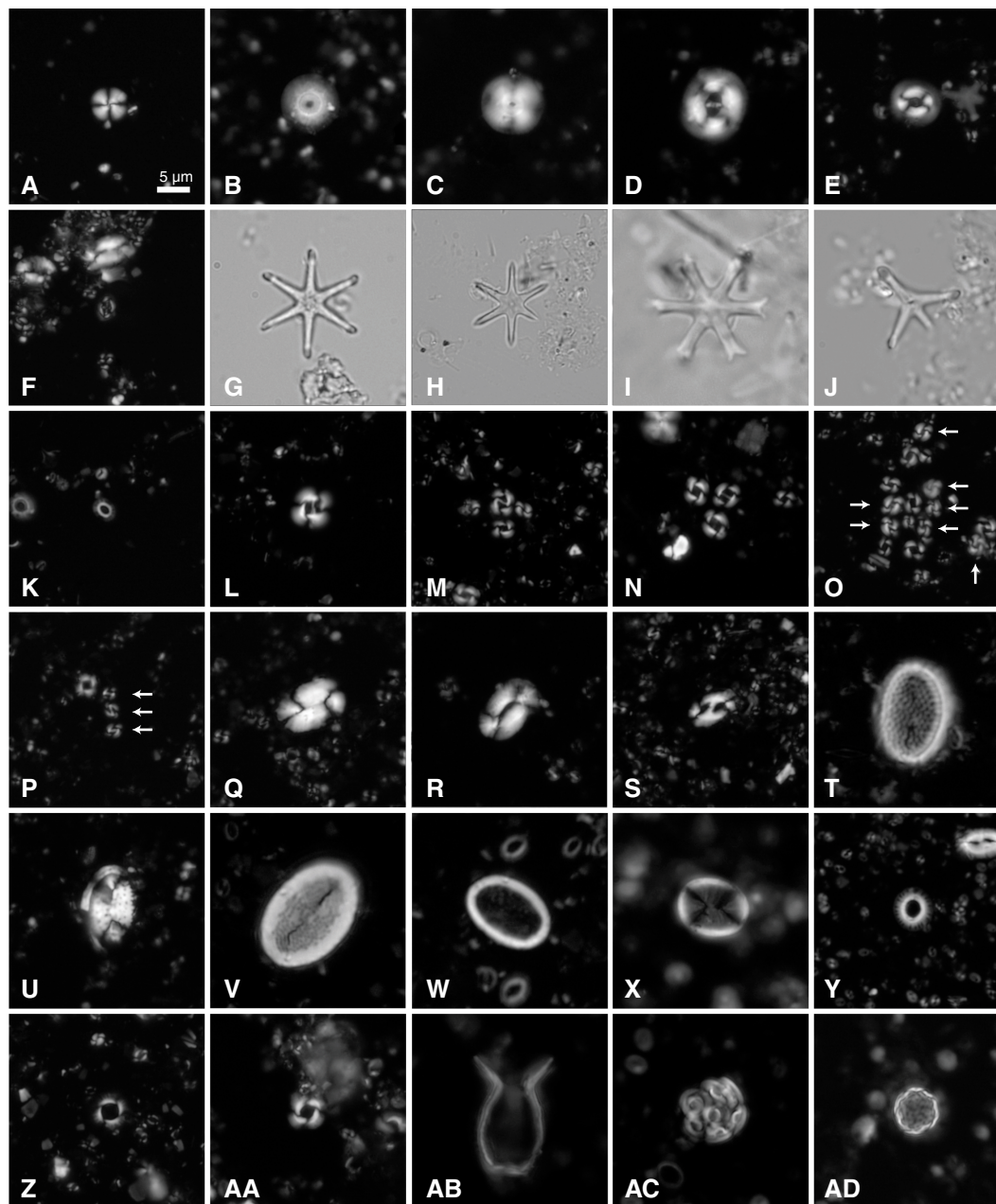
Figure F15. Calcareous nannofossils, Hole U1486B. A. Calcidiscus leptoporus (12H-CC). B, C. Calcidiscus macintyreii ; (B) 12H-CC; (C) 19H-CC. D, E. Coccolithus pelagicus (15H-CC). F. Cruciplacolithus neohelis (15H-CC). G, H. Discoaster brouweri (22H-6, 81 cm). I. Discoaster surculus (20H-6, 85 cm). J. Discoaster sp. (22H-6, 81 cm). K. Emiliana huxleyi (1H-CC). L. Gephyrocapsa sp. >5.5 \mu m (8H-CC). M. Gephyrocapsa oceanica and Gephyrocapsa caribbeanica (4H-CC). N. Gephyrocapsa oceanica (2H-CC). O. G. caribbeanica (arrows) (4H-3, 50 cm). P. Small Gephyrocapsa sp. (arrows) (10H-CC). Q. Helicosphaera carteri (10H-CC). R. Helicosphaera princei (9H-CC). S. Helicosphaera sellii (10H-CC). T, U. Pontosphaera spp.; (T) 5H-CC; (U) 20H-CC. V. Pontosphaera japonica (1H-CC). W. Pontosphaera discopora (1H-CC). X. Pontosphaera cf. P. alta (12H-CC). Y, Z. Pseudoemiliana lacunosa ; (Y) 8H-3, 130 cm; (Z) 7H-4, 120 cm. AA. Reticulofenestra asanoi (10H-6, 100 cm). AB. Scyphosphaera pulcherrima (13H-CC). AC. Umbilicosphaera sibogae coccosphere (1H-CC). AD. Coccosphere (19H-CC). A, C–F, L–U, X, Z, AA, and AB: XPL; B, K, V, W, Y, AC, and AD: CPL; G–J: PPL. All photos are at same magnification (scale bar in A).
