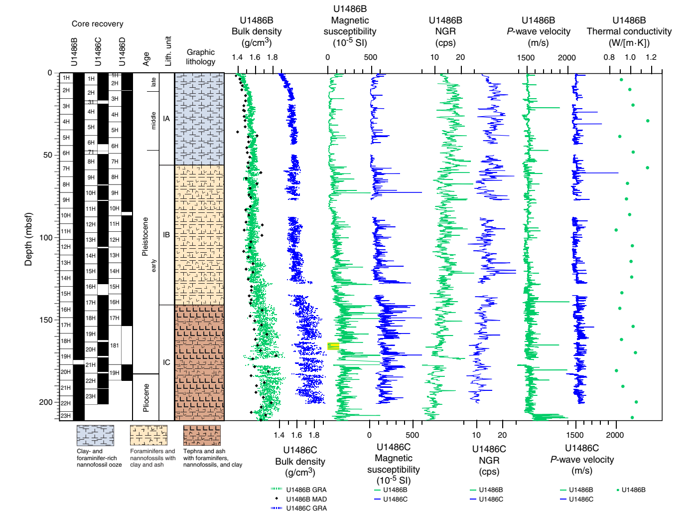
Figure F24. Physical property measurements, Holes U1486B and U1486C. GRA bulk density, magnetic susceptibility and P -wave data were measured on the WRMSL. Yellow shading in Hole U1486B magnetic susceptibility marks sections affected by instrumental offset. cps = counts per second.
