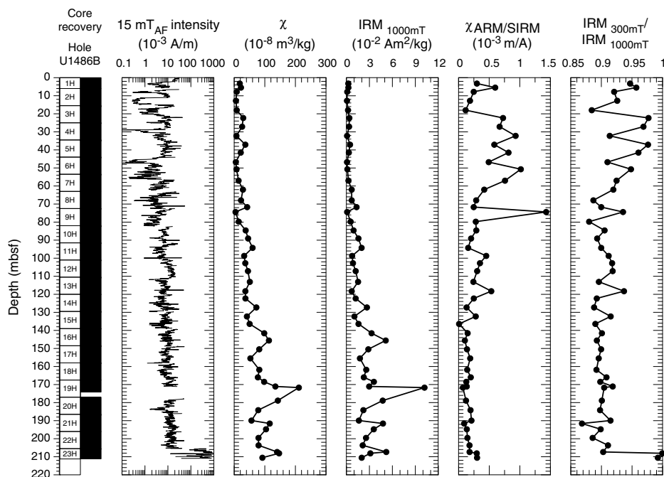
Figure F19. Archive-half NRM intensity after 15 mT AF demagnetization, discrete sample \chi and IRM, and discrete sample \chi_{\text{ARM}} /SIRM and IRM 300mT /IRM 1000mT ratios, Hole U1486B.
