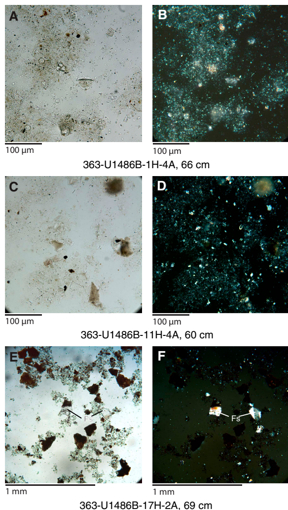
Figure F6. Main sedimentary components, Site U1486. A, B. Foraminifer- and clay-rich nannofossil ooze (Subunit 1A). C, D. Foraminifer-rich ashy nannofossil ooze (Subunit 1B). E, F. Silt- and sand-sized volcanogenic particles and feldspars (Fs) (Subunit 1C). A, C, and E: plane-polarized light (PPL); B, D, and F: cross-polarized light (XPL).
