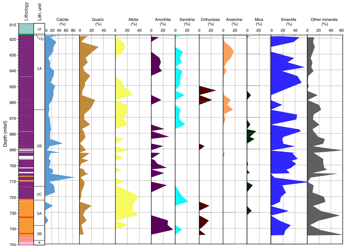
Figure F21. Bulk mineralogy, Cores 364-M0077A-40R through 95R (617.33–747.02 mbsf). Other minerals = those occurring at &lt;15%.
