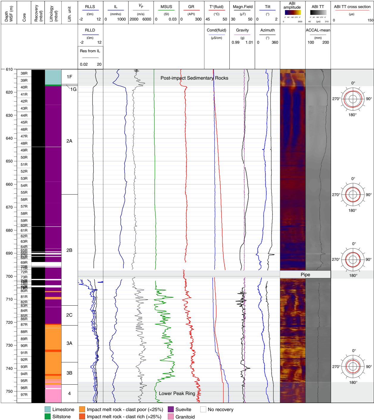
Figure F24. Wireline downhole log data, Hole M0077A. RLLS = shallow-reading resistivity, RLLD = deep-reading resistivity, Res from IL = resistivity from induction, IL = conductivity, V_p = P -wave velocity, MSUS = magnetic susceptibility, GR = total gamma ray, T^\circ(\text{fluid}) = borehole fluid temperature, Cond(fluid) = borehole fluid conductivity, Magn.Field = local magnetic field, ABI TT = travelttime acoustic image, ACCAL-mean = mean borehole diameter, ABI TT cross section = travelttime cross section of the borehole. See Downhole logging in the Expedition 364 methods chapter (Gulick et al., 2017a) for tool descriptions.
