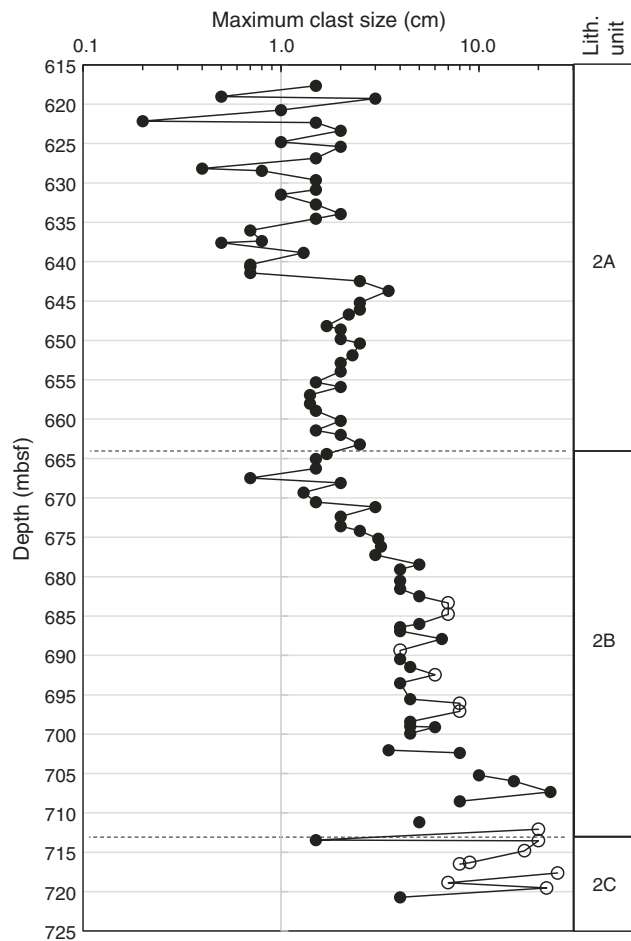
Figure F3. Maximum clast size for Unit 2, Hole M0077A. Depth information for maximum clasts was not described during visual core description, so the top depth of each section is used on the vertical axis. Open circles indicate a minimum value because the clast was truncated during drilling.
