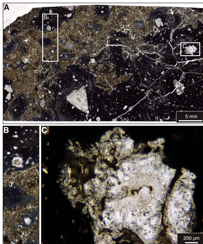
Figure F8. Impact melt rock sample from Subunit 3A, Hole M0077A. A. Inter-mix of green and black impact melt rocks with angular to subrounded clasts (89R-3, 39–43 cm). B. Microcrystalline black melt rock and green domains of smectite. C. Melted silica clast in black melt rock (PPL).
