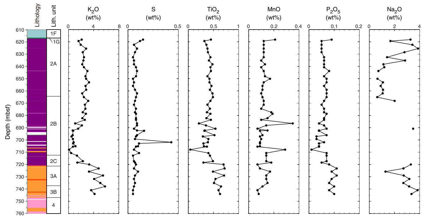
Figure F18. Minor element compositions, Cores 364-M0077A-40R through 95R (617.33–747.02 mbsf).
