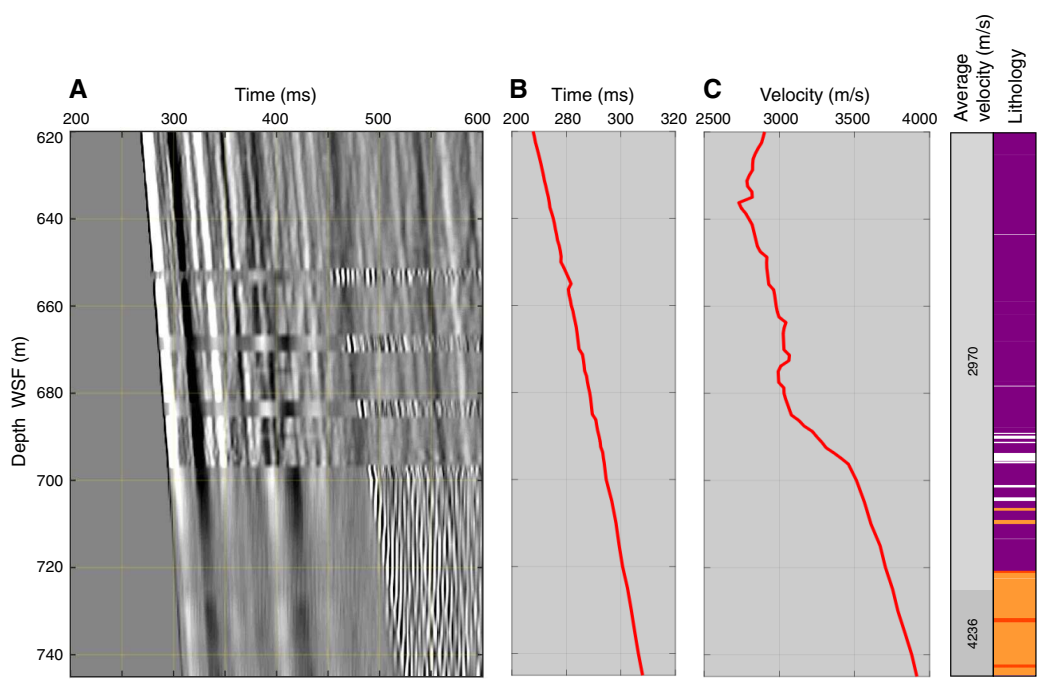
Figure F27. VSP, Hole M0077A. A. Vertical component data recorded on receiver depths between 620.0 and 745.0 m WSF. Noisy traces were removed. Data are stacked and plotted with an automatic gain control. A top mute was applied to remove noise prior to the first breaks. B. One-way traveltimes for the first-break picks. C. Differential P -wave velocity.
