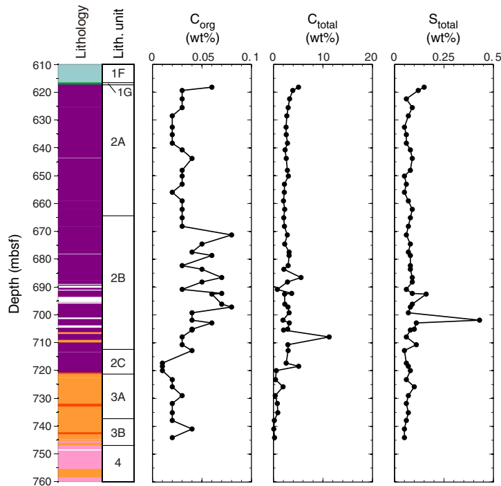
Figure F20. Carbon and sulfur contents, Cores 364-M0077A-40R through 95R (617.33–747.02 mbsf).
