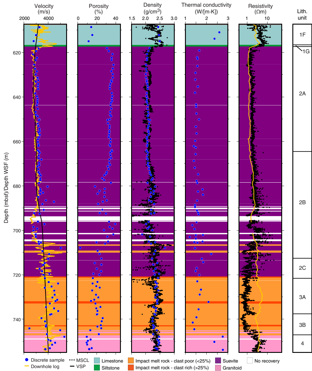
Figure F22. P -wave velocity, porosity, density, thermal conductivity, and resistivity from discrete core sample and downhole measurements, Hole M0077A. mbsf = discrete samples and MSCL data, WSF = downhole logs. Yellow curves = downhole measurements of sonic velocity and resistivity (converted from conductivity).
