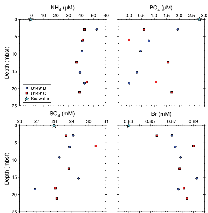
Figure F22. Interstitial water ammonium, phosphate, bromide, and sulfate concentrations, Site U1491. Bottom seawater values are from Mottl et al. (2003, 2004).
