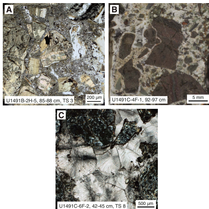
Figure F11. Carbonate breccia. A. Fine-grained carbonate matrix of breccia (white to mottled medium gray) embedded with small fibrous serpentine or bastite fragments (366-U1491B-2H-5, 85–88 cm; plane-polarized light [PPL]). B. Subangular to angular serpentinized harzburgite and serpentine clasts (dark) hosted by a carbonate matrix (white) (366-U1491C-4F-1, 92–97 cm). C. Carbonate breccia characterized by matrix of aragonite (white radiating clusters) and angular serpentinite (dark) clasts (Sample U1491C-6F-2, 42–45 cm; XPL).
