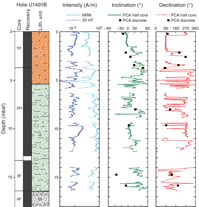
Figure F32. NRM intensity, inclination, and declination, Hole U1491B. Declination and inclination values are based on PCA fitting of the series of AF demagnetization declination and inclination data.
