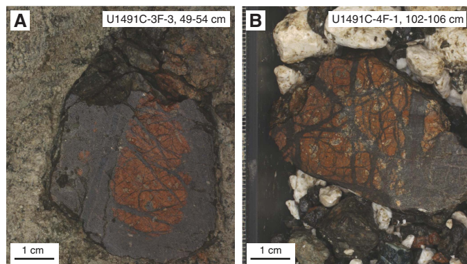
Figure F16. Serpentinized harzburgite clasts, Hole U1491C. A. Clast, which contains relict orthopyroxene and clinopyroxene, interpreted to be a highly altered, dark reddish brown harzburgite clast with crosscutting black serpentine veins. It is embedded in soft serpentinite mud (3F-3, 49–54 cm). B. Highly altered dark reddish brown harzburgite similar to A in a graded sequence of drilling-disturbed polymict gravel interval composed of smaller granule- to gravel-sized similar dark reddish brown harzburgite, white sub-rounded carbonate, and dark gray to black harzburgite (4F-1, 102–106 cm).
