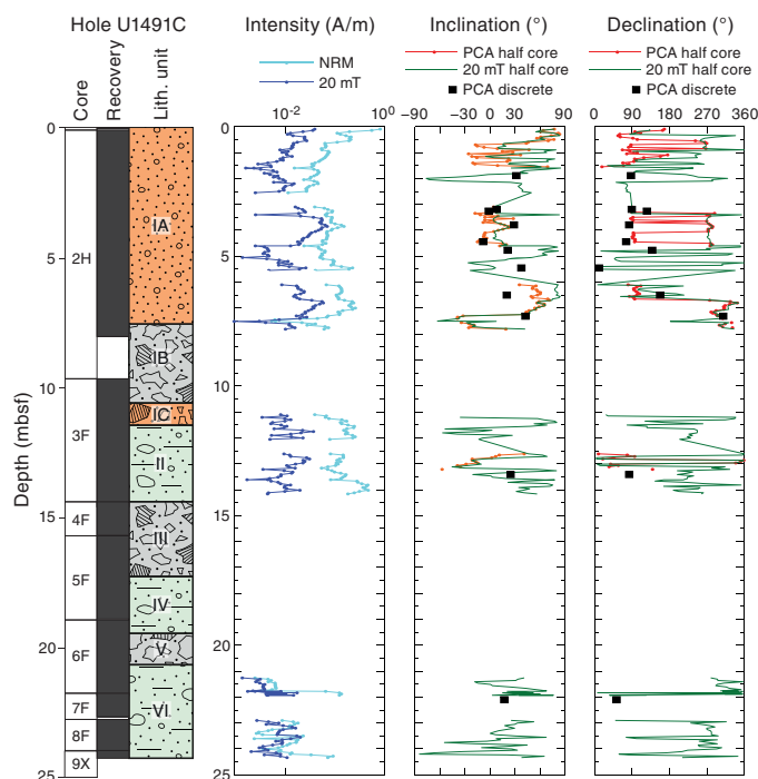
Figure F33. NRM intensity, inclination, and declination, Hole U1491C. Declination and inclination values are based on PCA fitting of the series of AF demagnetization declination and inclination data.
