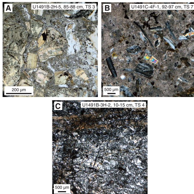
Figure F17. Microstructures of serpentinite breccias. A. Ultramafic breccia with carbonate matrix (366-U1491B-2H-5, 85–88 cm). B. Matrix of clast in Figure F11B showing small serpentinite fragments (elongate dark gray and light gray, low-order birefringence colors) embedded in micritic carbonate matrix (mottled medium-gray birefringence color) (366-U1491C-4F-1, 92–97 cm; XPL). C. Massive serpentinized harzburgite crosscut by veins of brownish and fibrous serpentine associated with carbonate and magnetite (366-U1491B-3H-2, 10–15 cm; XPL).
