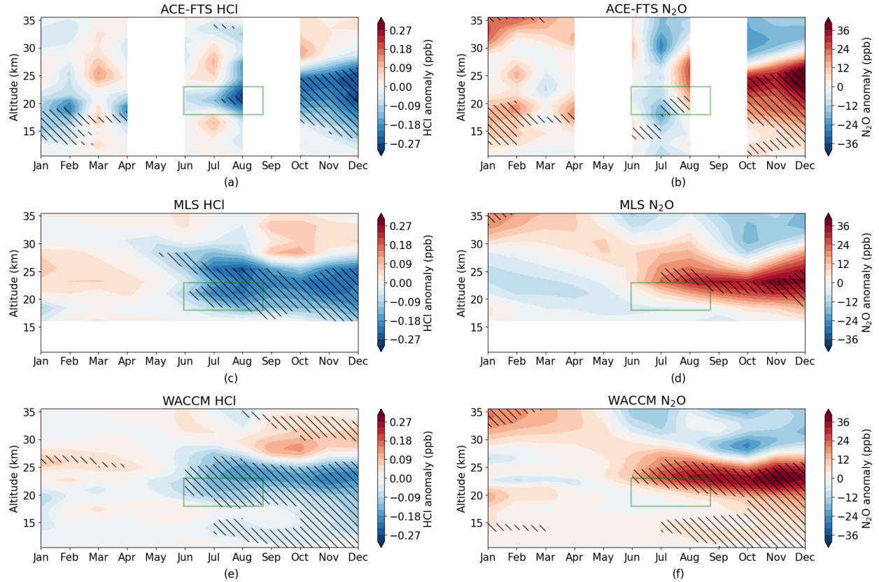
Figure 1. Calculated 2022 HCl anomaly in ppbv (panel a,c,e) and N 2 O anomaly in ppbv (panel b,d,f) relative to climatology (2007 to 2019) from ACE-FTS, MLS, and WACCM in the SH mid-latitudes (30-55°S). Hatched regions indicate where the 2022 anomalies are outside the range of all variability during 2007-2019.
