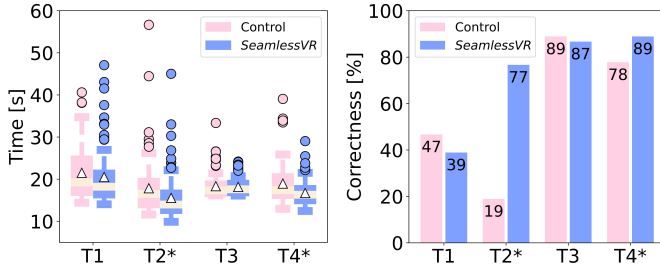
Fig. 6: Task completion times (left) and correctness (right) across tasks and conditions.
