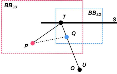
Fig. 2: Transition initialization and morphing. The 3D bounding box of the scene is translated and scaled from BB_{3D} to BB_{2D} , and, at the same time, BB_{2D} is morphed to the 2D screen S . A scene vertex P corresponds to a BB_{2D} point Q , which is used to define the final screen position T along the 2D visualization ray OQ . P is then gradually displaced to T . O is defined as the user's head position U when the transition is initiated.
