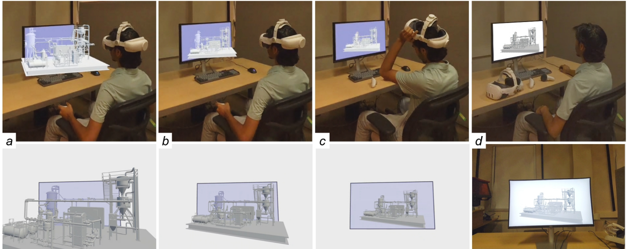
Fig. 1: SeamlessVR transition from immersive visualization in the headset (left) to non-immersive visualization on screen (right): illustration frames acquired with an XR headset in passthrough mode (top row), and actual frames seen by the user in the headset (bottom row). Once the user engages the transition (a), the 3D visualization morphs to a 2D visualization (a to b to c) that matches what the user sees once they remove the headset (c to d).
