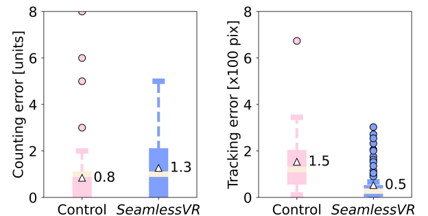
Fig. 7: Counting error magnitude for T1 (left) and target tracking error magnitude for T2 (right), for each of the two conditions.
