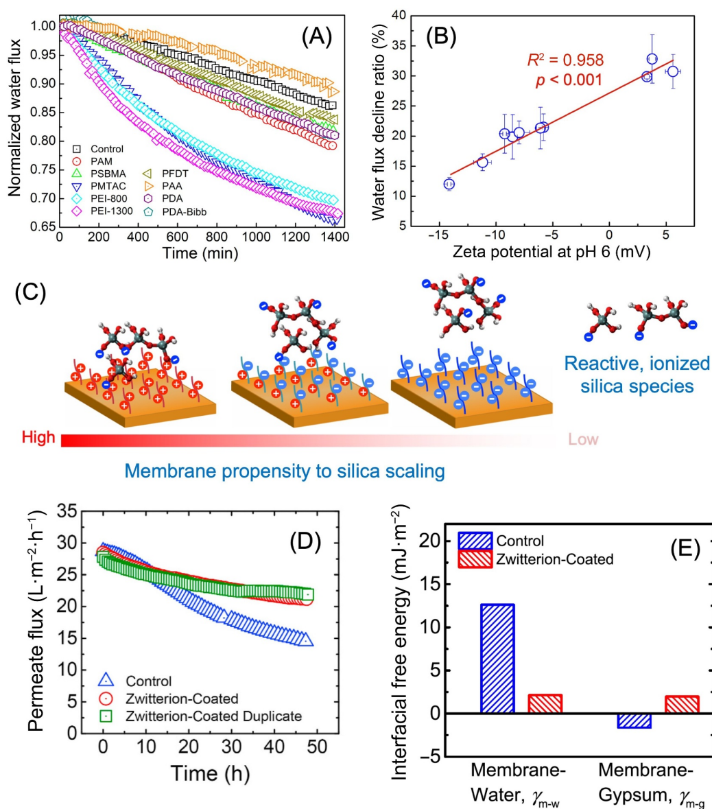
Fig. 5 (A) Water flux curve of RO desalinating feedwater containing supersaturated silica using membranes of different surface properties. (B) The water flux decline ratio of membranes shown in Fig. 5(A) demonstrates a strong correlation with surface charge, manifested by zeta potential, of the membranes. (C) Mechanisms underlying the relationship between membrane surface charge and propensity of silica scaling. (D) Water flux curve of RO desalinating feedwater containing supersaturated gypsum using a pristine polyamide membrane and membranes coated with zwitterionic polymer. (E) The membrane-water and membrane-gypsum interfacial free energies for the pristine polyamide and zwitterion-coated membranes. The figures are adapted with permission from Tong et al. (2017), copyright American Chemical Society; Jaramillo et al. (2021), copyright Elsevier.
