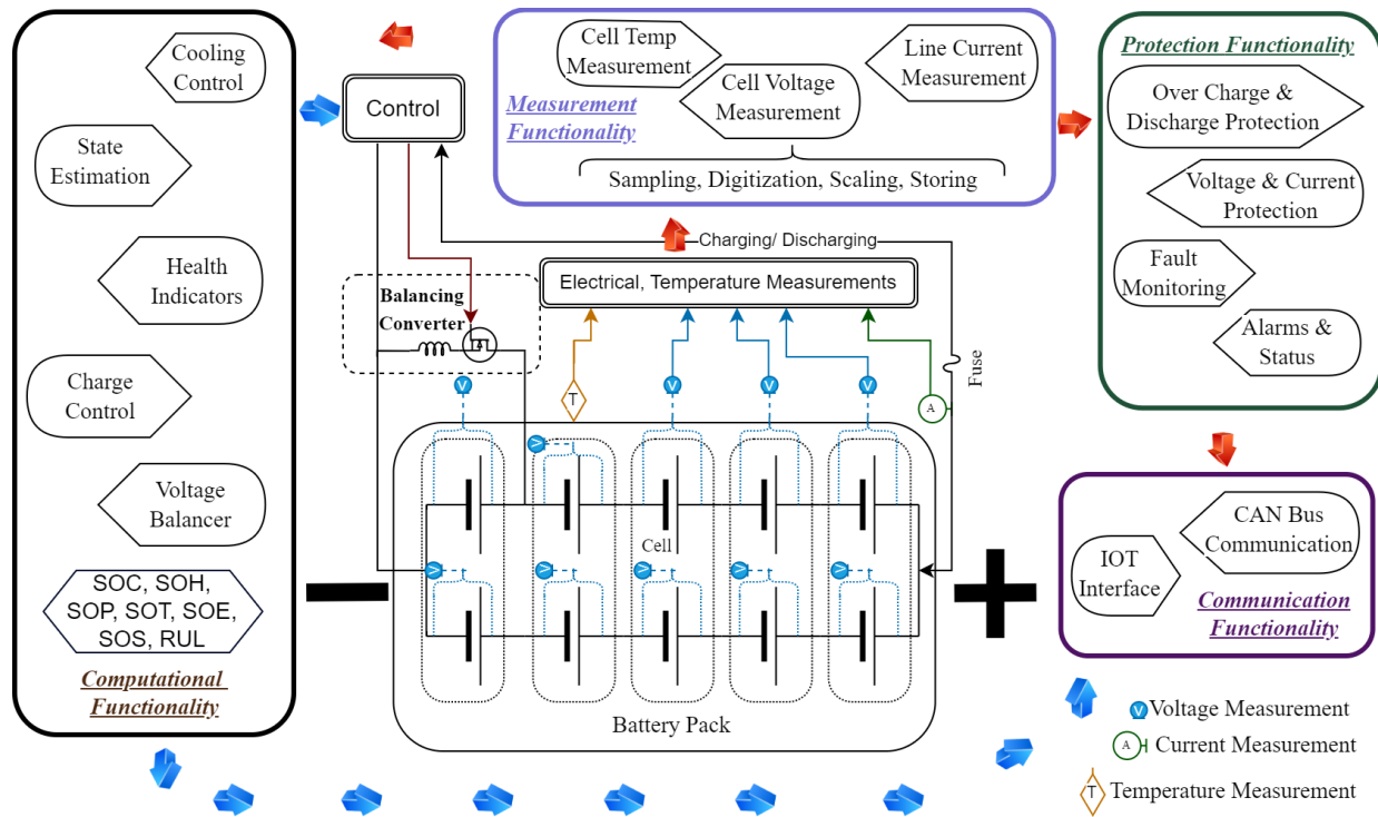
Figure 3. Battery management system (BMS).
