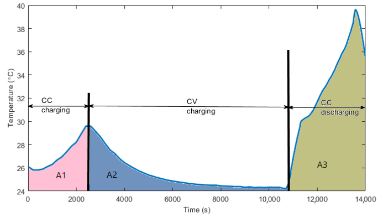
Figure 8. Temperature-integral-based HIs.
