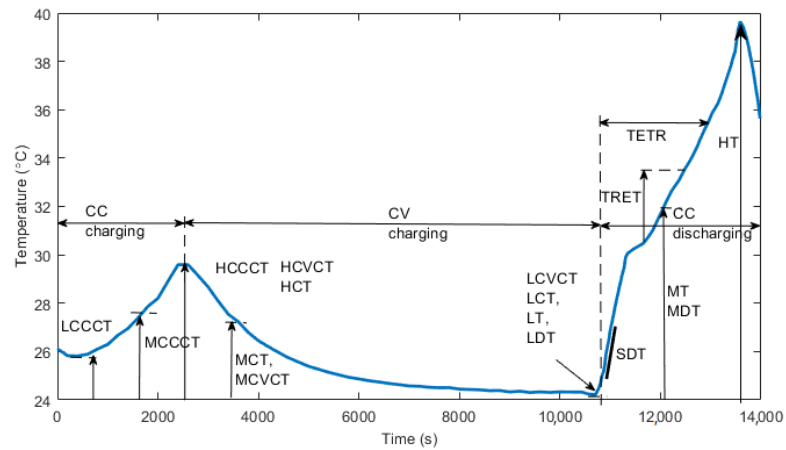
Figure 6. Temperature-based HIs.
