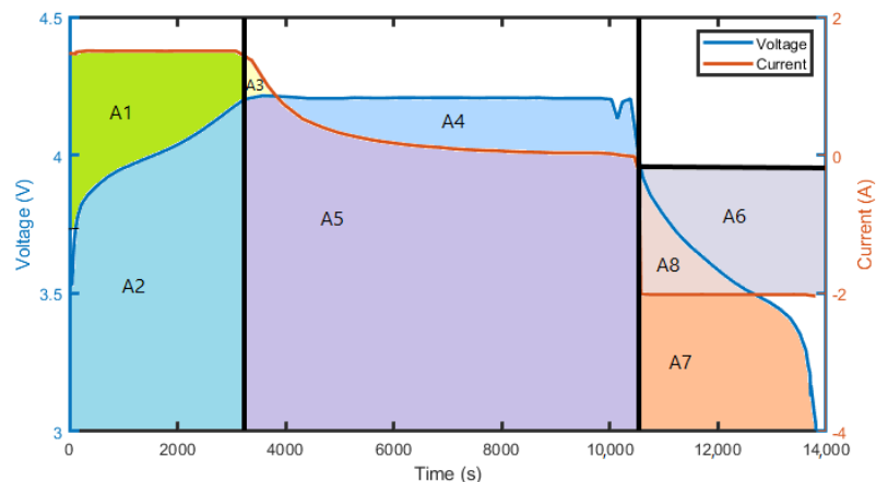
Figure 7. Voltage- and current-integral-based HIs.
