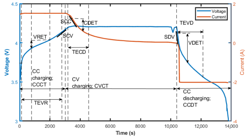
Figure 5. Voltage- and current-based HIs.
