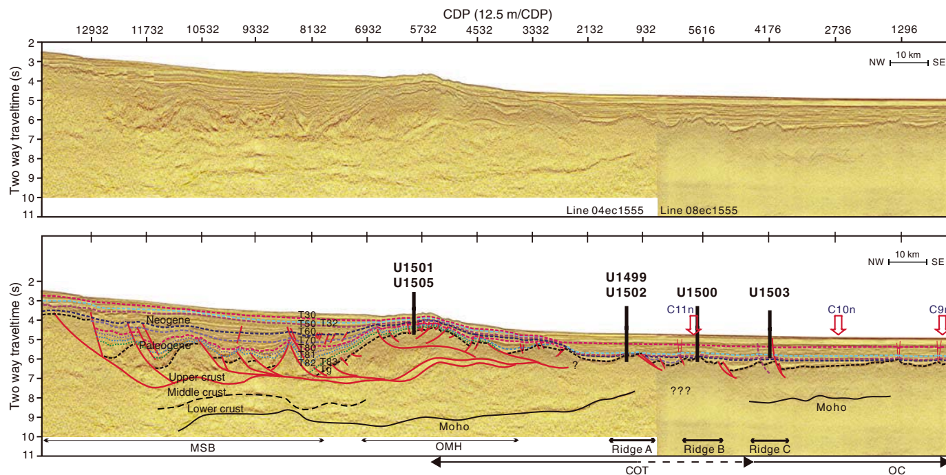
Figure F5. Deep crustal time-migrated seismic reflection data without and with interpretation. Note the rather thin lower crust (two layers) above a strong Mohorovičić seismic discontinuity (Moho) reflector that can be followed oceanward. Moho reflection is weak to absent seaward from around the interpreted COT. Wide-angle seismic data (Yan et al., 2001) confirm ~6 km thick ocean crust (OC) seaward of the COT. A large detachment fault ~150 km inland of the COT separates more stable crust landward from that of highly extended crust seaward. An OMH is a fairly consistent feature along this margin segment. Key seismic unconformities are shown in purple (T70; ~32 Ma breakup unconformity?) and blue (T60; ~23 Ma regional basin event). These ages are inferred from long-distance (>100 km) correlation of seismic unconformities with industry holes and ODP Leg 184 Site 1148 (T60); ages need confirmation by coring and are only tentative. Tg (black) is basement. Arrows = approximate position of seafloor magnetic anomalies with chron numbers. Seismic data are from Line 04ec1555-08ec1555 (courtesy of Chinese National Offshore Oil Corporation [CNOOC]). Location of line is shown in Figure F3. CDP = common depth point. C11n, C10n, and C9n = approximate location of normal polarity magnetic isochrons. MSB = midslope basin.
