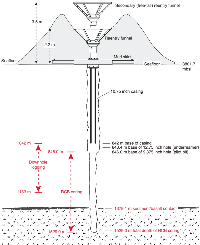
Figure F9. Reentry system and casing, Hole U1500B.
