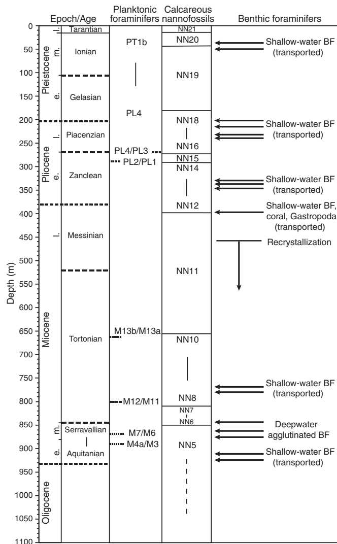
Figure F34. Biostratigraphic and paleoenvironmental summary, Site U1499. Calcareous nannofossil and planktonic foraminifer biozonal assignments with paleoenvironmental information are provided by benthic foraminifers (BF).
