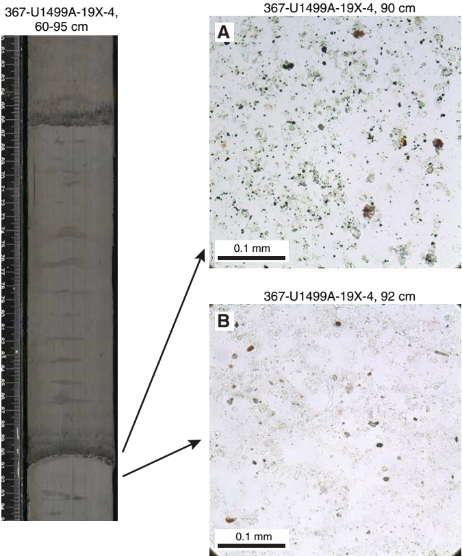
Figure F15. Representative section of clay with silt interbeds, Subunit IIIA. A. Very thin silt interbed showing mostly siliciclastic silt and clay. B. Dominant clay lithology showing mostly siliciclastic clay material (PPL).
