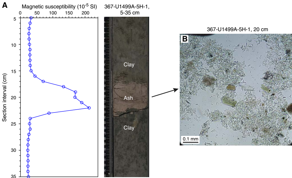
Figure F12. (A) Magnetic susceptibility, core image, and (B) smear slide image of pale brownish volcanic ash layer (plane-polarized light [PPL]), Unit I.
