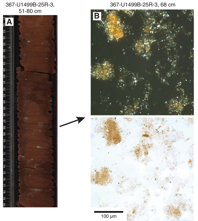
Figure F29. A. Red claystone. B. Abundant iron oxides that glow orange under XPL (top) and appear brownish orange in PPL (bottom).
