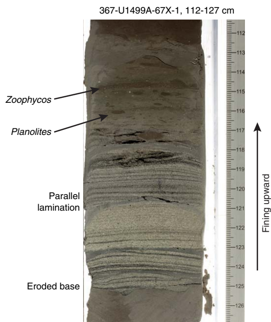
Figure F19. Foraminifer siltstone layer showing erosive base, parallel lamination, and fining-upward sequence, Unit VII. The clay at the top of the interval has Planolites and Zoophycos trace fossils.
