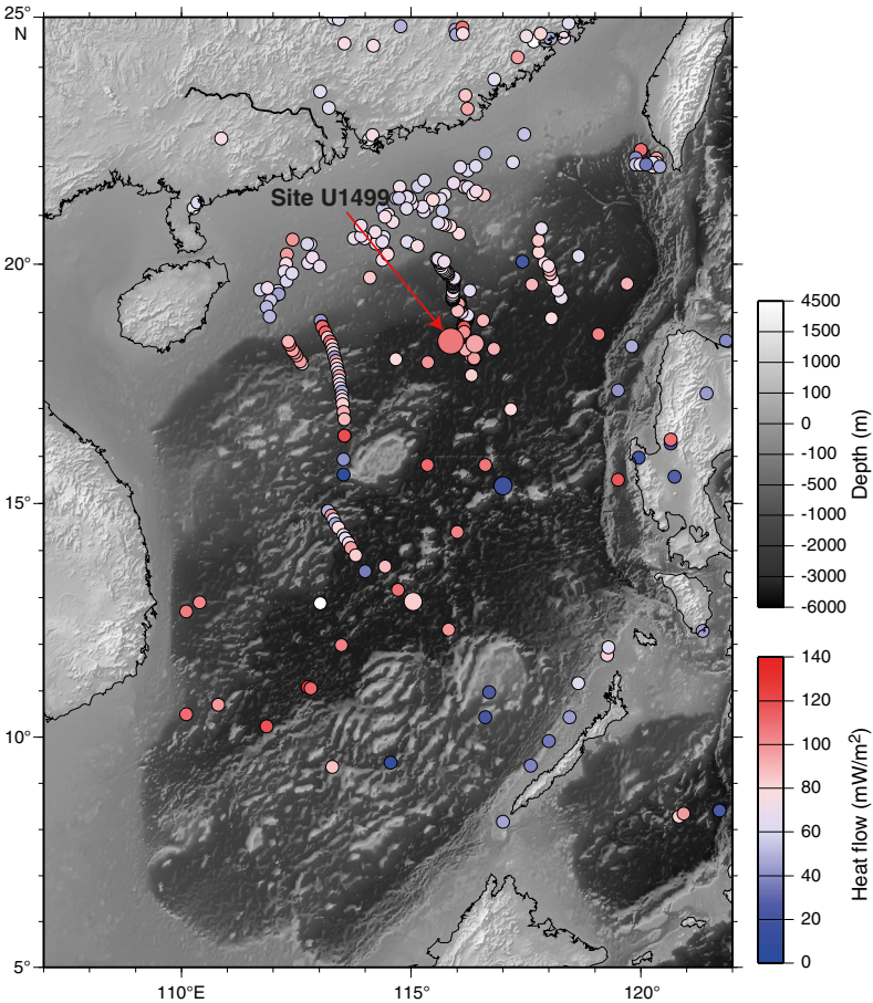
Figure F57. Seafloor heat flow values, South China Sea. Large circle = value calculated based on Site U1499 data, smaller circles = previous measurements compiled in Li et al. (2010, 2015c).
