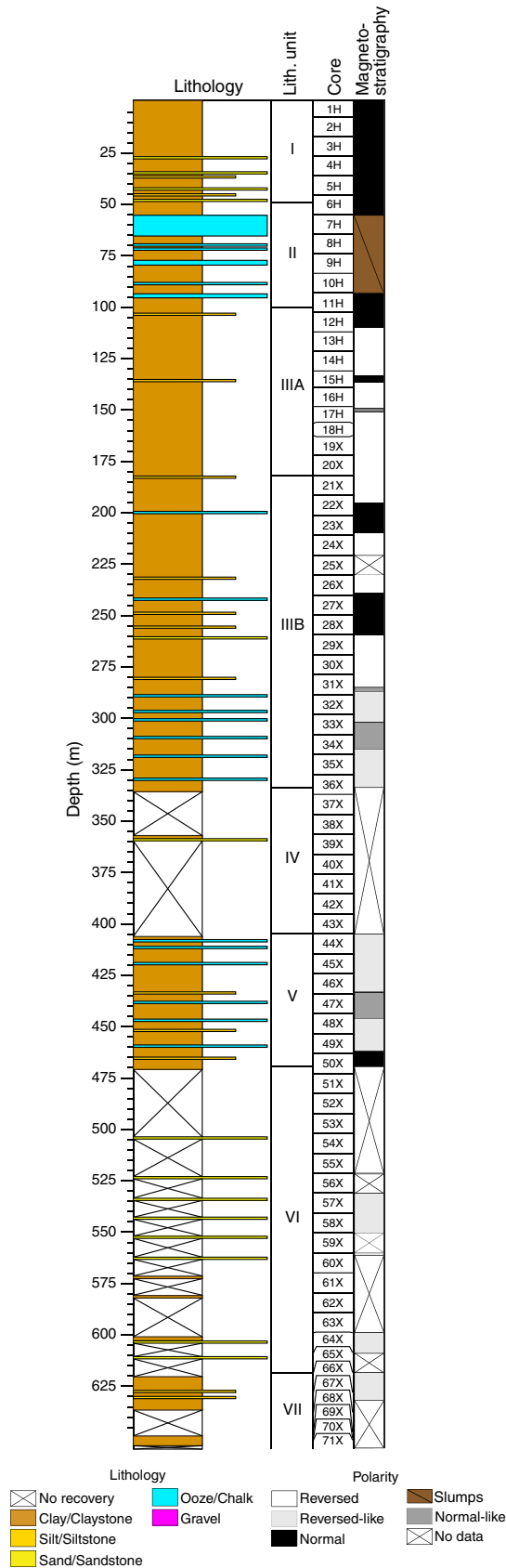
Figure F41. Magnetostratigraphy, Hole U1499A. Lithology column is simplified from the shipboard core description (see Figure F8).
