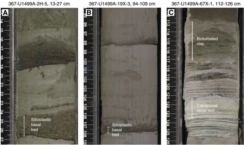
Figure F27. Fining-upward sequences seen throughout Site U1499 intervals. A. Sand-based fining-upward sequence. B. Silt-based fining-upward sequence. C. Fining-upward sequence with laminated foraminiferal sand at the base. The uppermost clay contains bioturbation, including Zoophycos and Planolites trace fossils. Note biscuiting drilling disturbance.
