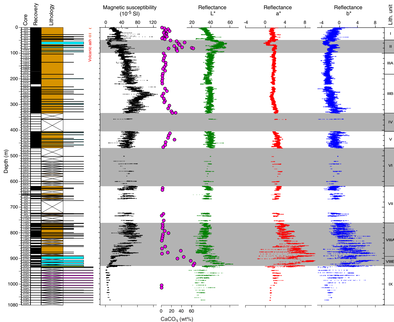
Figure F9. Correlation of lithostratigraphic units with magnetic susceptibility, reflectance spectroscopy, and carbonate content, Site U1499. Magnetic susceptibility and reflectance spectroscopy are displayed with a 10-point running average.
