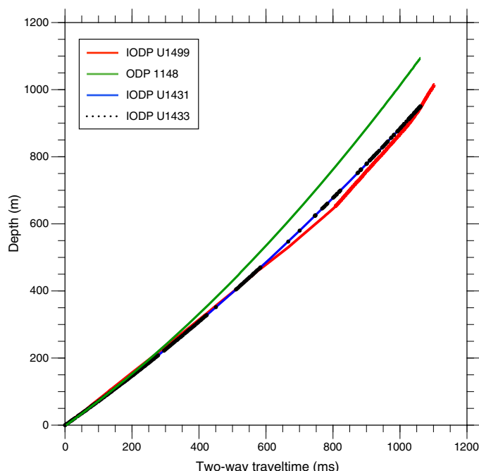
Figure F59. Site U1499 TDR curve compared to Sites U1431, U1433, and 1148 (Li et al., 2008).
