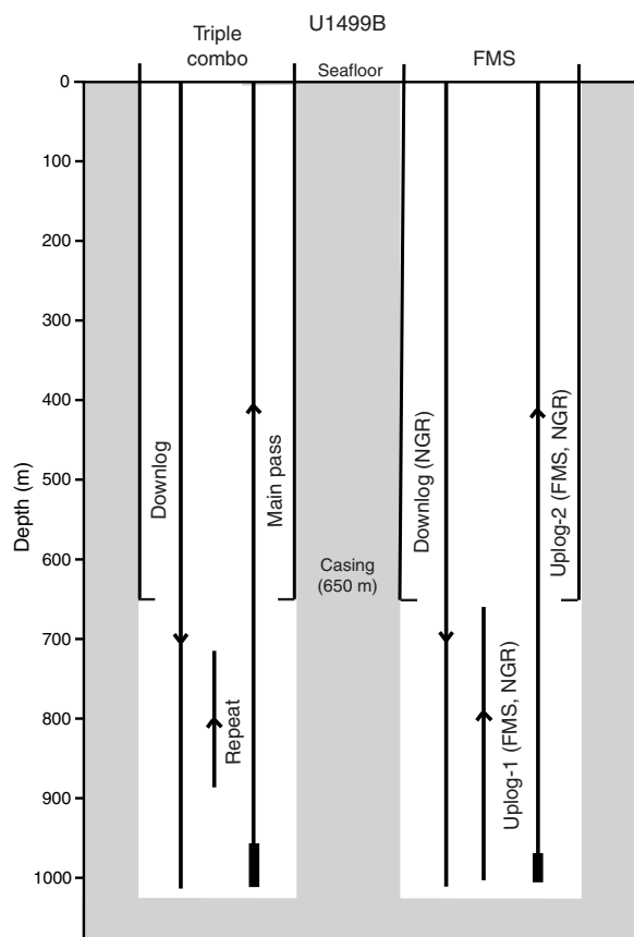
Figure F51. Logging operations summary, Hole U1499B.
