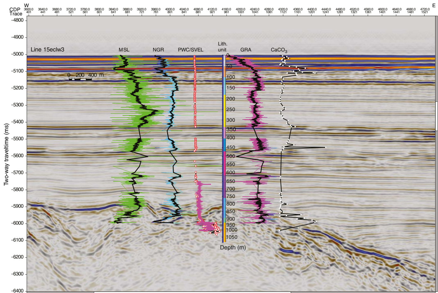
Figure F60. Seismic section across Site U1499. Site is located at lithostratigraphic unit plot (gray = Unit I, light brown = Unit II, light blue = Subunit IIIA, yellow = Subunit IIIB, pink = Unit IV, blue = Unit V, purple = Unit VI, violet = Unit VII, medium blue = Subunit VIIIA, cyan = Subunit VIIIB, orange = Unit IX). Other Site U1499 data are offset from site location: magnetic susceptibility logger (MSL), NGR, PWC velocity and VSI shear velocity (SVEL) logging data, GRA density, and \text{CaCO}_3 content.
