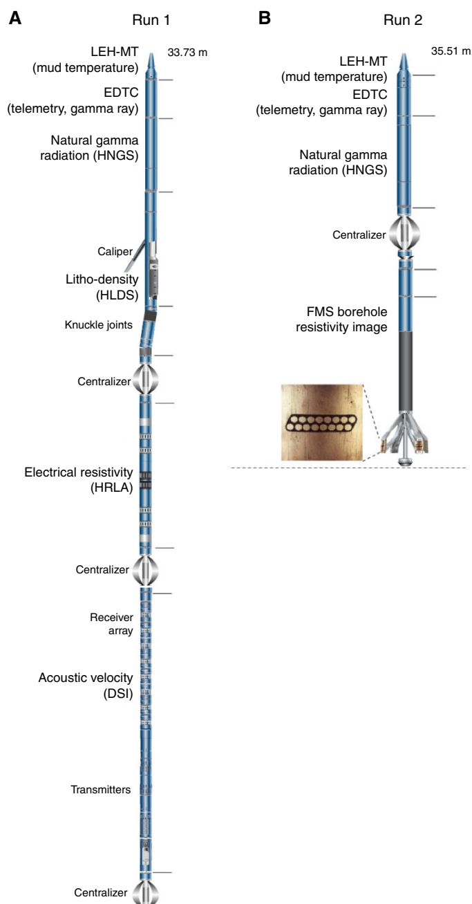
Figure F50. Downhole logging tool strings, Site U1499. A. Run 1. B. Run 2. LEH-MT = logging equipment head-mud temperature, EDTC = Enhanced Digital Telemetry Cartridge, HNGS = Hostile Environment Natural Gamma Ray Sonde, HLDS = Hostile Environment Litho-Density Sonde, HRLA = High-Resolution Laterolog Array, DSI = Dipole Sonic Imager, GPIT = General Purpose Incliner Tool, FMS = Formation MicroScanner.
