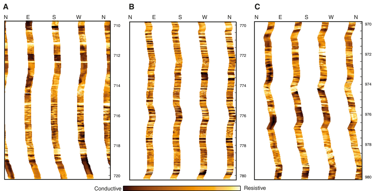
Figure F54. FMS images, Hole U1499B. These images use a 2 m interval dynamic normalization to enhance local contrast between conductive and resistive material. A. Contrasting smooth and irregular layers possibly reflecting claystones and sandstones in an interval of low core recovery, logging Unit 1/lithostratigraphic Unit VII. B. 10 cm relatively horizontal bedding in claystones and sandstones, logging Unit 1/lithostratigraphic Unit VII. C. Irregular, oblique, and chaotic structures or bedding in gravel/breccia, logging Unit 3 corresponding to lithostratigraphic Subunit IXC.
