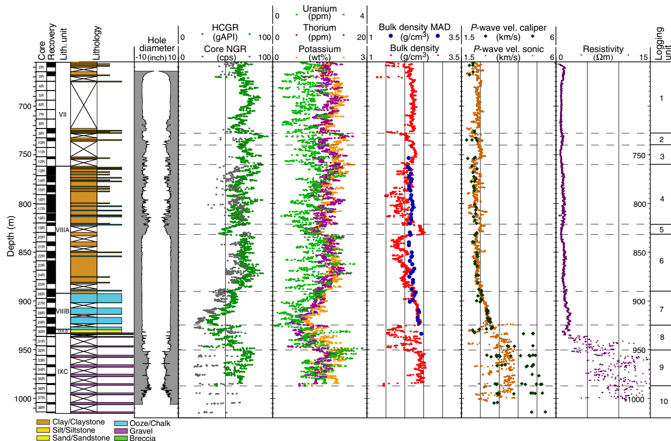
Figure F53. Downhole logs, Hole U1499B. Downhole logs are on the logging depth scale (WSF) and MAD discrete samples, PWC, and core recovery data are on the core depth scale (CSF-A). Small differences between these depth scales are usually <2 m. HCGR = computed gamma ray.
