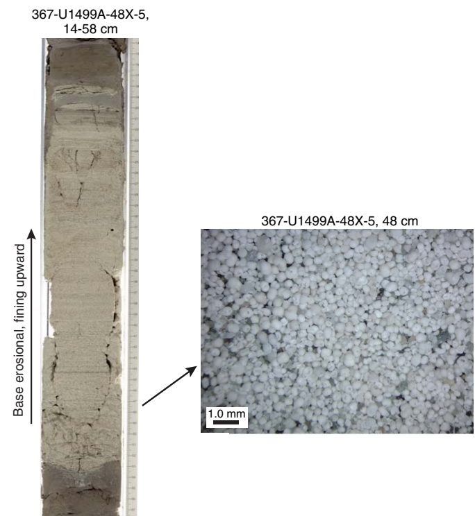
Figure F17. Thick interval of well-sorted foraminiferal sand with an erosive base and fining-upward sequence. Foraminifers consist mainly of planktonic Sphaeroidinellops seminulina (detailed image from sieved paleontology sample).
