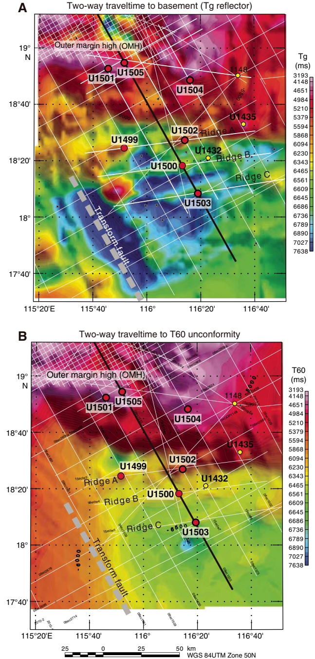
Figure F3. Two-way traveltimes to (A) acoustic basement (Tg reflector) and (B) Unconformity T60 and location of Expedition 367/368 sites. Proposed drilling transect (thick black line) was located approximately at the center of a margin segment bounded to the southwest by a transform fault. North-eastern boundary of margin segment is located around Expedition 349 Site U1435. In this location, the outer margin high and Ridge A seem to coalesce, and Ridges B and C of the COT become indistinct toward the northeast within the next margin segment. Note that outer margin high is slightly east-northeast to the more parallel Ridges A, B, and C.
