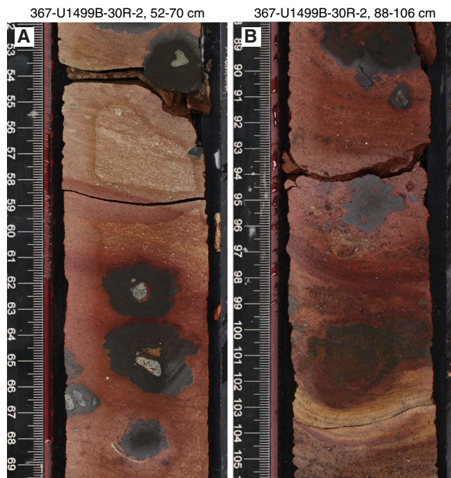
Figure F22. A. Black-brownish iron-manganese (composition confirmed by postcruise XRF scanning) nodules in lowest part of Subunit VIIIB. Angular to subrounded pebbles form center of nodules. B. Gradational contact with Subunit IXA below nodules.
