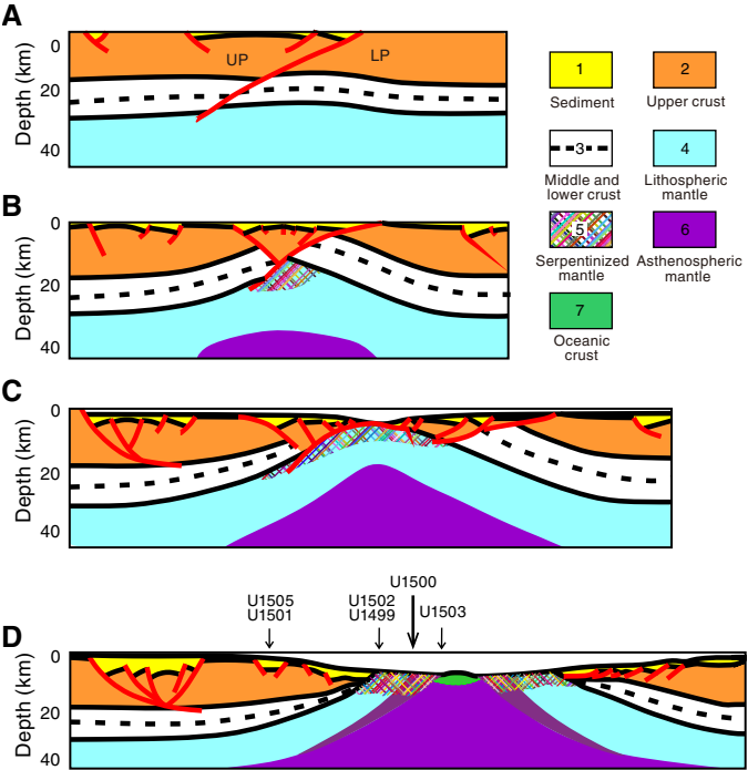
Figure F5. A–D. Schematic development of continental breakup initiated by a simple shear along a deep, low-angle fault. B–D are slightly modified from Huismans and Beaumont (2011) and illustrate modeling-based stages of extension at magma-poor rifted margins of the Iberia-Newfoundland type. Key features of D are thinning of upper crust, juxtaposition of lower crust (e.g., Site U1499), and serpentinized mantle (Site U1500) between outer margin and igneous oceanic crust. UP = upper plate, LP = lower plate.
