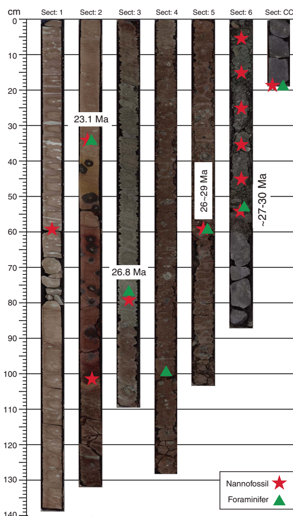
Figure F36. Additional samples, Core 367-U1499B-30R. The oldest age range estimate for Section 30R-6 is based on the last occurrence of S. predistentus (26.93 Ma) and the presence of S. distentus .
