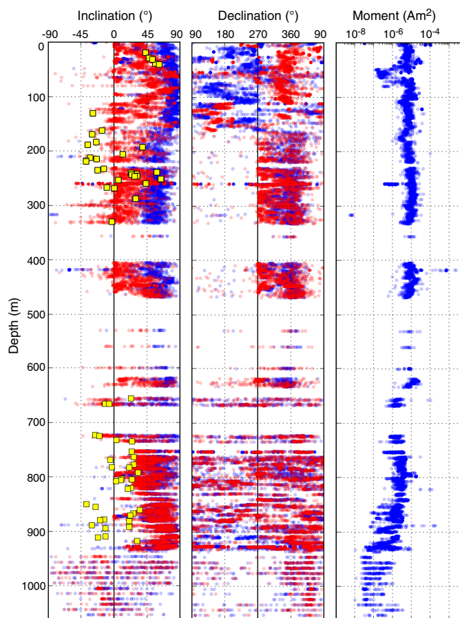
Figure F38. Remanent magnetization of archive-half sections, Site U1499. Declinations shallower than 162 m (APC coring) are corrected using orientation from Icefield MI-5 core orientation tool. Red = data determined by maximum AF treatment, blue = NRM, yellow = discrete samples.
