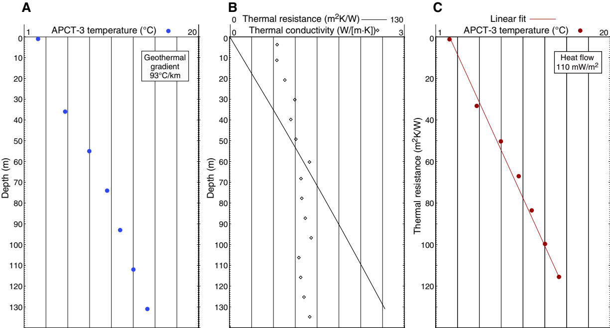
Figure F56. Heat flow calculations, Hole U1499A. A. Formation temperature measurements. B. Thermal conductivity data from core measurements and calculated thermal resistance. C. Thermal resistance plotted against formation temperature, providing heat flow estimate for Hole U1499A of 110 mW/m 2 .
