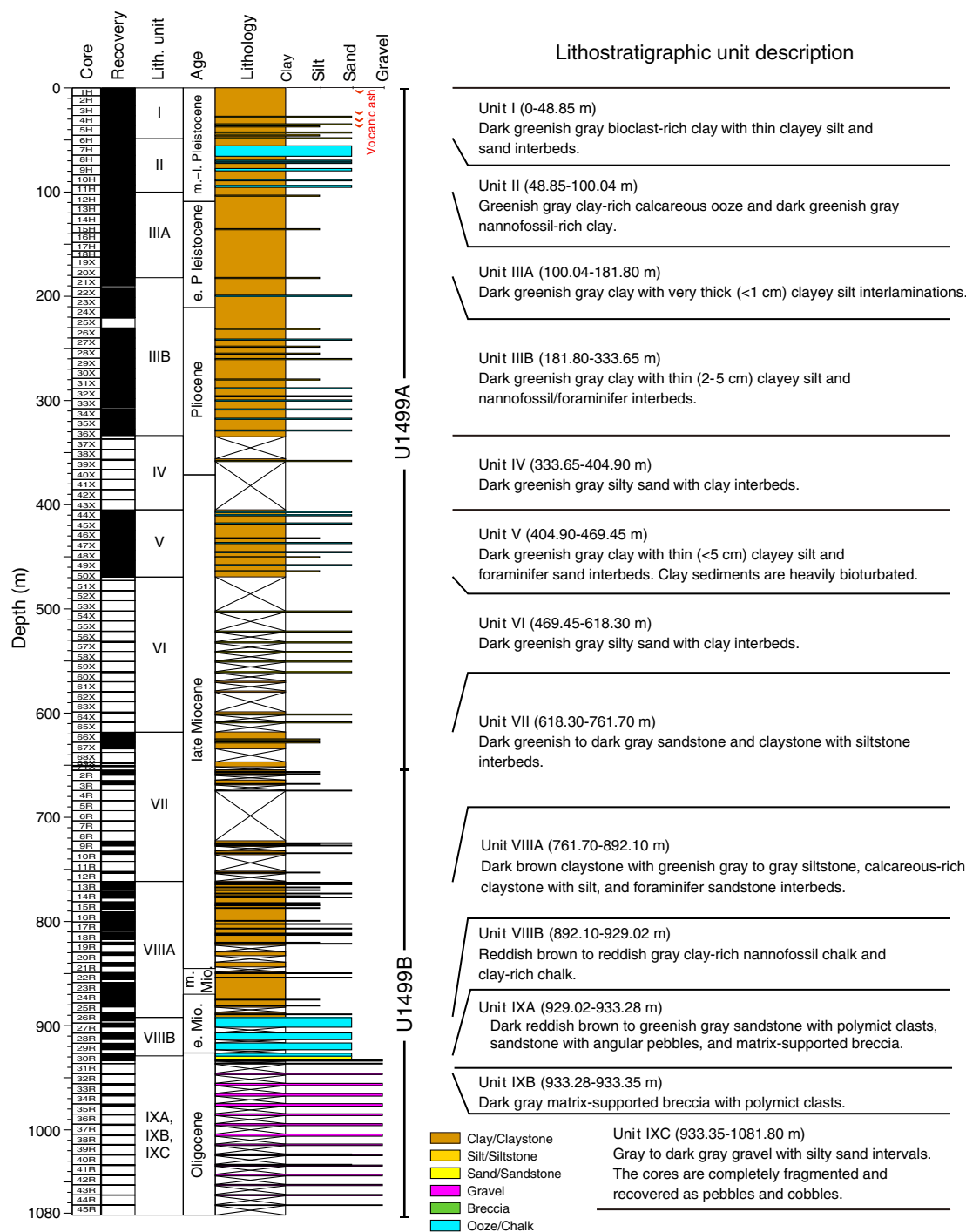
Figure F8. Lithostratigraphic summary of Site U1499 with simplified lithology and unit description of combined Holes U1499A and U1499B.
