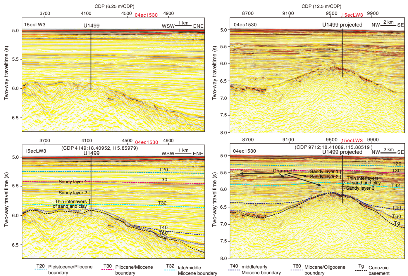
Figure F4. Original and interpreted seismic profiles across Site U1499. Seismic profile locations are shown in Figures F1, F2, and F3. Site U1499 is located on seismic Profile 15ecLW3 and projected onto seismic Profile 04ec1530. Red text and tick marks = locations of crossing seismic lines. CDP = common depth point. All seismic profiles are courtesy of the Chinese National Offshore Oil Corporation [CNOOC]).
