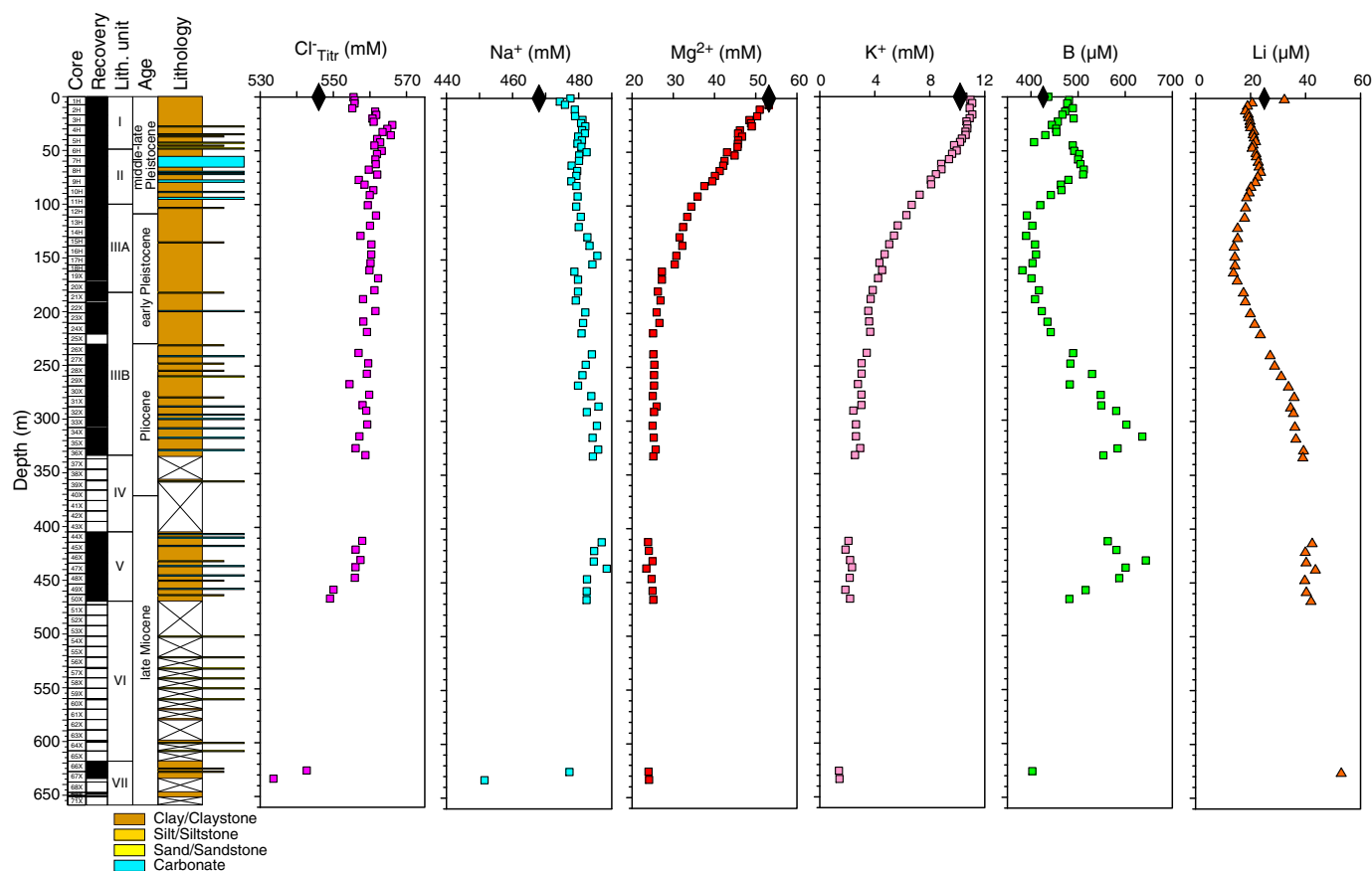
Figure F47. Interstitial water chloride, sodium, magnesium, potassium, boron, and lithium concentration profiles, Hole U1499A. Black diamonds = typical seawater values.
