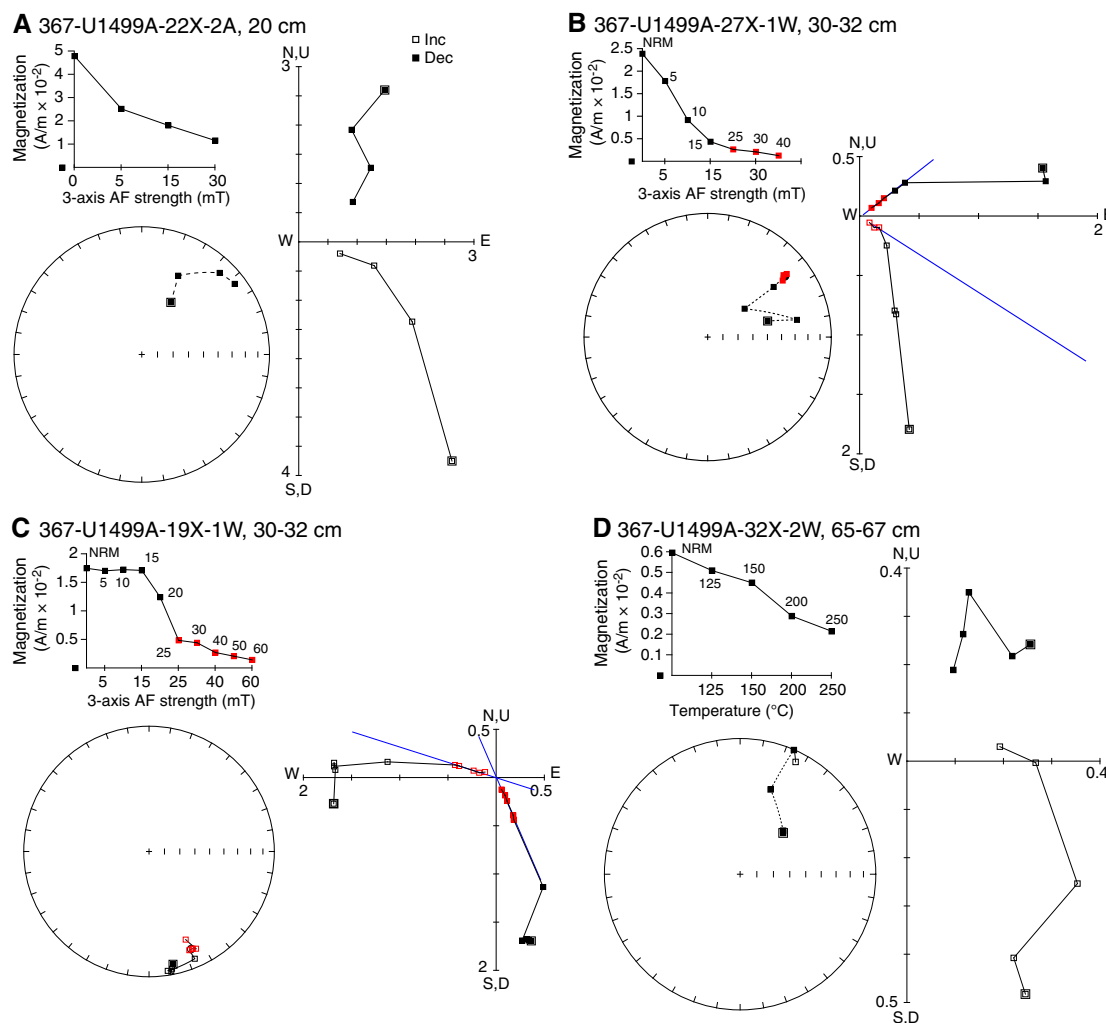
Figure F39. Demagnetization plots of (A) archive-half section and (B–D) discrete samples, Hole U1499A. Stereographic plots: solid squares = positive (down) inclination, open squares = negative (up) inclination. A. Normal polarity. B. Normal polarity; PCA calculated ChRM (blue line; red squares = measurements used in calculation) has 51^\circ declination and 21^\circ inclination. C. Reversed polarity with ChRM declination of 156^\circ and inclination of -16^\circ . D. Potential reversed polarity.
