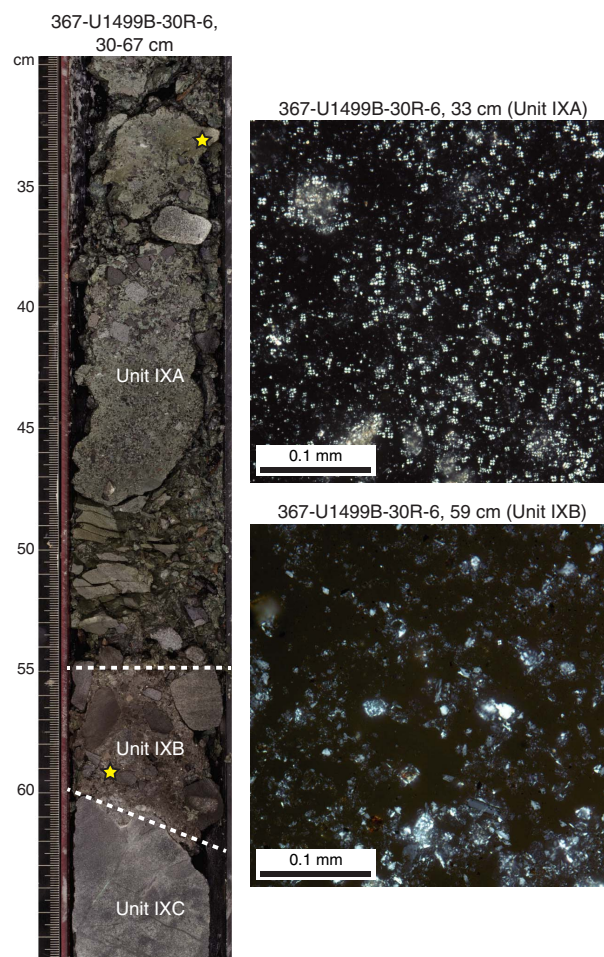
Figure F25. Breccia intervals showing matrix composition changes between subunits: reddish brown to greenish gray sandstone in Subunit IXA and brownish gray sandstone in Subunit IXB. Subunit IXA contains a higher concentration of calcareous microfossils compared to Subunit IXB. Yellow stars = locations of smear slides (XPL) taken from supporting matrix of the breccia intervals.
