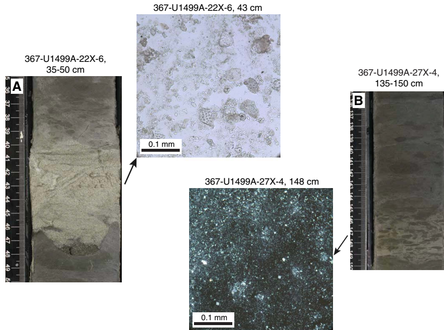
Figure F16. Increased carbonate content and bioturbation, Subunit VIII B. A. Foraminiferal sand interbed showing an erosive contact with underlying clay (PPL). B. Nannofossil-rich clay showing heavy bioturbation and lighter clay intervals with abundant nannofossils (XPL).
