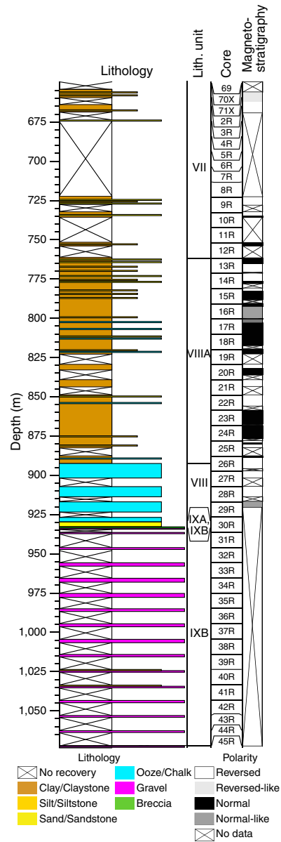
Figure F42. Magnetostratigraphy, Hole U1499B. Lithology column is simplified from shipboard core description (see Figure F8).
