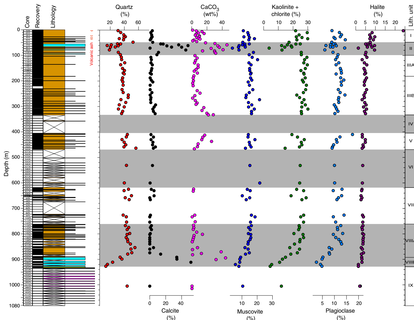
Figure F10. Bulk mineralogy by XRD with major mineral compositions and correlation of calcite with carbonate content, Site U1499.
