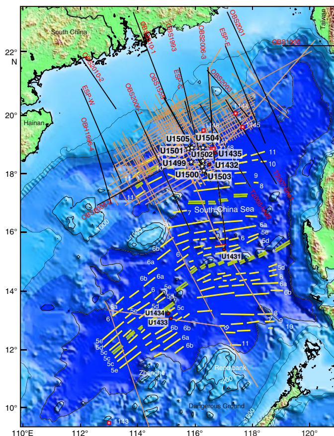
Figure F1. Seismic data coverage and magnetic anomalies of the SCS Basin, Expedition 367/368. Black lines = ocean-bottom seismometer refraction data. Other seismic lines are mostly multichannel seismic reflection data. White stars = Expedition 367/368 sites, red squares = Leg 184 sites, red circles = Expedition 349 sites. For more detail, see Figure F2.
