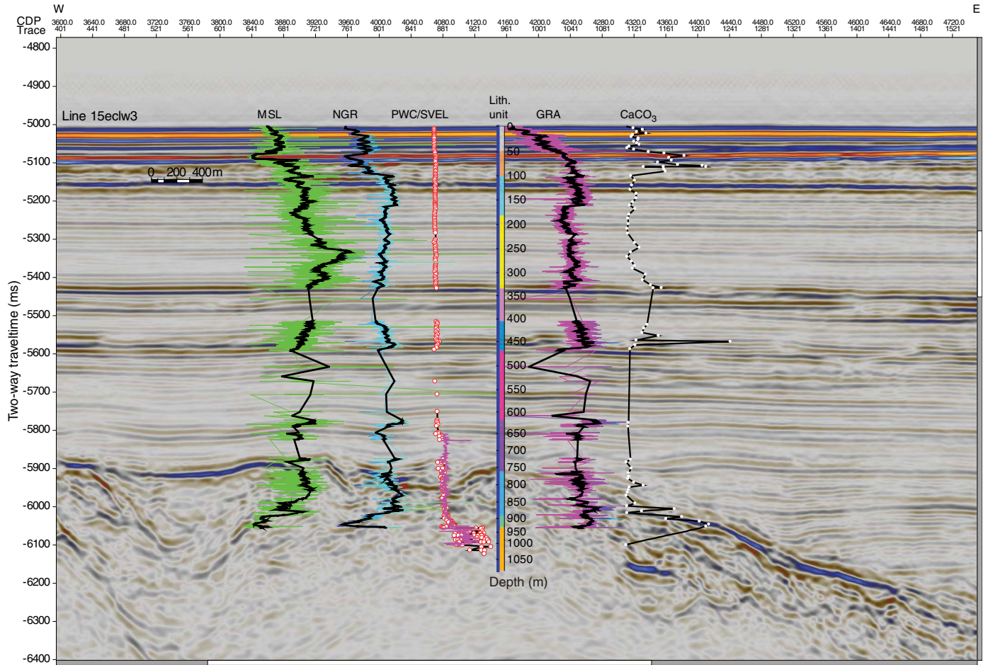
Figure F63. Seismic section across Site U1499 using alternative TDRs without constant velocity for sandy no-recovery zones. Site is located at lithostratigraphic unit plot (see Figure F60). Other Site U1499 data are offset from site location: MSL, NGR, PWC velocity and VSI shear velocity logging data, GRA density, and CaCO 3 content.
