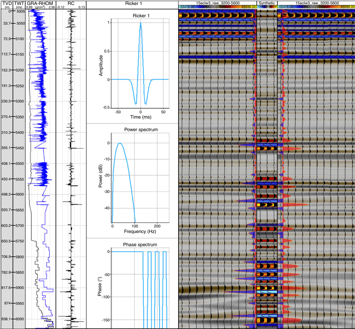
Figure F61. Synthetic seismogram computed for Site U1499. Panels from left to right: density (blue) and velocity (black) values, reflection coefficient (RC), seismic source properties, and real seismic traces with synthetic seismogram inserted in the center.
