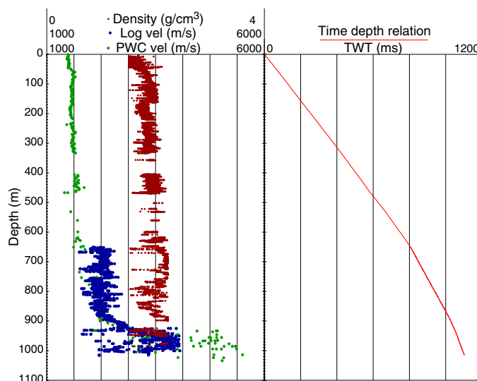
Figure F58. HLSL density and DSI velocity collected during logging, PWC velocity data, and TDR adjusted to seafloor, Site U1499. PWC velocity data were used from the seafloor to 655 m, and DSI velocity data were used below that depth (see Table T14).
