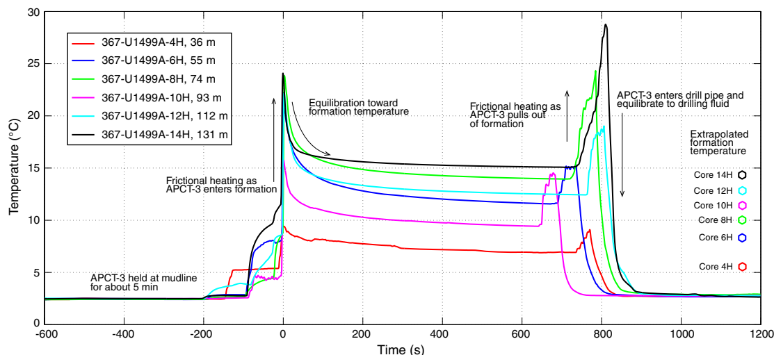
Figure F55. APCT-3 temperature-time series with extrapolated formation temperature estimates, Hole U1499A (see Table T13).
