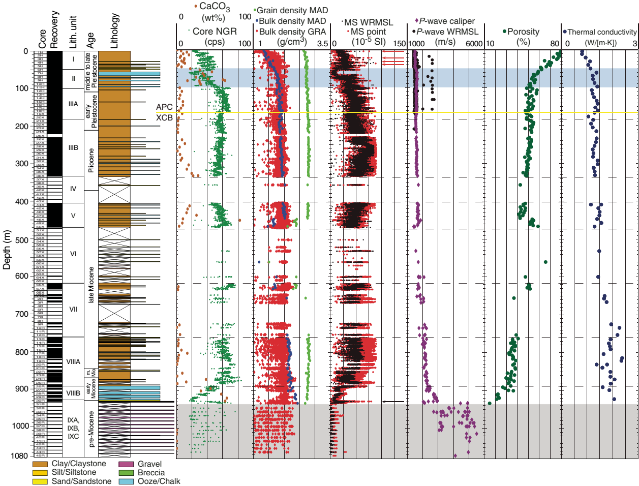
Figure F48. Petrophysics data summary, Holes U1499A and U1499B. Red arrows = magnetic susceptibility (MS) peaks associated with ash layers, black arrow = MS peak in layer of Core 367-U1499B-30R containing Fe-Mn nodule, yellow line = APC/XCB coring boundary where some physical properties values change, blue box = Unit II slump layer, gray box = gravel layer in Subunit IXC. cps = counts per second.
