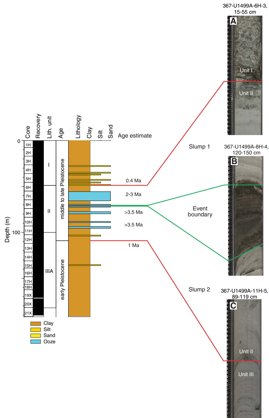
Figure F31. Lithostratigraphic summary correlated to biostratigraphic ages and slump events in Unit II, Site U1499. Age estimates are based on age correlation of foraminifers and nannofossils. A. Erosive contact separating Units I and II. B. Dark clayey silt layer separating two slump events. C. Erosive contact separating Units II and III.
