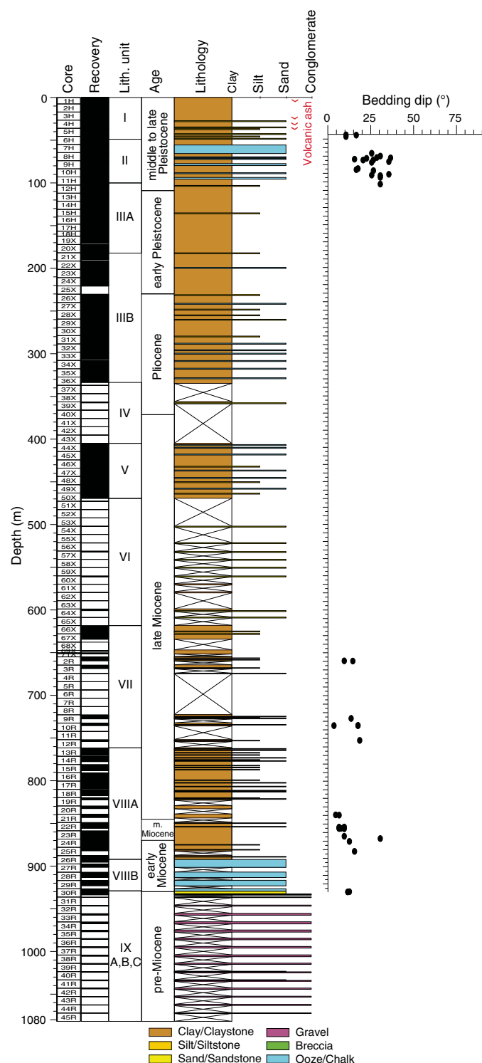
Figure F30. Lithostratigraphic summary of Site U1499 with bedding dips in Holes U1499A and U1499B. Flat-lying bedding and bedding dips <5^\circ were not measured.
