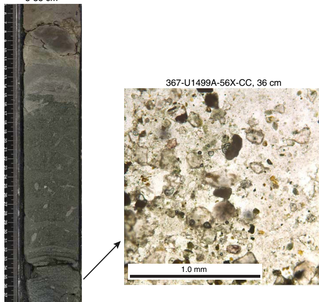
Figure F18. Unconsolidated medium-grained sand showing the dominant siliciclastic composition (PPL), Unit VI.
