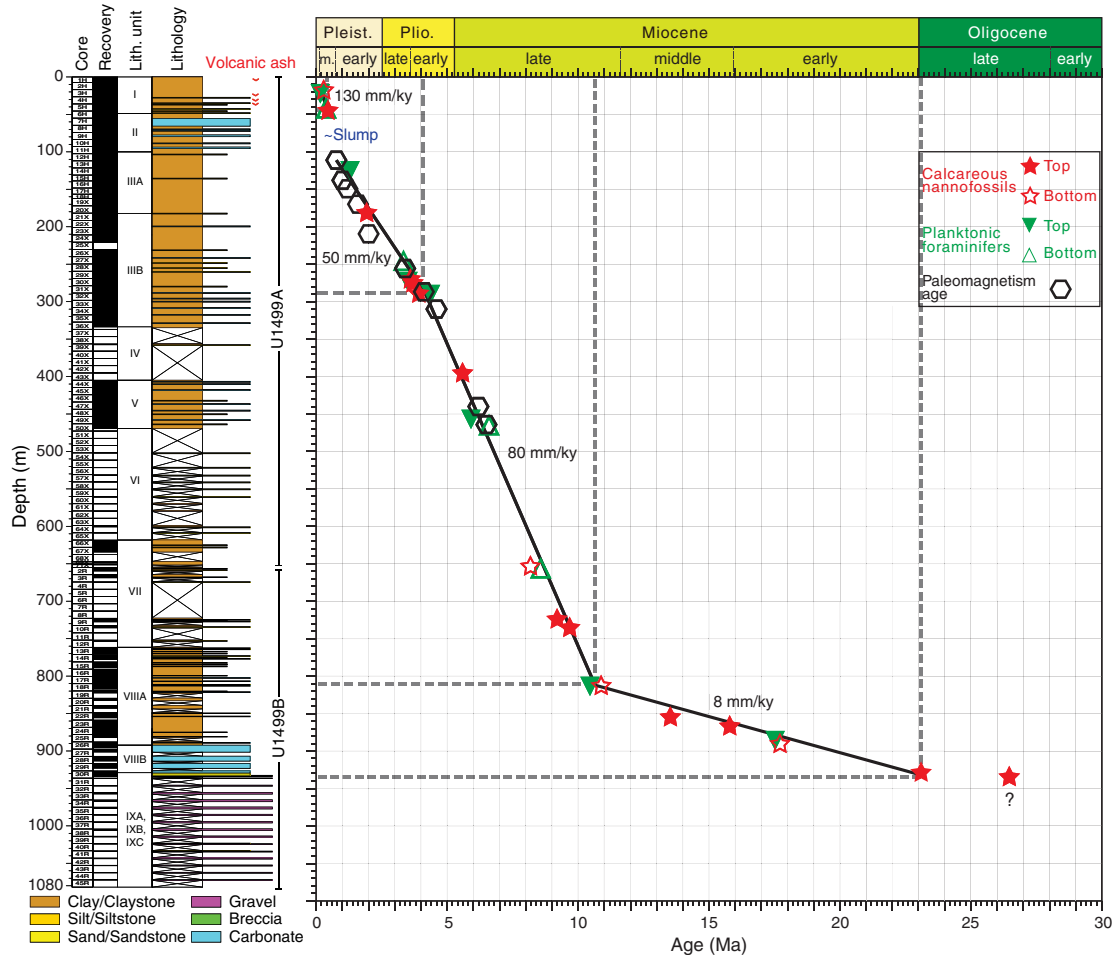
Figure F35. Age-depth model, Site U1499. Plotted event data are in Tables T4 and T8 (see Paleomagnetism). Top = last appearance datum, bottom = first appearance datum.
