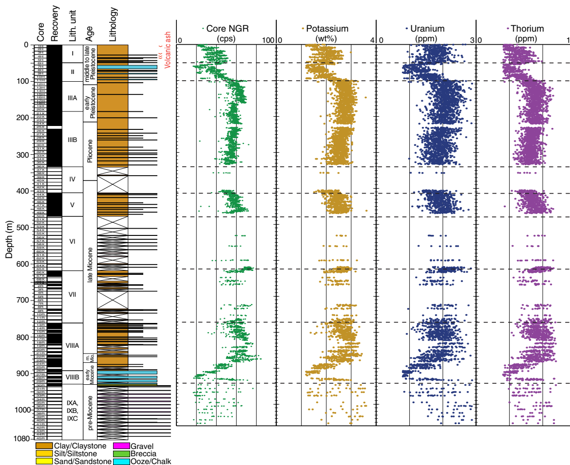
Figure F49. Core NGR measurements, Holes U1499A and U1499B. Estimates of K, U, and Th concentrations are derived from NGR measurements using method of De Vleeschouwer et al. (2017).
