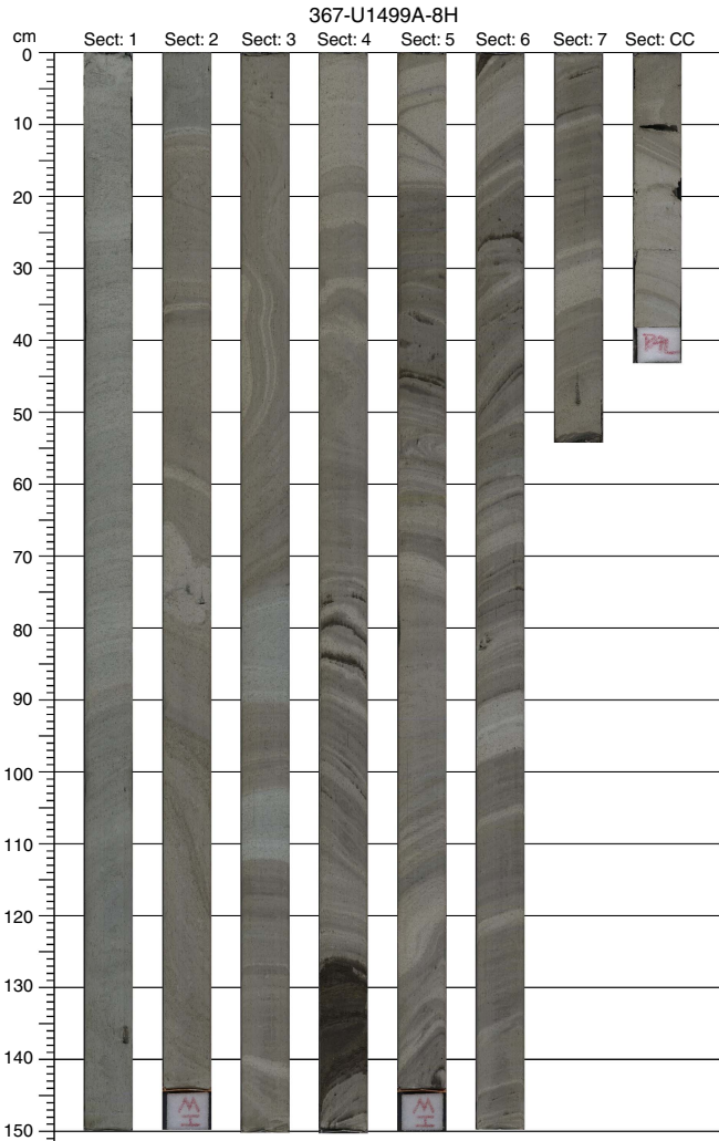
Figure F14. Core composite image showing syndimentary deformation with distinct fold, fault, and inclined bedding structures.
