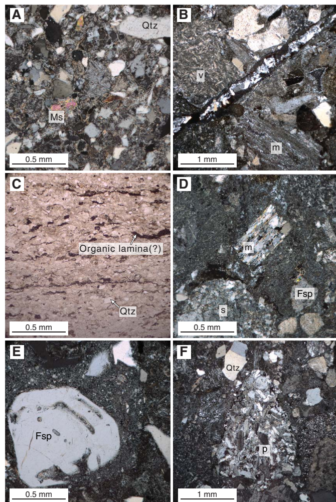
Figure F26. Sandstone cobbles from Subunit IXC, Hole U1499B. Qtz = quartz, Ms = muscovite, Fsp = feldspar, v = lithic volcanic, m = lithic metamorphic, s = lithic sedimentary, p = lithic plutonic. A. Silty sandstone (30R-CC). B. Gravelly sandstone (34R-2). C. Sandy siltstone (38R-1). D–F. Gravelly sandstone (39R-1).
