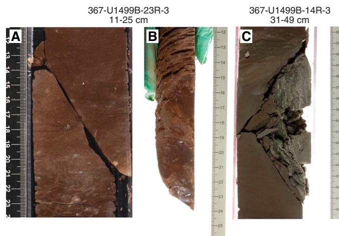
Figure F33. Structures in Subunit VIIIA, Hole U1499B. A. Compaction-related fault. B. Perpendicular view of compaction-related fault. C. Sedimentary structure with a mass of sand with deformed finer grained claystones above.
