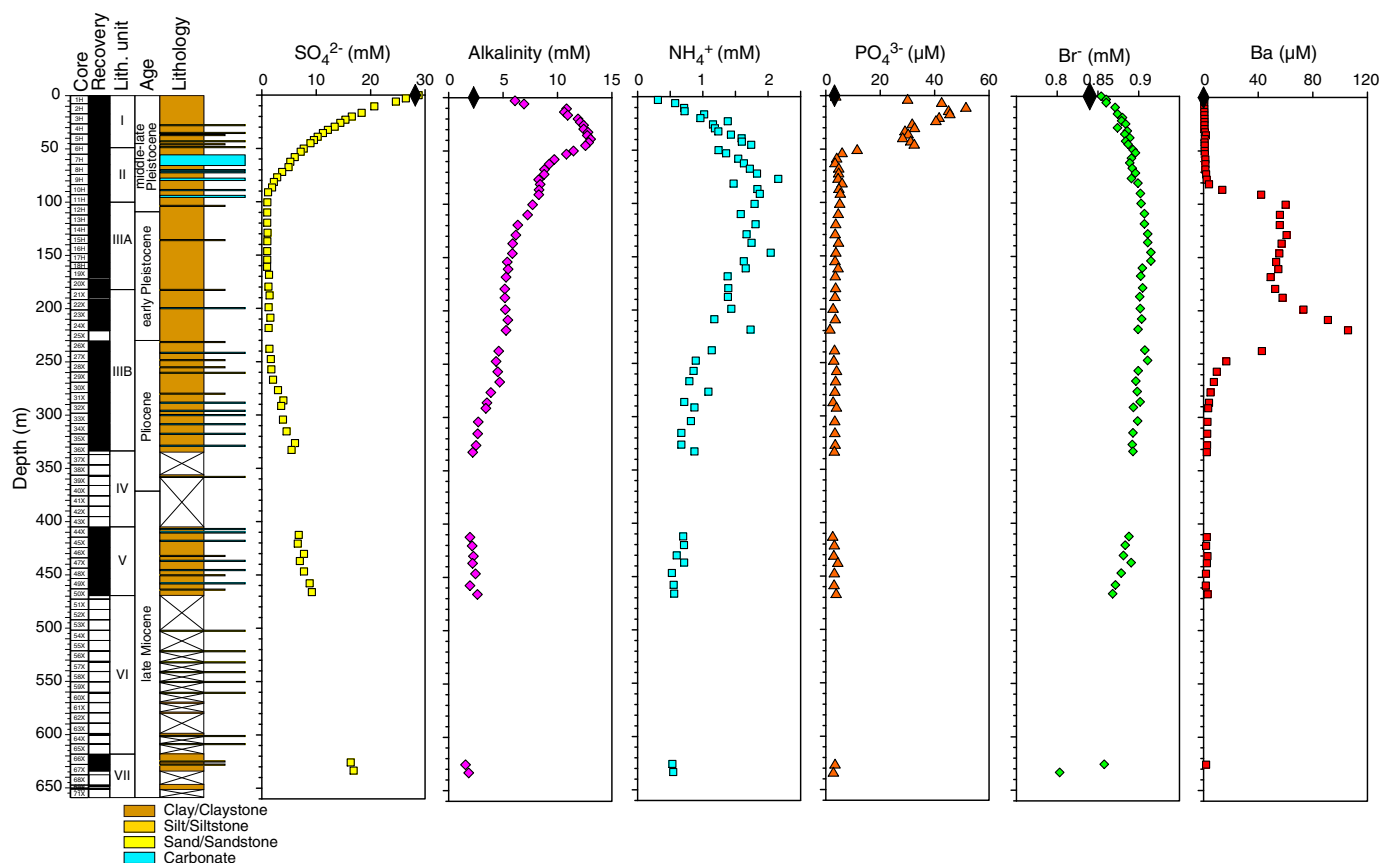
Figure F45. Interstitial water sulfate, alkalinity, ammonium, phosphate, bromide, and barium concentration profiles, Hole U1499A. Black diamonds = typical seawater values.
