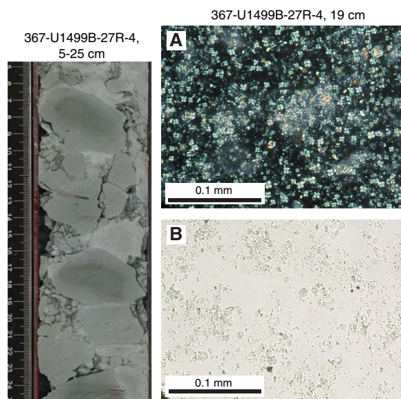
Figure F21. Greenish gray claystone interbedded in brown claystone sections showing abundant calcareous grains, Subunit VIIIB. A. XPL. B. PPL.
