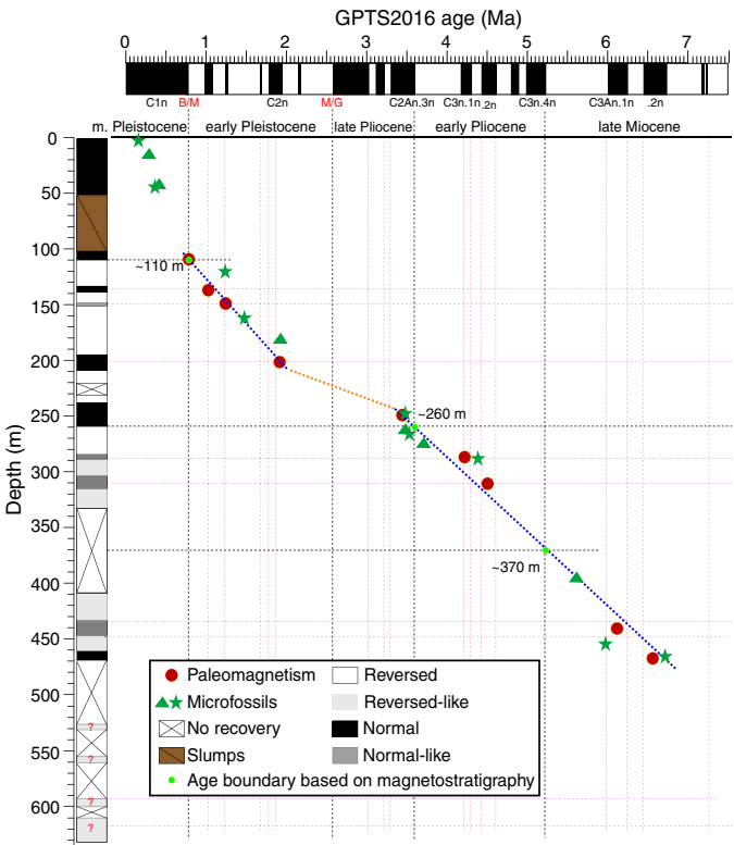
Figure F43. Age-depth model constructed from shipboard paleomagnetic analysis, Site U1499. A possible change in age-depth model was observed during late Pliocene and earliest early Pleistocene (dashed orange line). B/M = Brunhes/Matuyama Chron boundary, M/G = Matuyama/Gauss Chron boundary. GPTS2016 = geomagnetic polarity timescale of Ogg et al. (2016).
