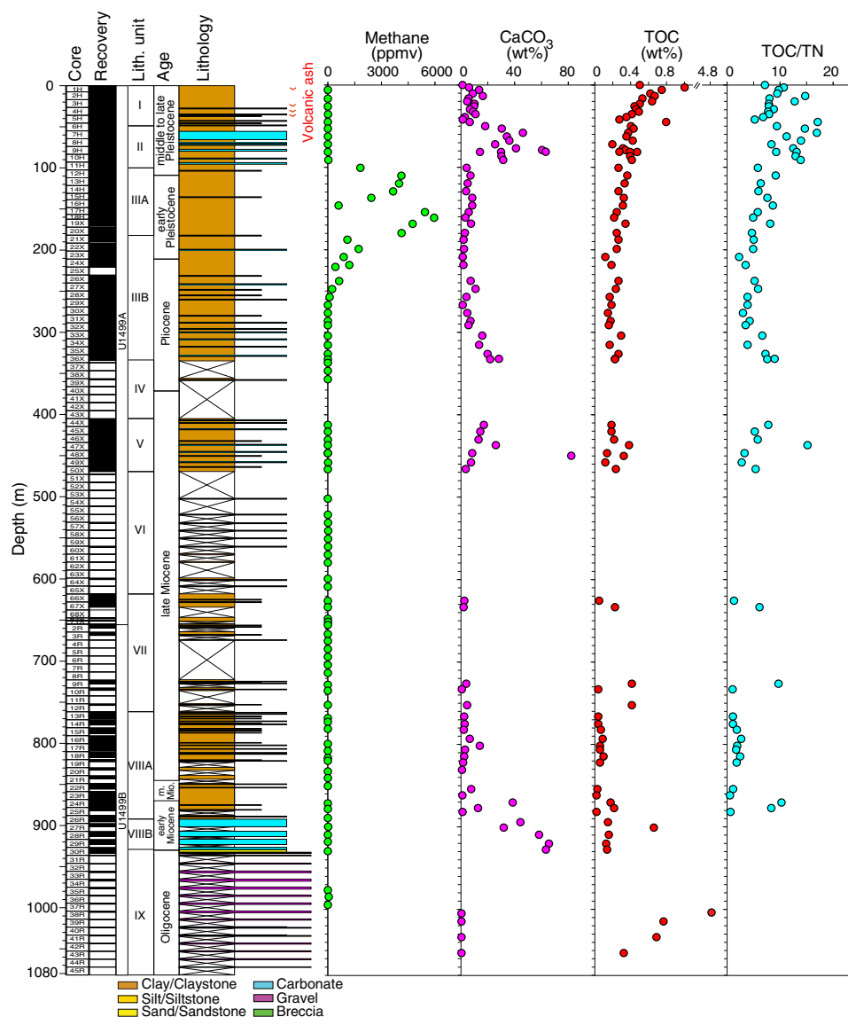
Figure F44. Lithology, methane, calcium carbonate, TOC, and TOC/TN profiles, Site U1499.
