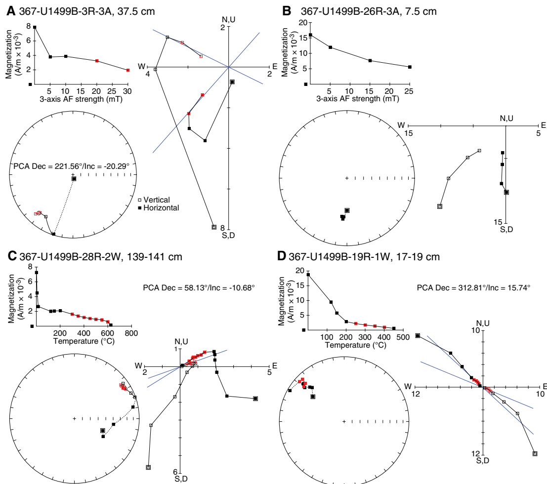
Figure F40. Demagnetization plots of (A, B) archive-half sections and (C, D) discrete samples, Hole U1499B. PCA calculated ChRM (blue line; red squares = measurements used in calculation) is also shown. Note the high coercivity of samples in A and B.
