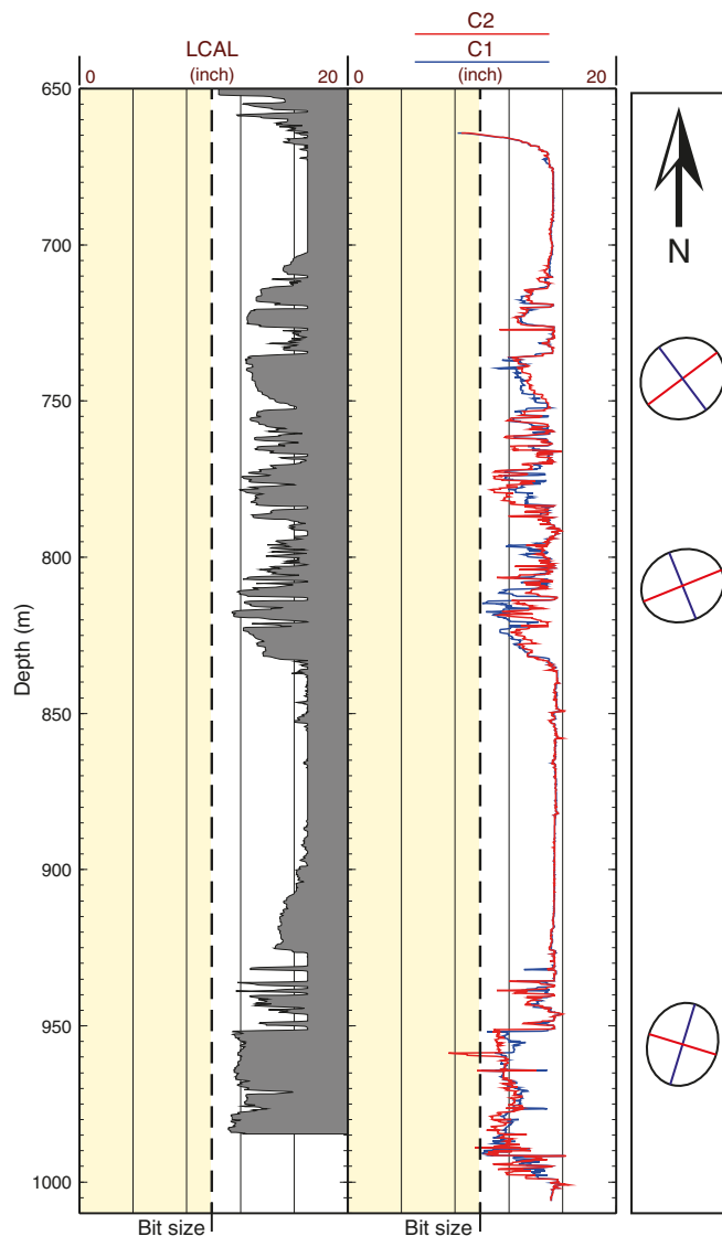
Figure F52. Hole U1499B diameter. Yellow box with dashed lines = size of drill bit (9.875 inches). Left: measurements from triple combo caliper (LCAL). Middle: measurements in two FMS directions. Right: three examples of borehole deformation.
