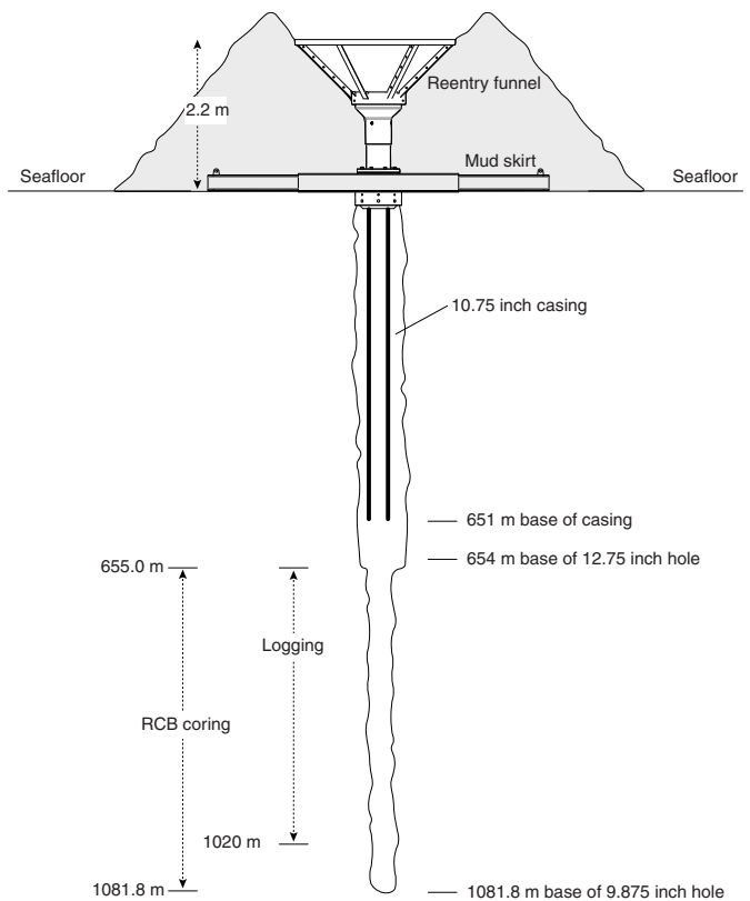
Figure F7. Hole U1499B reentry system and casing.
