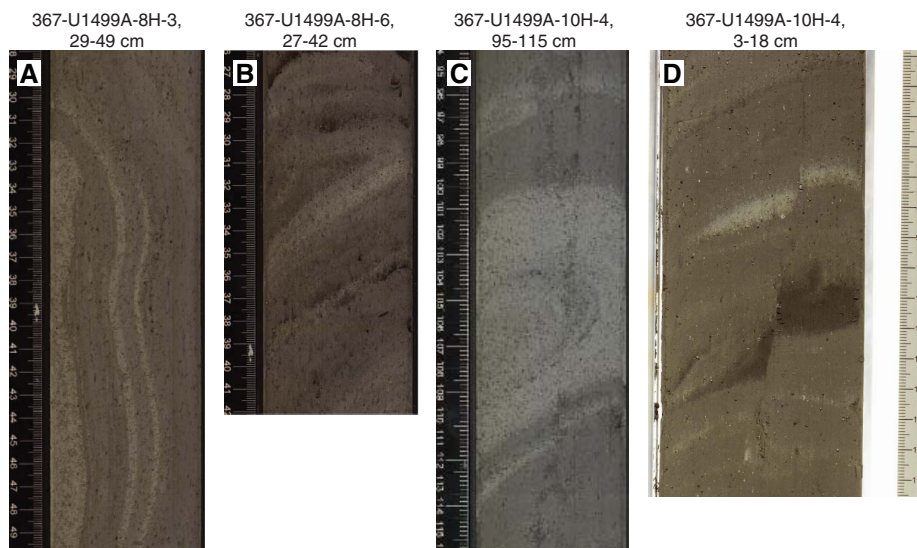
Figure F32. Structures in Unit II, Hole U1499A. A. Contorted subvertical beds. B. Centimeter-scale synsedimentary fold. C. Synsedimentary fold. D. Normal subvertical fault.
