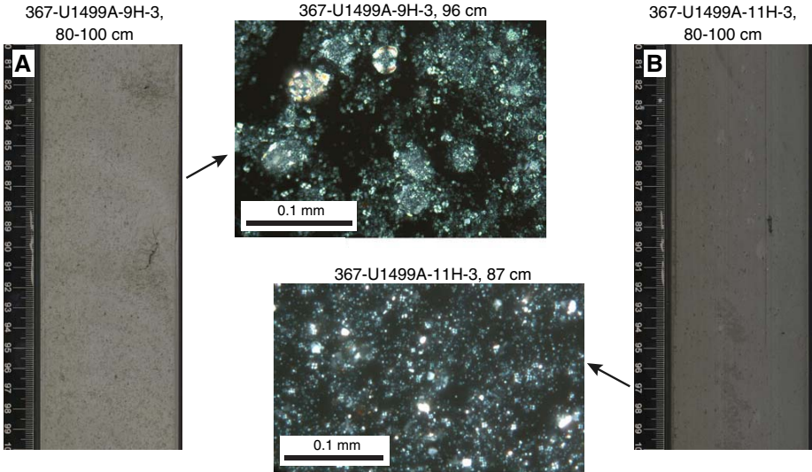
Figure F13. (A) Greenish gray clay-rich calcareous ooze and (B) dark greenish gray nannofossil-rich clay showing abundant foraminifers and nannofossils (cross-polarized light [XPL]), Unit II.
