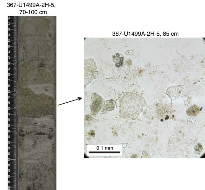
Figure F11. Dark greenish gray bioclast-rich clay of Unit I, consisting mainly of silty terrigenous clay with mixed biogenic grains, including foraminifers, nannofossils, radiolarians, and diatoms.
