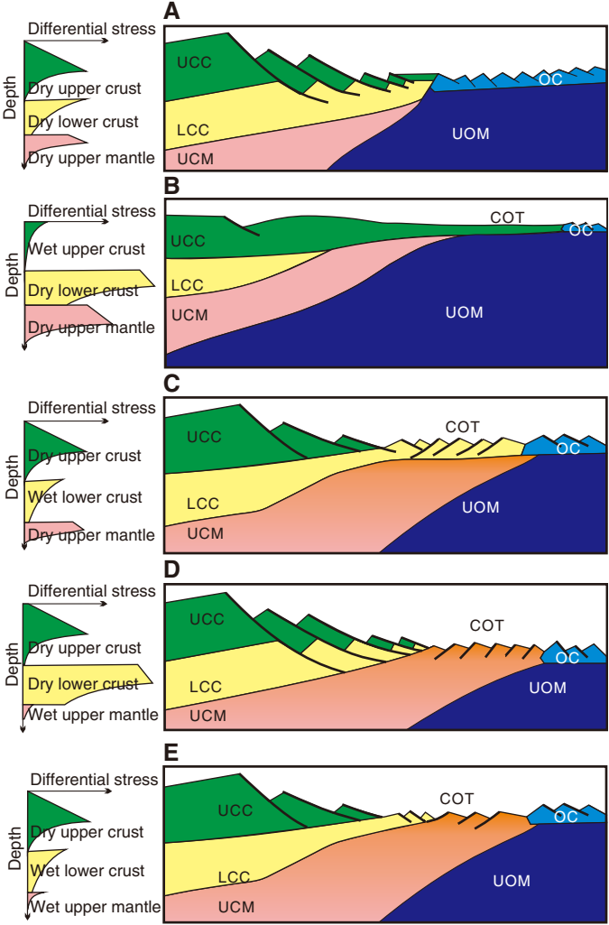
Figure F6. A–E. Composite figures redrawn from models in Huismans and Beaumont (2011), Sibuet and Tucholke (2012), Makris et al. (2012), and Sun et al. (2016) showing spectrum of possible magma-poor rifted margin models based on rheological differences. These models suggest that lithospheric layers with relatively lower strength will tend to stretch and thin more than other layers. Thus, the continent–ocean transition (COT) may be dominated by these weaker layers. D features a strong lower crust overlying a weak, wet upper mantle, resulting in upper subcontinental (serpentinized) mantle dominating the COT. C shows a particularly interesting alternative in which moderately weaker lower crust leads to its exhumation in the COT. UCC = upper continental crust, LCC = lower continental crust, UCM = upper continental mantle, UOM = upper oceanic mantle, OC = oceanic crust.
