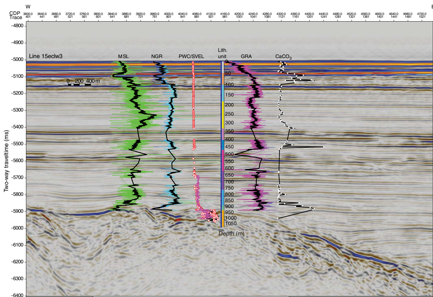
Figure F64. Seismic section across Site U1499 using alternative TDRs with an increase in velocity (blue line in Figure F62). Site is located at lithostratigraphic unit plot (see Figure F60). Other Site U1499 data are offset from site location: MSL, NGR, PWC velocity and VSI shear velocity logging data, GRA density, and \text{CaCO}_3 content.
