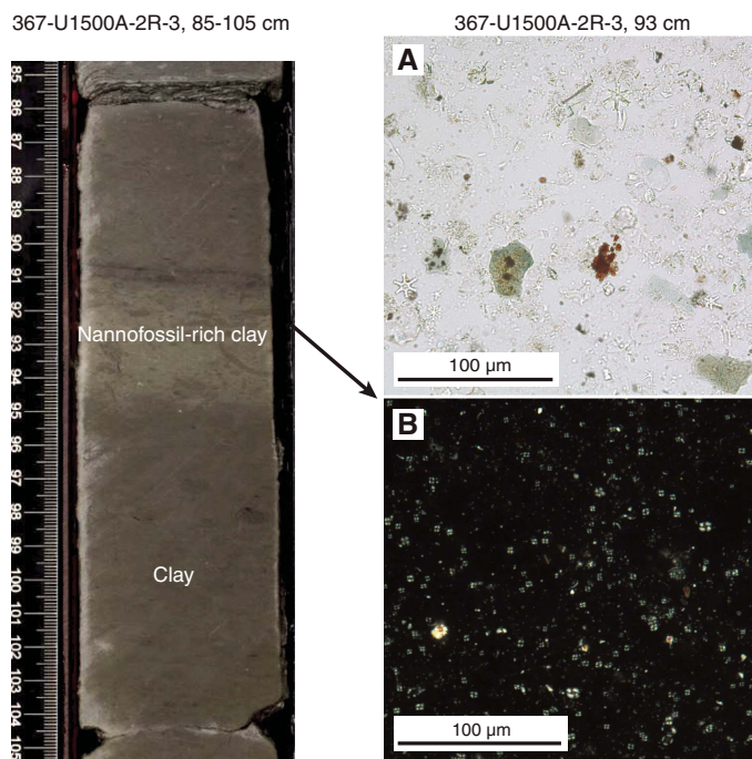
Figure F14. Heavily bioturbated nanofossil-rich clay between two darker clay intervals, Unit I. Abundant (A) discoasters (plane-polarized light [PPL]) and (B) coccolithophores (cross-polarized light [XPL]).
