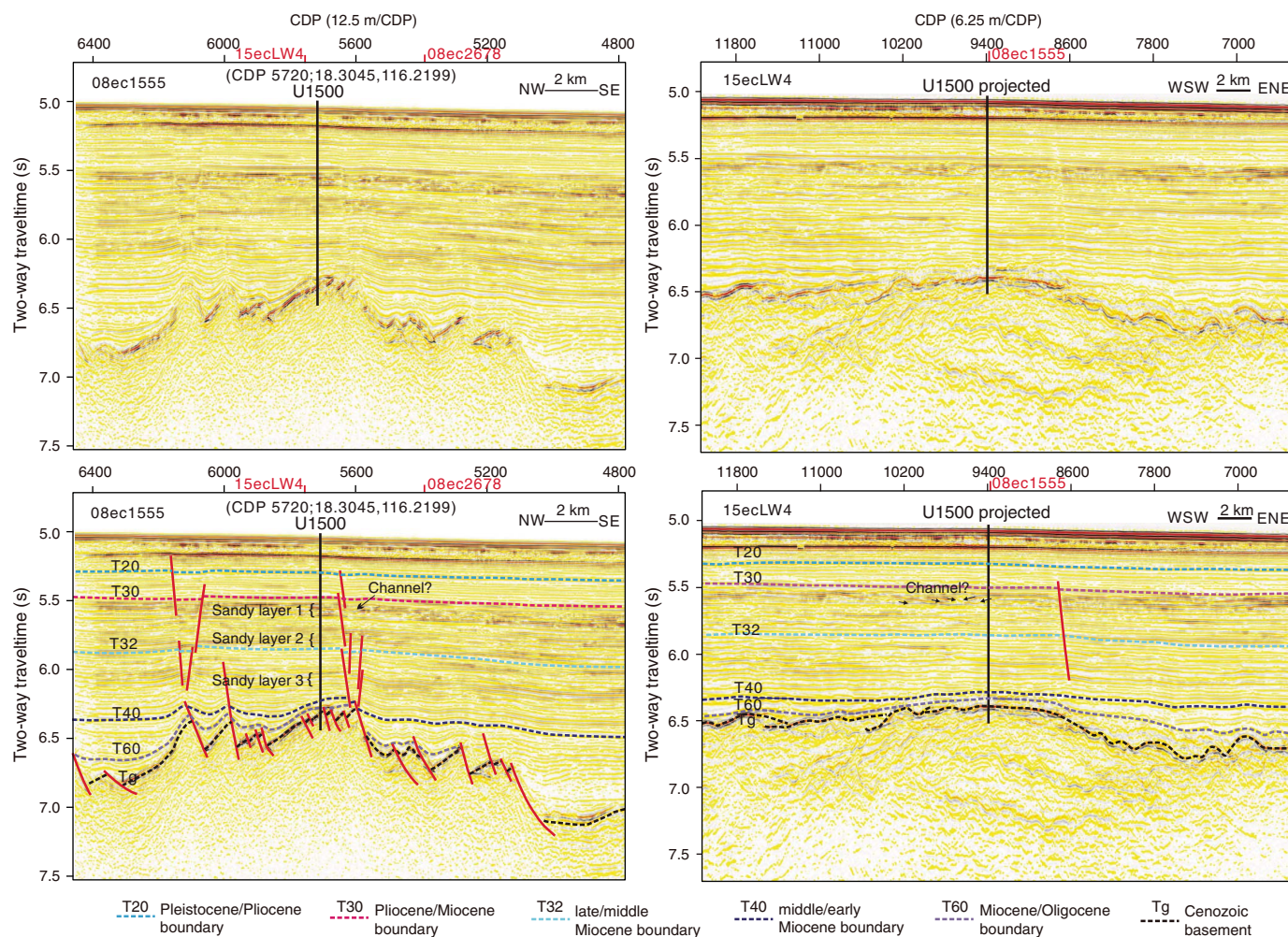
Figure F4. Original and interpreted multichannel seismic reflection profiles across Site U1500. Site U1500 is located on seismic Profile 08ec1555 and projected 75 m onto seismic Profile 15ecLW4. Red text and tick marks = locations of crossing seismic lines, red lines = faults interpreted from the seismic data. CDP = common depth point. All seismic profiles are courtesy of the Chinese National Offshore Oil Corporation [CNOOC].
