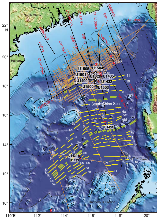
Figure F1. Seismic data coverage and magnetic anomalies of the SCS Basin, Expeditions 367 and 368. Black lines = ocean-bottom seismometer refraction data. Other seismic lines are mostly multichannel seismic reflection data. White stars = Expedition 367/368 sites, red squares = Leg 184 sites, red circles = Expedition 349 sites. For more detail, see Figure F2.
