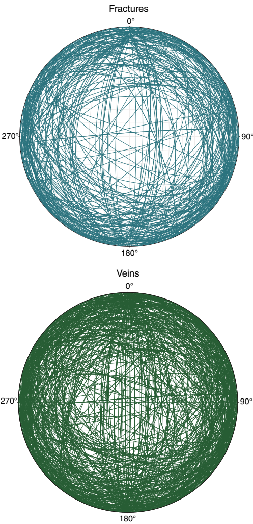
Figure F34. Stereographic projection of Unit VIII fractures and veins in core reference frame, Site U1500. Note random orientations of the fractures and veins.
