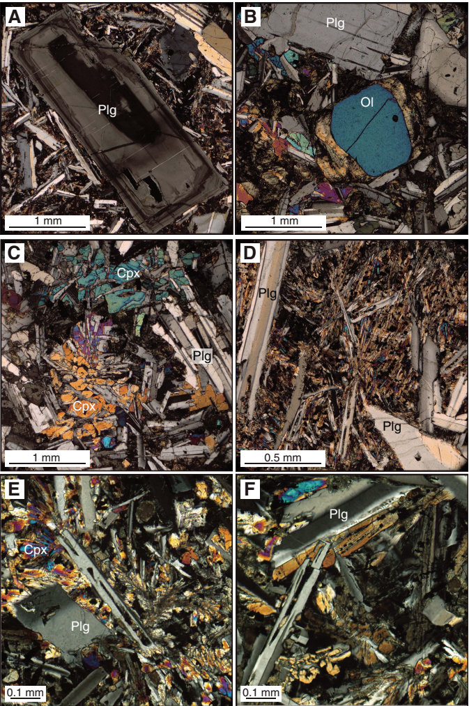
Figure F28. Representative primary rock-forming minerals and textures of basalts, Hole U1500B (XPL). A. Subhedral to euhedral plagioclase phenocrysts (Plg) found throughout Unit VIII basalts show resorption textures, inherited cores, and oscillatory zoning (59R-1, 67–70 cm). B. Olivine phenocryst (Ol) (59R-5, 112–114 cm). C. Subophitic texture showing poikilitic clinopyroxene (Cpx) enclosing laths of plagioclase (59R-5, 112–114 cm). D. Quenched texture showing plagioclase phenocrysts within radially oriented, dendritic intergrowths of plagioclase and clinopyroxene (59R-1, 67–70 cm). E. Intersertal texture in groundmass showing swallow-tail plagioclase with radially oriented, dendritic clinopyroxene (60R-4, 135–138 cm). F. Intersertal texture of swallow-tail plagioclase and comb-texture clinopyroxene with altered interstitial glass (60R-4, 135–138 cm).
