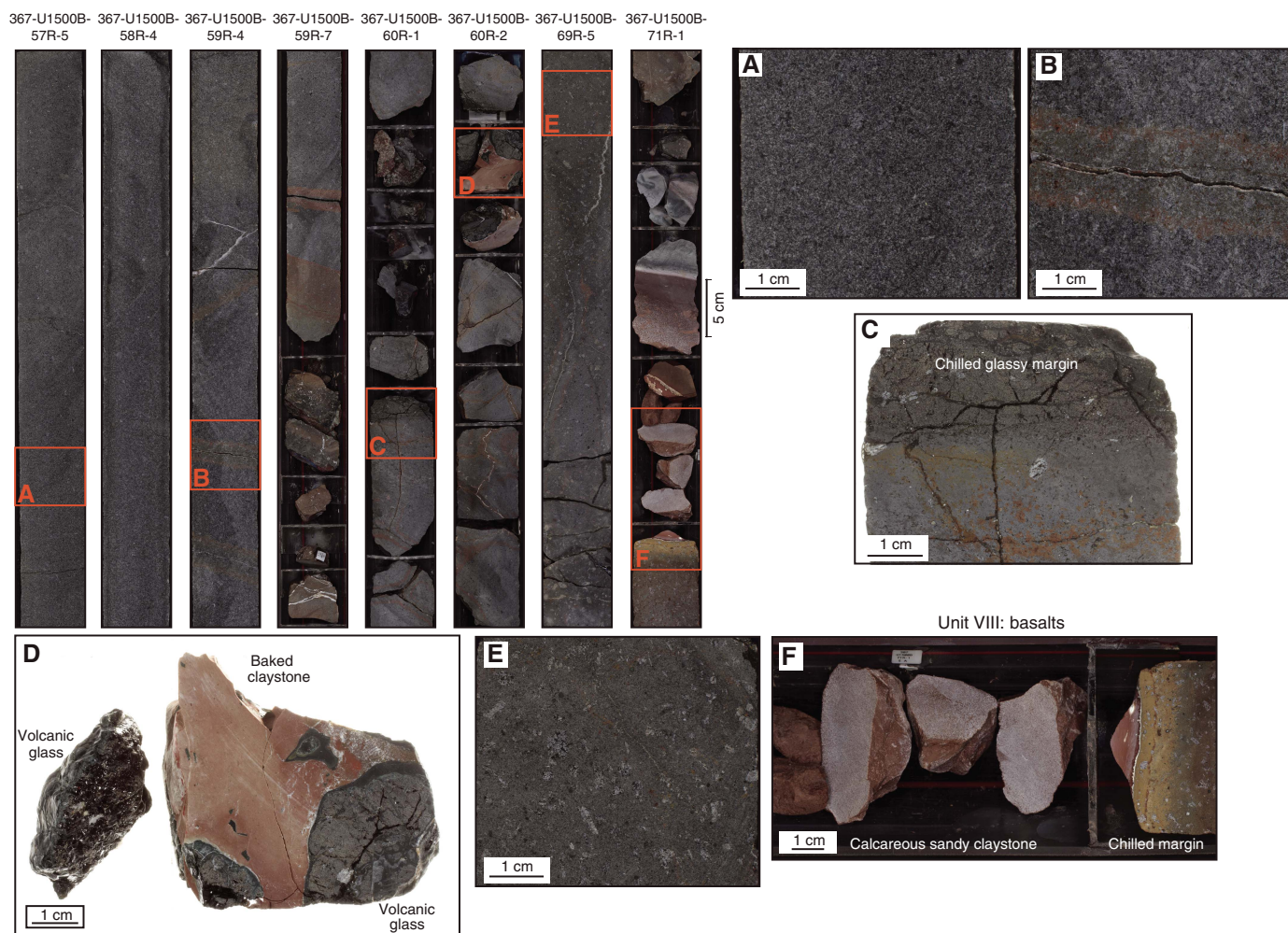
Figure F24. Homogeneous sparsely vesicular and sparsely to moderately plagioclase phyric basalts spanning 27 m in Hole U1500B interspersed with minor chilled margins (from left to right: 57R-5, 0–50 cm, 58R-4, 0–50 cm, 59R-4, 60–110 cm, and 59R-7, 30–90 cm), grading downhole into moderately to highly plagioclase phyric basalts with a higher abundance of glassy chilled margins and baked sediments (pillow lava flows; from left to right: 60R-1, 60–110 cm, 60R-2, 0–50 cm, 69R-5, 1–50 cm, and 71R-1, 75–125 cm). A. Sparsely plagioclase phyric basalt with sparse vesicularity (57R-5, 33–38 cm). B. Haloed vein containing carbonates and Fe (hydr)oxides with 2 cm thick alteration halo (59R-4, 91–96 cm). Alteration of host basalt is predominantly focused on groundmass alteration of glass to low-temperature green-yellow alteration minerals (e.g., zeolites or chlorite) and localized replacement of plagioclase by carbonate. C. Upper rim of sample with a black glassy chilled margin grading into aphyric basalt (dark gray) and a joint perpendicular to the glassy margin (60R-1, 90–95 cm). D. Hyaloclastite with mixing of rounded to angular quenched basaltic glass shards with baked claystone (69R-5, 6–13 cm). E. Highly plagioclase phyric basalt with sparse vesicles (69R-5, 4–9 cm). F. Basaltic chilled margin with a sharp contact to a baked reddish calcareous sandy claystone (top of section to the left; 71R-1, 106–120 cm).
