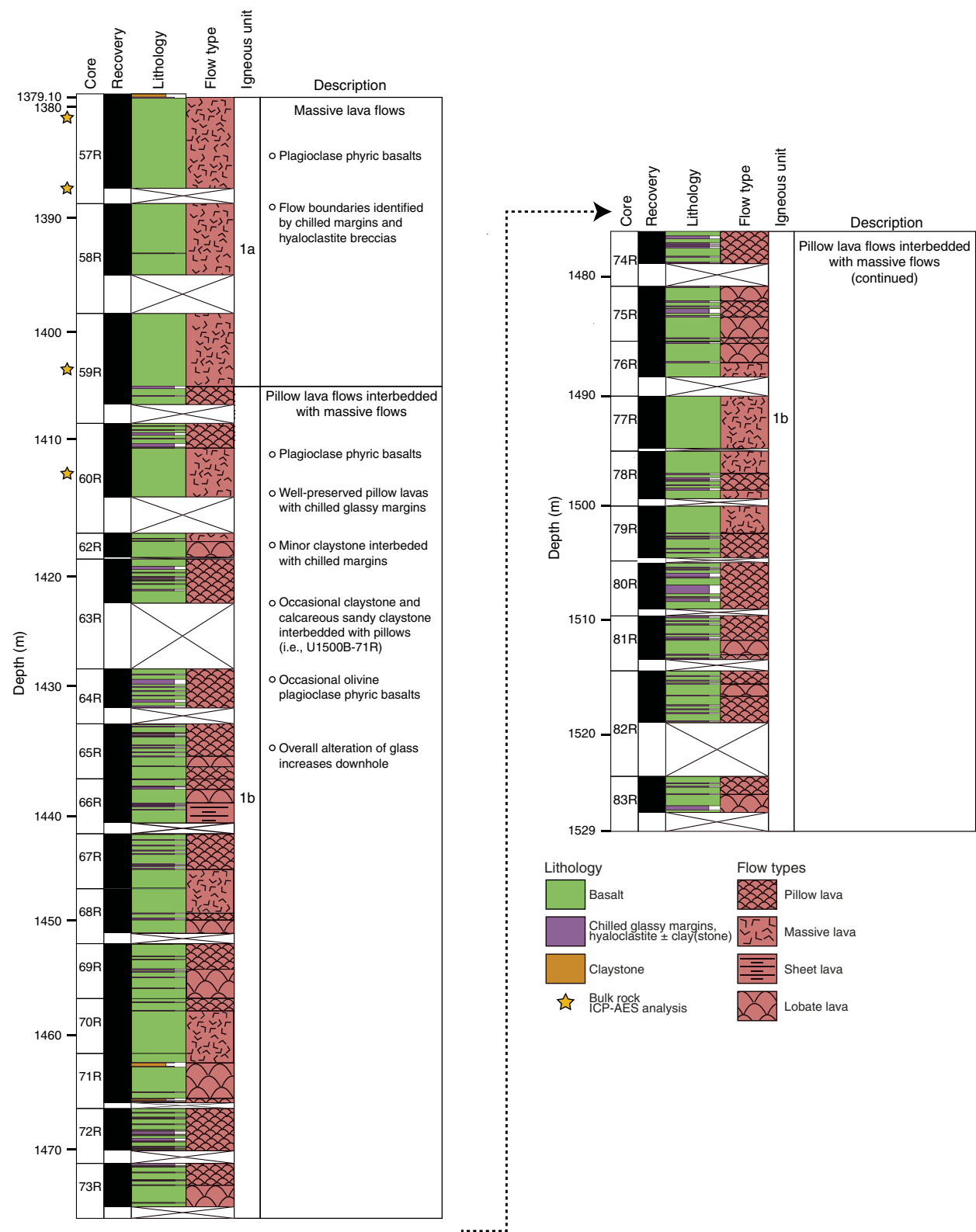
Figure F23. Lithostratigraphic summary of Unit VIII basalts showing lithology, lava flow types, and igneous Subunits 1a and 1b, Hole U1500B.
