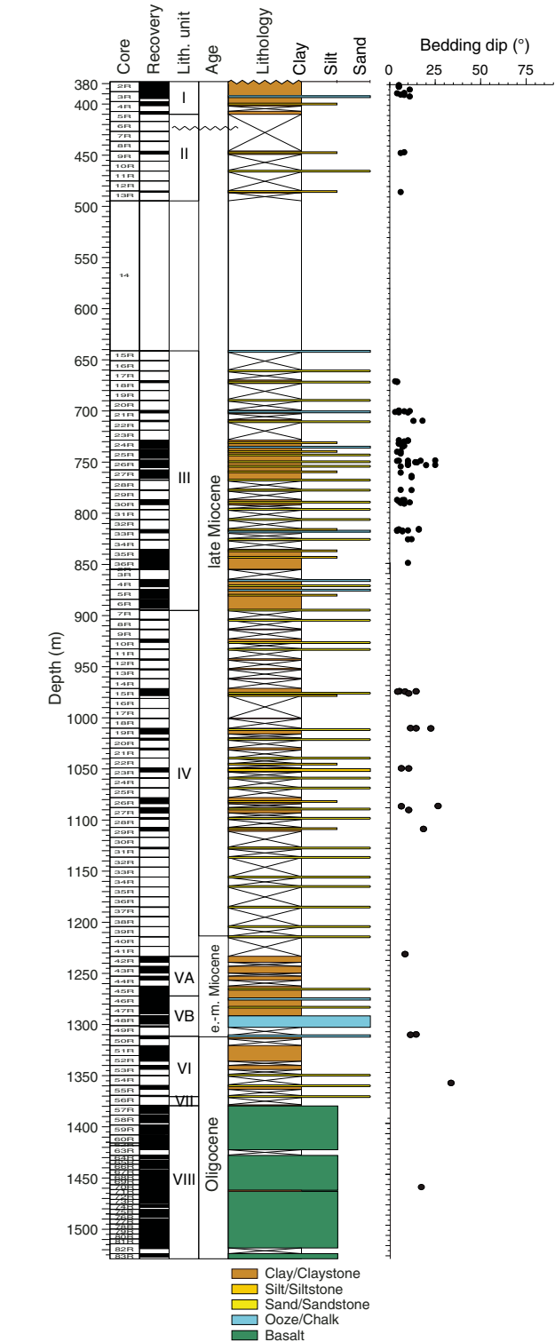
Figure F29. Lithostratigraphic summary with bedding dips, Site U1500.
