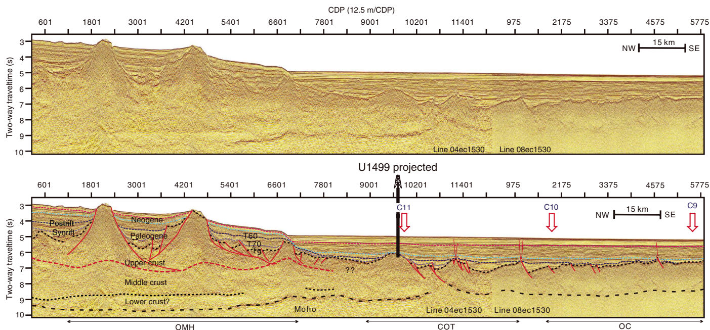
Figure F9. Uninterpreted and simplified interpretation of seismic Profile 1530. Note the presence of reflectors interpreted as major detachment faults that seem to sole out between the upper and middle/lower crust in the outer margin high. Location of ocean floor magnetic lineations C11n to C9n are projected from maps in Figure F2B.
