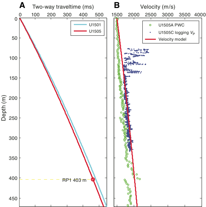
Figure F38. A. Site U1505 TDR curve compared to Site U1501 TDR curve. Red circle = reference Point RP1 at 403 m, which coincides with noticeable changes in density and velocity. B. Hole U1505C PWC, logging V_p , and calculated interval velocity model from TDR model.
