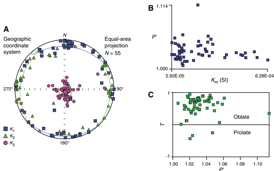
Figure F20. AMS data, Hole U1505C. A. Stereonet of AMS principal directions (lower hemisphere, equal-area projection). K_1 = maximum axis, K_2 = intermediate axis; K_3 = minimum axis. Confidence ellipses at 95% level (same color convention) show dominantly planar and subhorizontal fabric (oblate), consistent with sedimentary fabric acquired in a calm pelagic environment. Tensorial means are shown with larger symbols of same color. B. Degree of magnetic anisotropy ( P' ) vs. magnetic susceptibility ( K_m ). C. Shape parameter ( T ) vs. P' showing dominantly oblate symmetry of sedimentary fabric.
