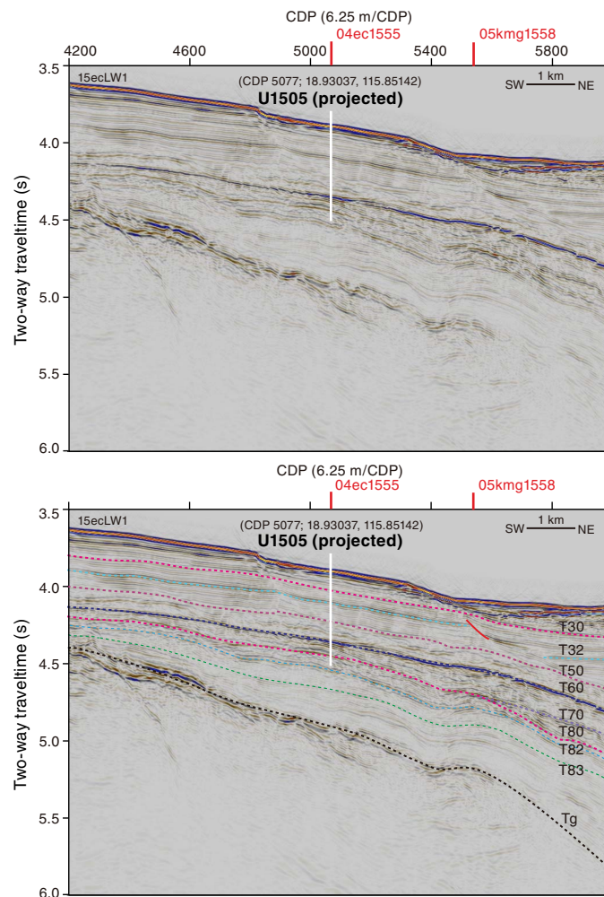
Figure F5. Site U1505 location and penetration depth on seismic dip Line 15ecLW1 (original predrilling interpretation). Seismic stratigraphic T30 (5.3 Ma), T32 (10.0 Ma), T50 (19.1 Ma), T60 (23.0 Ma), T80 (38.0 Ma), T82 (unknown age), and T83 (unknown age) unconformities and acoustic basement Tg reflector are shown (for inferred predrilling ages, see Seismic stratigraphic framework in the Expedition 367/368 methods chapter [Sun et al., 2018]).
