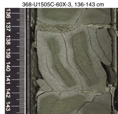
Figure F15. Deformation structures made of en echelon millimeter-scale normal faults and fractures, Unit II. Structures resemble those observed in Subunit IIA at Site U1501 (see Figure F27 in the Site U1501 chapter [Larsen et al., 2018a]).
