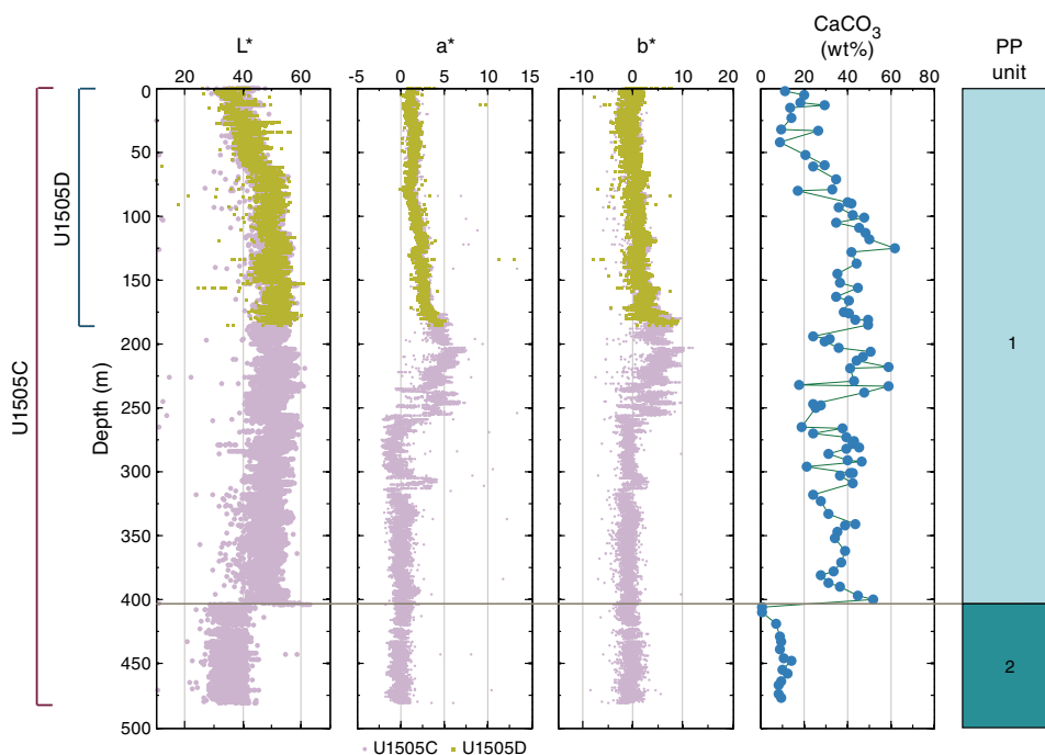
Figure F30. Sediment color reflectance parameters L^* , a^* , and b^* for Holes U1505C and U1505D and \text{CaCO}_3 content for Hole U1505C (see Geochemistry).
