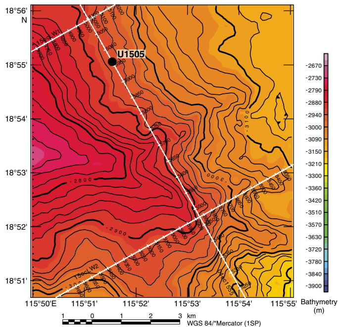
Figure F1. Bathymetry with seismic lines, Site U1505. Note that the site is not at the exact crossing of seismic Lines 04ec1555 and 15ecLW1. Seismic profiles across Site U1505 are shown in Figures F5 and F6. Common depth point (CDP) numbers are shown along seismic lines.
