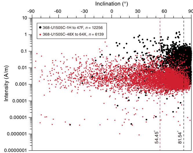
Figure F19. Magnetic measurements, Hole U1505C. Inclination was used to determine polarity. AFD = AF demagnetization. Magnetostratigraphic features are referred to as n1, etc., in a sequential manner for convenience and have no bearing on chrons. Discrete samples are yellow and green. GPTS2016 = geomagnetic polarity timescale of Ogg et al. (2016).
