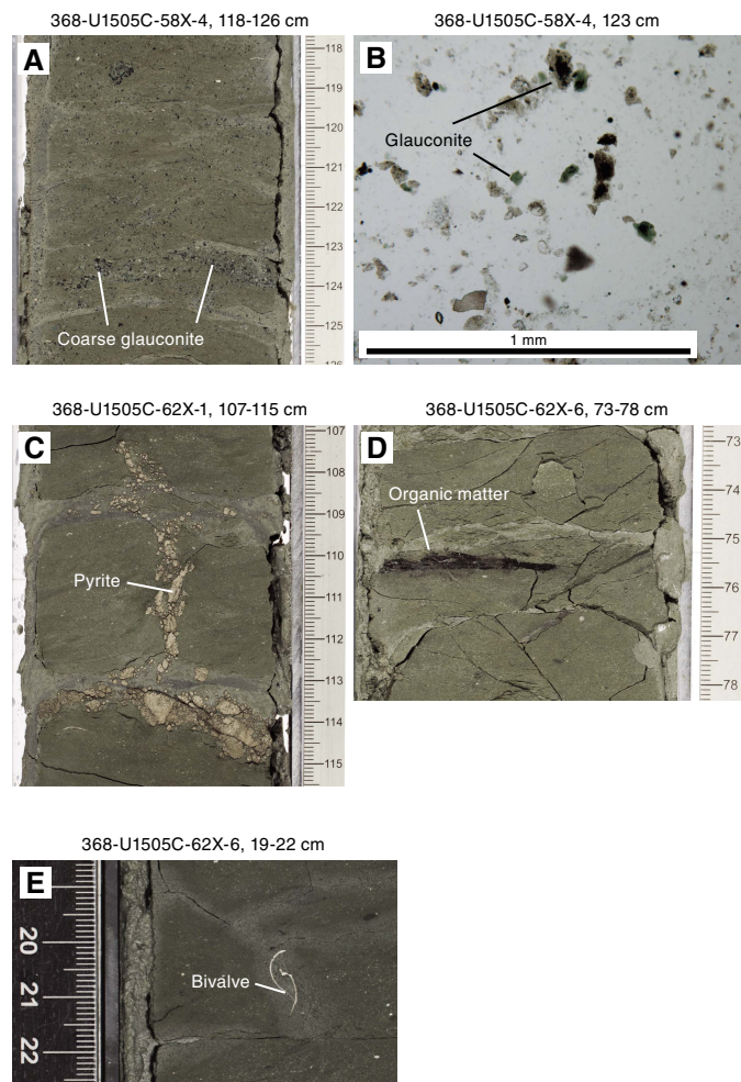
Figure F14. Special features in Unit II. A. Thick lamination rich in glauconite grains interbedded with dark greenish gray silty clay with disseminated glauconite. B. Glauconite grains in silty clay. C. Diagenetic pyrite grains possibly replacing a burrow fill and lamination in heavily bioturbated nannofossil-rich silty clay. D. Organic matter in nannofossil-rich silty clay. E. Bivalve macrofossil in nannofossil-rich silty clay. Note the small shelly fragments on the core surface.
