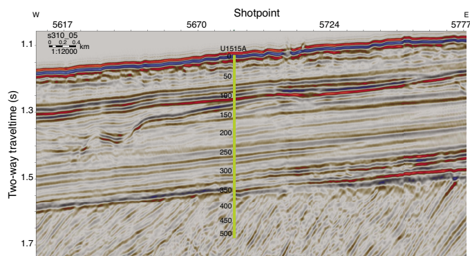
Figure F2. Time-migrated Geoscience Australia reflection seismic Profile s310_05 with location of Site U1515 along seismic shotpoints.
