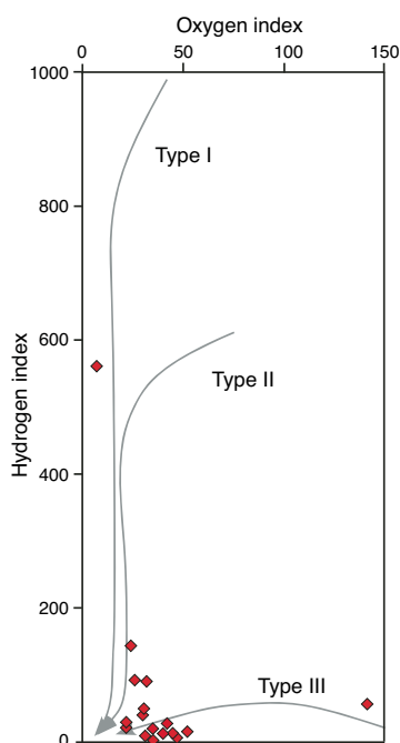
Figure F17. Source rock analysis (pyrolysis) results, Site U1515. Data from duplicate samples are not plotted.
