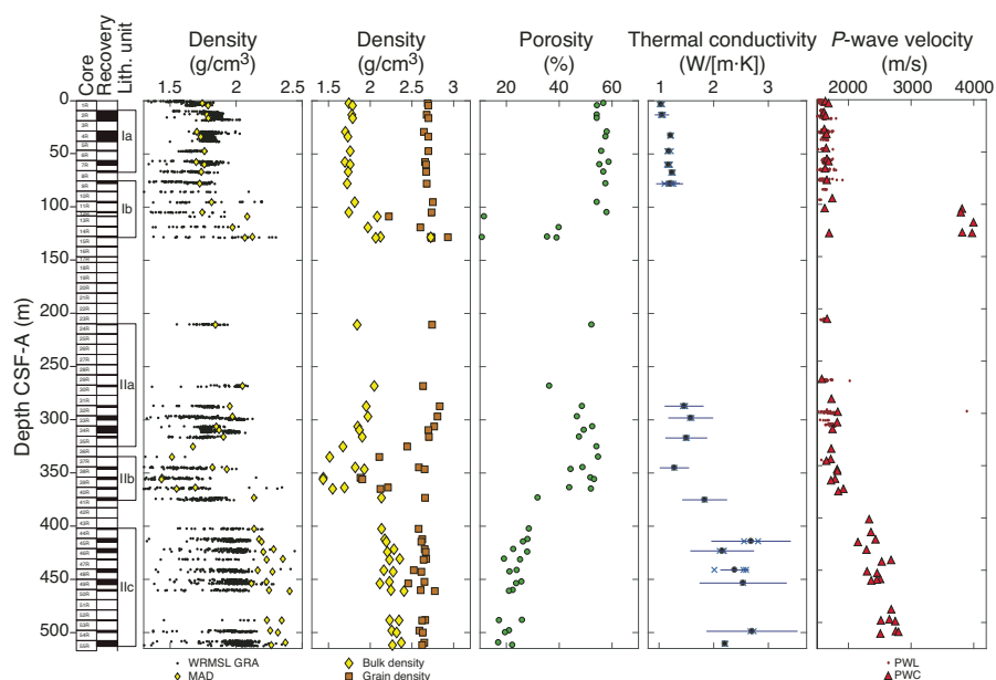
Figure F14. Density, porosity, thermal conductivity (bars = 1σ standard deviation), and P-wave velocity, Hole U1515A.
