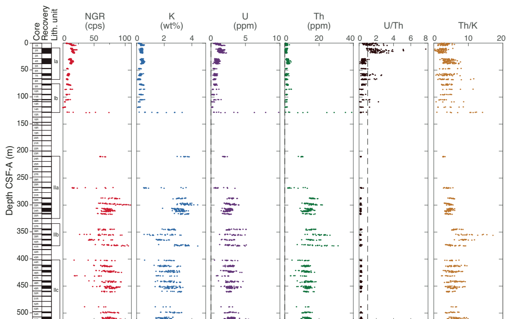
Figure F13. Whole-core NGR data, Hole U1515A. U/Th ratio: vertical dashed line = 1/1.
