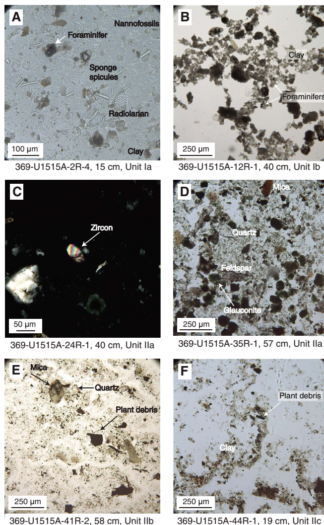
Figure F5. Sediment constituents in Subunits Ia, Ib, and IIa–IIc, Hole U1515A. A. Calcareous ooze with radiolarians and sponge spicules (plane-polarized light [PPL]). B. Calcareous chalk with clay (PPL). C. Zircon (cross-polarized light [XPL]). D. Glauconitic silty sandstone (PPL). E. Siltstone (PPL). F. Siltstone with clay (PPL).
