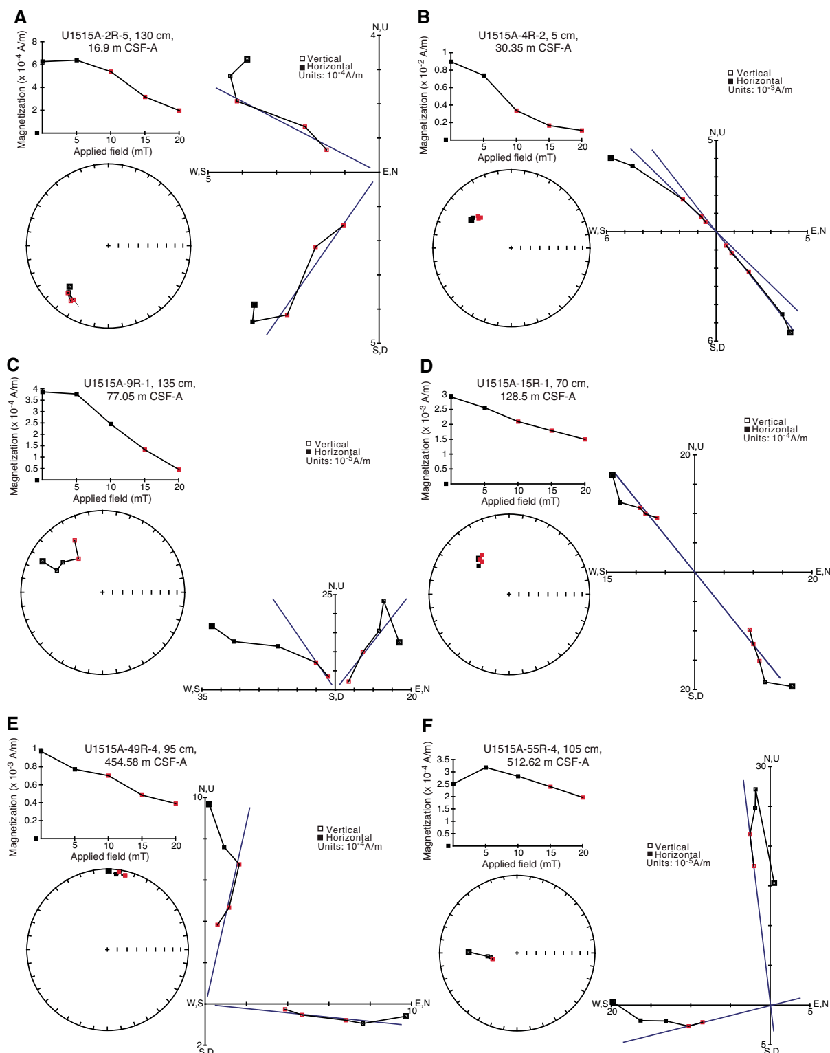
Figure F9. Vector endpoint diagrams (Zijderveld, 1967) of section halves, Hole U1515A.
