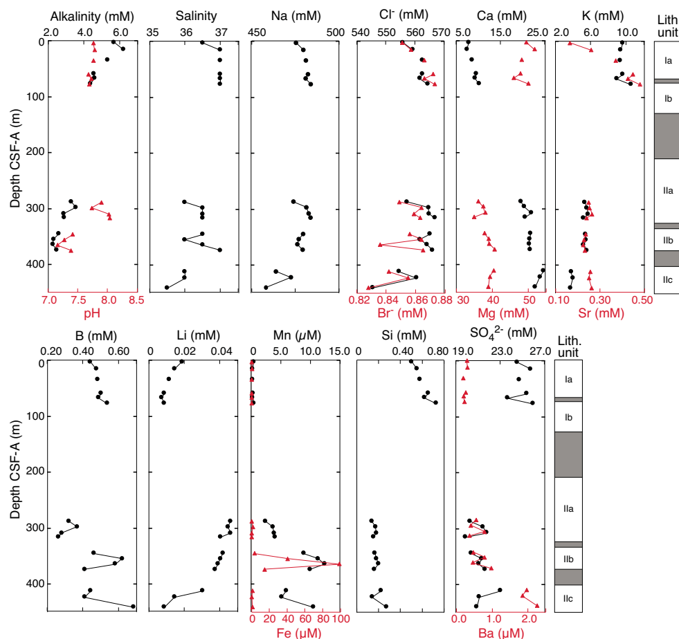
Figure F15. Interstitial water alkalinity, pH, and element and ion concentrations, Site U1515. Lith. unit: shaded areas = no or exceedingly low recovery.
