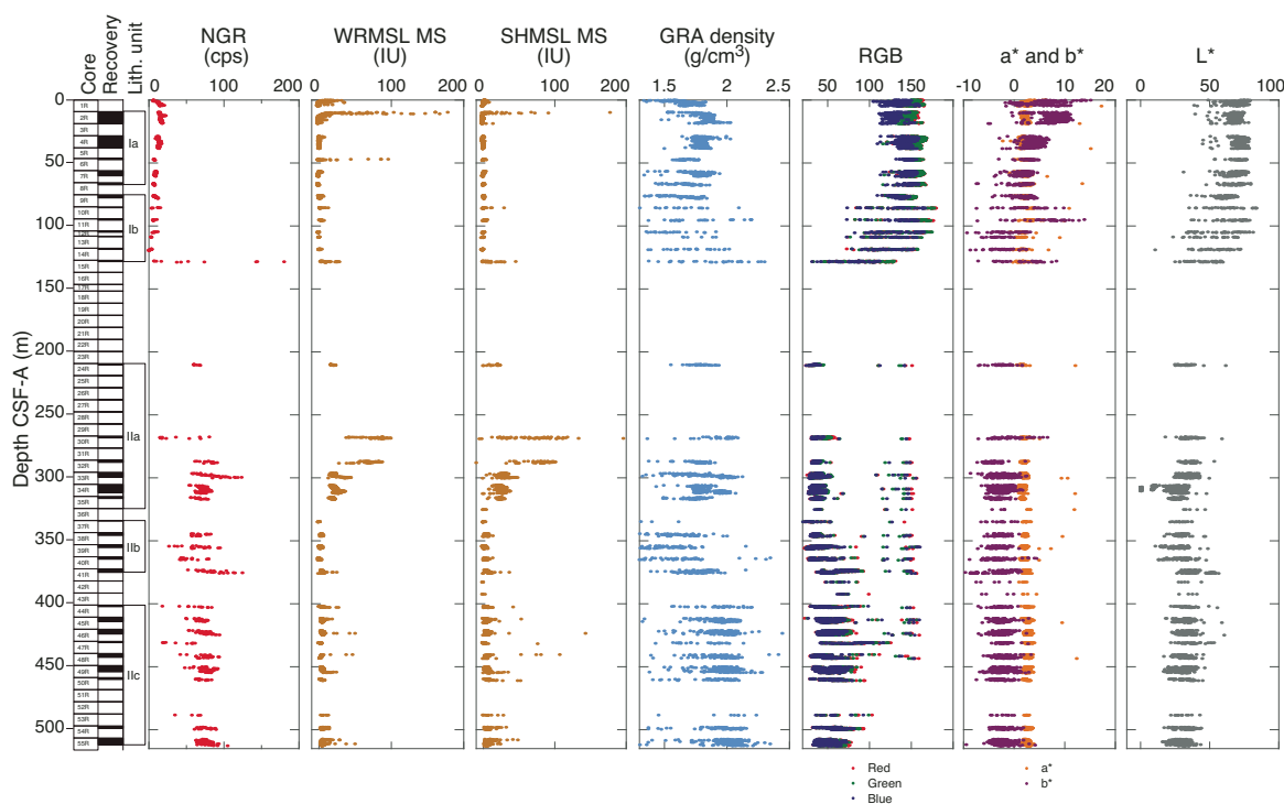
Figure F12. Whole-core physical properties, Hole U1515A.
