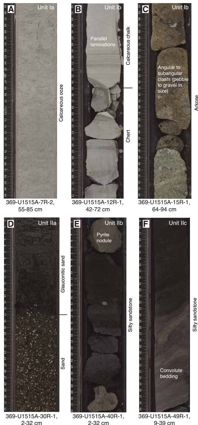
Figure F4. Primary lithologies and sedimentary features, Site U1515. A. Calcareous ooze, Subunit Ia. B. Calcareous chalk with parallel laminations and chert, Subunit Ib. C. Arkose, Subunit Ib. D. Glauconitic sand and sand, Subunit IIa. E. Pyrite nodule and silty sandstone, Subunit IIb. F. Silty sandstone with convolute bedding, Subunit IIc.
