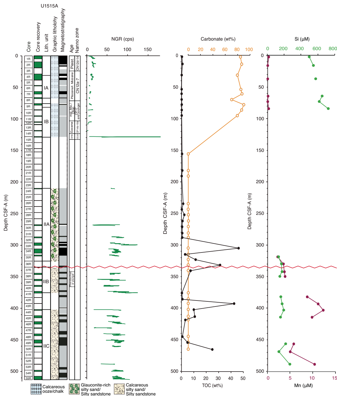
Figure F18. Site U1515 summary. Red wavy line = unconformity inferred from seismic and physical property data.
