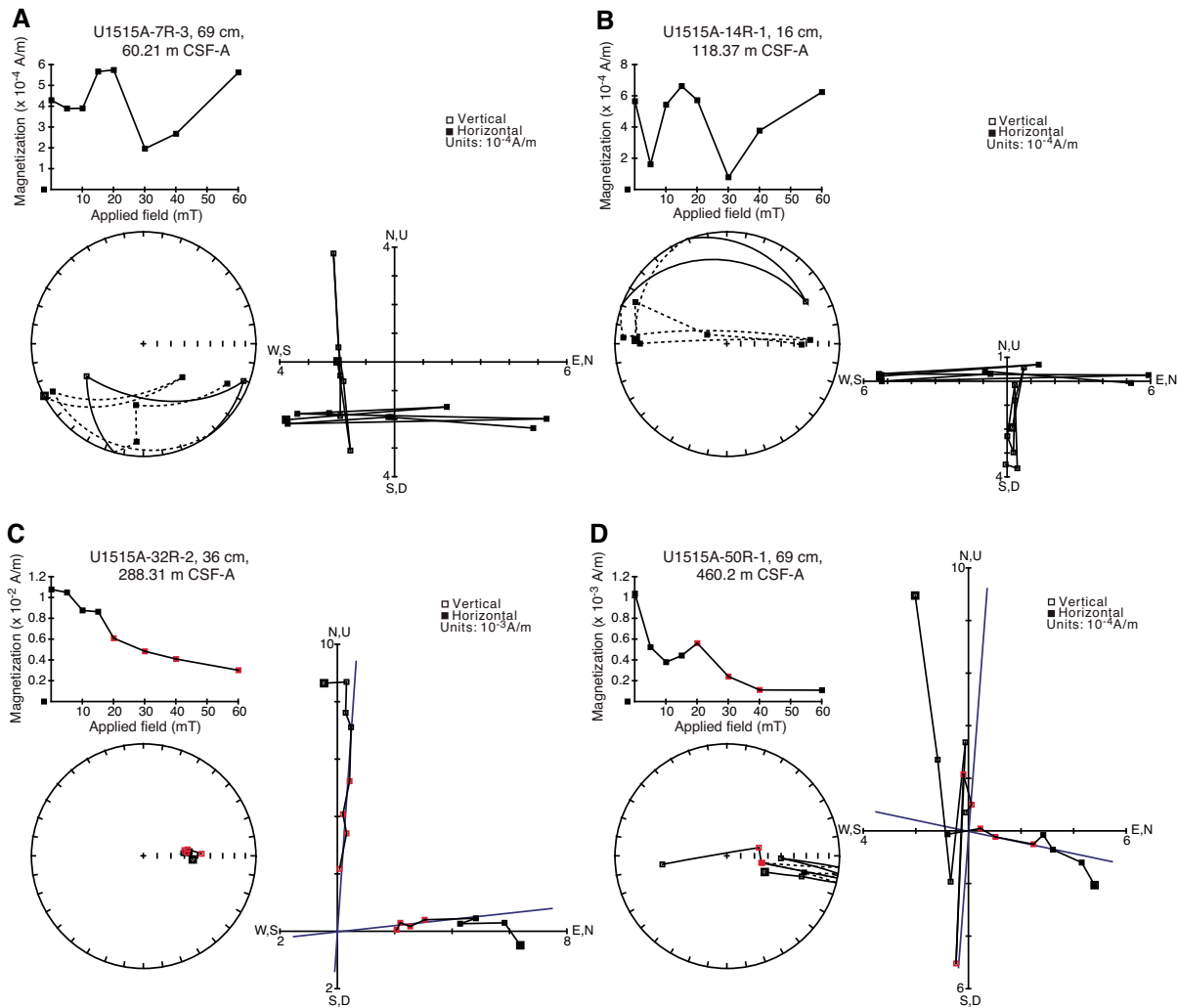
Figure F10. Vector endpoint diagrams (Zijderveld, 1967) for representative discrete samples, Hole U1515A.
