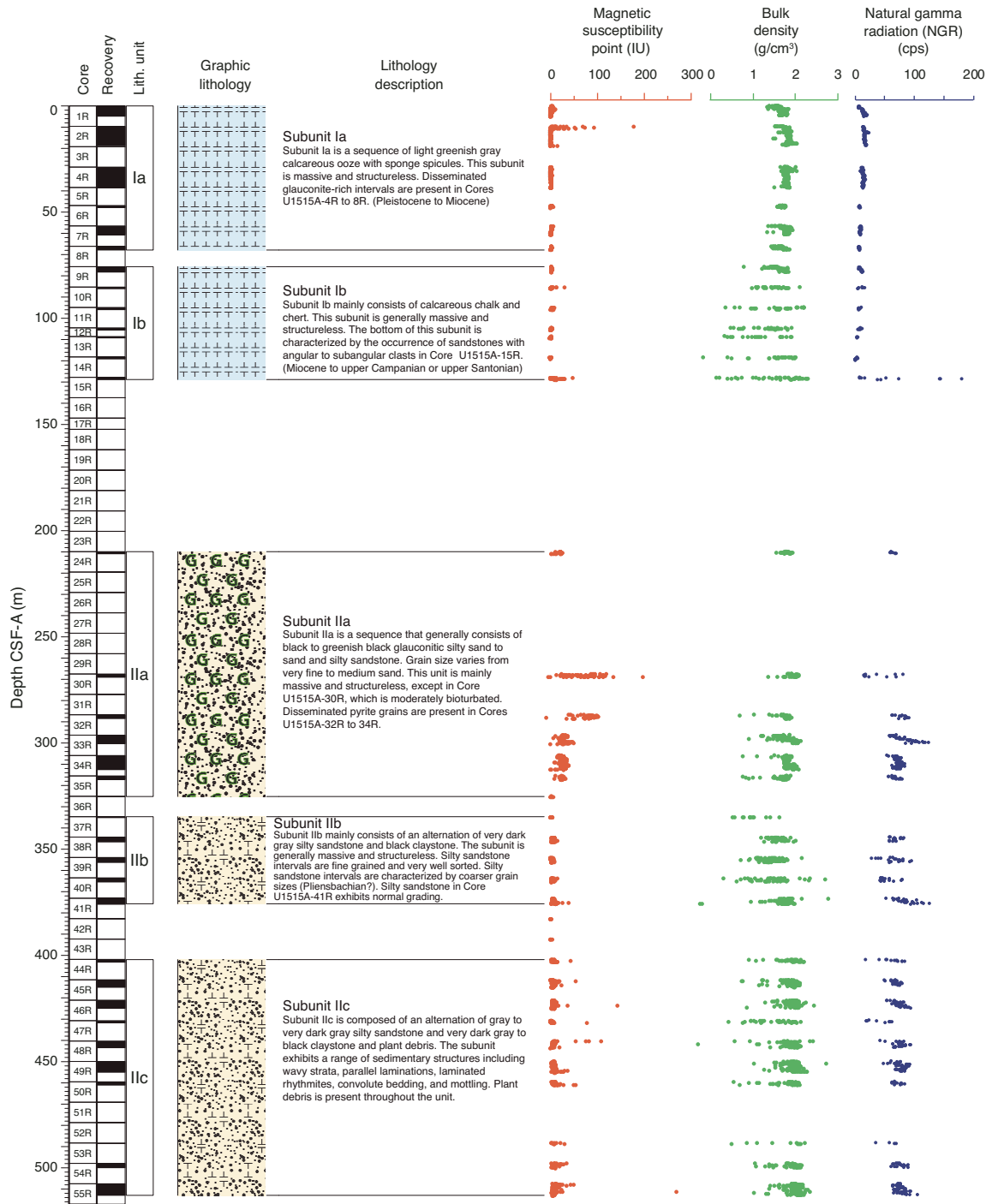
Figure F3. Lithostratigraphic summary, Site U1515.
