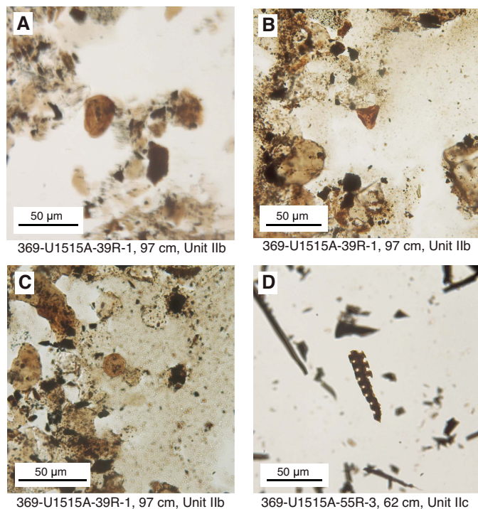
Figure F6. Characteristic plant debris and organic material in Subunits IIb and IIc, Hole U1515A (PPL). A. Jurassic spore, Contignisporites sp. (likely Contignisporites glebulentus ; Mesozoic with first occurrence in the Early Jurassic; Helby et al., 1987). B. Trilete spore, Gleicheniidites sp. (likely Gleicheniidites senonicus ; Mesozoic with first occurrence in the Early Jurassic; Helby et al., 1987). C. Algal cell, Leiosphaeridia sp. (not age diagnostic). D. Wood fragment.
