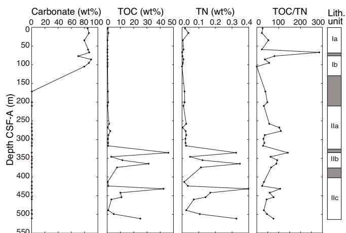
Figure F16. Carbon and total nitrogen (TN) contents and total organic carbon (TOC)/TN ratio, Site U1515. TOC and TN values are near the detection limit. Lith. unit: shaded areas = no or exceedingly low recovery.
