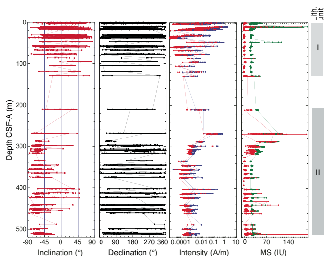
Figure F8. Paleomagnetic results, Hole U1515A. Intensity: blue = 0 mT AF demagnetization, red = 20 mT AF demagnetization. Magnetic susceptibility (MS): green = whole round (20 IU offset), red = point source.
