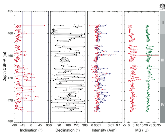
Figure F14. Paleomagnetic results, Hole U1516D. Intensity: blue = 0 mT AF demagnetization, red = 20 mT AF demagnetization. MS: green = whole round (20 IU offset), red = point source.
