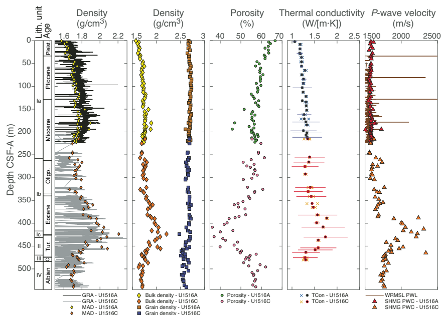
Figure F25. Density, porosity, thermal conductivity (bars = 1 \sigma standard deviation), and P -wave velocity, Site U1516.
