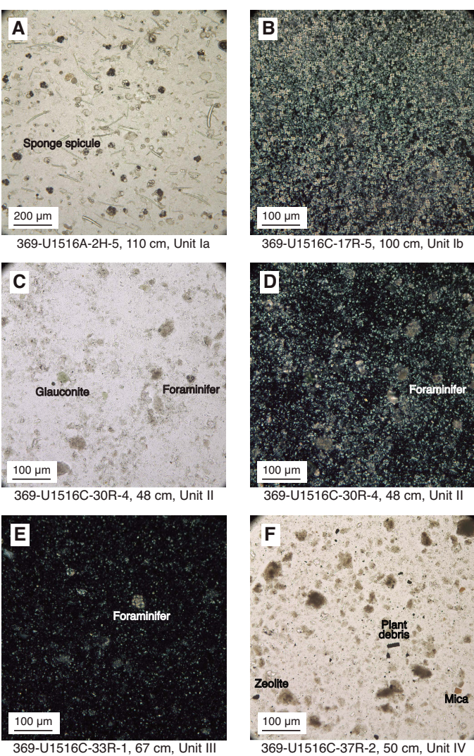
Figure F5. Sediment constituents in Units I–IV, Holes U1516A and U1516C. A. Calcareous ooze with sponge spicules (plane-polarized light [PPL]). B–D. Nanofossil chalk with (B) sponge spicules (cross-polarized light [XPL]) and clay; (C) PPL, (D) XPL. E. Clayey nanofossil chalk (XPL). F. Claystone with nanofossils (PPL).
