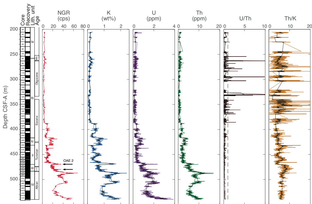
Figure F23. NGR data, Hole U1516C. U/Th ratio: vertical dashed line = 1:1 ratio. Black arrows = peaks that correspond to OAE 2 and possible MCE.
