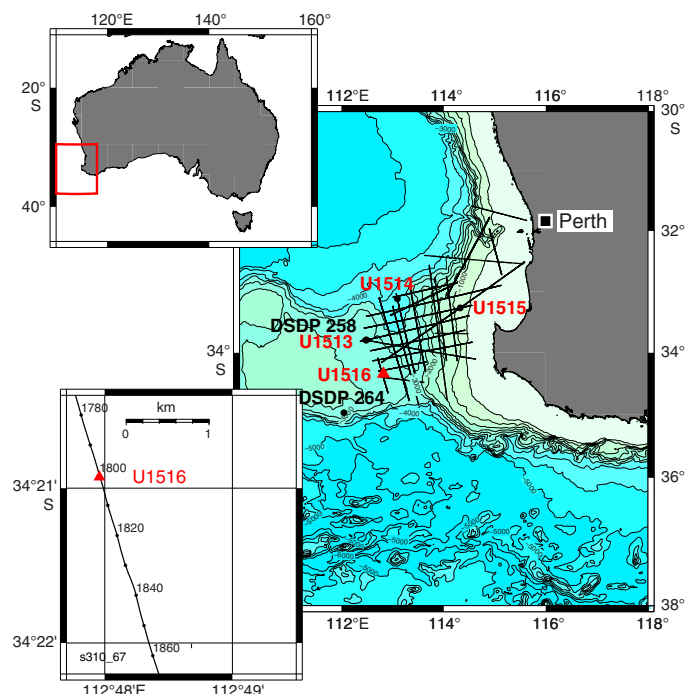
Figure F1. Location of Site U1516 on the western margin of the Mentelle Basin.
