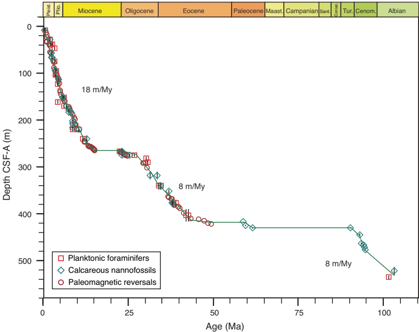
Figure F8. Age-depth plot, Site U1516. Vertical bars = depth uncertainty on events (see Tables T5 and T6 for values). Age estimates are from Gradstein et al. (2012).
