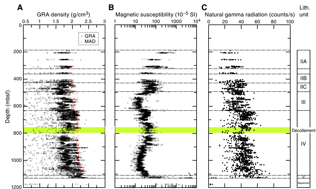
Figure F38. MSCL-W measurements, Hole C0023A. A. GRA density. B. Magnetic susceptibility. C. NGR.
