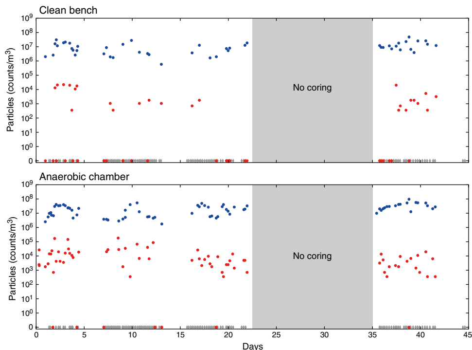
Figure F56. Monitoring of airborne contamination potential during microbiology sample processing on the Chikyu core processing deck, particle counts in 0.3 \mu\text{m} size fraction during coring operations of Expedition 370. Top: Clean bench with air filtration system and ionizer compared to microbiology laboratory. Bottom: Anaerobic chamber with air filtration system and ionizer compared to core processing laboratory. Blue = laboratory air, red = clean bench or anaerobic chamber air, gray diamonds (x-axes) = time of "core on deck."
