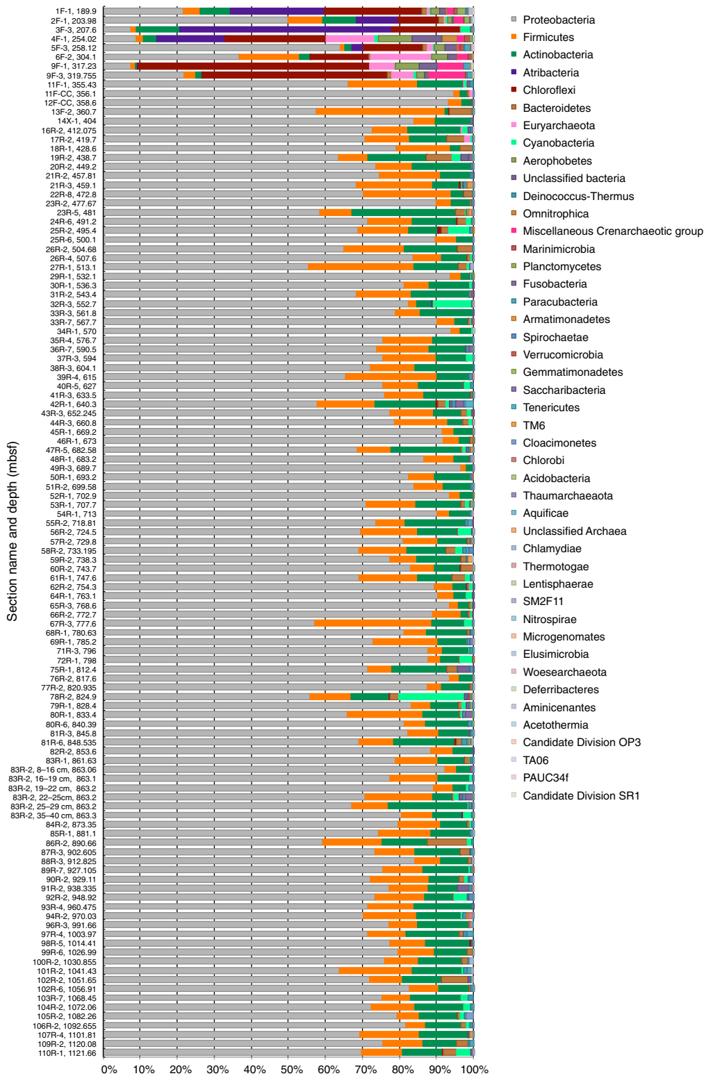
Figure F62. Phylum-level microbial composition of sediments, Site C0023. Hypervariable Region V3–V4 of 16S rRNA gene was amplified and sequenced by MiSeq sequencing. In total, 10,327,751 sequences were obtained from 115 sediment samples (for detailed sample information, see Table T29).
