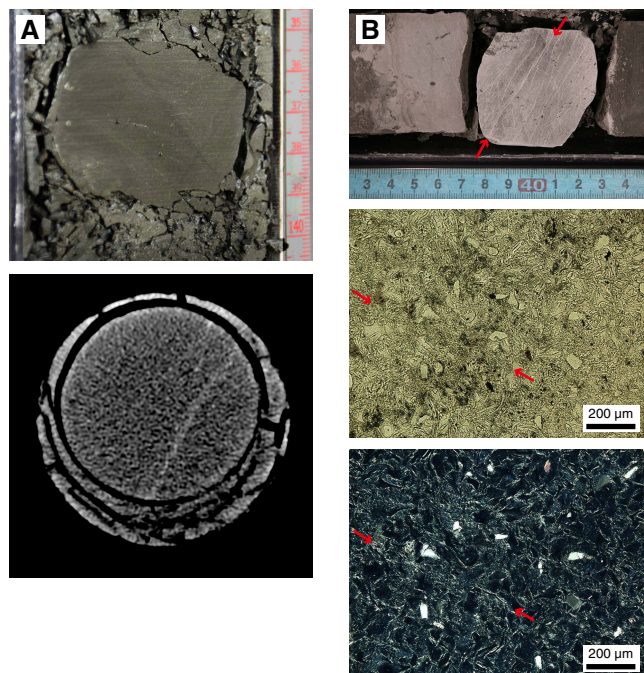
Figure F25. Occurrence of deformation bands. A. Mudstone (C0023A-7X-5, 135–140 cm [~311 mbsf]); top: photograph of split core surface, bottom: X-ray CT image. Deformation band corresponds to higher CT number, indicative that consolidation occurred along the band. B. Volcanic ash (35R-2, 32–45 cm [~575 mbsf]); top: photograph of split core surface, middle: PPL photomicrograph, bottom: crossed nicols. Arrows = position and direction of deformation band. No grain breakages occurred along the band.
