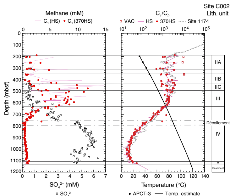
Figure F55. Depth profiles of dissolved sulfate concentrations (see Inorganic geochemistry and Figure F47), dissolved methane concentrations, and C_1/C_2 molar ratios, Hole C0023A. Hydrocarbon gas data are from core catcher headspace samples (HS) and vacutainer samples from gas voids (VAC) taken in core cutting area and from headspace sample COMGAS WRC slices (370HS) taken on core processing deck. Hole C0023A measured (APCT-3) and estimated in situ temperatures were adopted from Figure F44. Site 1174 C_1/C_2 depth profile is shown for comparison (Shipboard Scientific Party, 2001b).
