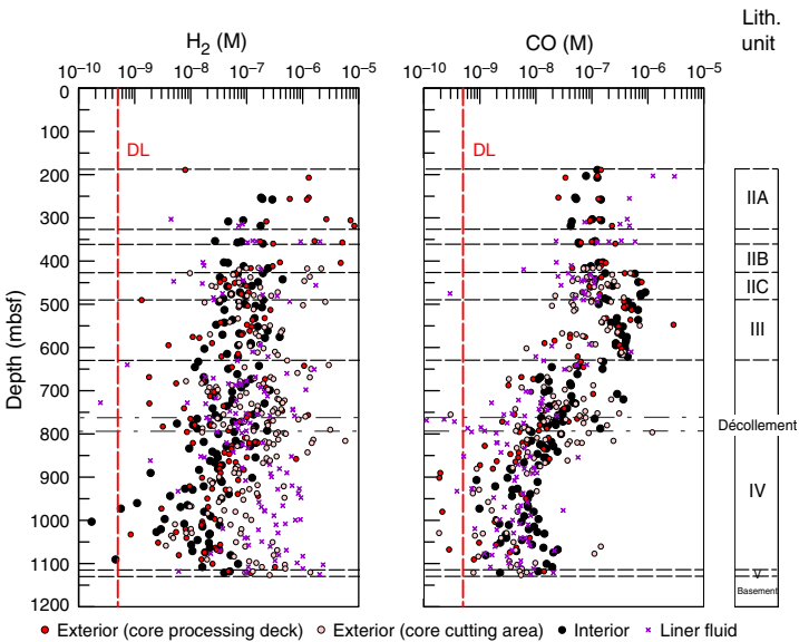
Figure F50. Downhole hydrogen and carbon monoxide concentrations measured in liner fluid and interior and exterior WRC samples, Hole C0023A.
