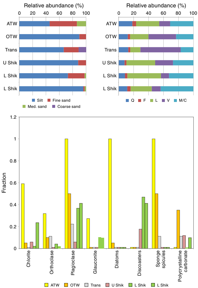
Figure F3. Bar charts illustrating formation characteristics based on smear slide description, Site C0023. ATW = axial trench wedge, OTW = outer trench wedge, Trans = trench-to-basin transition, U Shik = upper Shikoku Basin, L Shik = lower Shikoku Basin. Left: Relative abundance of silt and sand. Right: Relative abundance of silt types. Q = quartz, F = feldspar, L = lithic, V = volcanic, M/C = mud and clay. Bottom: Fraction of each formation containing a given component.
