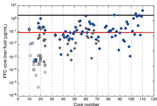
Figure F57. PFC tracer concentrations in core liner fluid (LCL) sampled in Falcon tubes (FAL-L) and headspace vials (CCA-L) when Hole C0023A cores were cut into sections in the Chikyu core cutting area. Open diamonds = FAL-L samples, solid diamonds = CCA-L samples, blue = highest values recorded per core when multiple FAL-L or CCA-L samples were collected from different sections of same core, gray = duplicate samples from same core with lower PFC concentrations, red line = assumed minimal PFC concentration supplied into the system (0.084 mg/L) as calculated based on PFC dosing rate and maximum drilling fluid pumping rate, black line = saturation of PFC in water (1.8 mg/L) (value assumed as maximum PFC concentration present).
