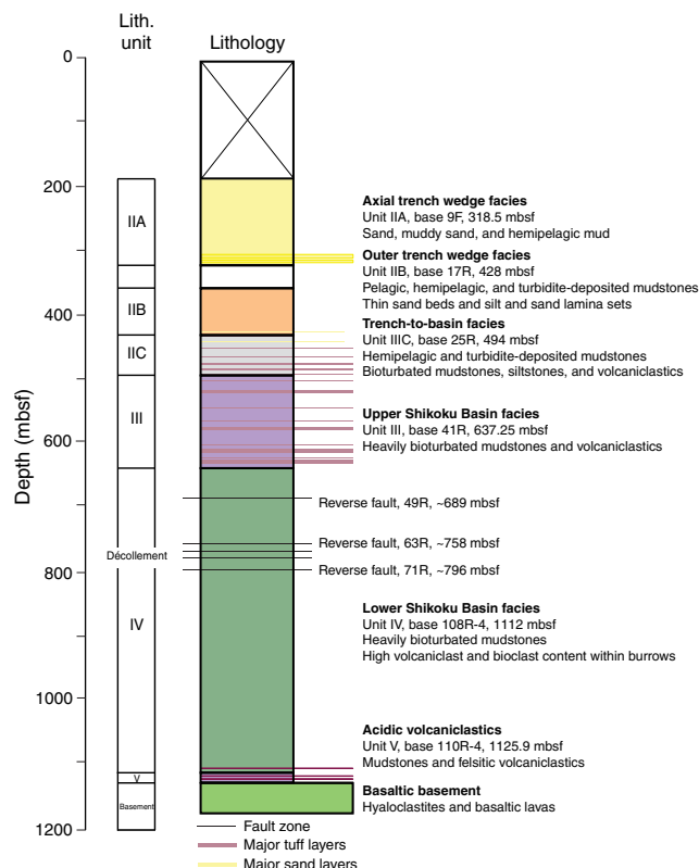
Figure F1. Lithostratigraphy of Hole C0023A, showing major formations, and core observations used to constrain formation boundaries.
