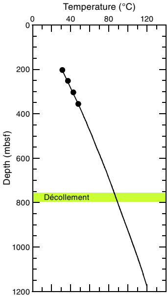
Figure F44. Temperatures projected to the bottom of Hole C0023A, using estimated heat flow of 140 mW/m 2 and measured thermal conductivity data. Estimated temperatures at top of the décollement and bottom of hole are 86° and 120°C, respectively. Circles = measured temperatures.
