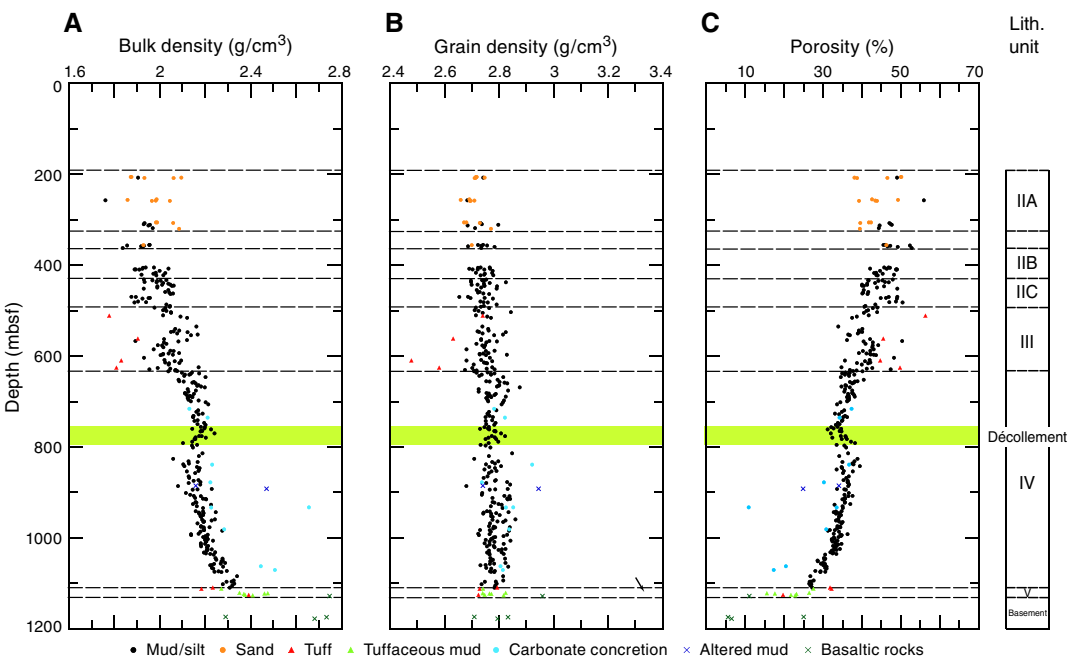
Figure F39. MAD measurements, Hole C0023A. A. Bulk density. B. Grain density. C. Porosity.
