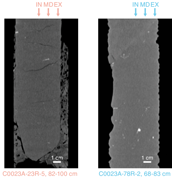
Figure F59. Impact of core quality on contamination of drilling cores with drilling fluid during Expedition 370. X-ray CT-images and PFC concentrations along cross sections are shown for WRCs taken from a section with microfractures (red) and an undisturbed section (blue). Presence of fractures within 23R-5 is clearly correlated with a higher PFC concentration further into core interior (i.e., present in MD sample). A PFC concentration below the LOQ at a similar radial depth (MD) in 78R-2 is consistent with the absence of apparent fractures in the X-ray CT image.
