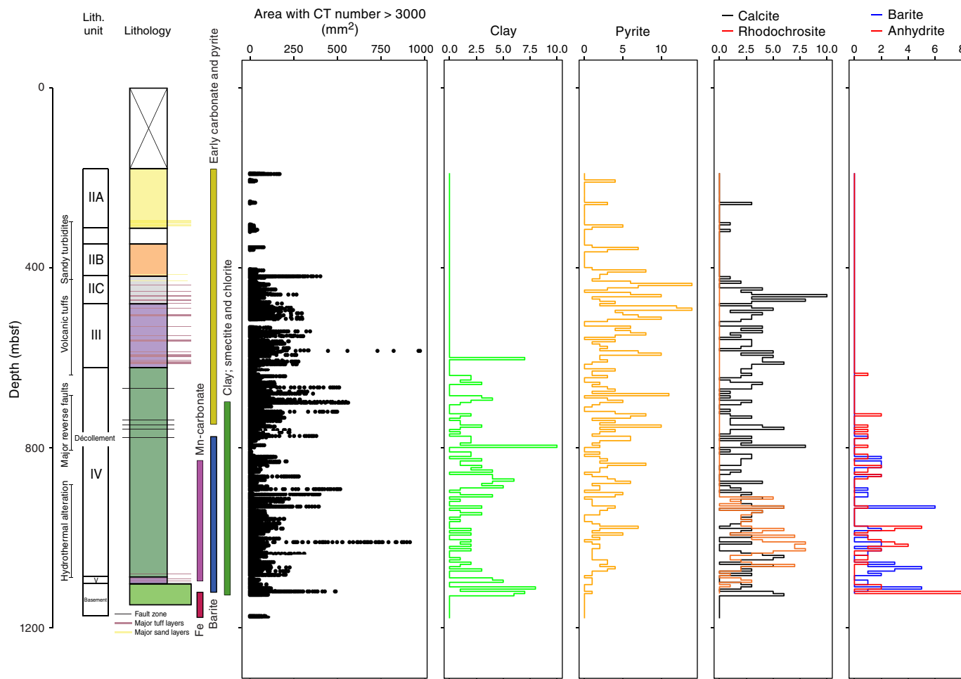
Figure F27. Downhole mineralization trends, Hole C0023A. CT number = ([\mu_t - \mu_w]/\mu_w) \times 1000 , where \mu_t = linear attenuation coefficient (LAC) for the target material and \mu_w = LAC for water.
