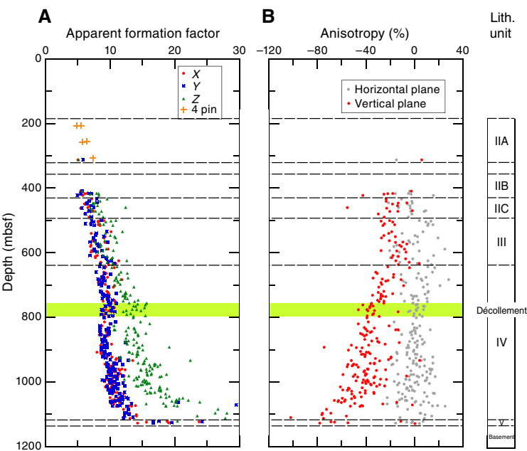
Figure F41. A. Apparent formation factor, Hole C0023A. Carbonate concretion at 931 mbsf and basaltic rock at 1127 mbsf exhibit a formation factor of ~70 and ~155, respectively, and are not shown. 4 pin = determined on working half sections along the y-direction with a 4-pin electrode. B. Anisotropy of formation factor in the horizontal (x- and y-axes) and vertical (z-axis) planes.
