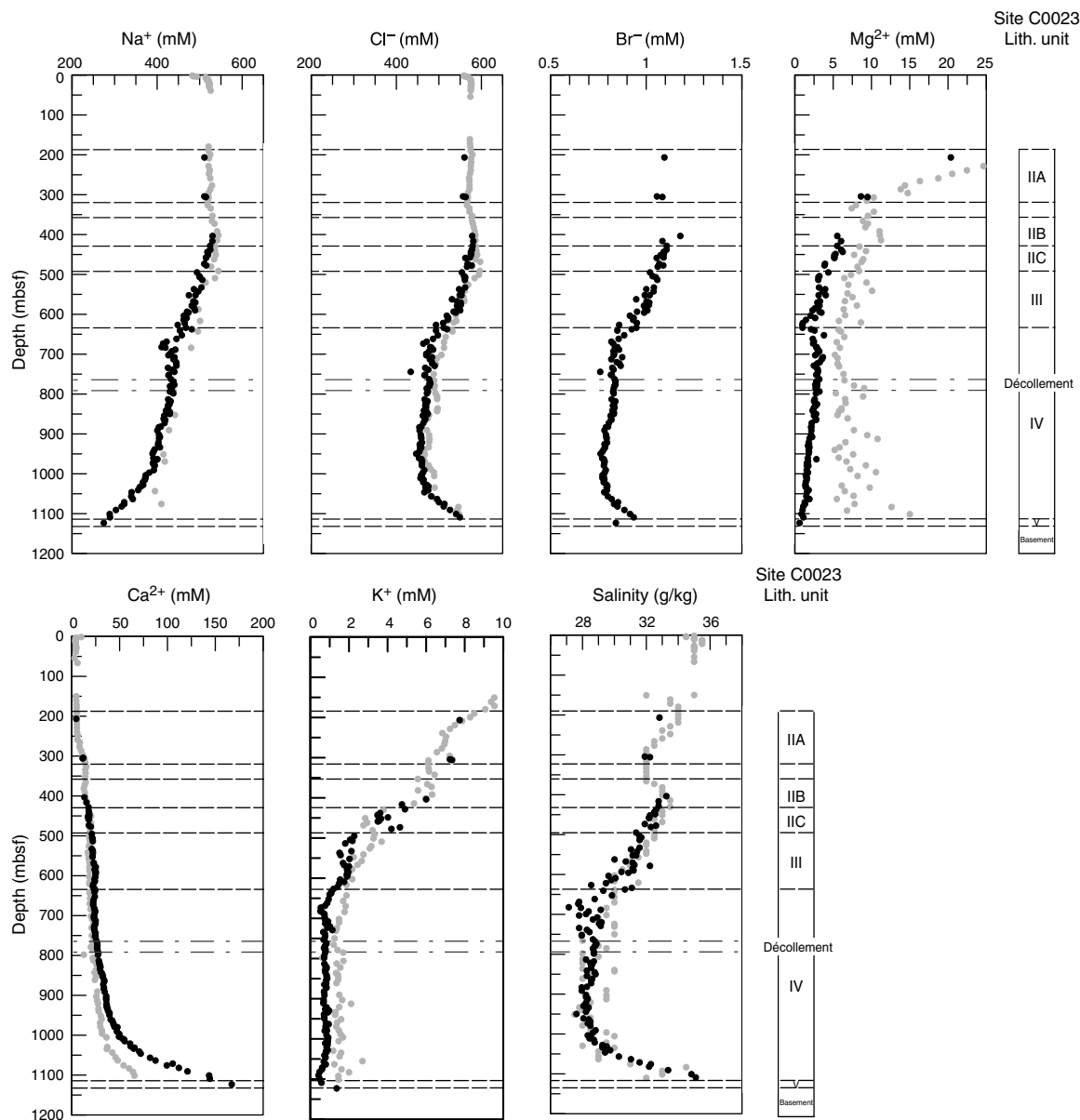
Figure F46. Major cations, \text{Cl}^- , and salinity (calculated from refractive index), Hole C0023A (black circles). Gray circles = data for Site 1174 (Shipboard Scientific Party, 2001b). Site 1174 data were clipped off at 25 and 10 mM for \text{Mg}^{2+} and \text{K}^+ , respectively.
