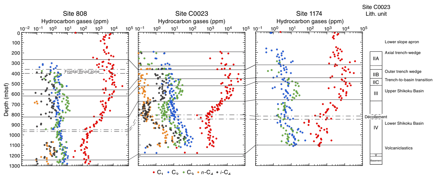
Figure F52. Mole fraction of hydrocarbon gases in headspace gas samples from Sites C0023 (see also Table T7), 808 (Shipboard Scientific Party, 1991), and 1174 (Shipboard Scientific Party, 2001b).
