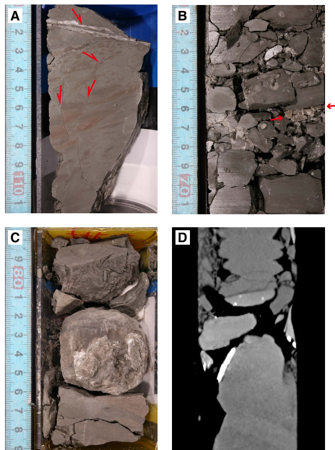
Figure F23. Mineral veins observed. A. Calcite vein (C0023A-103R-6, 101–111 cm [~1068 mbsf]) representing crosscutting relationship to minor normal faults (split arrows): vein cut the normal faults and vice versa. B. Close-up core photograph of barite (red arrows) (104R-5, 60–71 cm [~1075 mbsf]). C, D. Barite vein developed along the normal fault (77R-2, 78–89 cm [~821 mbsf]; C: split surface, D: X-ray CT image).
