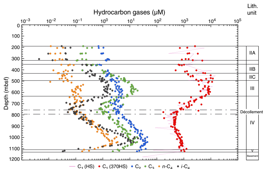
Figure F53. Concentrations of dissolved hydrocarbon gases, Hole C0023A. Data are from samples taken directly from the core catcher (HS) and gas voids (VAC) in core cutting area and from COMGAS WRC slices (370HS) taken on core processing deck. C_1 from headspace analyses of safety gas samples (HS) taken in core cutting area immediately after arrival on catwalk is also shown. All data are from Table T22.
