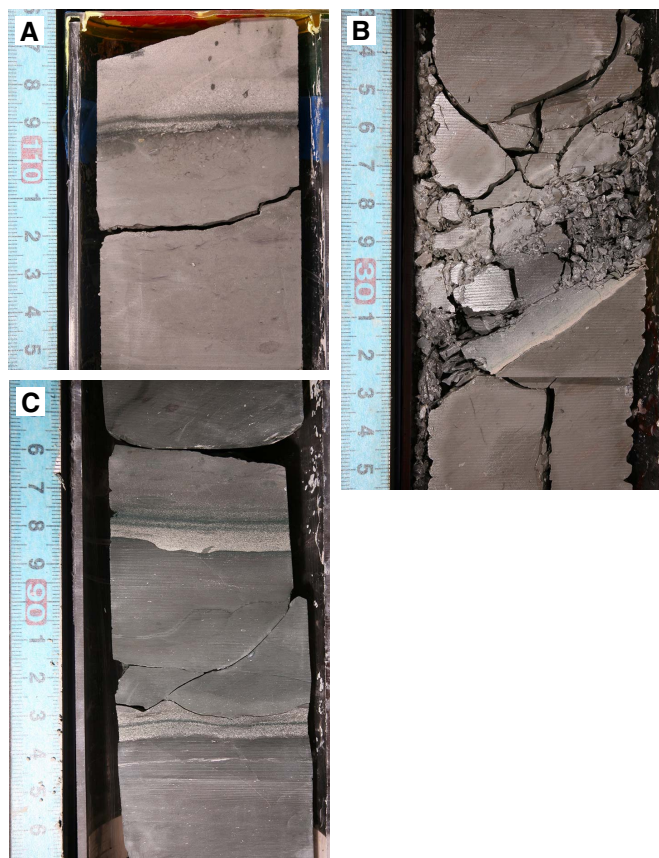
Figure F19. Bedding dip examples. A. C0023A-24R-6, 106–116 cm (~492 mbsf). B. 97R-7, 23–36 cm (~1007 mbsf). C. 110R-3, 85–97 cm (~1101 mbsf). Note the variation of bedding dips (also refer to Figure F18).
