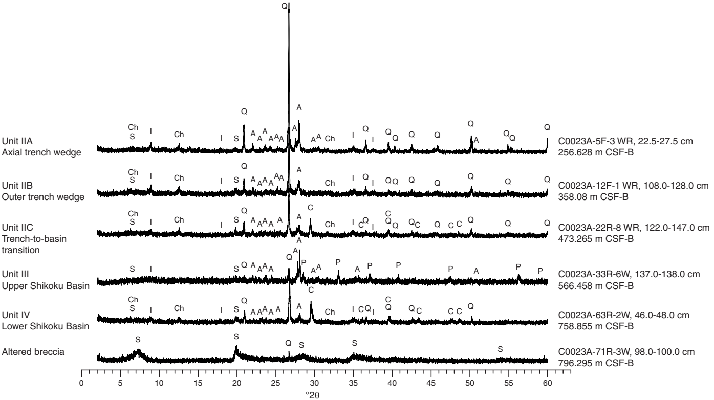
Figure F15. XRD profiles of 6 representative types of mudstone, Hole C0023A. Mineral compositions are superimposed to show each peak position. S = smectite, I = illite, Ch = chlorite, Q = quartz, A = anorthite, C = calcite, P = pyrite.
