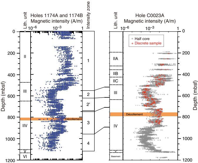
Figure F34. Downhole profile of magnetic intensity (after 20 mT demagnetization) in Hole C0023A compared to Holes 1174A and 1174B.
