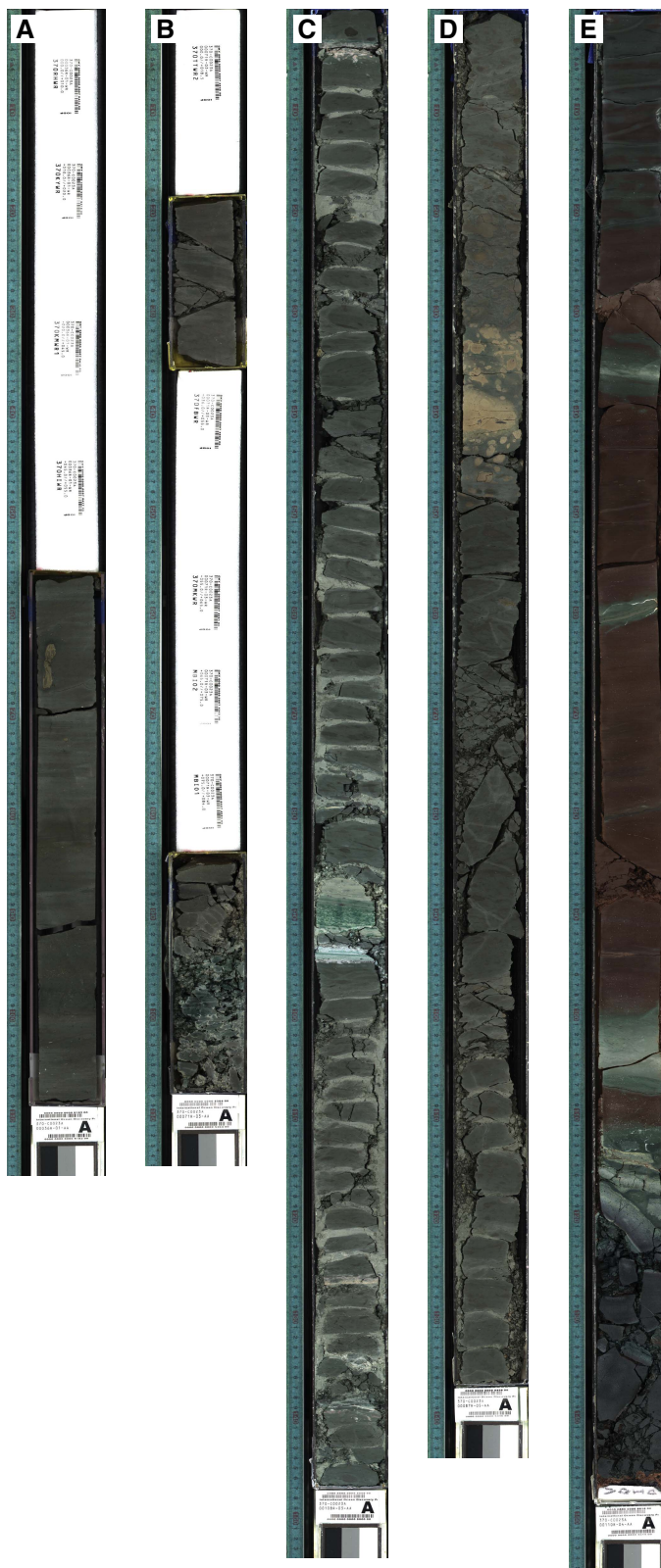
Figure F29. Core sections recovered from different mineralization zones. A. 5 cm long pyrite nodule (C0023A-36R-1, 63–68 cm). B. Green mineralization at décollement zone (71R-3). C. Green mineralization in zone of normal faulting below the décollement (108R-3). D. Red and yellow burrows filled with rhodochrosite (87R-5). E. Red clay above basement with magnetite, hematite, and goethite; green mineralization is also present (110R-4).
