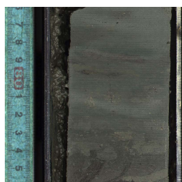
C0023A-22R-4, 76–86 cm
