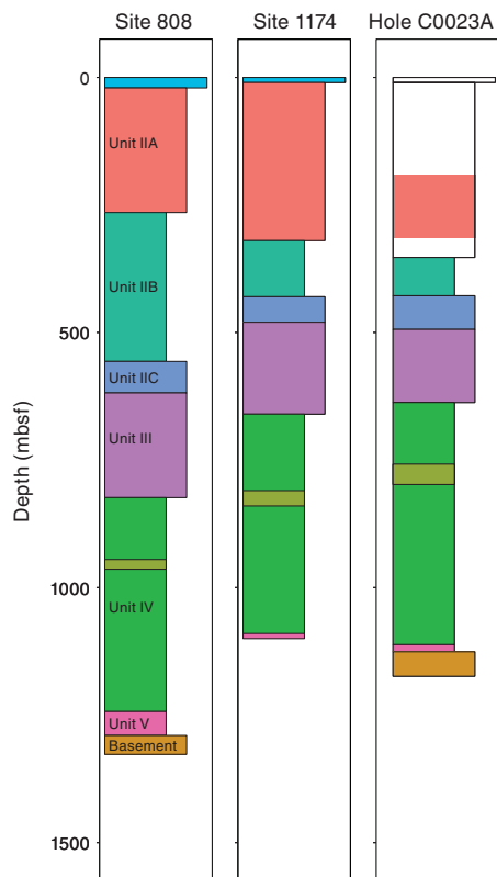
Figure F33. Comparison of Hole C0023A lithostratigraphic units to Sites 808 and 1174.
