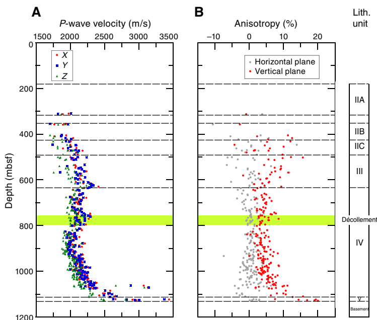
Figure F40. A. P -wave velocity, Hole C0023A. B. Anisotropy of P -wave velocity in the horizontal ( x - and y -axes) and vertical ( z -axis) planes. The horizontal plane anisotropy that compares velocity of x - and y -directions should average zero because cores are randomly rotated.
