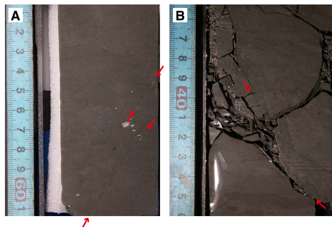
Figure F26. Split core surface images, showing (A) sand dikes and (B) a hydrofracture (A: C0023A-24R-5, 51–61 cm [~489 mbsf], B: 100R-5, 35–46 cm [~1034 mbsf]). Arrows = position and direction of dikes and contact between hydrofractured material and the host rocks, respectively.
