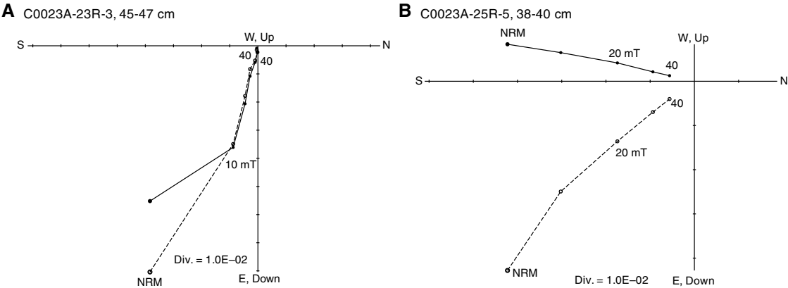
Figure F36. A, B. AF demagnetization of discrete samples. Solid circles = projection onto horizontal plane, open circles = projection onto either vertical X-Z or Y-Z planes.
