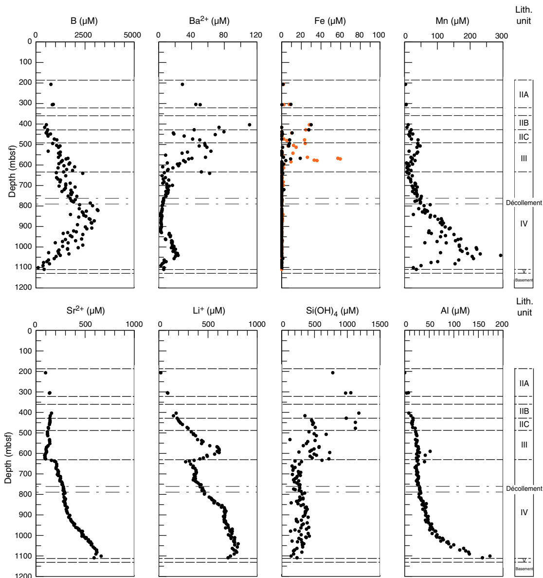
Figure F48. Minor cations in IW determined by inductively coupled plasma–atomic emission spectrometry (ICP-AES) analyses (black circles), Hole C0023A. Orange circles = \text{Fe}^{2+} determined photospectrometrically.
