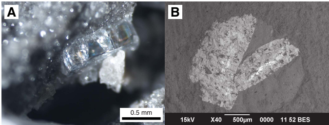
Figure F31. Vein and strata-bound sulfate mineralization. A. Barite crystals in a vein (C0023A-77R-2, 79–90 cm). B. Barite (white) in a burrow (87R-4, 6–7 cm; SEM [backscatter mode]).
