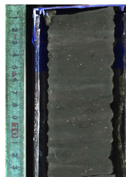
C0023A-41R-9, 0–14 cm
