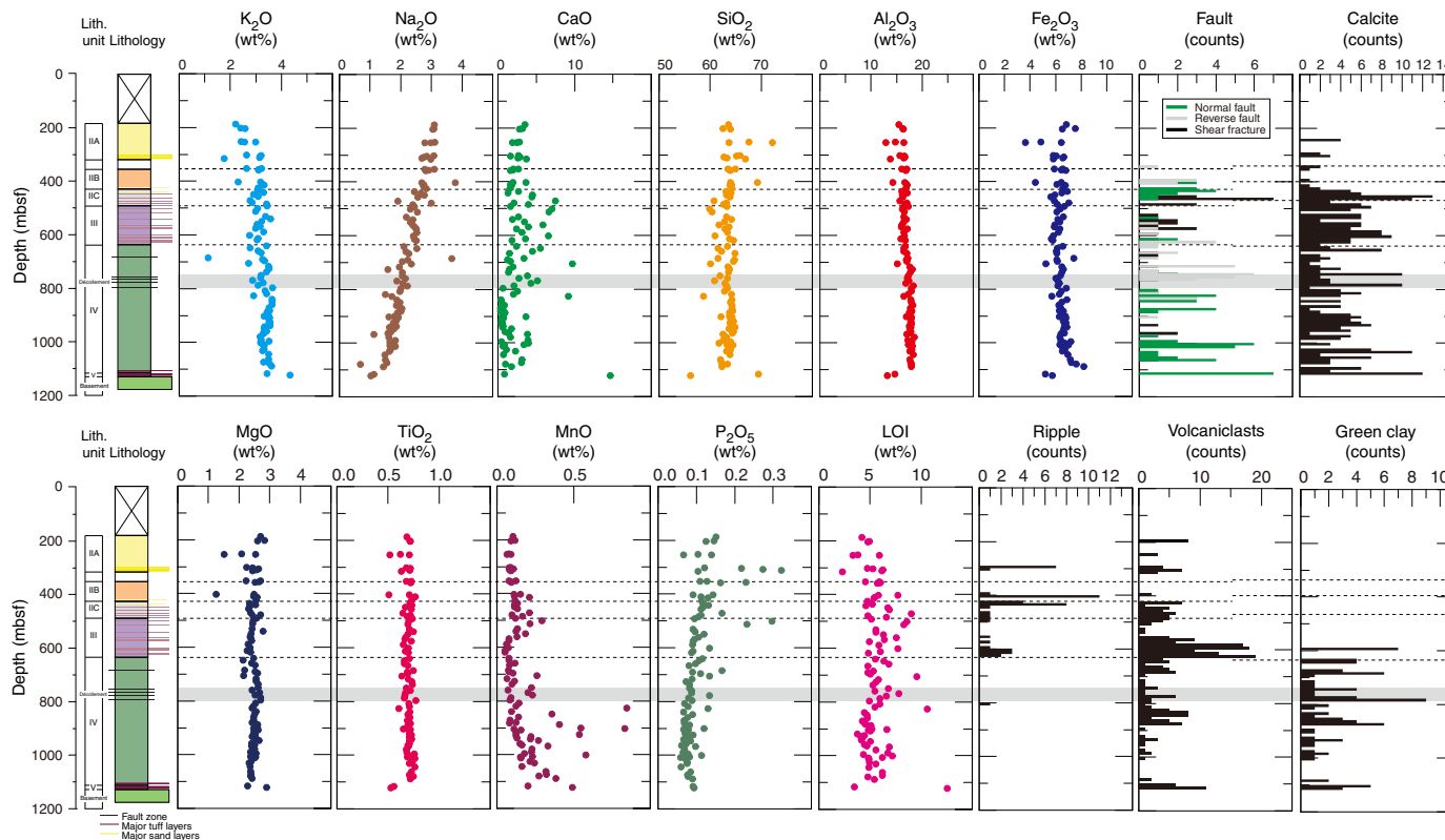
Figure F17. XRF relative abundance of major element oxides compared to total number of visual core description (VCD) observations of given type, Hole C0023A. Dashed lines = lithostratigraphic unit boundaries, gray bar = décollement. LOI = loss on ignition.
