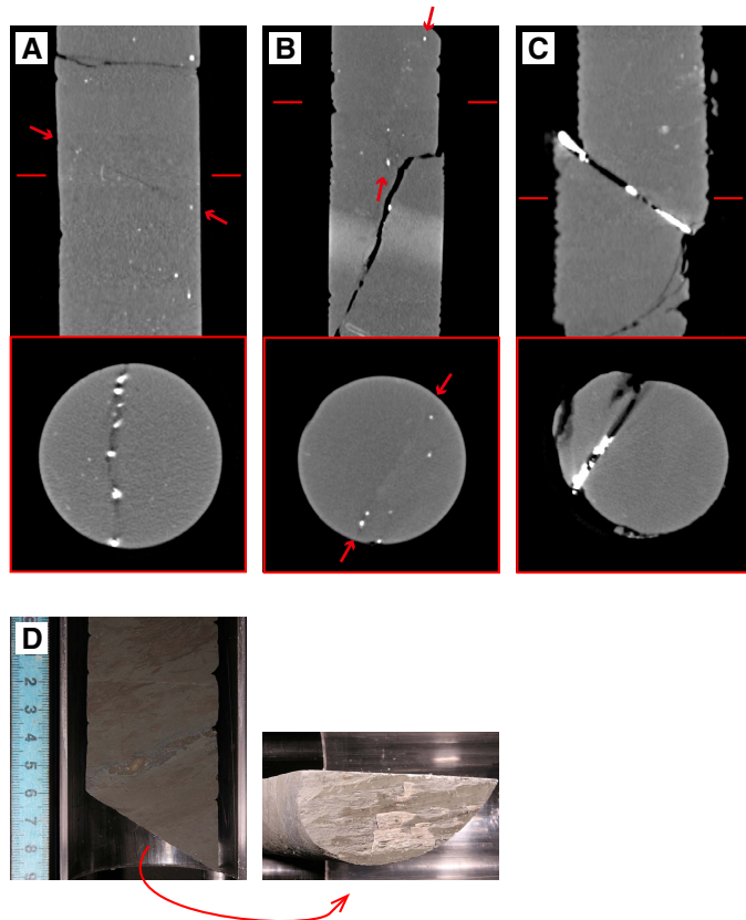
Figure F24. A–C. X-ray CT images of crystallized minerals along faults (A: C0023A-56R-3, 29–33 cm [~727 mbsf], B: 82R-1, 19–31 cm [~852 mbsf], C: 79R-3, 99–101 cm [~832 mbsf]); top: vertical sections, bottom: conical sections. Lines = position of conical section, arrows = position and direction of fault surface. Note that A and B represent scattered mineralization of barite along normal faults, whereas C shows architecture of vein along fault. D. Core photograph of normal fault (101R-4, 30–39 cm [~1043 mbsf]). Slickenlines and steps representing normal fault sense were identified along the fault surface.
