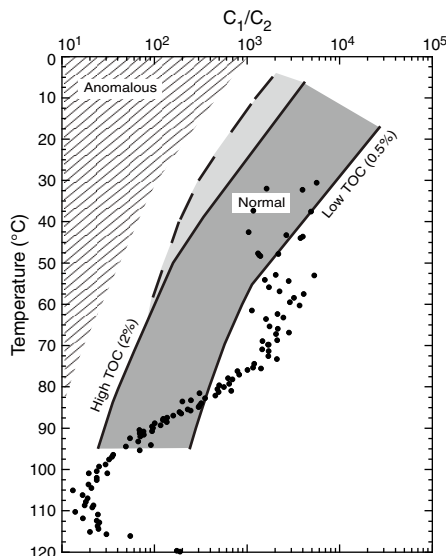
Figure F54. Methane/ethane ( C_1/C_2 ) molar ratios vs. temperature, Hole C0023A. In situ temperatures were adopted from Figure F44. The underlying diagram was modified from Pimmel and Claypool (2001).
