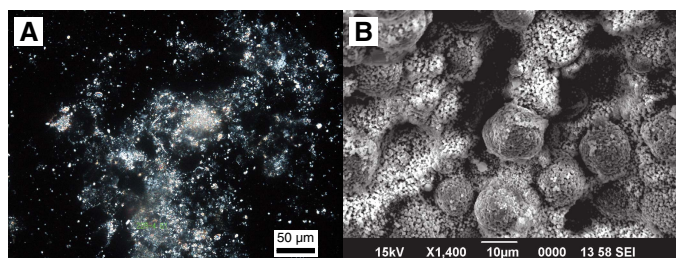
Figure F28. Calcite and pyrite in early-stage diagenesis. A. Polycrystalline carbonate in smear slide (C0023A-22R-4, 61 cm; XPL). B. Framboidal pyrite (30R-2, 115–129 cm; SEM).
