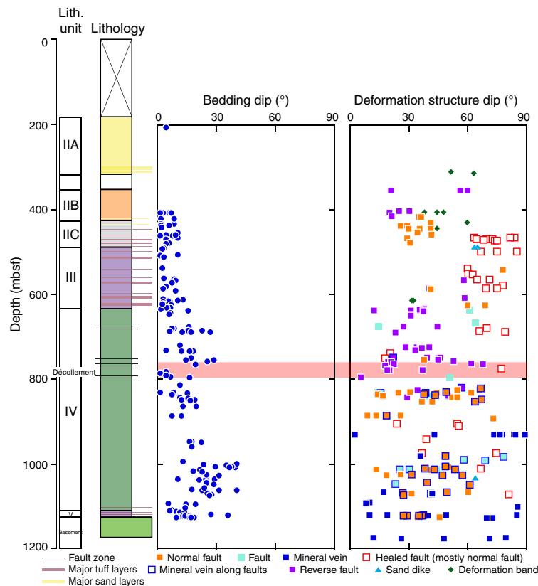
Figure F18. Bedding and deformation structure dip angles as a function of depth, Hole C0023A.
