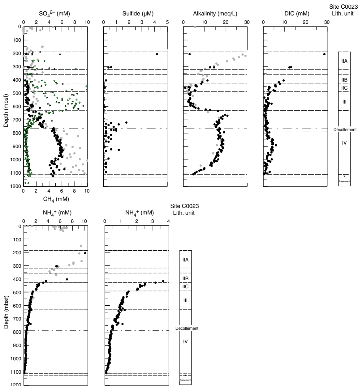
Figure F47. IW composition (sulfate, sulfide, alkalinity, dissolved inorganic carbon [DIC], and ammonium), Hole C0023A (black circles). Green diamonds = methane data from Organic geochemistry and were clipped at 10 mM here, gray circles = Site 1174 data. \text{SO}_4^{2-} and alkalinity data were clipped at 10 and 30 mM, respectively. Last plot: close-up of Site C0023 ammonium profile, showing slight offsets at lithostratigraphic boundaries.
