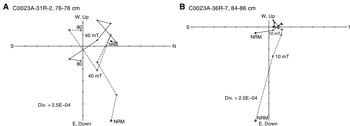
Figure F37. A, B. AF demagnetization of discrete samples. Some samples do not show stable component. Solid circles = projection onto horizontal plane, open circles = projection onto either vertical X-Z or Y-Z planes.
