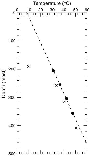
Figure F43. Temperatures obtained in situ by APCT-3 measurements during short HPCS coring, Hole C0023A. Least-squares fit yields an average thermal gradient of 111°C/km and intercept temperature of 8.5°C at the seafloor. Circles = temperature data used for calculating thermal gradient and heat flow, crosses = poor quality temperature data (see Table T11).
