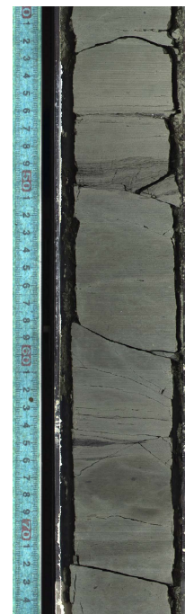
C0023A-16R-5, 40-75 cm
