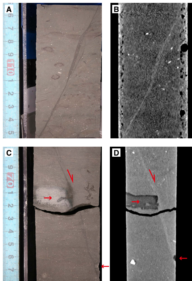
Figure F20. Core-scale healed faults. (A, C) Core photograph and (B, D) X-ray CT image of a healed fault (A, B: C0023A-33R-5, 95–108 cm [~565 mbsf]; C, D: 36R-2, 67–78 cm [~585 mbsf]). Note that ash layers (red arrows; dark color in D), are cut by the healed fault, representing normal fault sense (split arrow).
