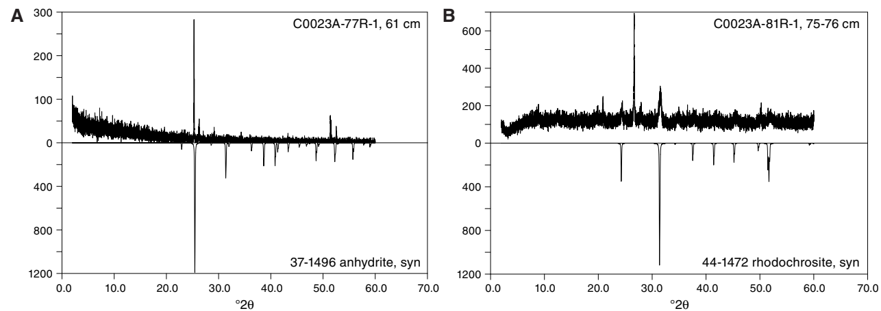
Figure F30. XRD data confirming the presence of (A) anhydrite and (B) rhodochrosite, Hole C0023A.
