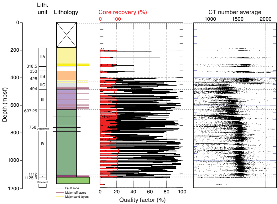
Figure F32. Site summary diagram of X-ray CT images for Hole C0023A from 0 to 1200 mbsf. CT number = ([\mu_t - \mu_w]/\mu_w) \times 1000 , where \mu_t = LAC for the target material and \mu_w = LAC for water.
