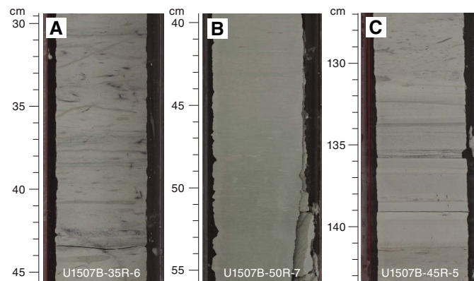
Figure F15. Common Unit II sedimentary lithologies, Site U1507. A. Middle Eocene nannofossil chalk with foraminifers (frm). mct = micrite. B. Middle Eocene foraminiferal limestone with recrystallized foraminifers.
