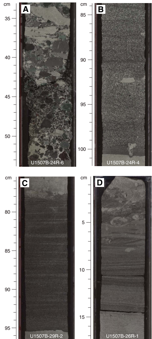
Figure F12. Common Subunit 1c sedimentary lithologies, Site U1507. A. Lower Oligocene tuffaceous conglomerate with vesicular basalt clasts and common nannofossil chalk rip-up clasts. B. Lower Oligocene massive to faintly planar-laminated tuffaceous sandstone. C. Lower Oligocene planar-laminated tuff sharply overlain by bioturbated clayey nannofossil chalk. D. Lower Oligocene planar- to ripple-laminated tuffaceous sandstone.
