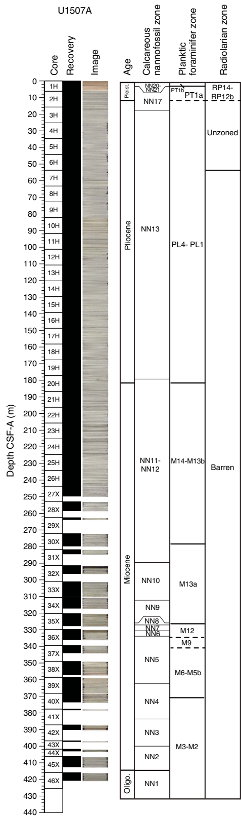
Figure F17. Biozonations, Hole U1507A.
