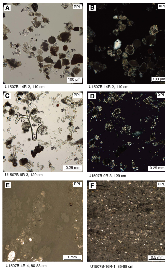
Figure F10. Common Subunit 1b sedimentary lithologies, Site U1507. A, B. Upper Oligocene clayey tuffaceous sandstone. Note the common glass (gls) fragments and rare quartz (qtz) grains. frm = foraminifer. C, D. Upper Oligocene clayey tuffaceous sandstone. Note the sponge spicule (sp) fragments. E. Lower Miocene disrupted clayey foraminiferal chalk. F. Upper Oligocene clayey foraminiferal chalk with silt-sized volcanic material.
