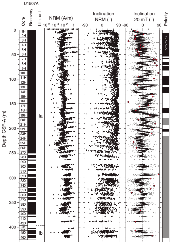
Figure F24. Pass-through paleomagnetic data, Hole U1507A. Black dots = NRM intensity and inclination, gray dots = inclination after 20 mT AF cleaning interpolated by 10-point moving average (black line), red dots = inclination of ChRM directions from discrete sample analysis. Magnetic polarity: black = normal, white = reversed, gray = unidentified.
