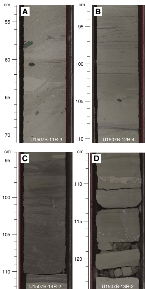
Figure F9. Common Subunit 1b sedimentary lithologies, Site U1507. A. Upper Oligocene disrupted clayey foraminiferal chalk with scattered volcanic clasts and rip-up clasts of foraminiferal chalk. This section is part of a very thick, strongly disrupted bed. B. Upper Oligocene clayey foraminiferal chalk with rare volcanic clasts displaying wispy planar laminations. C. Upper Oligocene sharp-based, normally graded clayey tuffaceous sandstone with rippled and convoluted laminations. D. Upper Oligocene sharp-based, normally graded, planar-laminated clayey tuffaceous siltstone.
