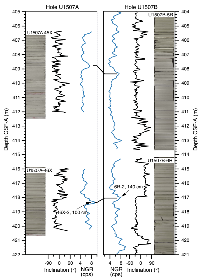
Figure F38. Depth correlation between overlapping intervals of Holes U1507A and U1507B based on NGR (blue) records and confirmed with magnetic inclination (black) and core images. The overlapping interval was XCB cored in Hole U1507A and RCB cored in Hole U1507B.
