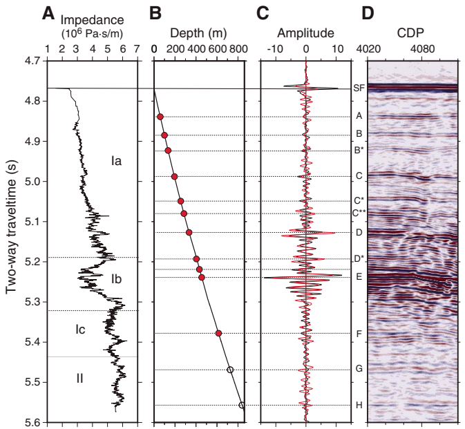
Figure F35. Borehole data to MCS data tie, Site U1507. A. Impedance calculated from combined rebound-corrected velocity data from cores and wireline log P -wave velocity and density data vs. TWT. Horizontal line = lithostratigraphic unit boundary, dashed horizontal lines = subunit boundaries. B. TWT calculated from depths below seafloor, rebound-corrected PWC P -wave velocity data (0–70 m), and in situ wireline log P -wave velocity (70–860 m WMSF). Numerical solution for TWT ( t ) with depth ( z ) is given by z = 306.57t^2 - 823.43t . Circles = positions of strong reflectors shown in C and D (red = strongly correlated, open = not correlated), dashed lines = fit between seismic survey data in D and synthetic trace in C. C. Synthetic trace (red) and MCS trace data at Line TAN1409-NCTN-11, CDP 4020 (black). Seismic Reflectors A–H and seafloor (SF) are labeled. D. MCS data.
