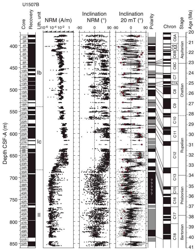
Figure F25. Pass-through paleomagnetic data, Hole U1507B. Black dots = NRM intensity and inclination, gray dots = inclination after 20 mT AF cleaning interpolated by 10-point moving average (black line), red dots = inclination of ChRM directions from discrete sample analysis. Magnetic polarity: black = normal, white = reversed, gray = unidentified. Correlation with GPTS2012 is shown.
