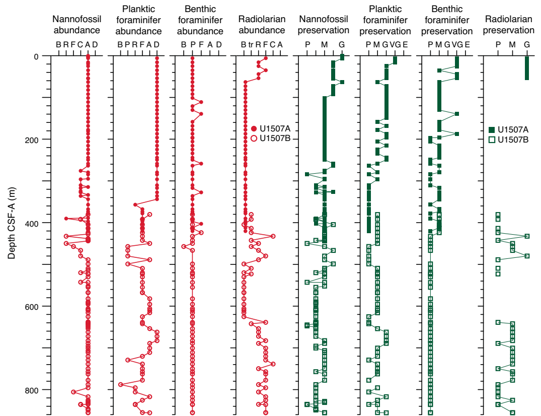
Figure F19. Microfossil abundance and preservation, Site U1507. Abundance: D = dominant, A = abundant, C = common, F = few, R = rare, P = present, tr = trace, B = barren. Preservation: E = excellent, VG = very good, G = good, M = moderate, P = poor.
