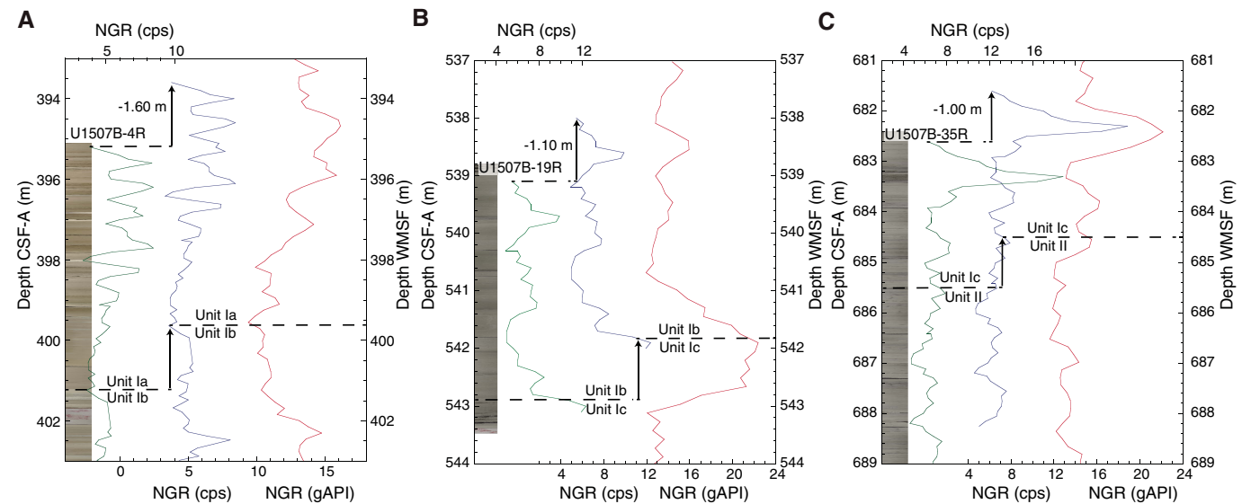
Figure F39. Depth correlation between Hole U1507B core data and wireline data based on NGR records. A. Subunit Ia/Ib boundary. B. Subunit Ib/Ic boundary. C. Subunit Ic/Unit II boundary. Green = whole-round core NGR data on CSF-A scale, blue = shifted NGR core data on WMSF scale, red = wireline logging NGR data.
