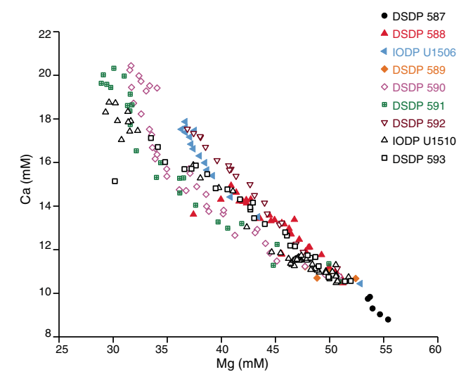
Figure F33. Dissolved Ca vs. Mg in IW, Sites U1506 and U1510 and DSDP Sites 587–593 (Baker, 1986).
