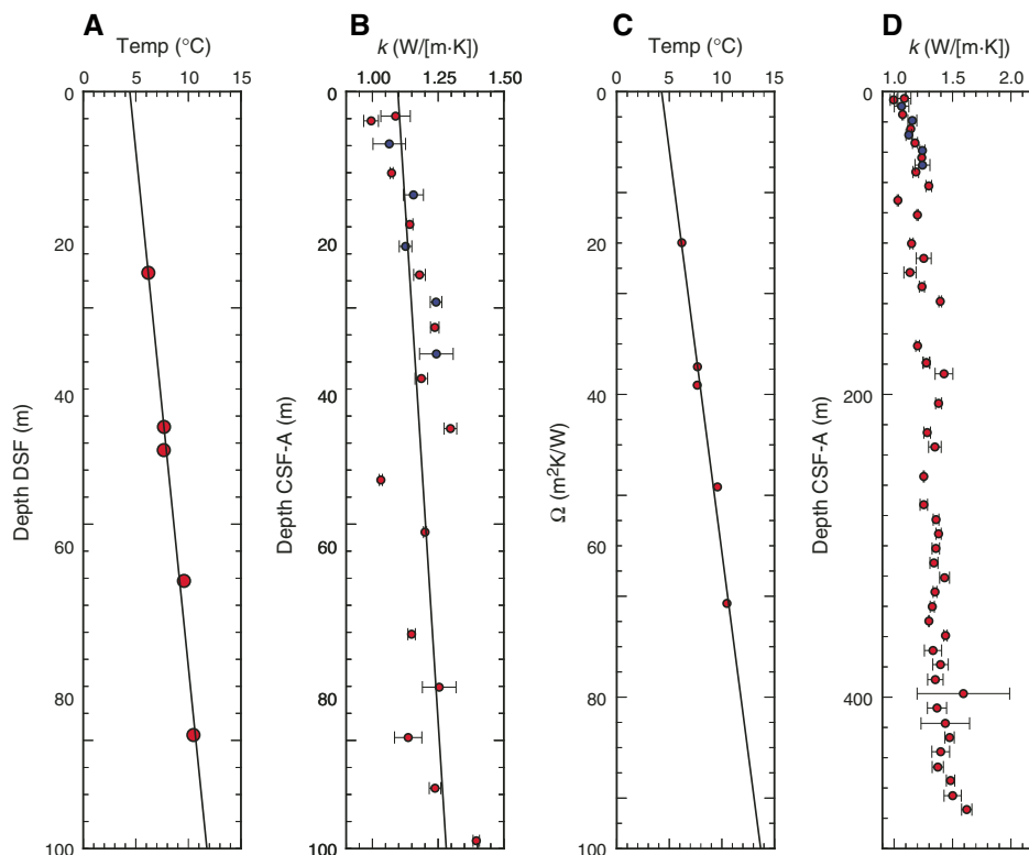
Figure F27. Heat flow. Note the vertical scale unit changes. A. APCT-3 temperature with depth profile measured in Holes U1510A and U1510B. B, D. Thermal conductivity with 95% confidence interval estimate with three repeat measurements shown as error bars, Hole U1510A (red) and U1510B (blue) cores. C. Bullard plot (see Petrophysics in the Expedition 371 methods chapter [Sutherland et al., 2019a]) showing thermal resistance ( \Omega ) vs. measured temperature.
