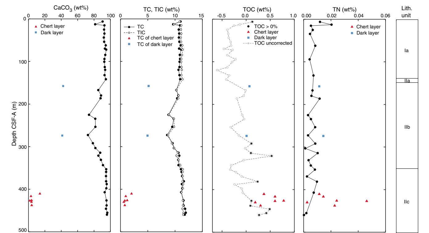
Figure F32. Bulk sediment profiles of calcium carbonate ( \text{CaCO}_3 ), total carbon (TC), total inorganic carbon (TIC), TOC, and total nitrogen (TN), Site U1510.
