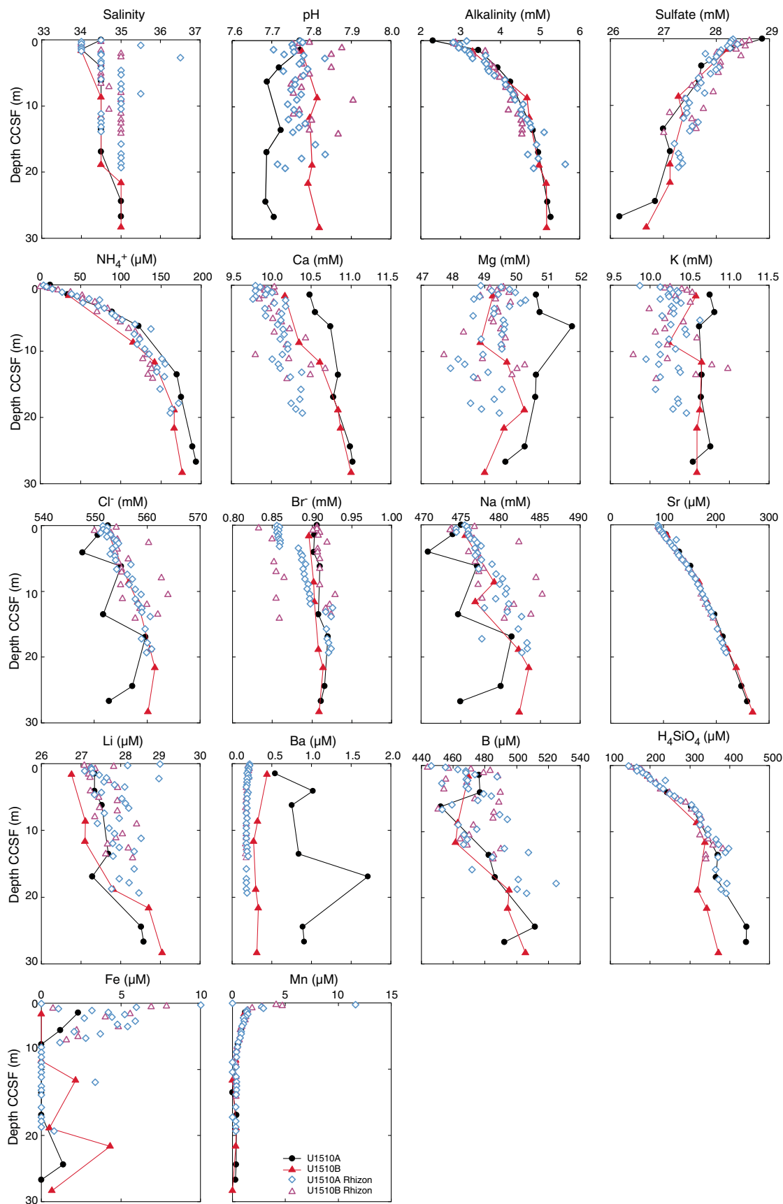
Figure F31. Squeeze and Rhizon IW chemistry for uppermost 30 m CCSF, Site U1510.
