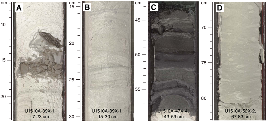
Figure F12. Representative Subunit IIc lithologies, Hole U1510A. A. Nannofossil chalk with chert (dark gray). B. Nannofossil chalk with foraminifers. C. Tuff. D. Nannofossil chalk.
