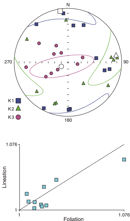
Figure F24. AMS data for 10 discrete samples, Site U1510. Top: stereoscopic plot. Blue squares = \kappa_{\max} axes, green triangles = \kappa_{\text{int}} axes, purple circles = \kappa_{\min} axes. Mean directions of \kappa_{\max} (open square), \kappa_{\text{int}} (open triangle), and \kappa_{\min} (open circle) axes, shown along with their 95% confidence ellipses. Bottom: corresponding lineation ( \kappa_{\max}/\kappa_{\text{int}} ) vs. foliation ( \kappa_{\text{int}}/\kappa_{\min} ) data.
