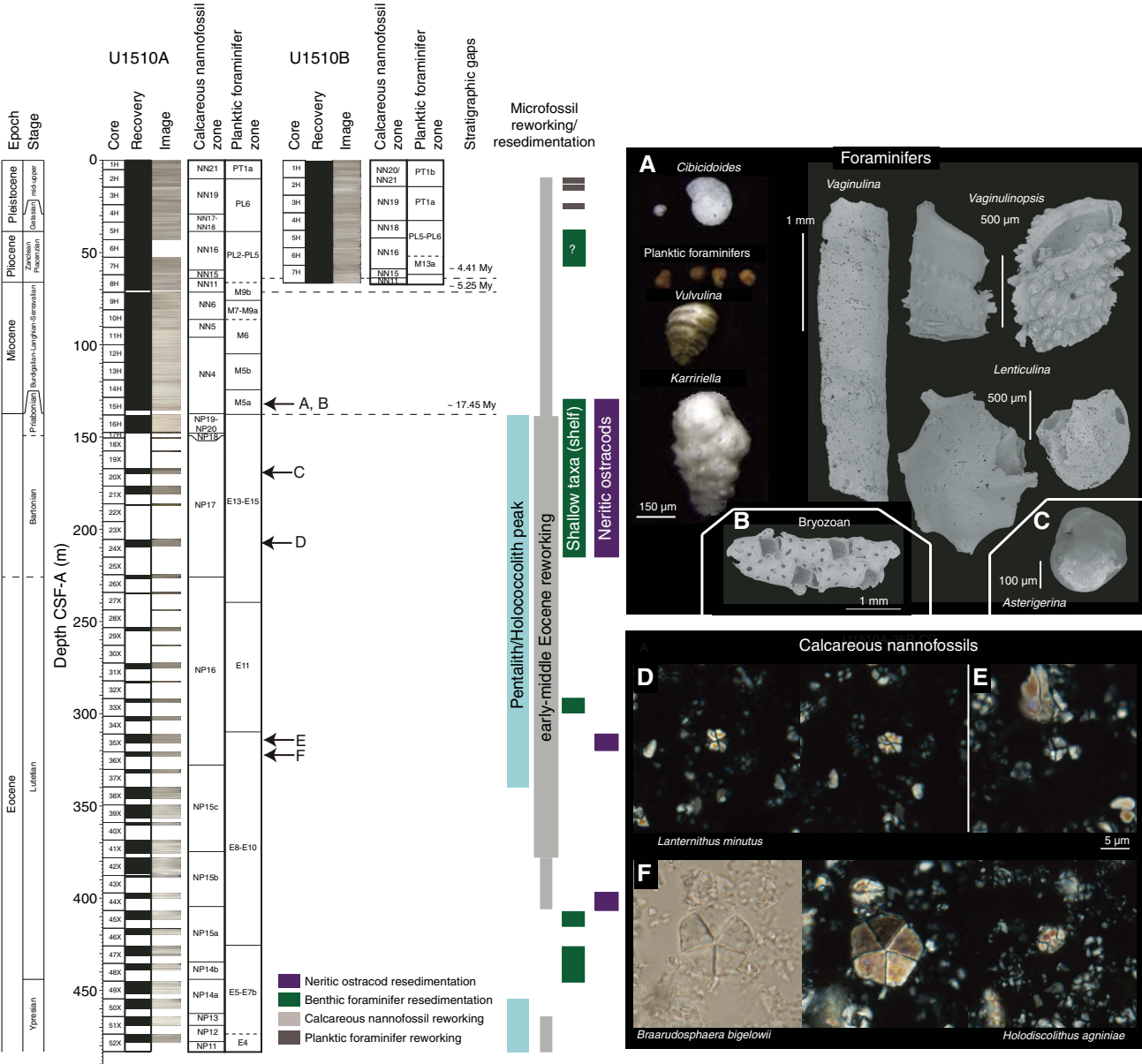
Figure F18. Biozonations, reworking/resedimentation of microfossil assemblages, and plates of reworked/resedimented fossils, Site U1510. Blue vertical bar = peak in abundance of pentalith/holococcolith nannofossil species that usually inhabit shallow-water settings and occur frequently throughout reworked intervals, green vertical bar = benthic foraminifer resedimentation, purple bar = presence of neritic ostracods. A, B. 371-U1510A-15H-CC (135.33–135.43 m). C. 20X-CC (169.90–170.00 m). D. 24X-CC (209.22–209.32 m). E. 35X-CC (315.74–315.84 m). F. 36X-CC (323.07–323.17 m). Planktic foraminifer zones with dashed lines indicate zones defined on assemblages and are, therefore, approximations.
