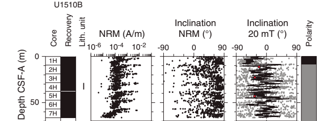
Figure F21. Pass-through paleomagnetic data, Hole U1510B. Black dots = NRM intensity and inclination, gray dots = inclination after 20 mT AF cleaning interpolated by 10-point moving average (black line), red dots = inclination from discrete sample analysis. Magnetic polarity: black = normal, white = reversed, gray = unidentified.
