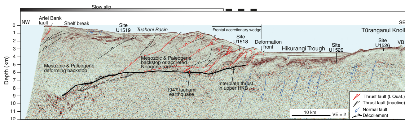
Figure F2. Depth-converted Seismic Profile 05CM-04 showing locations and depths of sites drilled during Expedition 375 and structural interpretation (modified from Barker et al., 2018). Star = projected location of March 1947 tsunami earthquake. Location of the profile coincides with the drilling transect shown in Figure F1. VB = volcanic cone. VE = vertical exaggeration.
