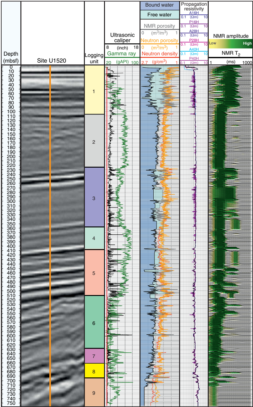
Figure F12. Composite plot of seismic image (Profile 05CM-04) and selected LWD measurements, Site U1520. PSDM from Barker et al. (2018).
