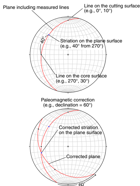
Figure F26. Lower hemisphere equal-area projections showing procedure for converting 2-D measured data to 3-D data, Expedition 375. Plane attitude determined using two apparent dips on two surfaces. Striation on the plane is also plotted.
