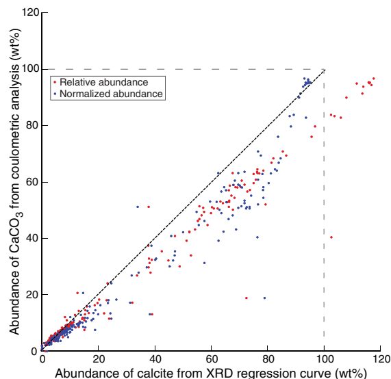
Figure F13. Statistical fits between relative and normalized abundance of calcite (from XRD analyses, MacDiff software) and carbonate (from coulometric analyses) values using co-located specimens from Site U1520. See Figure F12 for regression curve. Black dashed line represents 1:1 fit. XRD overestimates calcite abundance because of a mismatch in crystallinity between the calcite standard (nannofossil-rich Cyprus chalk) and variably recrystallized marls and chalks from Site U1520. See M.B. Underwood and N. Lawler (unpubl. data) for additional assessments of error, including interlaboratory and intralaboratory comparisons.
