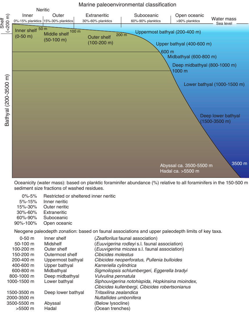
Figure F19. Adopted marine paleoenvironmental classification and environmental thresholds after Hayward et al. (2010), calibrated paleodepth markers after Crundwell et al. (1994), and unpublished GNS Science data used during Expedition 375.
