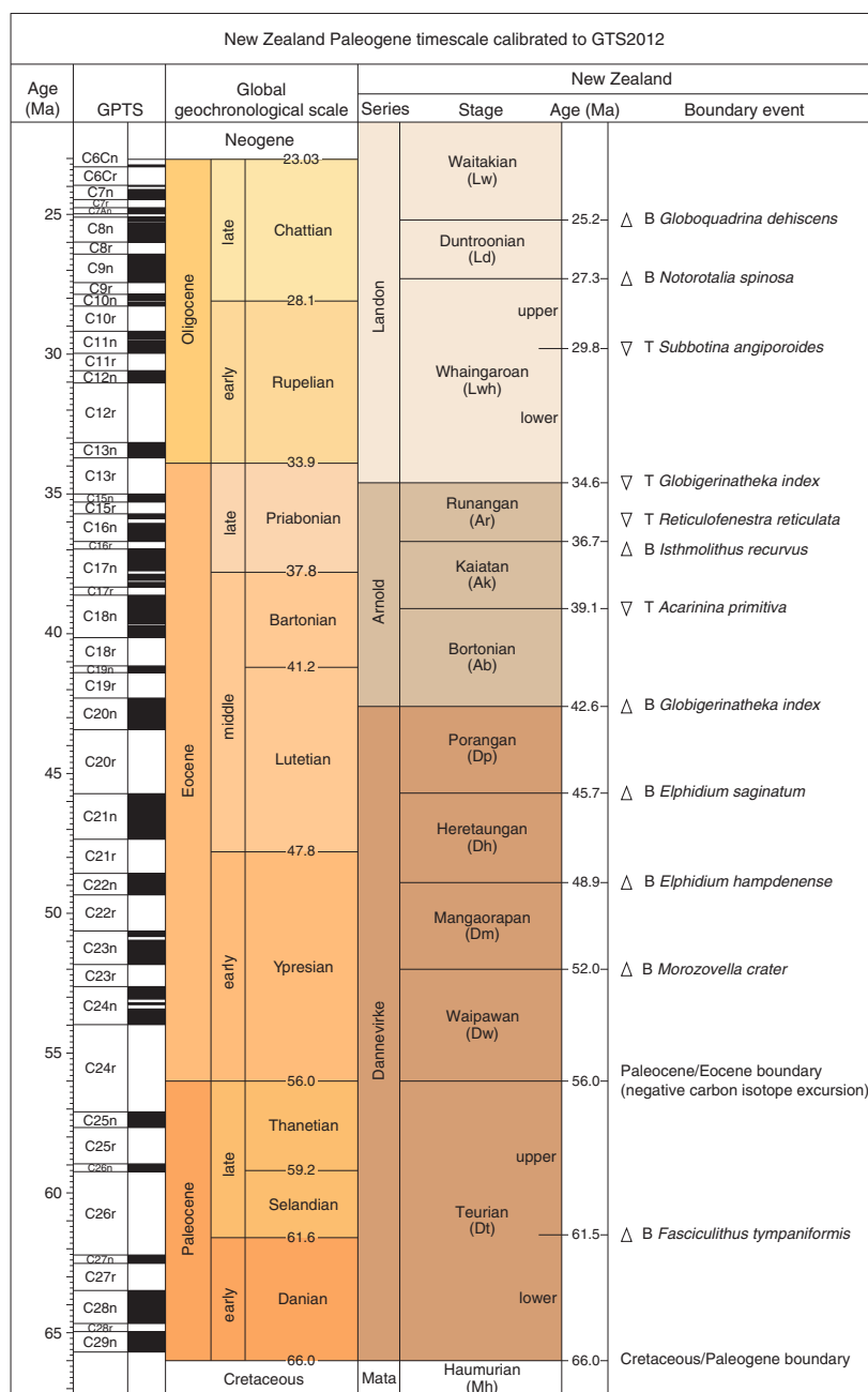
Figure F17. New Zealand Paleogene (Paleocene, Eocene, and Oligocene) timescale calibrated to GTS2012 (Gradstein et al. 2012) after Raine et al. (2015) used during Expedition 375. Black = normal polarity, white = reversed polarity. Triangles = base (B), inverted triangles = top (T), solid triangles = formally defined SSP, open triangles = no formally defined SSP.
