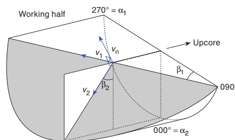
Figure F24. Calculation of plane orientation (shaded) from two apparent dips, Expedition 375. Intersections of split-core surface, section perpendicular to split-core surface, and section parallel to core direction with plane of interest are shown. ( \alpha_1 , \beta_1 ) and ( \alpha_2 , \beta_2 ) are the azimuths ( \alpha ) and plunges ( \beta ) of traces of the plane on two sections, v_1 and v_2 are unit vectors parallel to traces of the plane on two sections, and v_n is the unit vector normal to plane.
