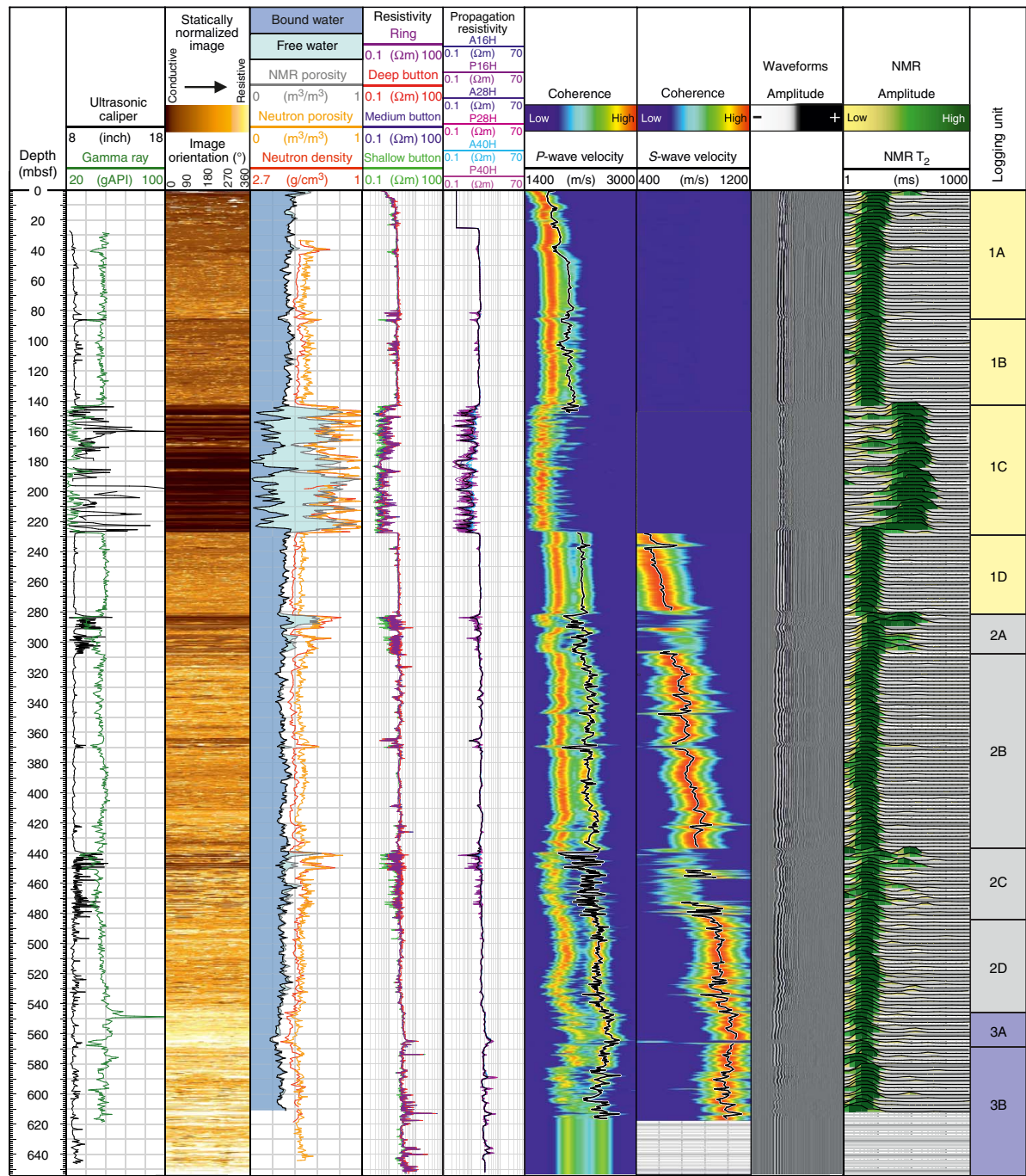
Figure F33. LWD measurements, Hole U1519A.
