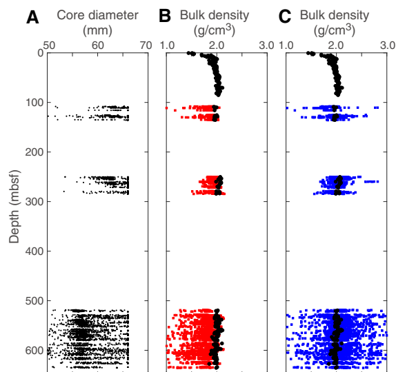
Figure F27. (A) RCB core diameter and (B) uncorrected and (C) corrected GRA bulk density with MAD bulk density (black dots), Hole U1519C.
