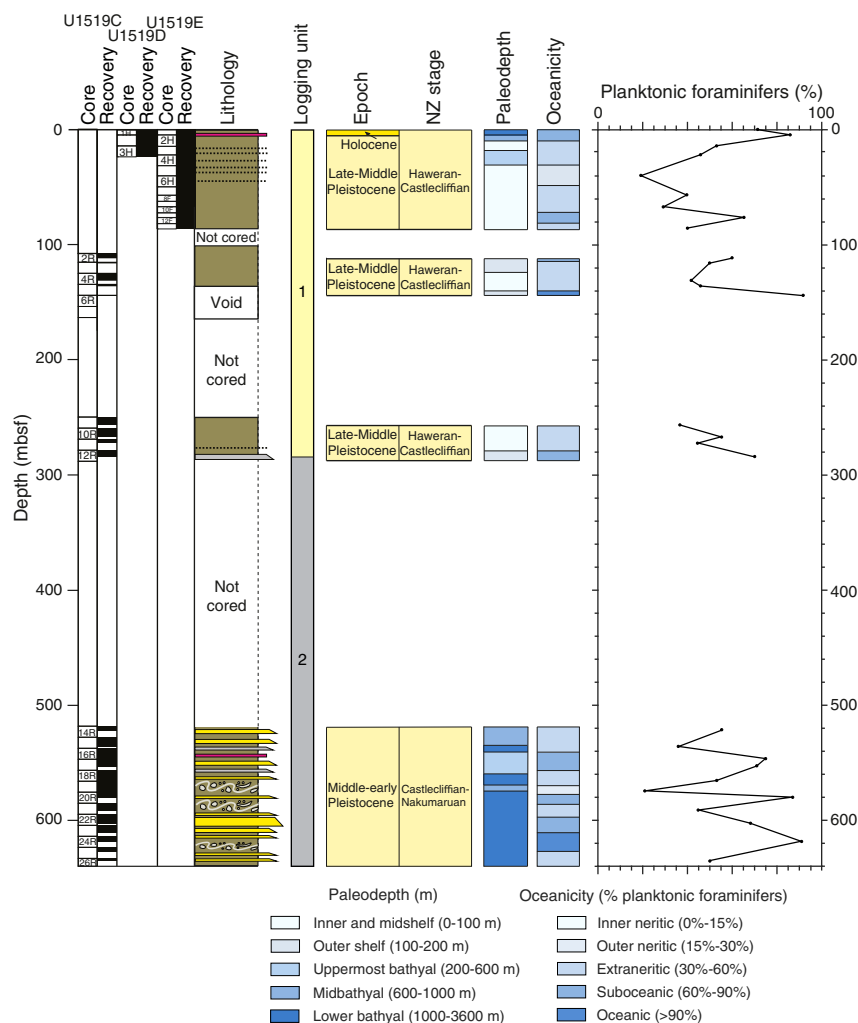
Figure F10. Summary of lithostratigraphy, planktonic foraminifer abundance, interpreted oceanicity, paleowater depths, and biostratigraphic datums, Site U1519. NZ = New Zealand.
