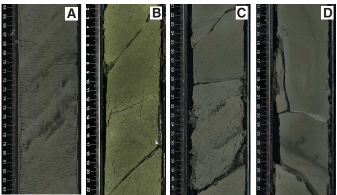
Figure F18. Examples of bedding and related structures recovered from Structural Domain 1. A. Dipping strata in upper part of Domain 1 (375-U1519E-13F-1, 64–84 cm). B. Dipping strata near base of Domain 1 (375-U1519C-15R-6, 2–22 cm). C. Unconformable bedding contact (375-U1519C-18R-1, 21–41 cm). D. Overturned bedding terminating along a planar zone of sheared sediment (375-U1519C-18R-4, 11–31 cm).
