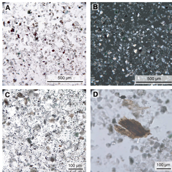
Figure F7. Silt layers in Unit I, Hole U1519E. A, B. Quartz-feldspathic siltstone with calcareous bioclasts (foraminifers and nannofossils), volcanic glass, glauconite, and heavy minerals (3H-4, 110 cm; A: plane-polarized light [PPL]; B: cross-polarized light). C. Pyrite-rich siltstone (5H-4, 40 cm; PPL). D. Terrigenous organic fragments (3H-4, 110 cm; PPL).
