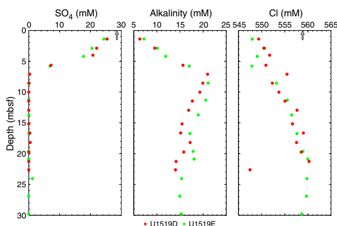
Figure F20. Sulfate, alkalinity, and chloride concentration profiles, Holes U1519D and U1519E (0–30 mbsf). Arrows = average seawater values.
