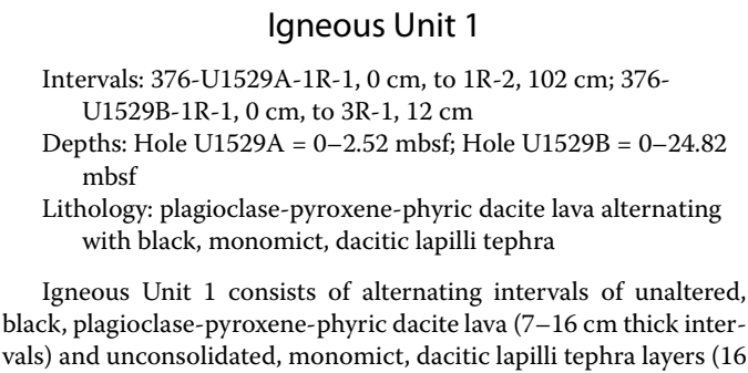
Figure F3. Lithostratigraphic summary, Holes U1529A and U1529B.
