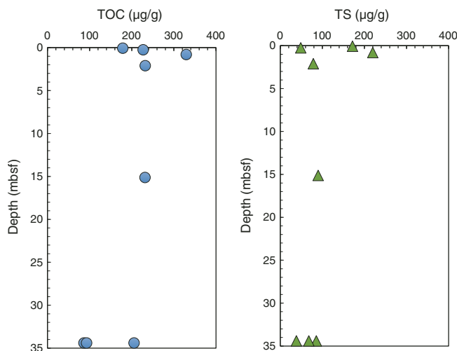
Figure F8. Downhole variations of total sulfur (TS) and TOC of dacitic clasts and lapilli, Holes U1529A and U1529B.
