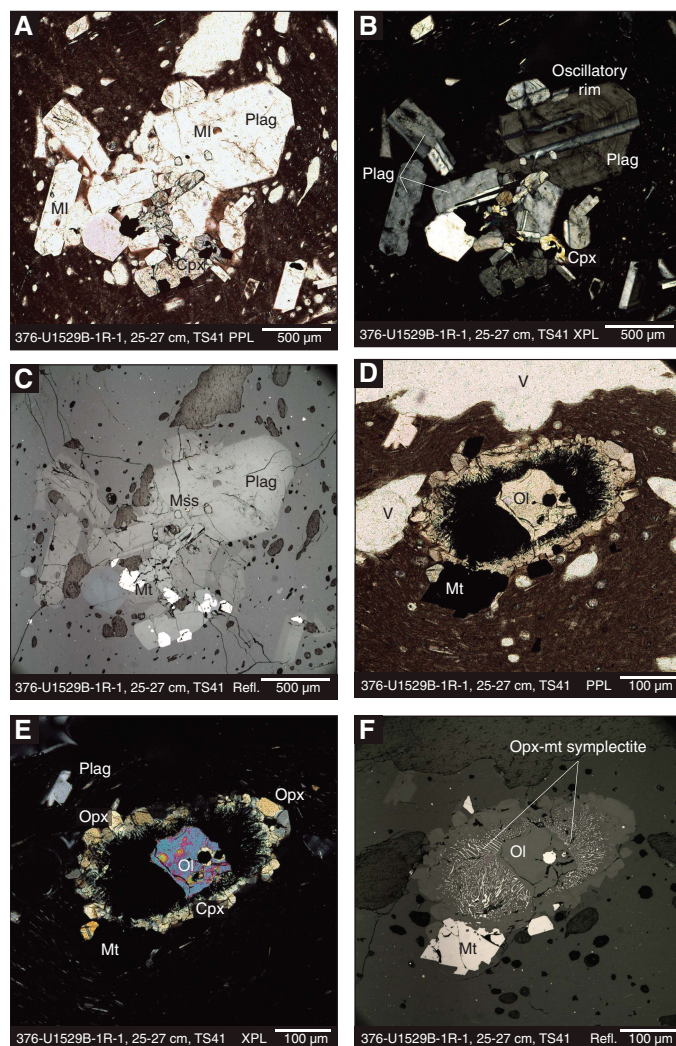
Figure F6. Representative microscopic images, Hole U1529B. A–C. Glomero-cryst of plagioclase (Plag), clinopyroxene (Cpx), Fe-Ti oxides, and aphyric glass. MI = melt inclusion, Mss = monosulfide solid solution, Mt = magnetite. A. Transmitted, PPL. B. Transmitted, XPL. C. Reflected, PPL. Note the melt and sulfide inclusions hosted in plagioclase. D–F. Orthopyroxene–Fe-Ti oxide symplectite entrained in dacite lava. V = vesicle, Ol = olivine, Opx = orthopyroxene. D. Transmitted, PPL. E. Transmitted, XPL. F. Reflected, PPL.
