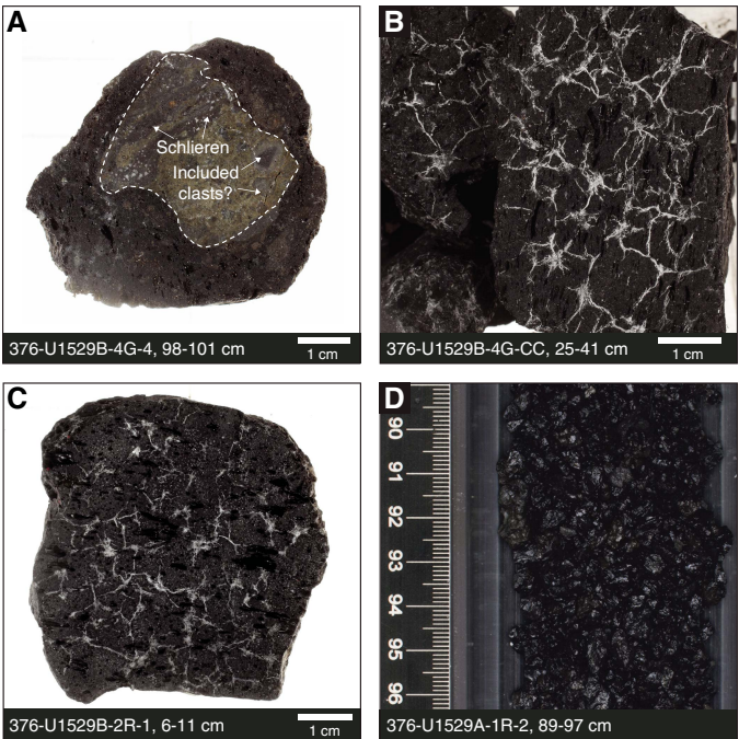
Figure F4. Representative macroscopic samples, Holes U1529A and U1529B. A. Volcaniclastic xenocryst included in dacite lava. B, C. Dacite with fractures accentuated by white halite. D. Lapilli-sized fragments of dacite lava.
