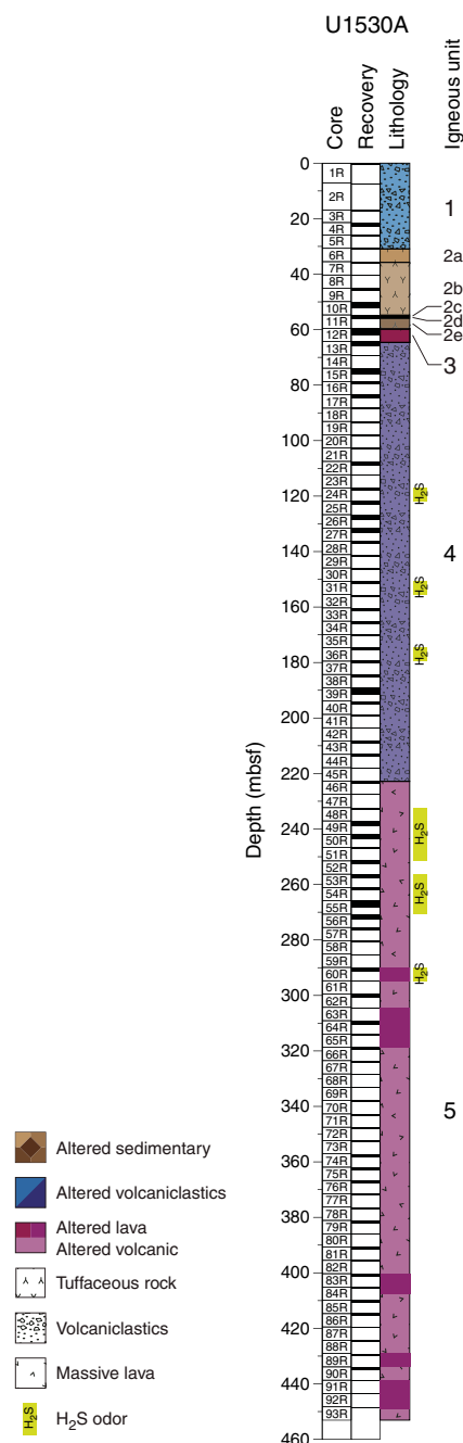
Figure F3. Lithostratigraphic summary, Hole U1530A.
