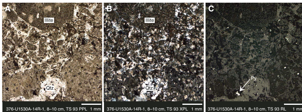
Figure F18. Alteration Subtype IIIa, Hole U1530A. Green-gray clasts are clearly definable from matrix material and are illite rich. Matrix is dominated by coarse-grained quartz (Qtz) intergrown with illite-rich fragments. Pyrite (Py) is a minor phase but generally limited to the matrix.
