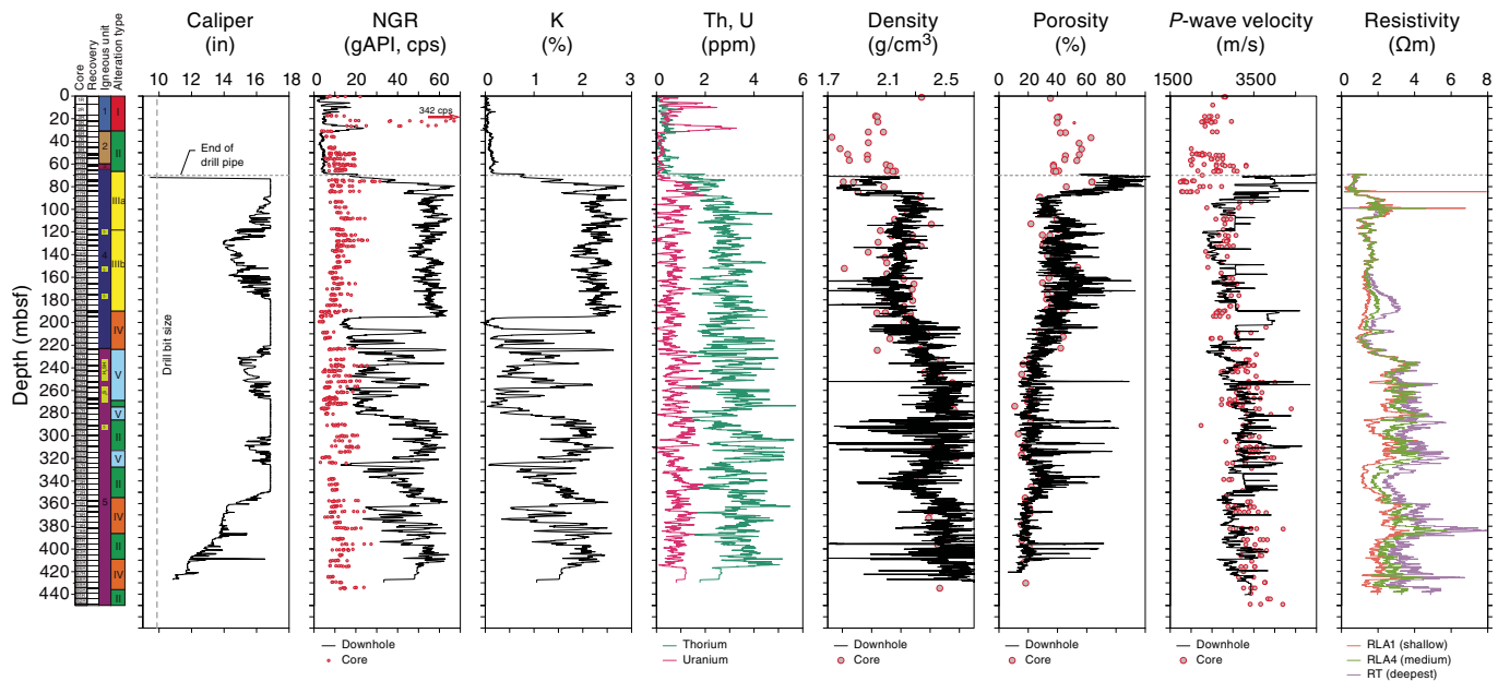
Figure F62. Downhole measurements, Hole U1530A.
