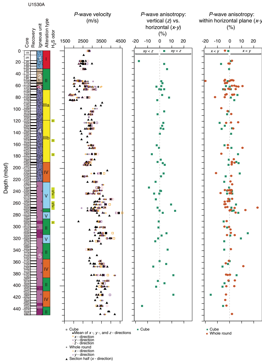
Figure F58. P -wave velocity and anisotropy, Hole U1530A.
