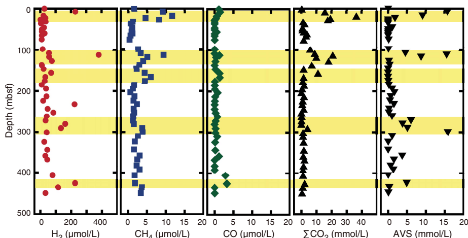
Figure F43. Pore space gas concentrations determined via headspace analysis, Hole U1530A. Shaded yellow bars = locations of possible subseafloor hydrothermal fluid flow in the borehole.
