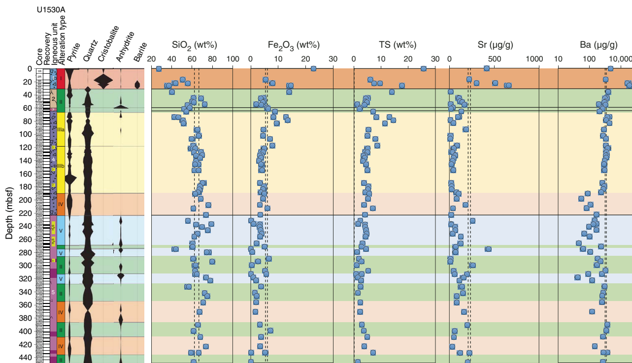
Figure F38. \text{SiO}_2 , \text{Fe}_2\text{O}_3 , total sulfur (TS), Sr, and Ba concentrations in altered volcanoclastic rocks and lavas in Hole U1530A and a comparison with macroscopic estimates of selected mineral abundances in each core. Average values for unaltered dacites recovered in Hole U1527A and Site U1529 are shown. Dashed vertical lines = 2\sigma from average values.
