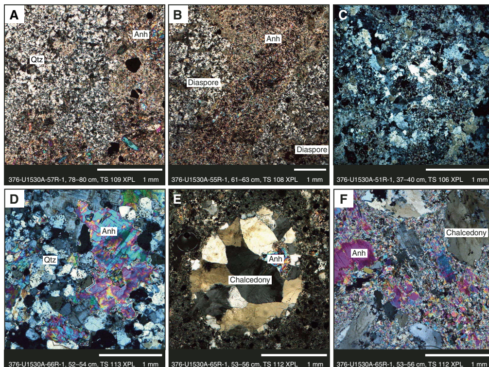
Figure F24. Alteration Type V, Hole U1530A. A. Intergrown anhydrite (Anh) with quartz (Qtz) of variable grain size. B. Fine-grained anhydrite vein cutting quartz with patchy diaspora. C. Quartz intergrown with fine-grained diaspora. D. Coarse-grained anhydrite intergrown with euhedral quartz. E. Vug that is likely a relict vesicle infilled with chalcedony with minor anhydrite. F. Large patches of chalcedony associated with prolific anhydrite; note the two clear sizes of anhydrite grain: early large crystals and a groundmass of finer grained anhydrite.
