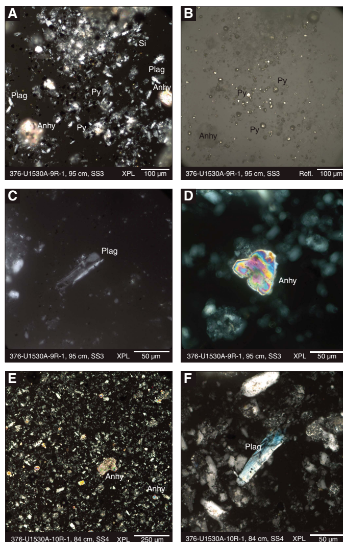
Figure F7. Representative smear slide images from Igneous Unit 2, Hole U1530A. A–D. Smear Slide (SS) 3 showing (A, B) relative proportions of silica (Si), plagioclase (Plag), pyrite (Py), and anhydrite (Anhy); (C) plagioclase microlite; and (D) an anhydrite crystal. E, F. SS4 (E) overview image and (F) plagioclase microlite with unusual blue interference color as a consequence of the greater thickness of the smear slide relative to a thin section.
