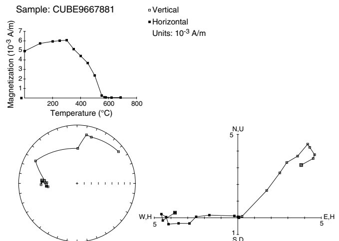
Figure F54. TD experiment on Sample 376-U1530A-12R-1, 37–39 cm, from Igneous Unit 5. This sample shows a simple TD curve with a rapid decline in NRM intensities at 500^\circ – 600^\circ\text{C} .
