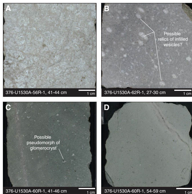
Figure F10. Representative macroscopic samples from Igneous Unit 5, Hole U1530A. A. Altered volcanic rock with no preserved volcanic features. B. Altered volcanic rock with possible relics of infilled vesicles. C. Pervasively altered, originally plagioclase phyric lava with silica-filled vugs after pseudomorphs of glomerocrysts D. Pervasively altered, originally plagioclase phyric lava.
