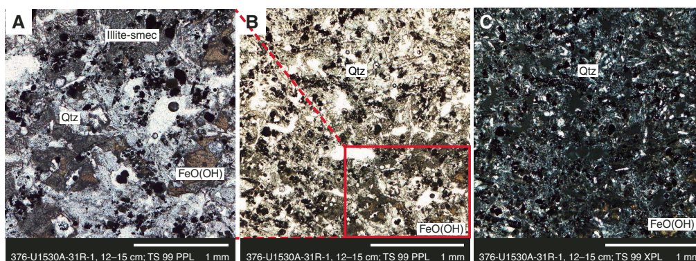
Figure F20. A–C. Alteration Subtype IIIb, Hole U1530A. Illite-smectite (smec) matrix with intergrowth of quartz (Qtz) and disseminated pyrite locally oxidized to \text{FeO}(\text{OH}) .
