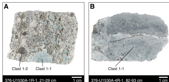
Figure F4. Representative macroscopic samples from Igneous Unit 1, Hole U1530A. A. Altered polymict volcanoclastic rock containing Clast Types 1-1 and 1-2. B. Bomb-sized clast in a clast-supported polymict lapillistone.
