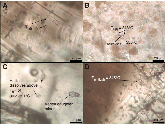
Figure F26. Types of Fls. A. Subtype 1a. B. Subtype 1b. C. Type 2. Complex array of Fls in anhydrite with multiple anisotropic daughter minerals that are probably sulfates. D. Type 3. Homogenizes to the critical point. diss = dissolved.
