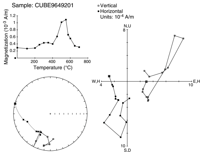
Figure F48. TD experiment on Sample 376-U1530A-10R-2, 31–33 cm, from Igneous Unit 2. This sample shows a complex TD curve with significant increase in NRM intensities for temperatures above \sim 400^\circ\text{C} , suggesting the irreversible transformation of original minerals after heating.
