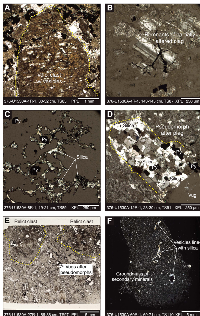
Figure F5. Representative thin sections of igneous units, Hole U1530A. A. Vesicular altered volcanic (Volc.) clast from Unit 1. B. Remnant of partially altered plagioclase (Plag) from Unit 1. C. Framework of secondary silica minerals of a tuffaceous sandstone from Subunit 2b. D. Pseudomorph after plagioclase filled with secondary silica minerals and pyrite (Py) from Unit 3. E. Relict volcanic clasts and empty pseudomorphs (vugs) after plagioclase from Unit 4. F. Texturally less altered lava interval from Unit 5 showing completely altered groundmass and vesicles filled with secondary silica minerals.
