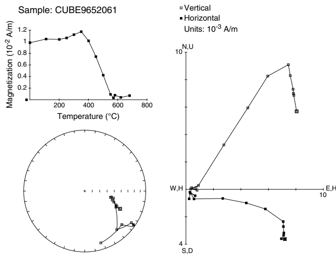
Figure F50. TD experiment on Sample 376-U1530A-12R-1, 37–39 cm, from Igneous Unit 3. This sample shows a simple TD curve with a rapid decline in NRM intensities at 500^\circ – 600^\circ\text{C} .
