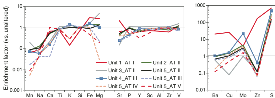
Figure F42. Chemical enrichment factors for major igneous units according to Alteration Types (ATs) I–V, Site U1530. The average composition of each alteration type in each igneous unit was calculated and then normalized to the average composition of the least altered dacites (black horizontal line) recovered in Igneous Unit 1 of Hole U1527A and Site U1529.
