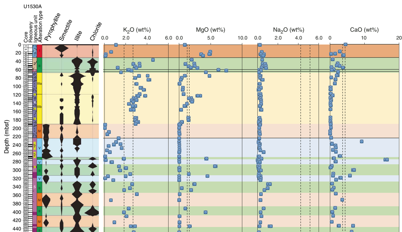
Figure F37. K_2O , MgO , Na_2O , and CaO concentrations in altered volcanoclastic rocks and lavas in Hole U1530A and comparison with macroscopic estimates of selected mineral abundances in each core potentially controlling major element abundances. Average values for unaltered dacites recovered from Hole U1527A and Site U1529 are shown. Dashed vertical lines = 2\sigma from average values.
