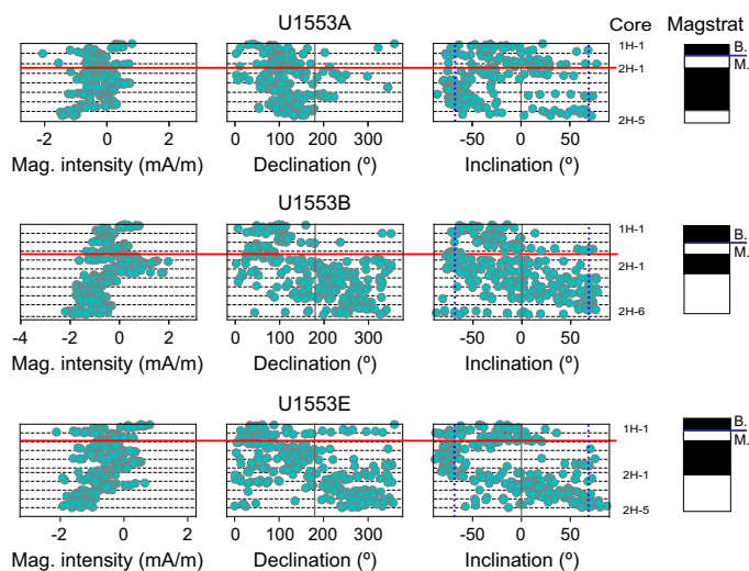
Figure F35. Paleomagnetic data at an alternating field of 6 mT from the uppermost two cores, Holes U1553A, U1553B, and U1553E. B. = Brunhes Chron, M. = Matuyama Chron, Magstrat = magnetostratigraphy. Red lines = unconformity levels of each hole based on magnetic reversals.
