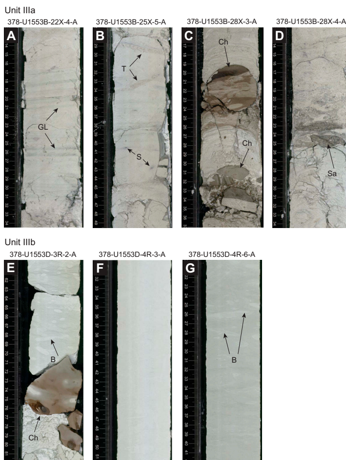
Figure F11. Characteristic lithologies in Unit III, Holes U1553B and U1553D. A–D. Subunit IIIa shows a consistent presence of green laminations (GL) and thin beds, Teichichnus -type trace fossils (T), sulfides (S), chert (Ch), and sandstone (Sa). E–G. Subunit IIIb is characterized by a transition to (F) bright white (N 9.5), homogeneous sediment in which bioturbation is expressed as green and white beds with burrows (B).
