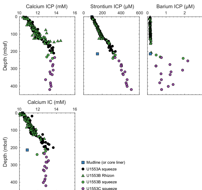
Figure F43. Pore water calcium, strontium, and barium concentrations, Site U1553. ICP = inductively coupled plasma-atomic emission spectroscopy, IC = ion chromatography.
