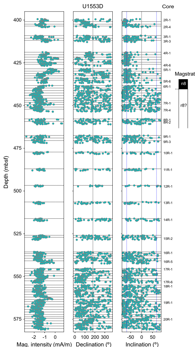
Figure F37. Paleomagnetic data at an alternating field of 6 mT, Hole U1553D. The marked magnetic reversal correlates to the second reversal (n8/r8) in Hole U1553C. AF = alternating field, Magstrat = magnetostratigraphy.
