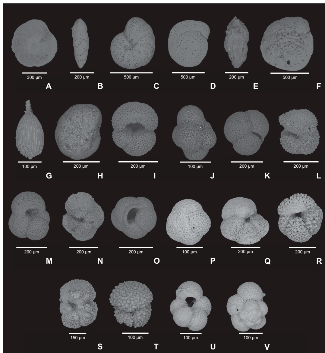
Figure F28. Foraminifer species. A. Nuttallides truempyi (U1553D-7R-CC). B. Buliminoides chattonensis (U1553B-2H-CC). C. Anomalinoidea orbiculus (U1553D-7R-CC). D. Cibicides maculatus (U1553A-22X-CC). E. Uvigerina bortotara (U1553B-2H-CC). F. Cibicides parki (U1553B-29X-CC). G. Lagena sulcata (U1553B-2H-CC). H. Gavelinella beccariiiformis (U1553C-31R-CC). I. Globigerinathea index (U1553A-26X-CC). J. Cassigerinelloita amekiensis (U1553C-21R-CC). K. Subbotina angiporoides (U1553A-20H-CC). L. Acarinina coalingensis (U1553C-22R-CC). M. Globoturborotalita labiacrassata (U1553C-4R-CC). N. Morozovella subbotinae (U1553C-21R-CC). O. P. cf. Neoglobobadrina pachyderma (U1553C-40R-CC). Q. Globanomalina australiformis (U1553D-2R-CC). R. Globigerinathea senni (U1553D-2R-CC). S. Morozovella crater (U1553D-2R-CC). T. Acarinina primitiva (U1553D-2R-CC). U, V. Unidentified planktonic foraminifers (U1553-40R-CC). For taxonomic information, see Table T19.
