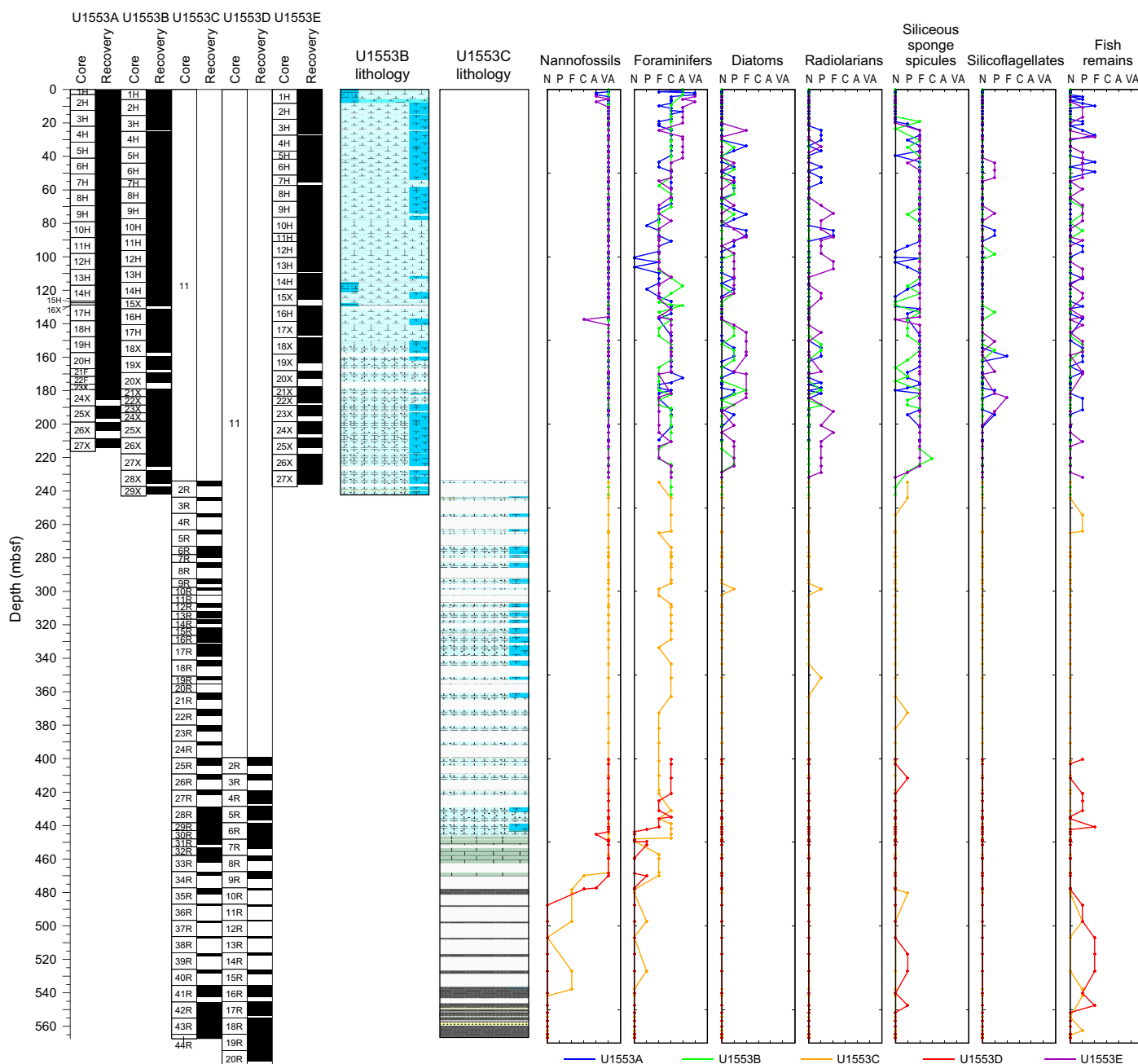
Figure F8. Abundance of selected components in smear slide observations, Site U1553. VA = very abundant (>50%), A = abundant (25%–50%), C = common (10%–25%), F = few (1%–10%), P = present (<1%), N = not observed (0%).
