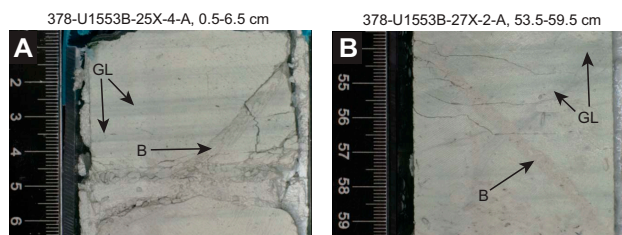
Figure F12. Trace fossil burrows (B) cutting green layers (GL) in Unit III, Hole U1553B. A. Green layers overprint the burrow, suggesting a diagenetic origin of the green layers. B. Burrow cuts across the green layers.
