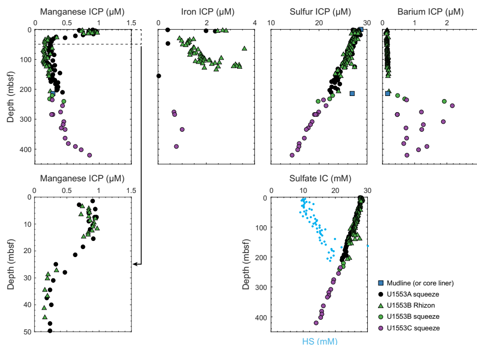
Figure F46. Pore water manganese, iron, sulfur and sulfate, and barium concentrations, Site U1553. Hydrogen sulfide ( \text{HS}^- ) concentrations are calculated from total alkalinity and dissolved inorganic carbon. ICP = inductively coupled plasma spectroscopy, IC = ion chromatography.
