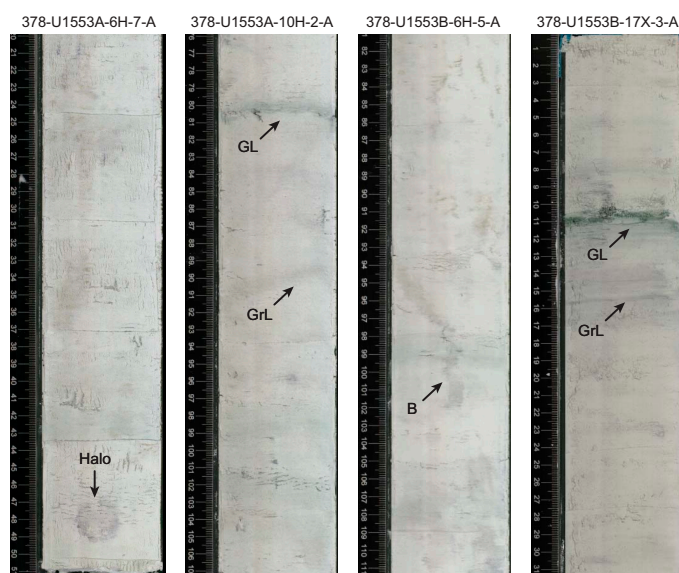
Figure F6. Characteristic lithologies in Unit II, Holes U1553A and U1553B. Halo = diagenetic halo, GL = green layers, GrL = gray layers, B = burrow.
