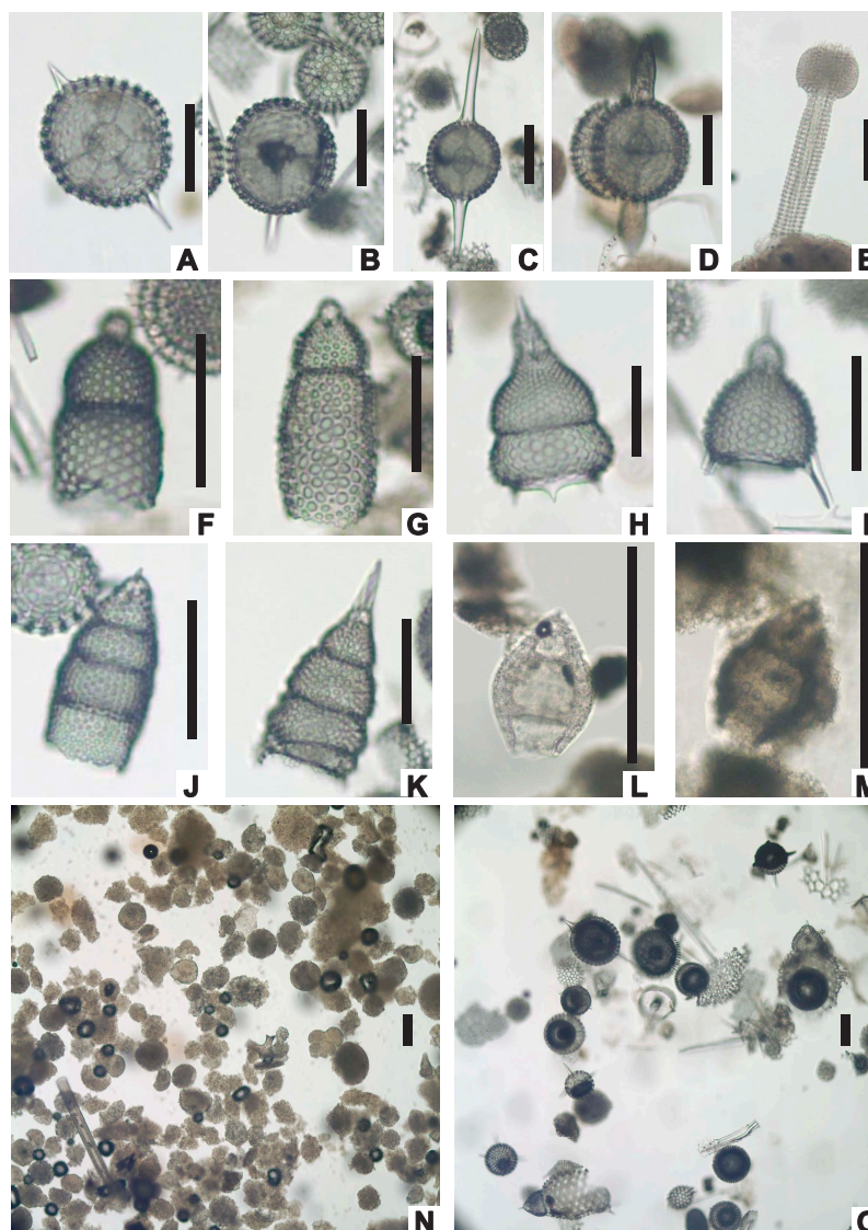
Figure F29. Selected radiolarian index species and radiolarian assemblages. Scale bar = 100 µm. Specimen locations are identified by slide letter and England Finder location. A. Axoprunum? irregularis (378-U1553E-4H-CC; B-M47/4). B. Axoprunum bispiculum (378-U1553D-7R-CC; A-S37/0). C. Axoprunum pierinae gr. (378-U1553E-23X-CC; B-W28/2). D. Axoprunum aff. pierinae (378-U1553E-26H-CC; A-D28/0). E. Amphicraspedum prolixum s.s. (378-U1553D-2R-CC; A-Q46/1). F. Aphetocyrtis gnomabax (378-U1553E-21X-CC; A-E40/1). G. Aphetocyrtis rossi (378-U1553E-23X-CC; A-W19/0). H. Lamprocyclus matakoho (378-U1553E-5H-CC; A-T11/1). I. Lychnocanium aff. conicum (378-U1553-7H-CC; A-E36/4). J. Eucyrtidium antiquum (378-U1553E-9H-CC; A-W41/1). K. Eucyrtidium spinosum (378-U1553-23X-CC; B-O4/1). L. Buryella tetratica (378-U1553D-5R-CC; A-W17/4). M. Buryella foremanae (378-U1553D-9R-CC; A-Y42/4). N. Radiolarians with poor preservation (378-U1553C-29R-CC). O. Pyritized radiolarians (378-U1553B-23X-CC). For taxonomic information, see Table T7 in the Expedition 378 methods chapter (Röhl et al., 2022).
