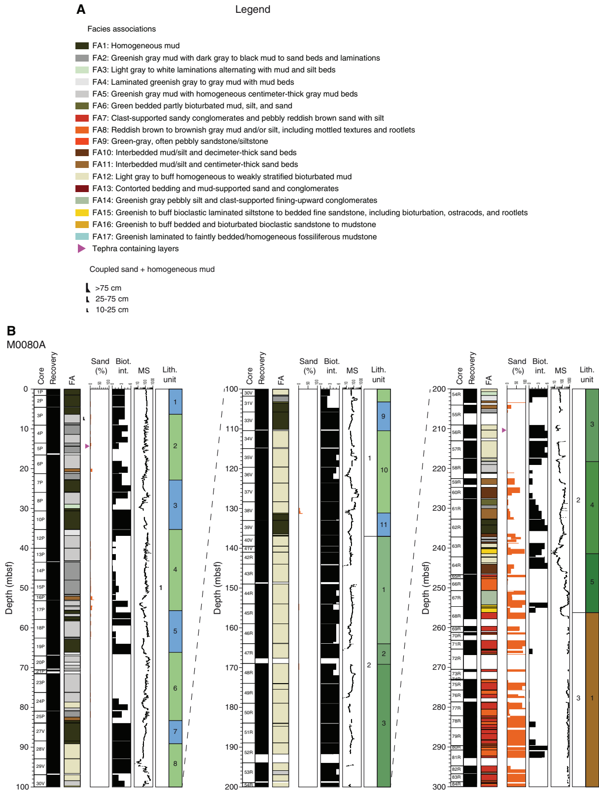
Figure F3. Composite stratigraphic log, Hole M0080A. FA = facies association, Biot. int. = bioturbation intensity, MS = magnetic susceptibility. A. Legend. B. 0–300 mbsf. Lithostratigraphic subunits in Unit 1: blue = marine, green = isolated/semi-isolated. Unit 2–4 colors are purely for visual differentiation and do not have any paleoenvironmental meaning. (Continued on next page.)
