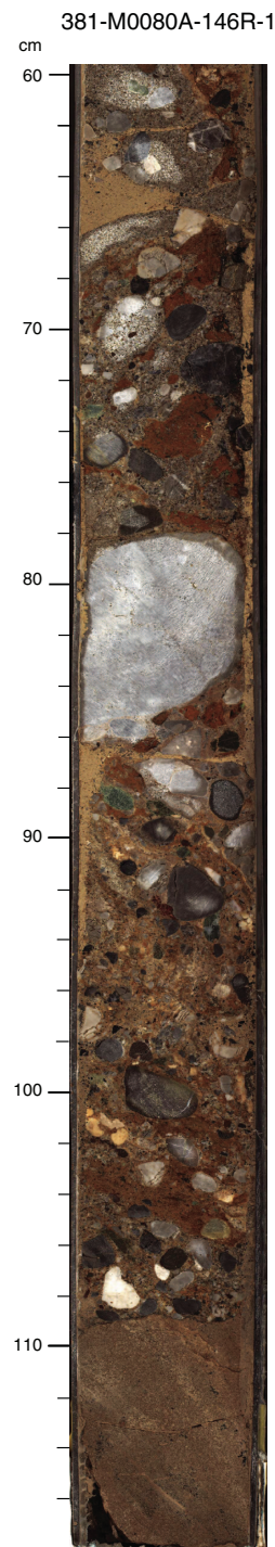
Figure F9. Clast-supported pebble to cobble conglomerate (FA7) at base of Hole M0080A (Subunit 4-3). Clast lithologies include various limestones, red chert, mafic/ultramafic rocks, and coarse pebbly sandstone. Top of core image is at 533.50 mbsf.
