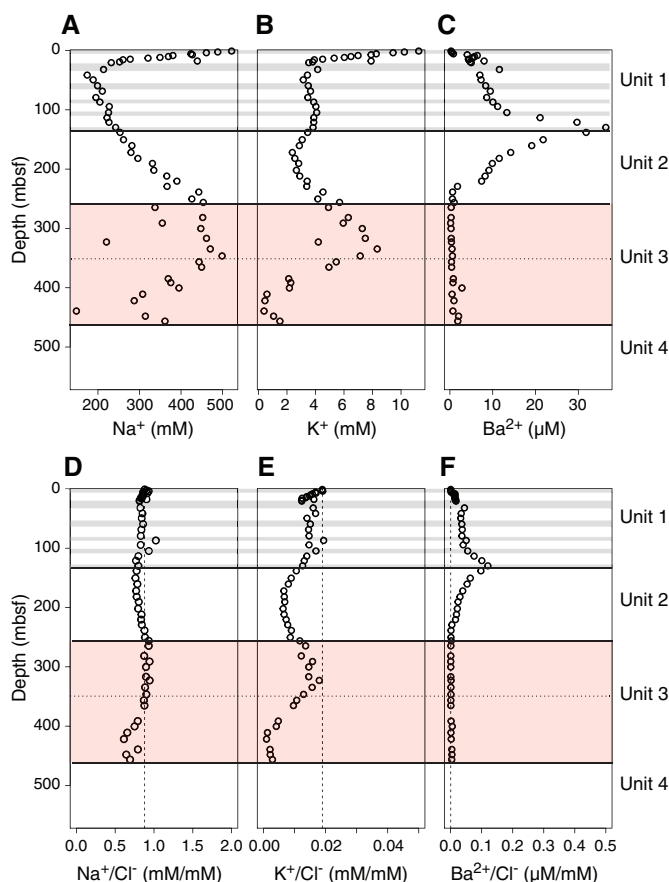
Figure F22. Pore water (A) sodium, (B) potassium, and (C) barium and (D) \text{Na}^+/\text{Cl}^- , (E) \text{K}^+/\text{Cl}^- , and (F) \text{Ba}^{2+}/\text{Cl}^- ratios, Hole M0080A. Solid lines = unit boundaries, gray = marine subunits in Unit 1, pink = Unit 3, horizontal dashed line = subunit boundary separating conglomerates above and silt below (see Lithostratigraphy). Vertical dashed line = seawater values.
