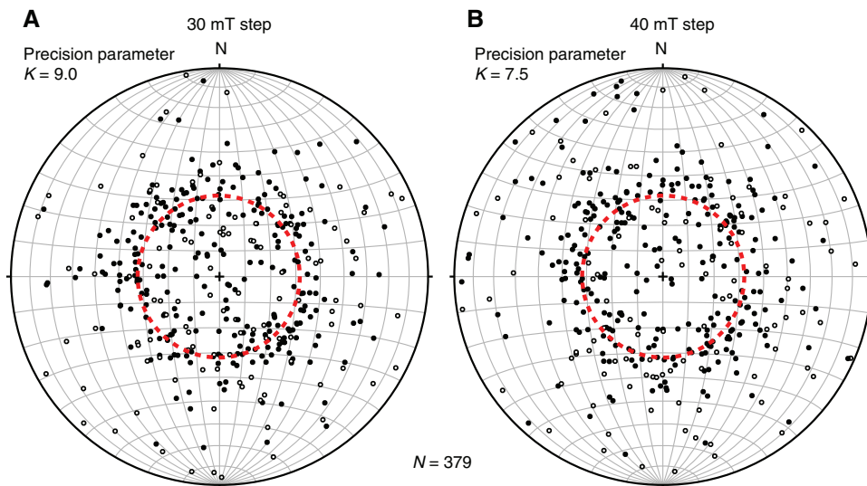
Figure F45. Lower hemisphere equal-area stereographic projections of remanence directions for all Hole M0080A samples after application of (A) 30 mT and (B) 40 mT AF. Red dashed circle = geocentric axial dipole expected inclination (i.e., 57.5°) for the site latitude. Solid dots = directions with a positive (normal polarity) inclination, open dots = directions with a negative (reversed polarity) inclination.
