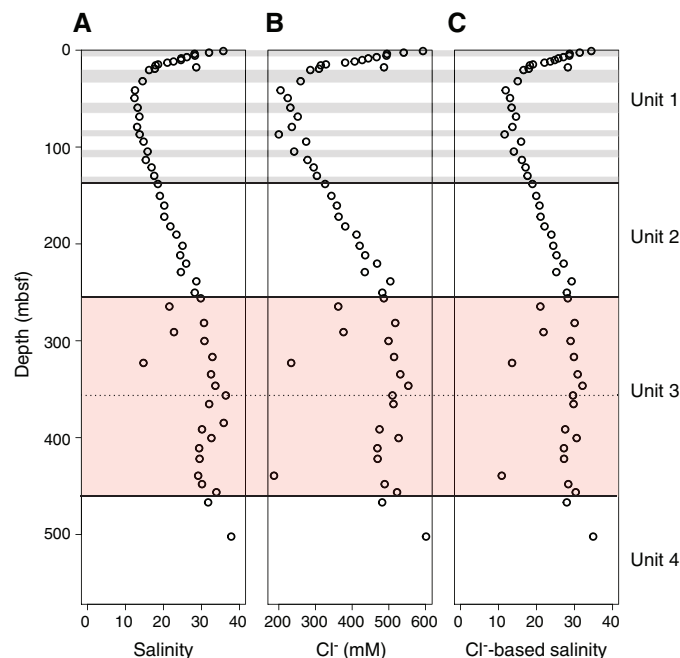
Figure F18. Pore water (A) salinity, (B) chloride, and (C) \text{Cl}^- -based salinity, Hole M0080A. Solid lines = unit boundaries, gray = marine subunits in Unit 1, pink = Unit 3, dashed line = subunit boundary separating conglomerates above and silt below (see Lithostratigraphy).
