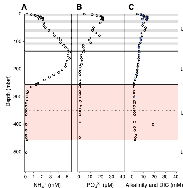
Figure F20. Pore water (A) ammonium, (B) phosphate, and (C) alkalinity (dots) and DIC (crosses), Hole M0080A. Solid lines = unit boundaries, gray = marine subunits in Unit 1, pink = Unit 3, dashed line = subunit boundary separating conglomerates above and silt below (see Lithostratigraphy).
