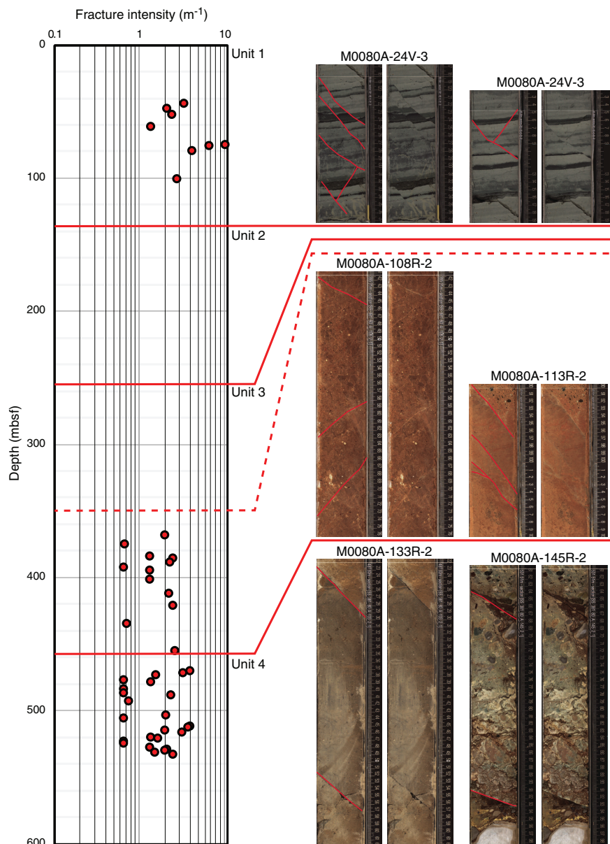
Figure F10. Fracture intensity (number of fractures per meter; log scale) and core images with examples of fault traces observed in the different lithostratigraphic units (left: interpreted, right: uninterpreted), Hole M0080A. Thick red lines = lithostratigraphic unit boundaries, dashed red line = boundary between Subunit 3-1 unconsolidated conglomerates (above) and Subunit 3-2 siltstones (below). Interpreted: thin red lines = faults. Note the absence of fractures from 101.70 to 367.60 mbsf (Unit 2 and Subunit 3-1).
