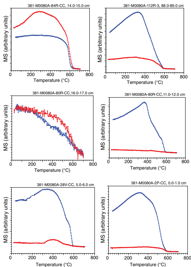
Figure F43. Low-field susceptibility vs. temperature ( k - T ) experiment results for six samples obtained before the OSP, Hole M0080A. Red = heating path from room temperature to 700°C, blue = cooling path from 700°C back to room temperature.
