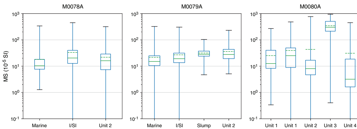
Figure F34. MSCL magnetic susceptibility box and whisker plots grouped by subunits, Expedition 381. Top and bottom of boxes correspond to 1st and 3rd quartiles, solid line in middle of box shows the median, dashed line shows the mean. Ends of whiskers indicate minimum and maximum values. I/SI = isolated/semi-isolated, slump = slumped subunit.
