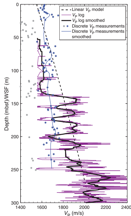
Figure F50. V_p data sets available for 0–300 mbsf, Site M0080. Comparison of pre-expedition linear V_p model (see Core-log-seismic integration in the Expedition 381 methods chapter [McNeill et al., 2019b] for details), filtered (discrete sample V_p (gray = low values that were filtered out, blue = retained data, blue line = 10-point average smoothed), downhole sonic V_p log, and 7.5 m average smoothed downhole log. The comparison suggests that discrete sample V_p measurements yielded more realistic velocity values than the downhole log to about 140 mbsf.
