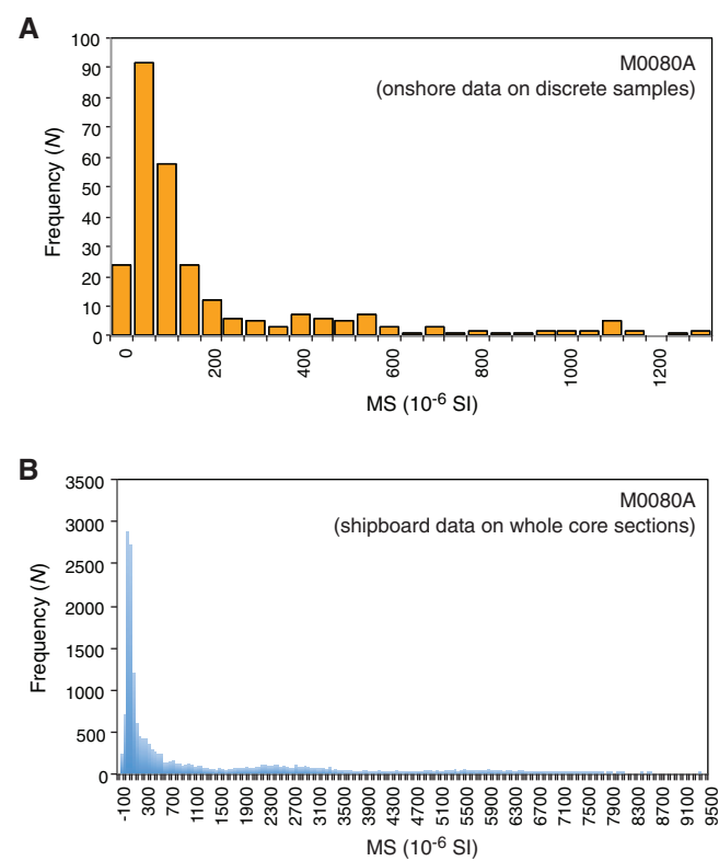
Figure F40. Magnetic susceptibility frequency distribution from (A) discrete samples and (B) whole core sections (MSCL), Hole M0080A.
