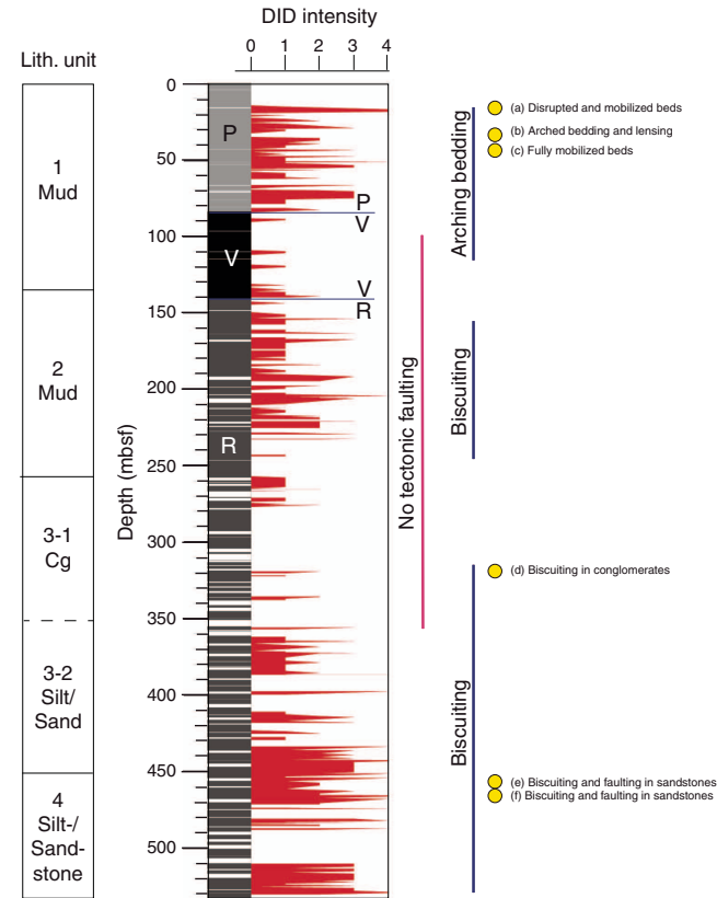
Figure F14. DID intensity (0–4), Hole M0080A. Coring method is represented in shades of gray from push (P) to percussive (V) to rotary (R). White = no core recovery. Right: distribution of principal DID features (biscuiting and arching bedding) and natural faulting. Cg = conglomerate. Yellow dots = locations of DID in Figure F15.
