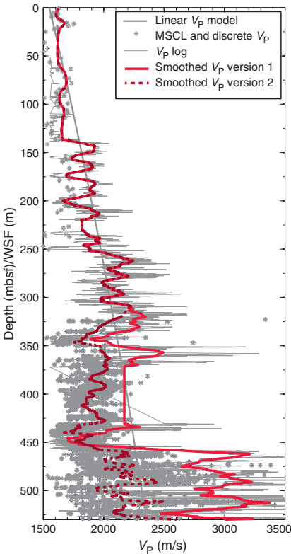
Figure F52. Two versions of composite V_p data used for synthetics generation with original data sets in gray (see Figures F50 and F51 for details), Site M0080. Both versions are based on smoothed V_p from discrete samples measurements in the upper 140 mbsf and smoothed downhole log from 140 to 310 mbsf. The difference is in the deeper section: smoothed downhole sonic log was used in Version 1 and smoothed MSCL data were used in Version 2.
