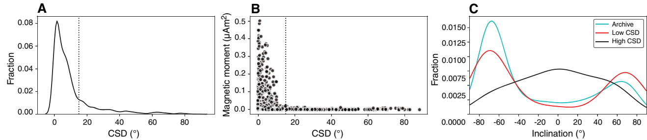
Figure F18. Behavior of CSD at 15 mT demagnetization step for discrete specimens, Hole U1538A. A. Histogram of CSDs. B. CSD vs. remanence intensity. C. Histogram of inclinations for all archive-half measurements, discrete specimens with low CSD (<15°), and discrete specimens with high CSDs.
