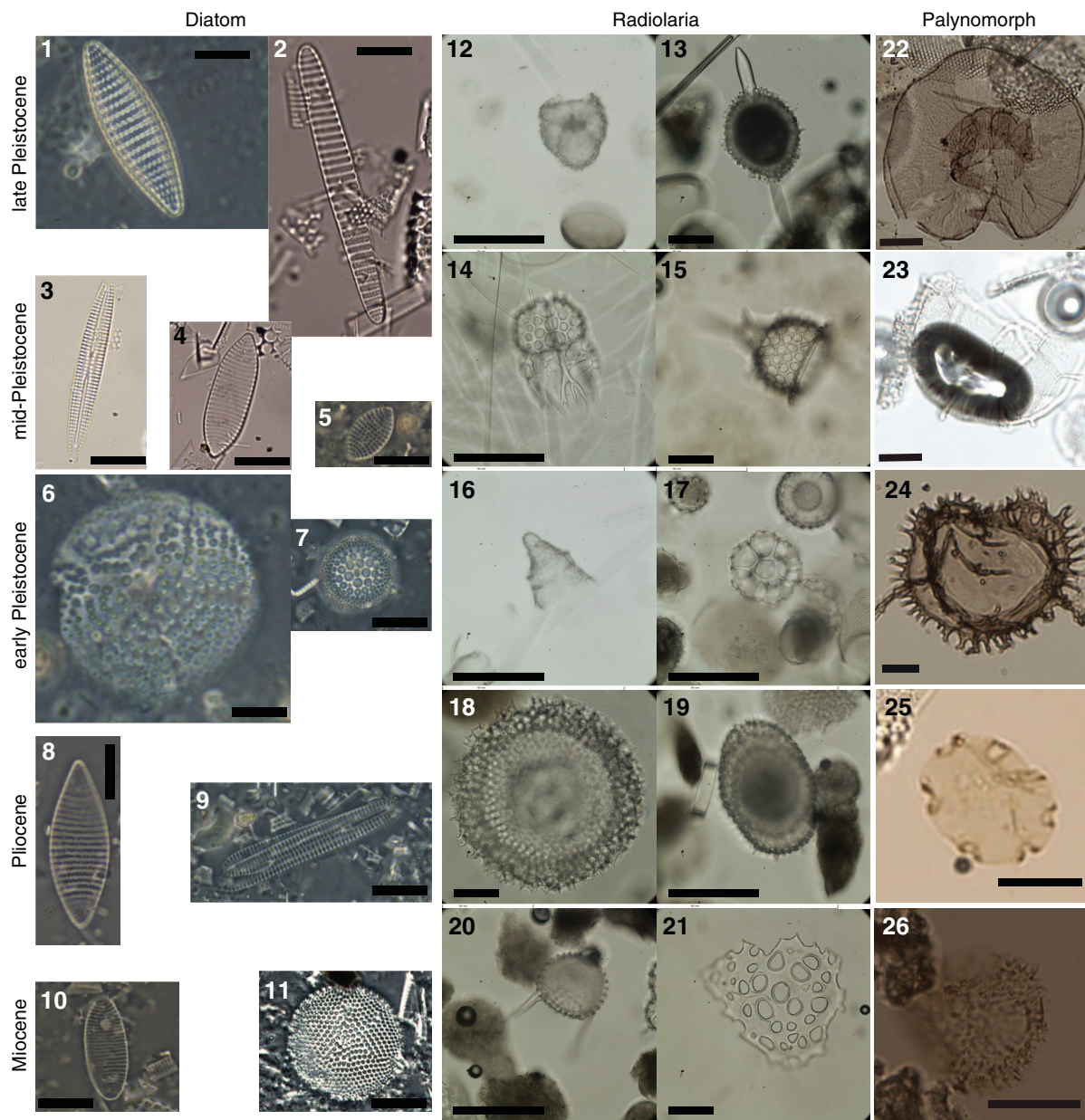
Figure F12. Biostratigraphically important diatoms and radiolarians and selected palynomorphs found at Expedition 382 sites. Diatoms (scale bars = 10 \mu m): 1. Fragilariopsis kerguelensis (382-U1538A-16H-CC), 2. Fragilariopsis obliquecostata (382-U1537A-3H-CC), 3. Rouxia constricta (382-U1536A-14H-CC), 4. Fragilariopsis rhombica (382-U1537A-3H-CC), 5. Fragilariopsis separanda (382-U1536A-10H-1, 75 cm), 6. Actinocyclus fasciculatus (382-U1538A-49X-3, 75 cm), 7. Shionodiscus oestrupii var. reimeri (382-U1538A-45X-CC), 8. Fragilariopsis barronii (382-U1536A-40F-CC), 9. Rouxia antarctica (382-U1538A-51X-1), 10. Fragilariopsis aurica (382-U1536C-40F-CC), 11. Thalassiosira miocenica (382-U1536E-22R-CC). Radiolarians (scale bars = 50 \mu m): 12. Antarctissa cylindrica (382-U1537A-10H-CC), 13. Stylatractus universus (382-U1536A-14H-CC), 14. Phormospyris antarctica (382-U1538A-6H-CC), 15. Cycladophora pliocenica (382-U1534A-29F-CC), 16. Cycladophora davisiana (382-U1537A-13H-CC), 17. Helotholus? vema (382-U1537D-40F-CC), 18. Lampromitra coronata (382-U1536E-4R-CC), 19. Larcopyle polyacantha titan (382-U1538A-73X-CC), 20. Lychnocanium grande (73X-CC), 21. Acrosphaera labrata (382-U1536E-18R-CC). Palynomorphs (scale bars = 20 \mu m): 22. Selenopemphix sp. 1 sensu Esper and Zonneveld (2007) (382-U1536A-3H-CC), 23. Impagidinium spp. (382-U1534A-9H-CC), 24. Selenopemphix dionaeacysta (16F-CC), 25. Nothofagidites flemingii (382-U1538A-60X-CC), 26. Operculodinium? eirikianum (382-U1536E-26R-CC).
