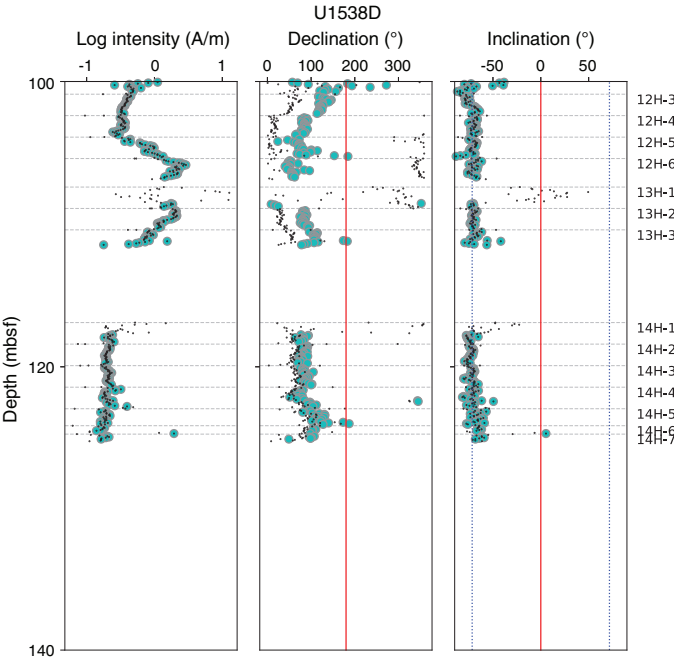
Figure F17 (continued).
