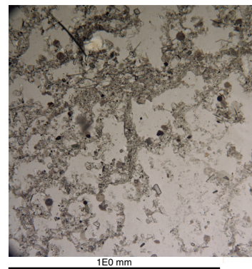
Figure F4. Biosilica-rich silty clay (382-U1538A-24H-1, 128 cm).
