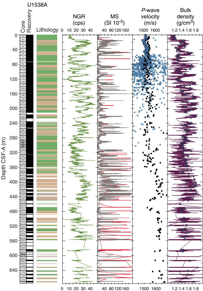
Figure F28. Physical property data, Hole U1538A. MS: red = WRMSL, gray = SHMSL (MSP). P -wave velocity: dots = WRMSL, squares = PWC. Wet bulk density: line = WRMSL, dots = discrete. cps = counts per second.
