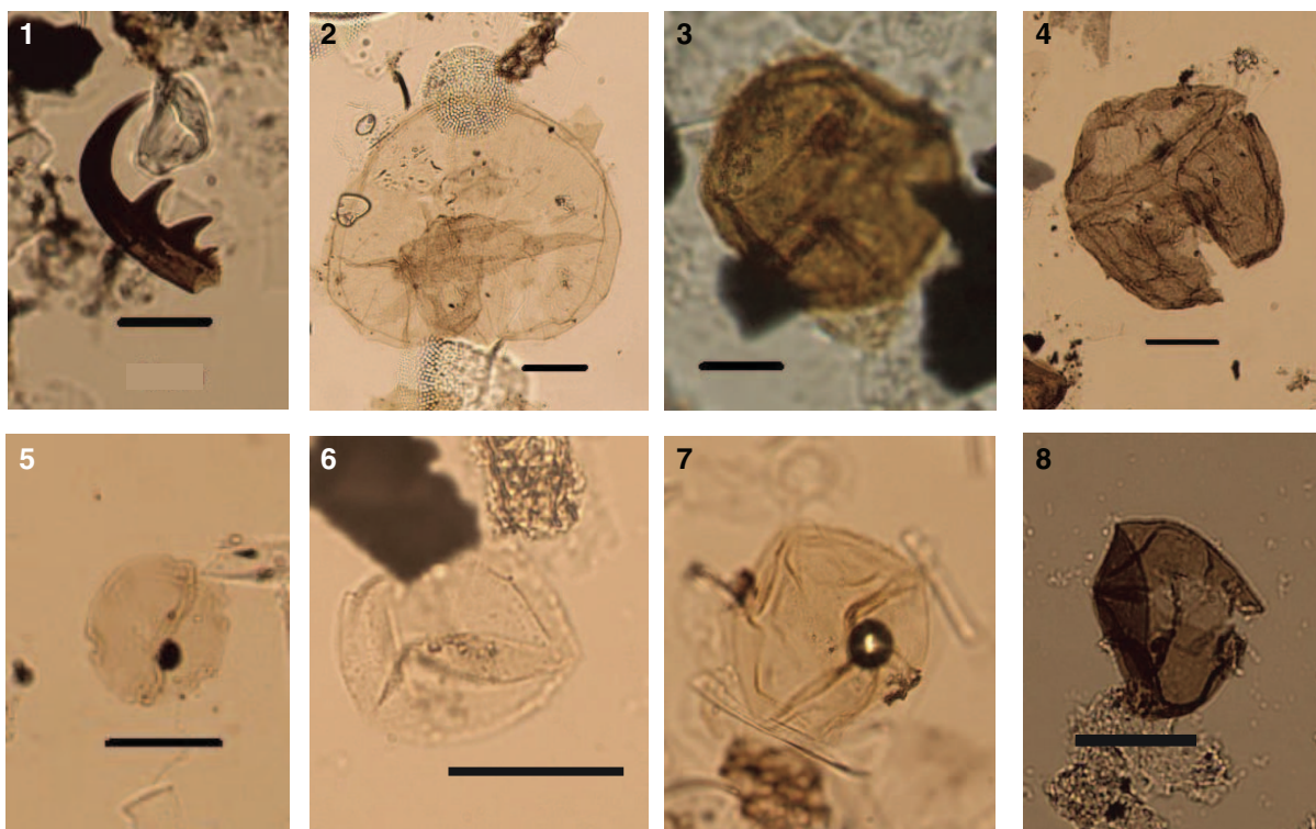
Figure F13. Selected palynomorphs. All scale bars = 20 \mu m. 1. Copepod remain (382-U1538A-4H-CC). 2. Selenopemphix sp. 1 sensu Esper and Zonneveld (2007) (4H-CC). 3. Deflandrea antarctica (10H-CC). 4. Nucicla umbiliphora (17H-CC). 5. Nothofagidites flemingii (38X-CC). 6. Batiacasphaera micropapillata (56X-CC). 7. Leiosphaeridia sp. (29H-CC). 8. Brigantedinium simplex (71X-CC).
