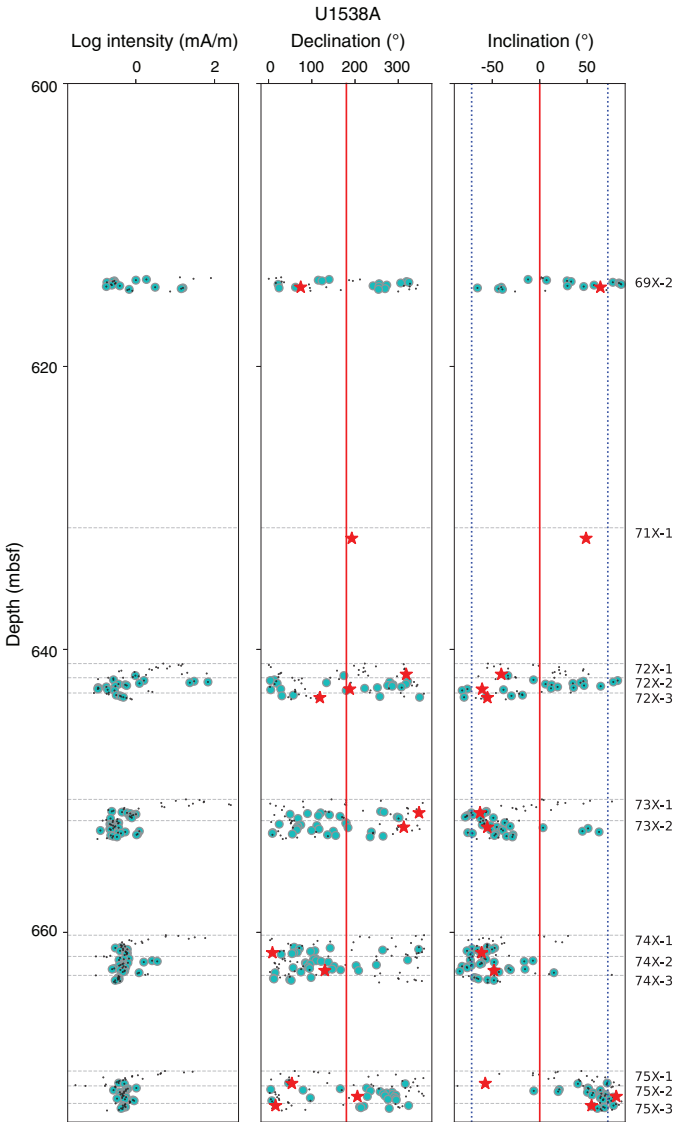
Figure F14 (continued).
