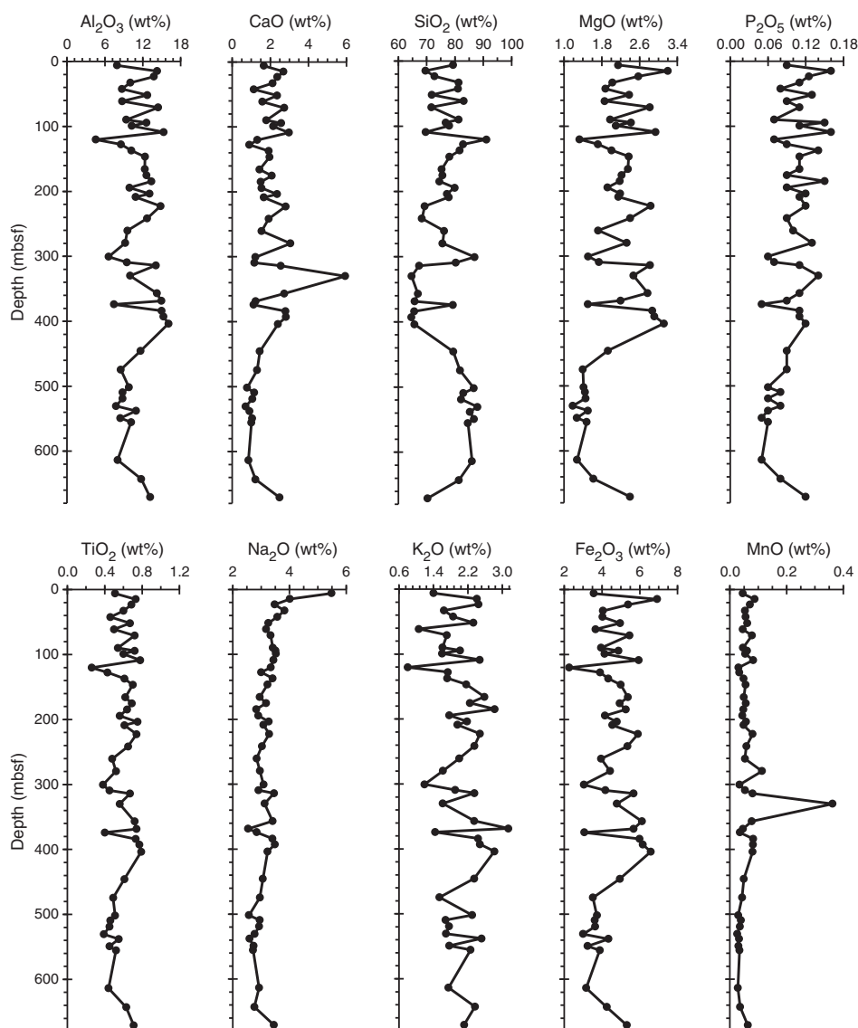
Figure F25. Bulk sediment major element compositions ( \text{Al}_2\text{O}_3 , \text{CaO} , \text{SiO}_2 , \text{MgO} , \text{P}_2\text{O}_5 , \text{TiO}_2 , \text{Na}_2\text{O} , \text{K}_2\text{O} , \text{Fe}_2\text{O}_3 , and \text{MnO} ), Site U1538.
