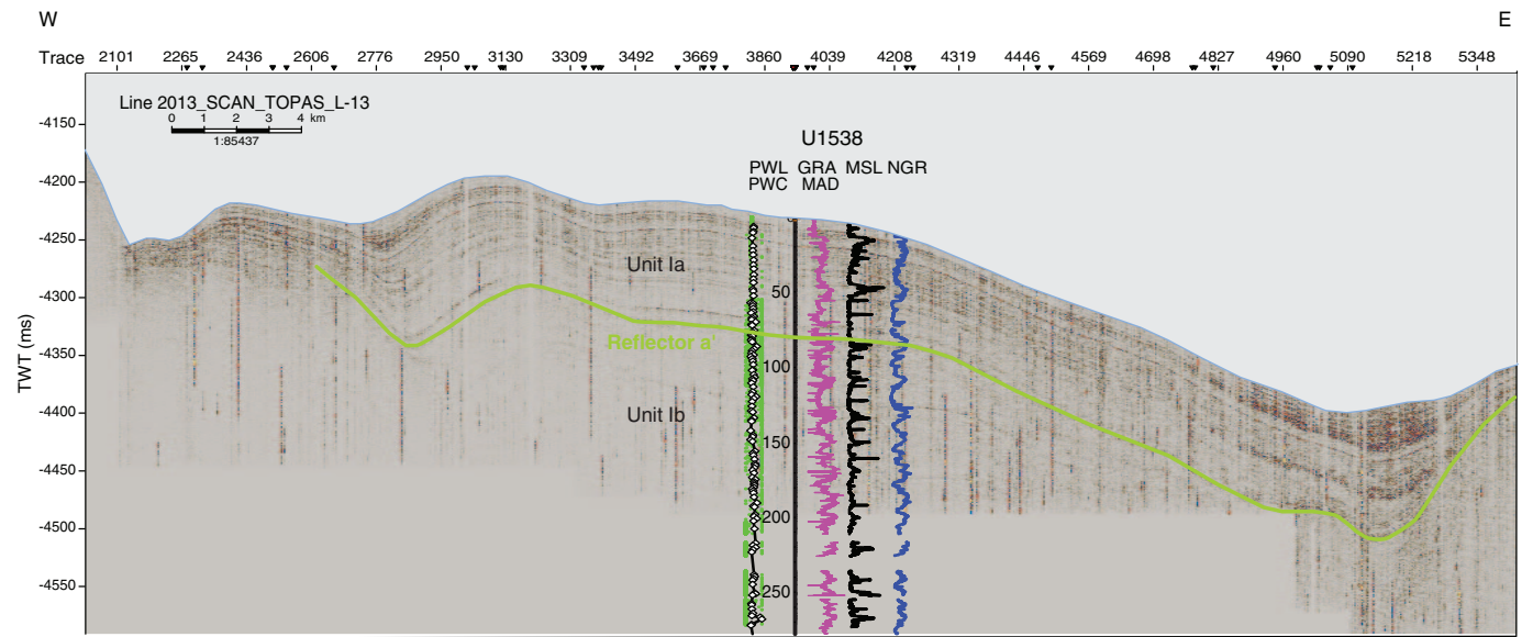
Figure F44. TOPAS Line SCAN2013-L13 and physical properties, Hole U1538A. Green dots = PWL, diamonds linked with black line = PWC, magenta line = GRA, black line = MSL, blue line = NGR.
