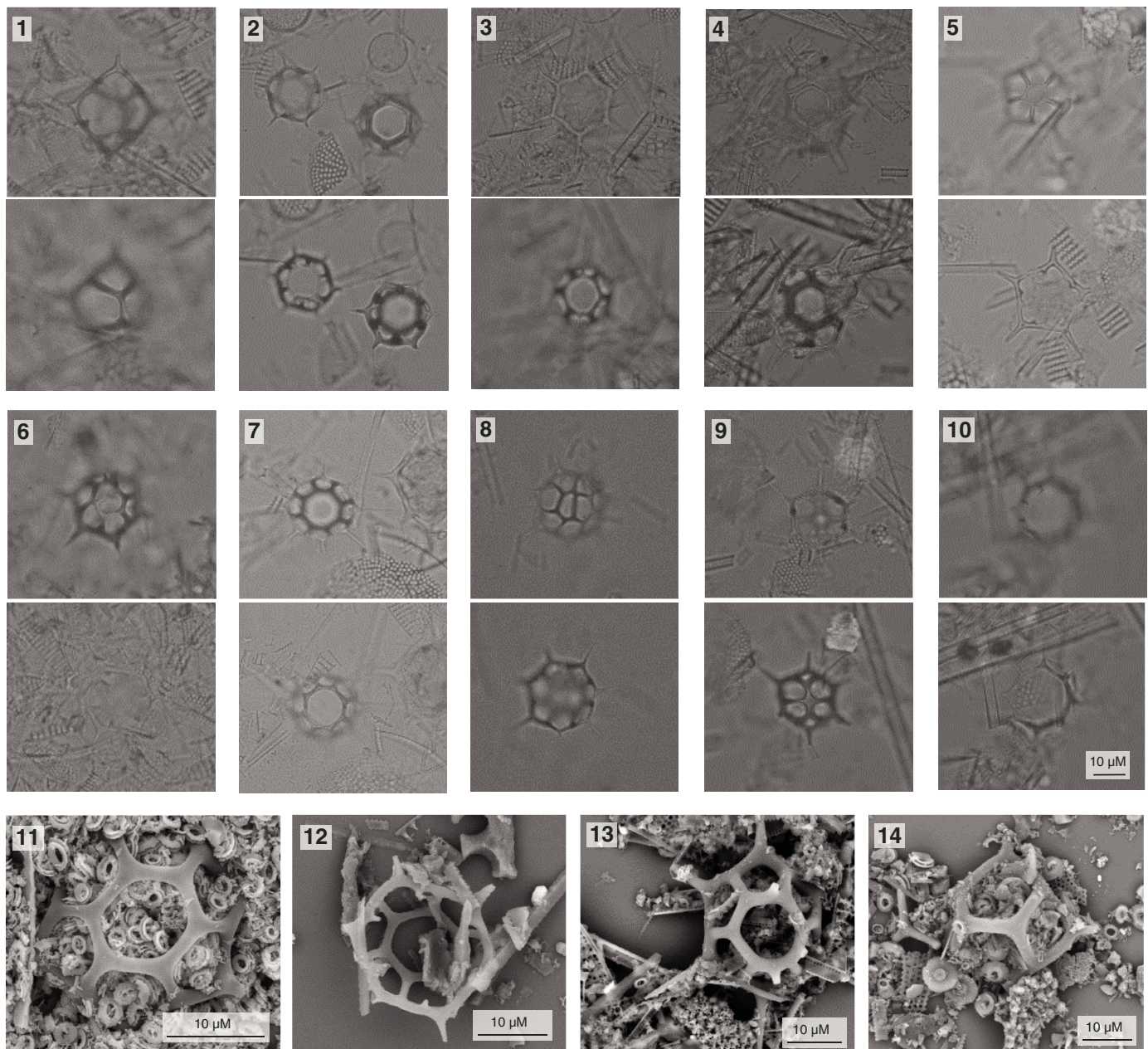
Figure F22. Silicoflagellates, Holes U1539A and U1539C. A–J: Light microscope, K–N: scanning electron microscope. 1. Dictyocha stapedia (383-U1539C-7H-CC). 2. Stephanocha speculum var. speculum (short-spined) (383-U1539C-14H-CC). 3. S. speculum var. bispicata (383-U1539A-2H-CC). 4. S. speculum B (large variety) (383-U1539C-23H-CC). 5, 7. 383-U1539C-10H-CC. (5) S. speculum var. pentagona . 6. S. speculum var. binocula (383-U1539A-5H-CC). (7) S. speculum var. octonaria . 8. S. speculum var. septenaria ( binocula ; 383-U1539A-11H-CC). 9. Malformed S. speculum (383-U1539C-30F-CC). 10. Octactis pulchra (383-U1539C-24H-CC). 11. S. speculum in nannofossil ooze (383-U1539A-9H-1, 134 cm). 12. S. speculum var. speculum in abapical view (383-U1539C-18H-CC). 13. S. speculum var. bispicata (383-U1539A-3H-CC). 14. Dictyocha stapedia (383-U1539C-29F-2, 16 cm).
