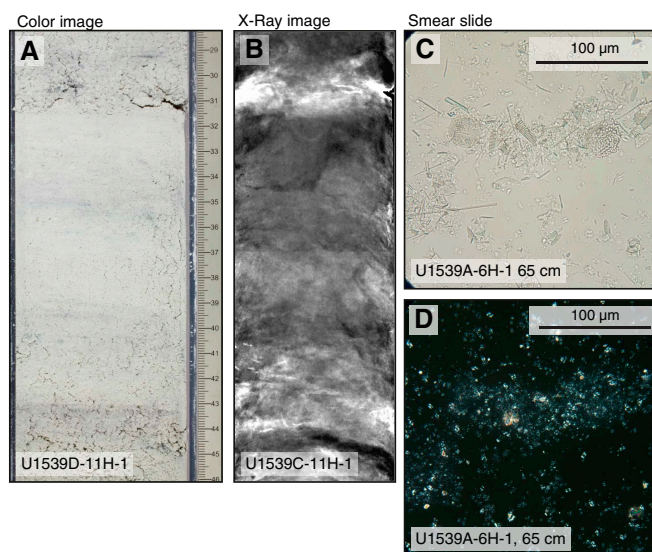
Figure F8. Representative (A) core and (B) X-ray and photomicrograph images of mineral properties of Lithofacies 3 (diatom-bearing to diatom-rich nannofossil or calcareous ooze) in (C) PPL and (D) XPL, Holes U1539A, U1539C, and U1539D.
