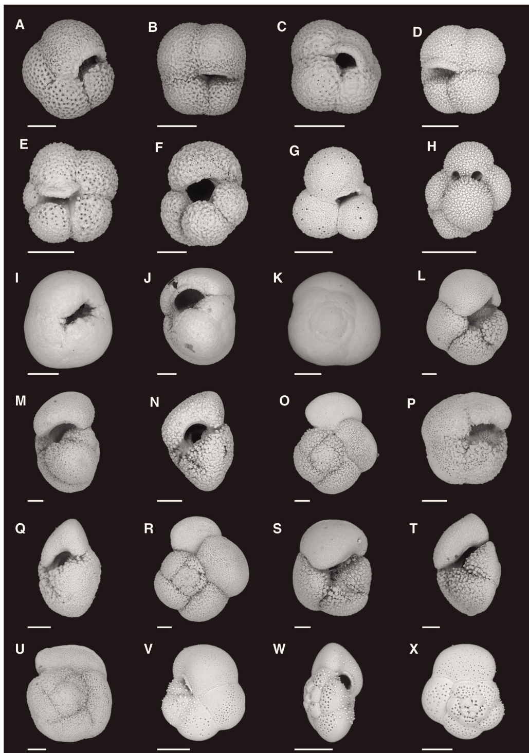
Figure F25. Planktonic foraminifers, Site U1539. Scale bars = 100 \mu m. A–C. Varieties of Neogloboquadrina pachyderma with the final chamber (A) larger than, (B) similarly sized, and (C) smaller than the penultimate chamber. D. Neogloboquadrina incompta . E. Turborotalita quinqueloba . F. Globigerina bulloides . G. Globigerinita glutinata (note signs of dissolution on all chambers in final whorl). H. Globigerinita uvula . I–K. Globoconella inflata in (I) umbilical, (J) side, and (K) spiral view. L–O. Globoconella punctulata puncticuloides with typical final chamber in (L) umbilical, (M, N) side, and (O) spiral view. P–R. G. punctulata puncticuloides with kummerform final chamber in (P) umbilical, (Q) side, and (R) spiral view. S–U. Truncorotalia crassaformis in (S) umbilical, (T) side, and (U) spiral view. V–X. Hirsutella scitula in (V) umbilical, (W) side, and (X) spiral view (note signs of dissolution on earliest chambers).
