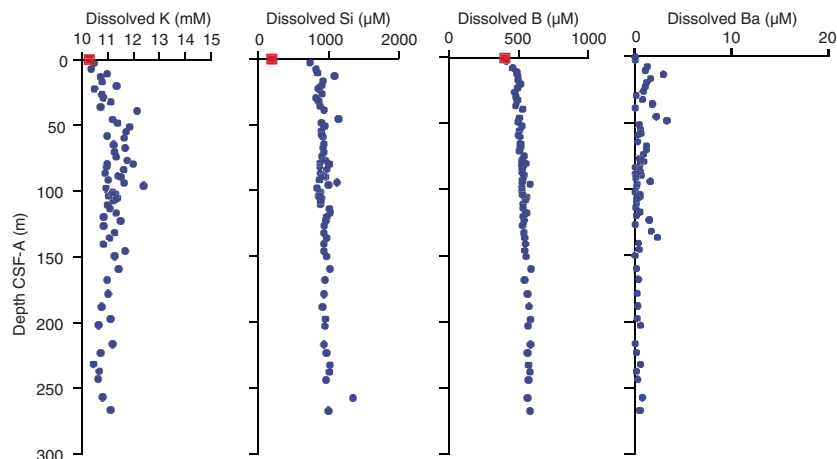
Figure F37. Interstitial water potassium, silica, boron, and barium, Site U1539. Barium was below detection limit in the overlying water. Red square = overlying seawater sample.
