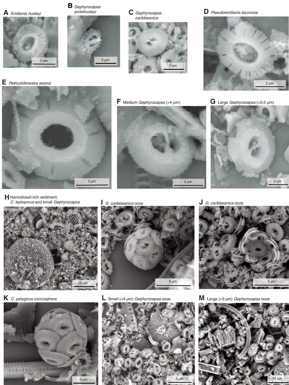
Figure F24. Scanning electron microscope images of calcareous nannofossils, Site U1539. A. E. huxleyi (383-U1539A-2H-CC). B. Gephyrocapsa protohuxleyi (383-U1539A-5H-4). C. G. caribbeanica (383-U1539C-8H-5, 29 cm). D. P. lacunosa (383-U1539C-28F-CC). E. R. asanoi (383-U1539C-18H-CC). F, G. Gephyrocapsa ; (F) medium (4–5.5 \mu\text{m} ) (383-U1539C-18H-CC), (G) large (>5.5 \mu\text{m} ) (383-U1539C-29F-2, 16 cm). H. Nannofossil-rich sediment. Calcidiscus leptoporus and small Gephyrocapsa (Hole U1539C mudline). I, J. Ooze of G. caribbeanica (383-U1539C-8H-5, 29 cm). K. Coccosphere of C. pelagicus (383-U1539C-18H-CC). L. Ooze of small (<4 \mu\text{m} ) G. caribbeanica (383-U1539C-15-CC). M. Ooze of large (>5.5 \mu\text{m} ) Gephyrocapsa (383-U1539C-29F-2, 16 cm).
