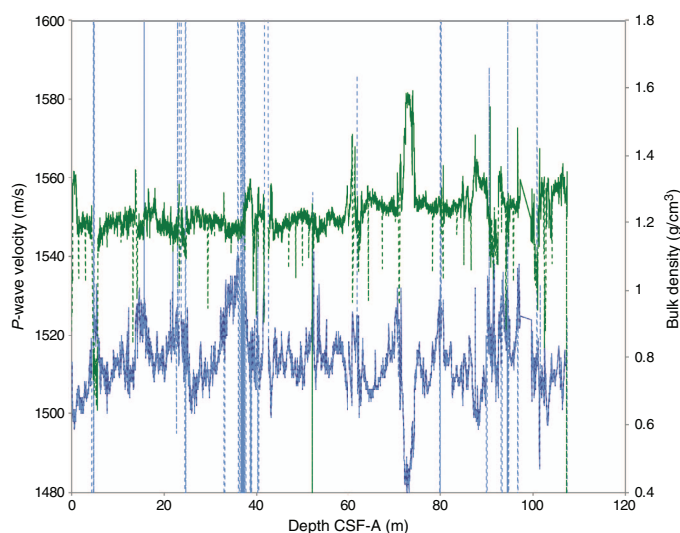
Figure F46. Gamma ray attenuation bulk density (green) and P -wave velocity (blue), Hole U1539A. Dashed lines = raw data, solid lines = processed data.
