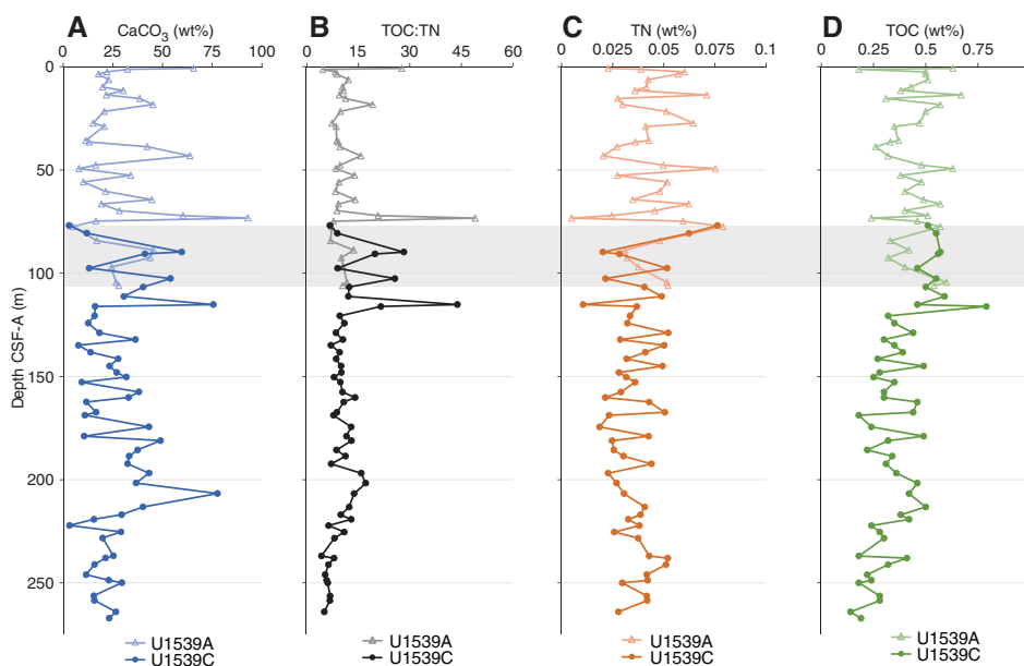
Figure F38. Solid phase geochemistry of (A) \text{CaCO}_3 , (B) total organic carbon (TOC):total nitrogen (TN), (C) TN, and (D) TOC. Gray bar indicates sample overlap between Holes U1539A and Hole U1539C.
