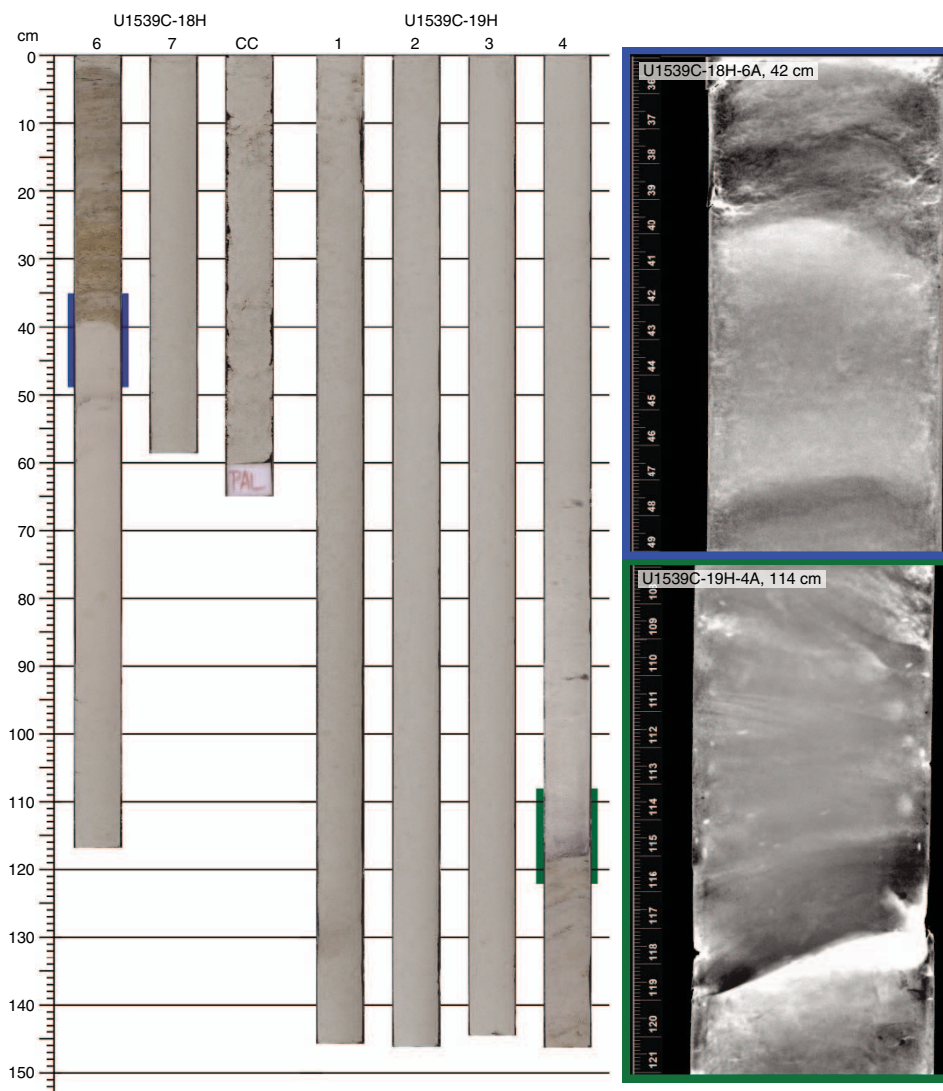
Figure F9. Representative images and mineral properties of Lithofacies 5 (foraminiferal ooze and sand associated with turbidites), Hole U1539C. Note the sharp contact of Lithofacies 5 with over- and underlying units in X-radiographs from Sections 18H-6 (blue) and 19H-4 (green).
