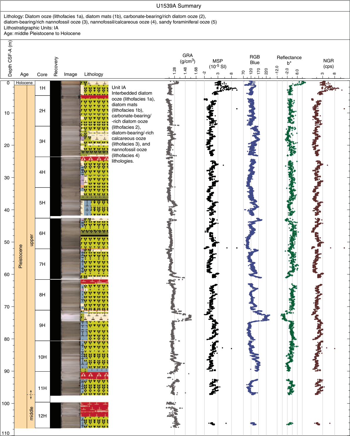
Figure F4. Hole summaries, Site U1539. GRA = gamma ray attenuation, MSP = point magnetic susceptibility, RGB = red-green-blue, NGR = natural gamma radiation. cps = counts per second. (Continued on next three pages.)
