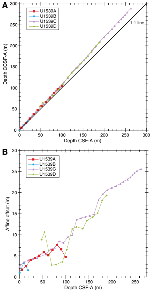
Figure F52. A. Comparison of coring depth and composite depth scales in the Site U1539 splice. B. Comparison of the growth of cumulative depth offset and core depth.
