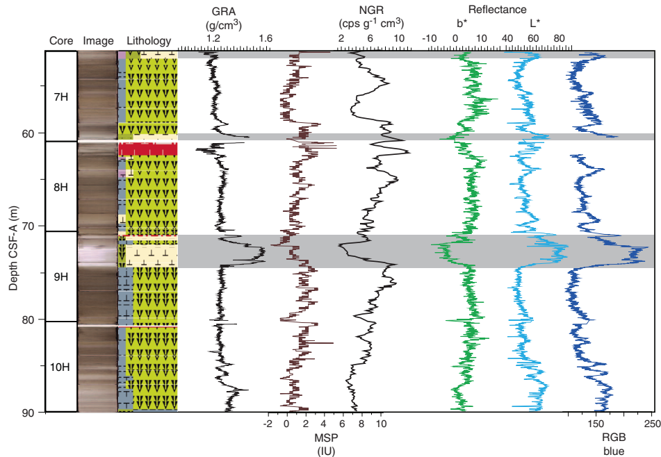
Figure F14. Characteristic variations in major lithologies and physical properties, Hole U1539A. Lithologies are determined by visual core description, smear slide analyses, and X-ray imaging. Shaded bars show intervals of light-colored nannofossil ooze. GRA = gamma ray attenuation, NGR = natural gamma radiation, MSP = point magnetic susceptibility, RGB = red-blue-green.
