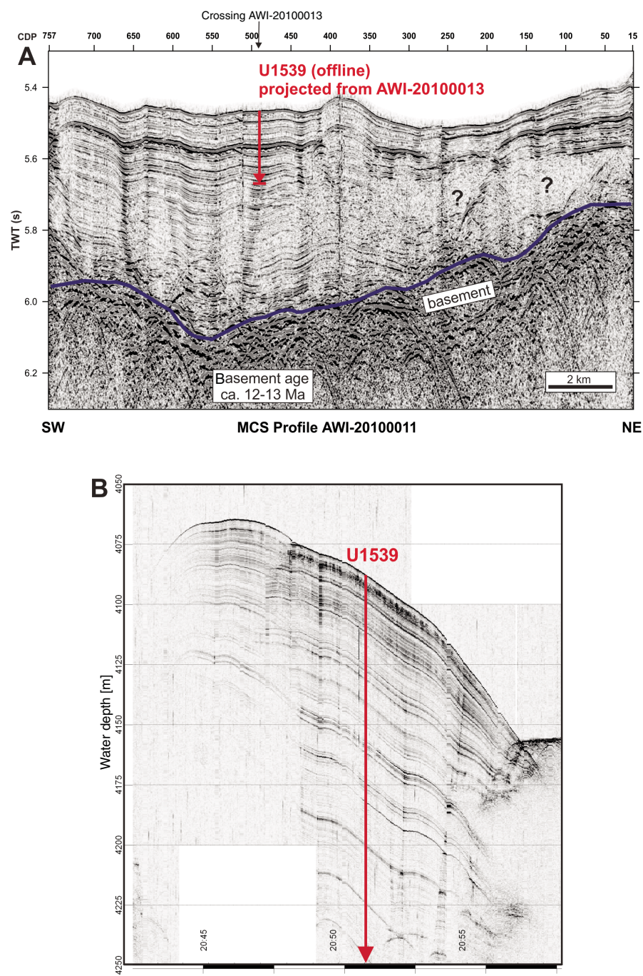
Figure F2. (A) Multichannel seismic (MCS) and (B) Parasound profiles across Site U1539.
