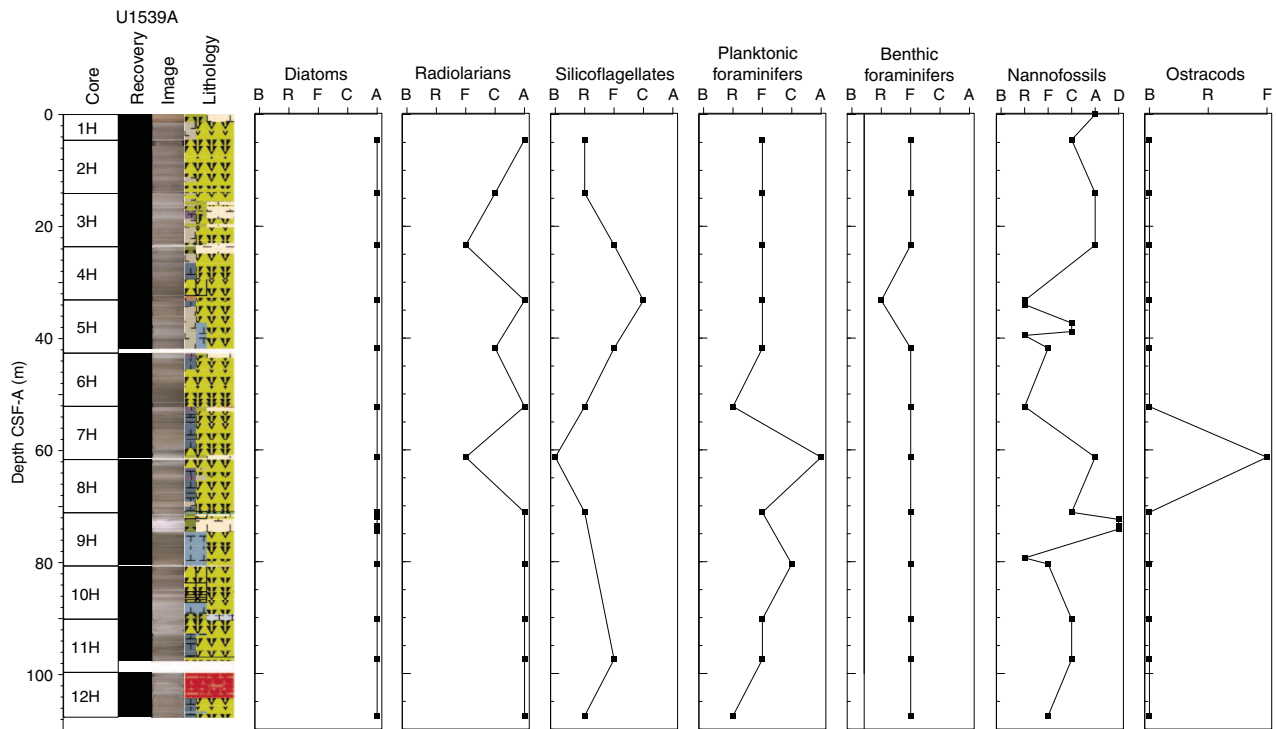
Figure F18. Distribution of siliceous and calcareous microfossils, Hole U1539A. B = barren, R = rare, F = few, C = common, A = abundant, D = dominant.
