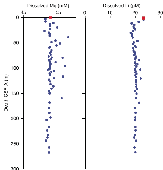
Figure F34. Interstitial water magnesium and lithium, Site U1539. Red square = overlying seawater sample.
