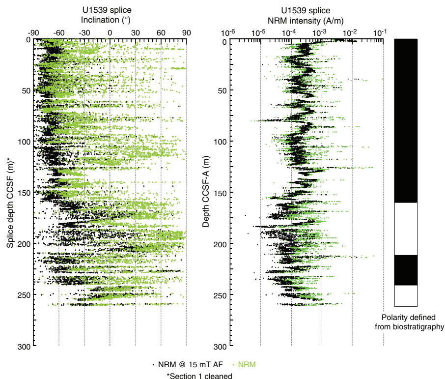
Figure F30. Inclination and natural remanent magnetization (NRM) intensity before and after 15 mT peak alternating field (AF) demagnetization, Site U1539.
