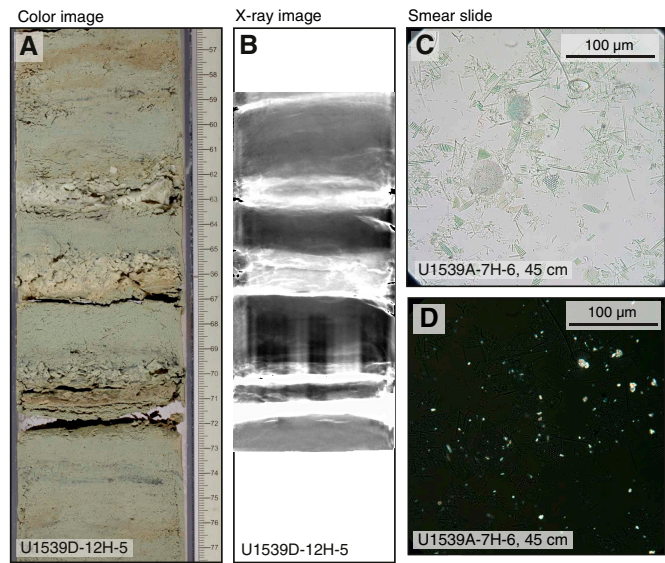
Figure F5. Representative (A) core and (B) X-ray and photomicrograph images in (C) plane-polarized light (PPL) and (D) cross-polarized light (XPL), Holes U1539A and U1539D.
