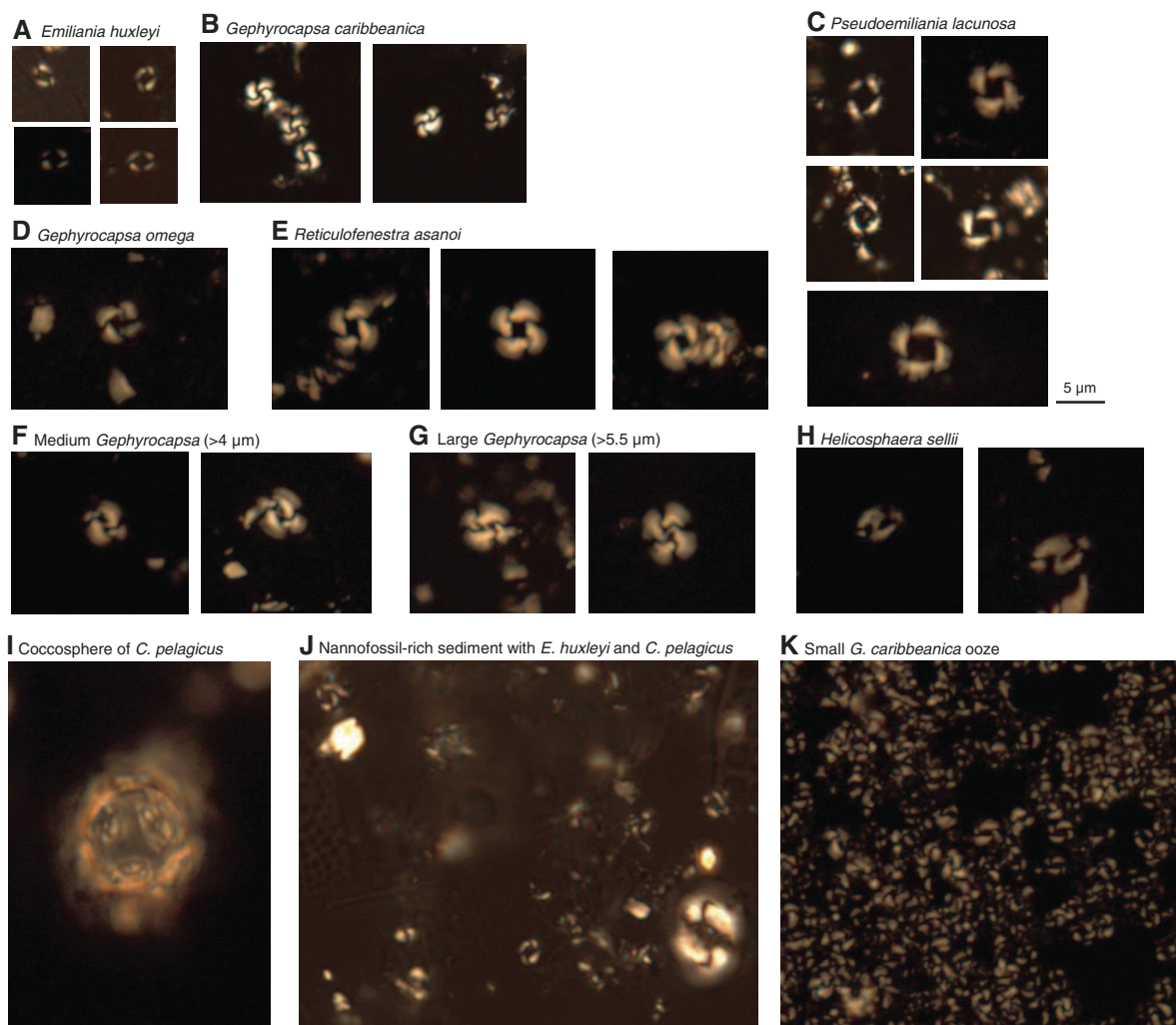
Figure F23. Calcareous nannofossils, Holes U1539A and U1539C. A. Emiliania huxleyi (383-U1539A-2H-CC). B. Gephyrocapsa caribbeanica . C. Pseudoemiliania lacunosa . D. Gephyrocapsa omega . E. Reticulofenestra asanoi . F, G. Gephyrocapsa , (F) medium (4–5.5 µm), (G) large (>5.5 µm). H. Helicosphaera sellii . I. Coccosphere of Coccolithus pelagicus (383-U1539C-22H-6). J. Nannofossil-rich sediment with E. huxleyi and C. pelagicus (383-U1539A-3H-CC). K. Ooze of small (<4 µm) G. caribbeanica (383-U1539A-9H-CC).
