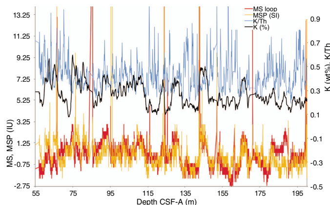
Figure F42. Natural gamma radiation–derived K% (black), K/Th 7-point smoothed (blue), Whole-Round Multisensor Logger magnetic susceptibility (MS; red), and Section Half Multisensor Logger point magnetic susceptibility (MSP; orange), Hole U1539C.
