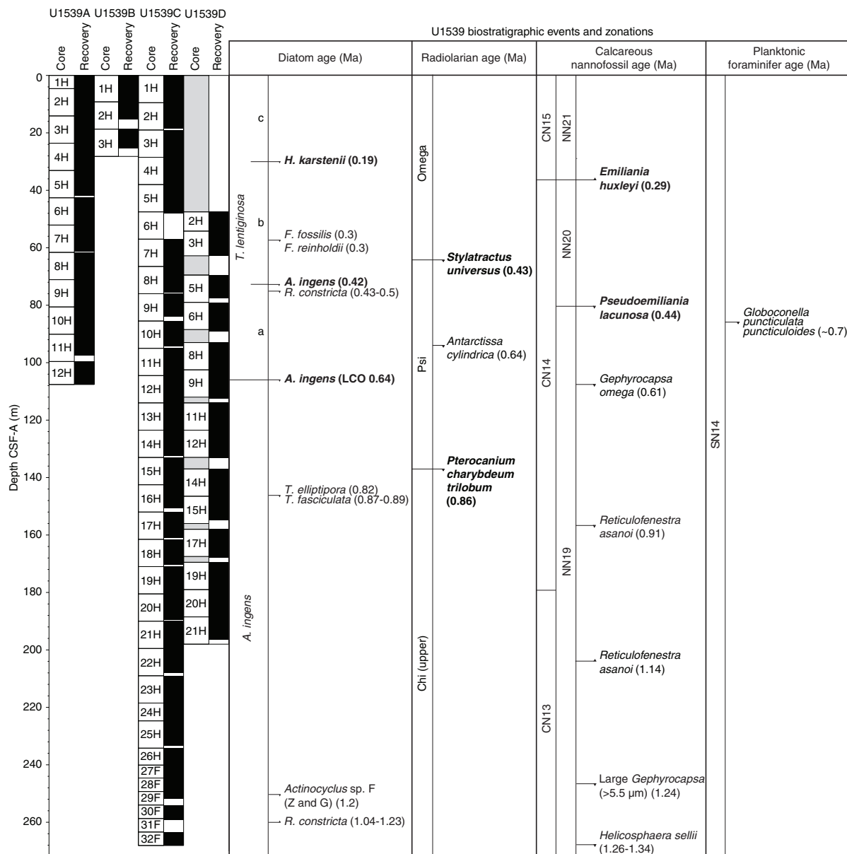
Figure F16. Diatom, radiolarian, calcareous nannofossil, and planktonic foraminifer zonations and biostratigraphic events, Site U1539.
