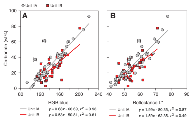
Figure F15. Relationships between bulk sedimentary carbonate content and (A) red-green-blue (RGB) blue and (B) color reflectance L^* for samples from Subunit IA (gray circles) and Subunit IB (red squares). Symbols in parentheses are data points from the Holocene that were excluded from the regression analysis.
