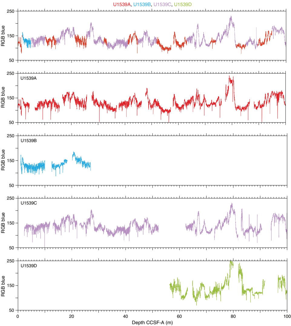
Figure F49. Red-green-blue (RGB) blue data vs. composite depth, Holes U1539A–U1539D. Data are divided into 100 m intervals. Top: cleaned RGB blue splice constructed by combining data from all holes. (Continued on next page.)
