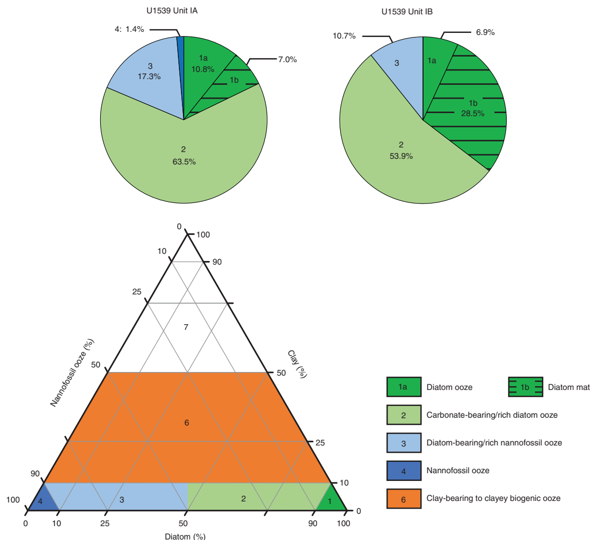
Figure F10. Primary lithologies used to define sedimentary lithofacies, Site U1539. Pie charts show the lithofacies' relative contributions to Lithostratigraphic Subunits IA and IB. Lithofacies 5 (turbiditic lithofacies) is excluded from this comparison.
