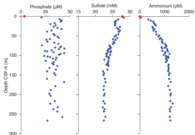
Figure F36. Interstitial water phosphate, sulfate, and ammonium, Site U1539. Red square = overlying seawater sample.
