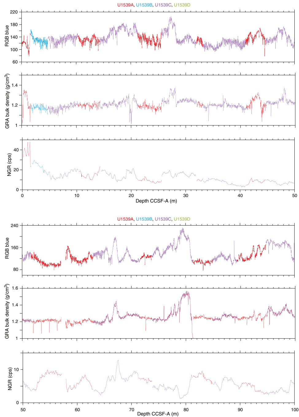
Figure F50. Spliced composite records of red-green-blue (RGB) blue, Whole-Round Multisensor Logger gamma ray attenuation (GRA) bulk density, and natural gamma radiation (NGR) vs. composite depth, Site U1539. Data are divided into 50 m intervals. cps = counts per second. (Continued on next two pages.)
