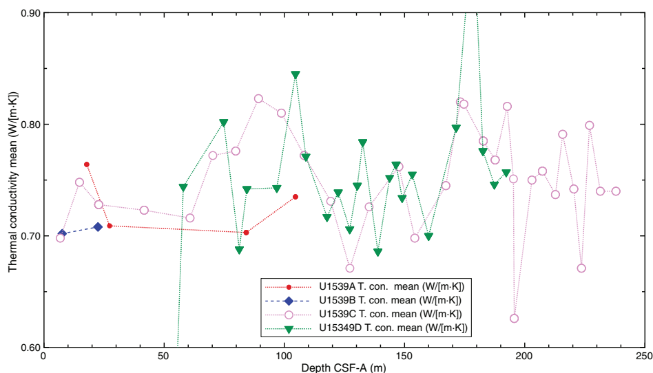
Figure F47. Thermal conductivity data from needle probe measurements, Holes U1539A–U1539D. 0.5 W heating power over 80 s interval. Mean values are taken from three measurements or less in cases with insufficient solution to calculate temperature conductivity.
