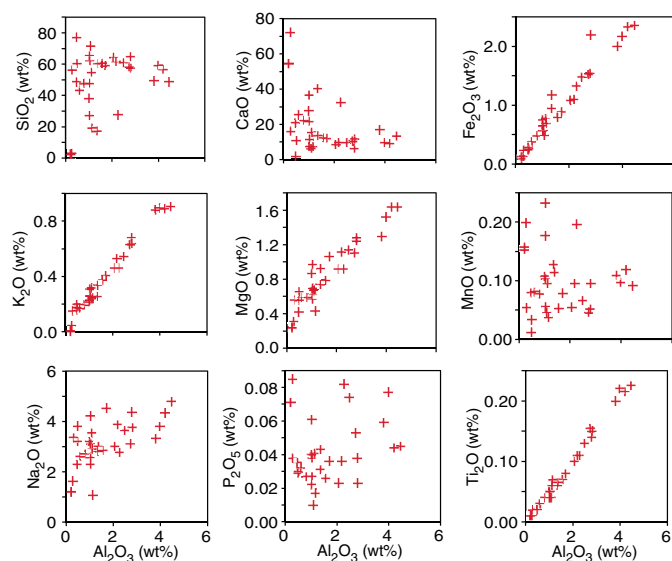
Figure F39. Bulk sediment elemental (Na, K, Si, P, Mg, Ca, Ti, Mn, and Fe) oxides vs. aluminum oxide, Site U1539.
