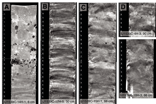
Figure F12. A–D. Examples of dropstone occurrence, Hole U1539C.
