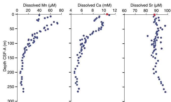
Figure F35. Interstitial water manganese, calcium, and strontium, Site U1539. Manganese was below detection limit in the overlying water. Red square = overlying seawater sample.
