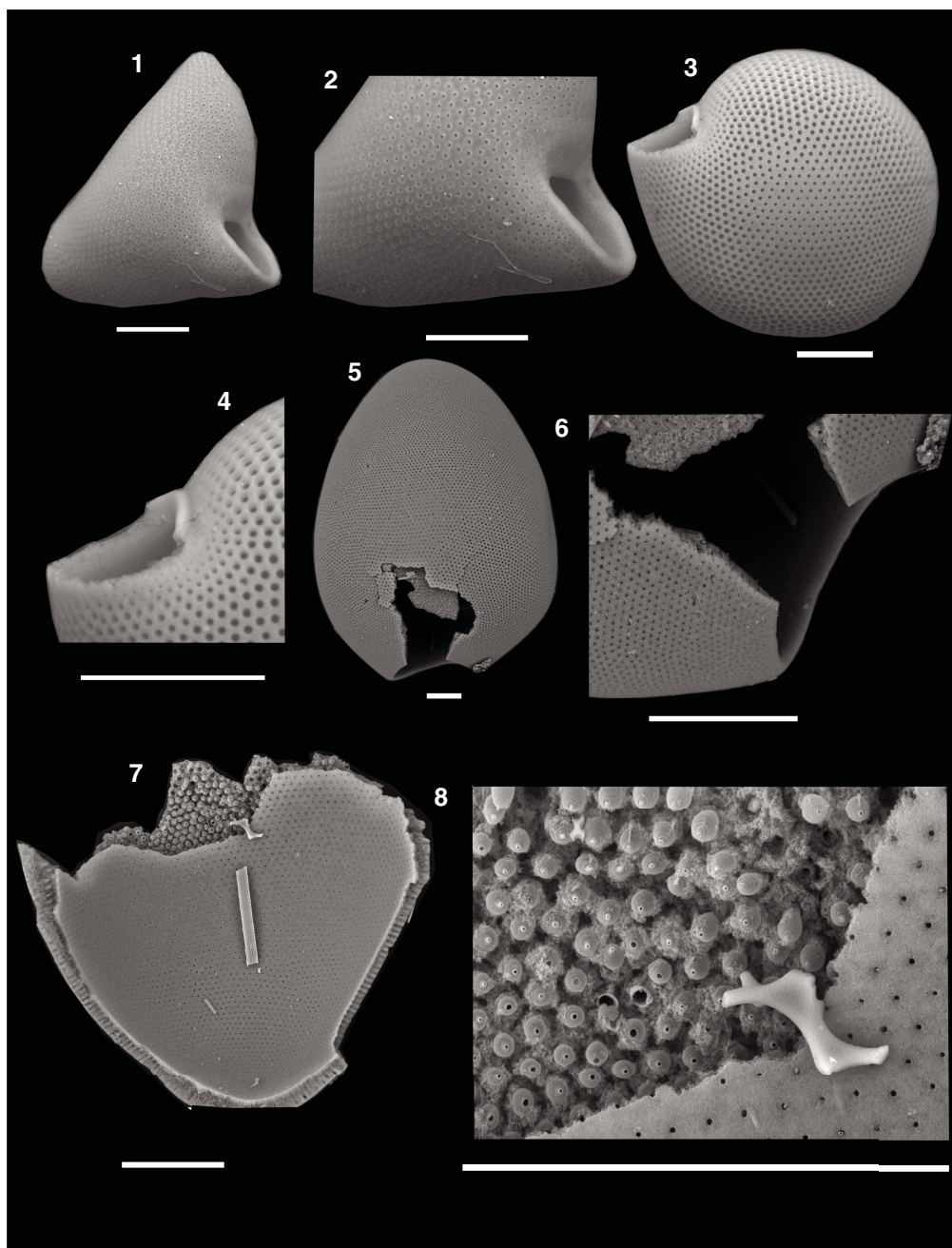
Figure F21. Phaeodarian radiolarians, Holes U1539A and U1539C. Scale bars = 50 \mu\text{m} . 1, 2. Triangular shape (383-U1539A-5H-CC), (2) aperture. 3, 4. Kettle shape (383-U1539A-12H-CC), (4) aperture. 5-8. Oval shape (383-U1539C-14H-CC), (6) aperture, (7) internal shell view, (8) close-up of internal shell.
