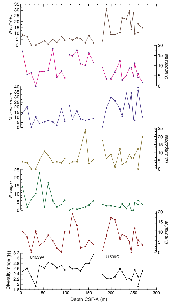
Figure F27. Species diversity index (H) and abundance of dominant benthic foraminifer species Cibicidoides mundulus , Epistominella exigua , Globocassidulina subglobosa , Melonis barleeanum , Oridorsalis umbonatus , and Pullenia bulloides , Holes U1539A and U1539C.
