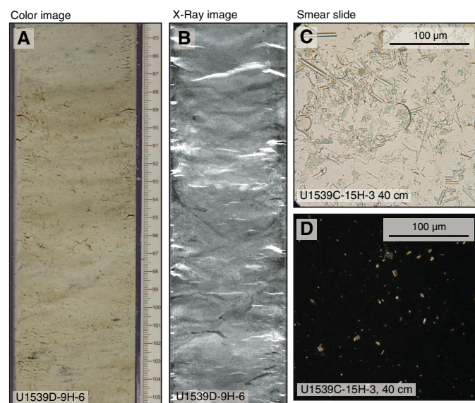
Figure F7. Representative (A) core and (B) X-ray and photomicrograph images of mineral properties of Lithofacies 2 (carbonate-bearing to carbonate-rich diatom ooze) in (C) PPL and (D) XPL, Holes U1539C and U1539D.
