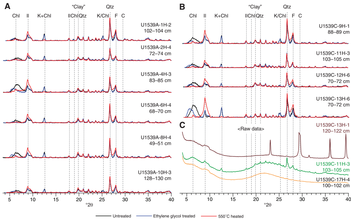
Figure F13. X-ray diffractograms of discrete samples from Holes (A) U1539A and (B) U1539C corrected for baseline variations resulting from significant proportions of amorphous biogenic silica in the samples (cf. black line in C). Minerals occurring in the samples include quartz (Qtz), feldspar (F; i.e., plagioclase), and calcite (C) and phyllosilicates including illite (Il), chlorite (Chl), kaolinite (K), and their composite ("Clay"). C. Data show characteristic baseline-uncorrected diffractograms of foraminifer-bearing, diatom-rich nannofossil ooze (brown line; Lithofacies 3), diatom-bearing calcareous ooze (green line; Lithofacies 3), and carbonate-rich diatom ooze (orange line; Lithofacies 2).
