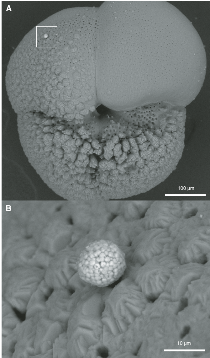
Figure F26. A. Pyrite framboid (upper left) on planktonic foraminifer Truncorotalia crassaformis . B. Close-up of pyrite framboid in A.
