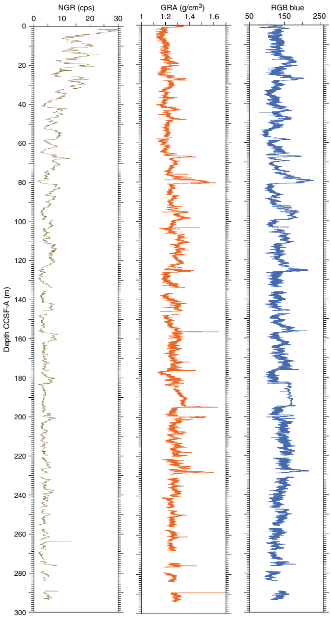
Figure F51. Complete spliced composite records of cleaned red-green-blue (RGB) blue, Whole-Round Multisensor Logger gamma ray attenuation (GRA) bulk density, and natural gamma radiation (NGR), Site U1539. cps = counts per second.
