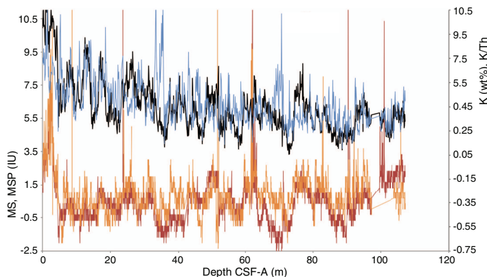
Figure F41. Natural gamma radiation–derived K% (black), K/Th 7-point smoothed (blue), Whole-Round Multisensor Logger magnetic susceptibility (MS; red), and Section Half Multisensor Logger point magnetic susceptibility (MSP; orange), Hole U1539A.
