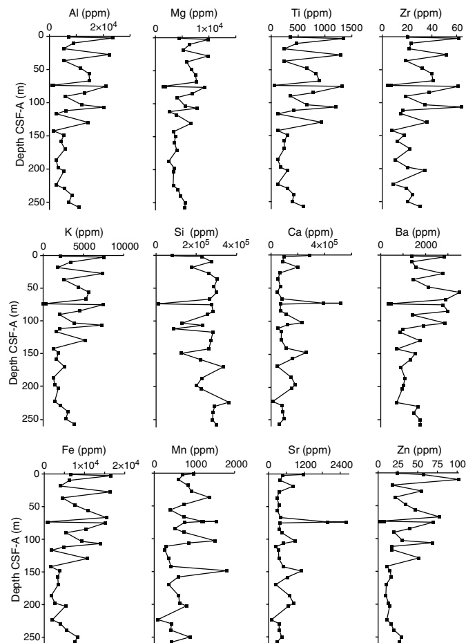
Figure F40. Bulk sediment major and minor element concentrations, Site U1539.
