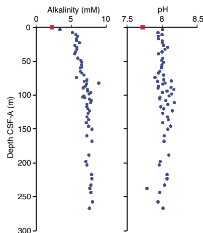
Figure F32. Interstitial water alkalinity and pH, Site U1539.
