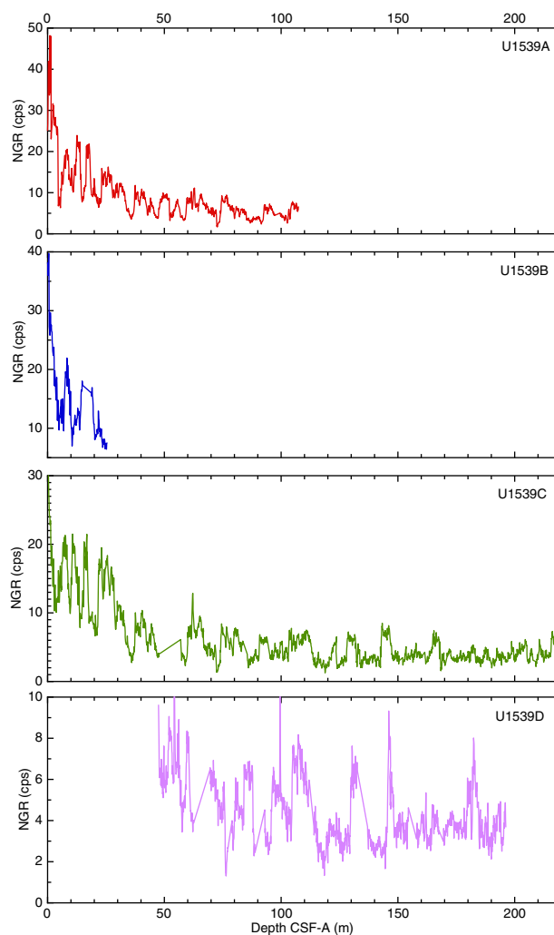
Figure F43. Natural gamma radiation (NGR) total counts, Holes U1539A–U1539D. Scales on NGR counts (y-axis) decrease from 50 to 10 from upper to lower panels.
