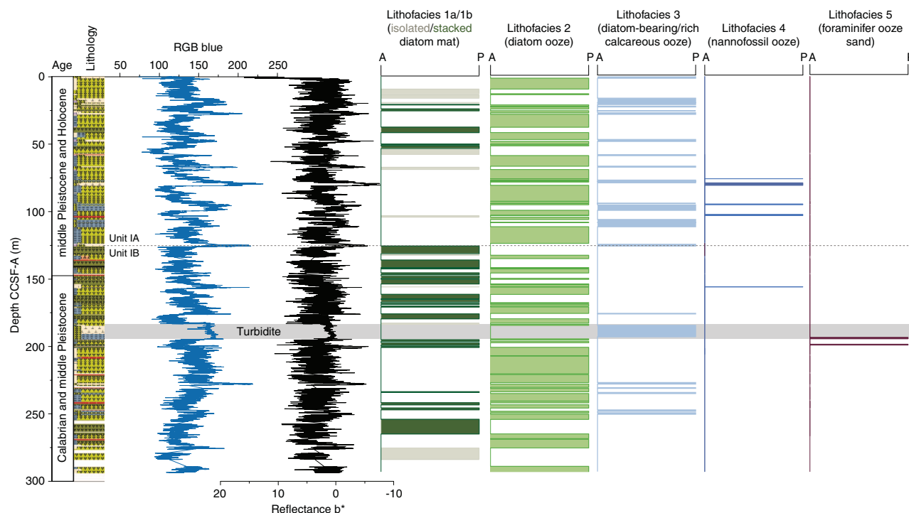
Figure F11. Primary lithostratigraphic variations, Site U1539. The unit boundary at ~125 m CCSF-A separates high diatom mat (Lithofacies 1b) abundance in the early part of the record from more frequent and thicker nanofossil ooze facies (Lithofacies 3 and 4) in the latter part of the record. Relative ages of units are based on the preliminary Site U1539 shipboard age model (see Stratigraphic correlation).
