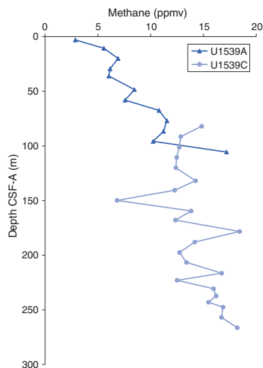
Figure F31. Headspace methane concentrations, Holes U1539A and U1539C.
