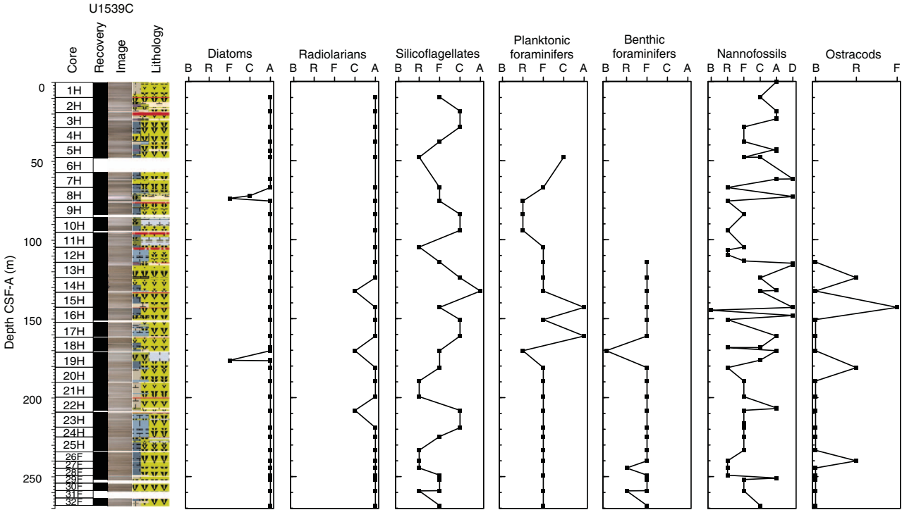
Figure F19. Distribution of siliceous and calcareous microfossils, Hole U1539C. B = barren, R = rare, F = few, C = common, A = abundant, D = dominant.
