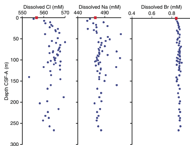
Figure F33. Interstitial water chloride, sodium, and bromide, Site U1539. Chloride: data points represent the mean of triplicate measurements. Red square = overlying seawater sample.
