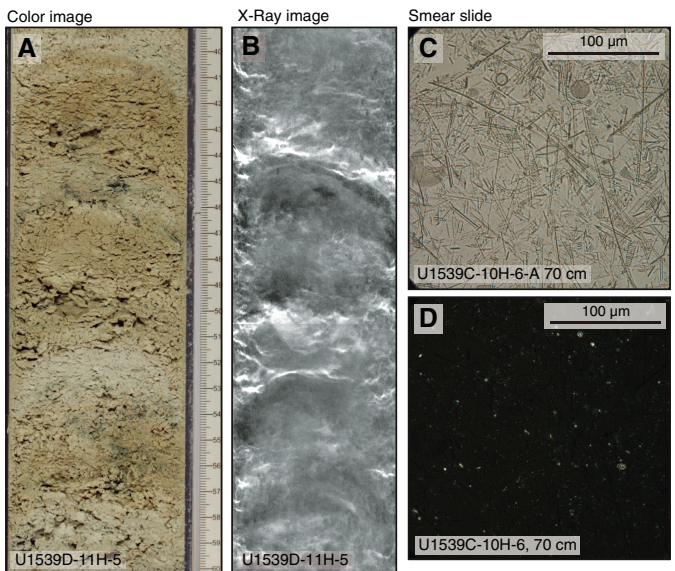
Figure F6. Representative (A) core and (B) X-ray and photomicrograph images of mineral properties of Lithofacies 1b (densely stacked diatom mats) in (C) PPL and (D) XPL, Holes U1539C and U1539D.
