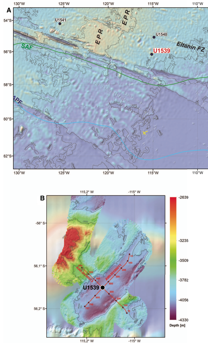
Figure F1. Oceanographic and bathymetric setting, Site U1539. A. Marine geological features and oceanic fronts. FZ = fracture zone, SAF = Subantarctic Front, APF = Antarctic Polar Front (after Orsi et al., 1995). B. Detailed bathymetry with seismic lines and shotpoints.
