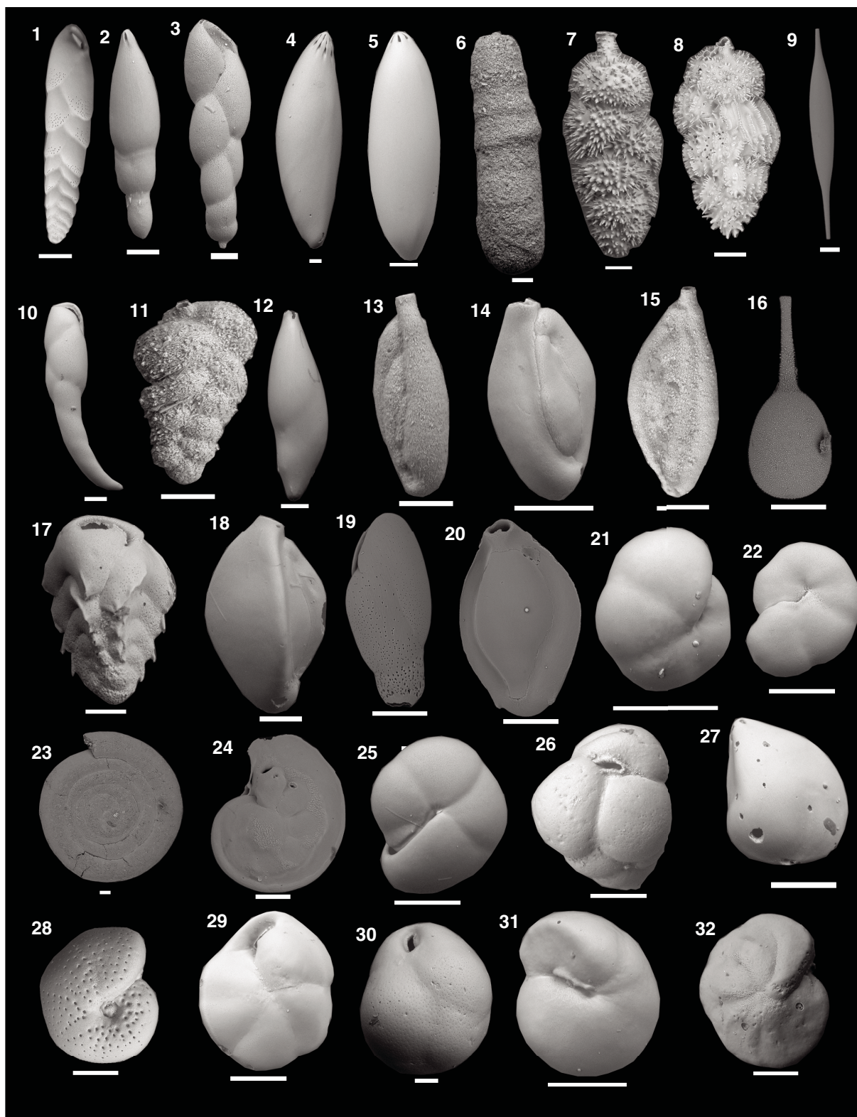
Figure F28. Benthic foraminifers, Holes U1539A and U1539C. Scale bars = 100 \mu m. 1–3, 13–15, 21. 383-U1539A-3H-CC. (1) Bolivina pacifica . (2) Nodosaria sp. (3) Fursenkoina complanata . 4–8, 12, 26, 27, 29–32. 383-U1539A-7H-CC. (4) Dentalina ariena . 5. Dentalina sp. (6) Martinottiella communis . (7) Uvigerina hispida . (8) Uvigerina peregrina . 9, 23. 383-U1539C-32F-CC. (9) Procerolagena sp. 10, 11. 383-U1539A-12H-CC. (10) Cassidulinoides sp. (11) Siphotextularia rolshauseni . (12) Pyrulina sp. (13) Schlumbergerina sp. (14) Quinqueloculina sp. (15) Spirosigmoilina sp. 16. Lagena hispidula (383-U1539C-24H-CC). 17, 18. 383-U1539A-1H-CC. (17) Ehrenbergina carinata , (18) Triculina tricarinata . 19, 20. 383-U1539C-19H-CC. (19) Fursenkoina bradyi , (20) Pyrgo sp. (21) Pullenia quinqueloba . 22, 28. 383-U1539A-5H-CC. (22) Astrononion sp. (23) Ammodiscus tenuis . 24. Laticarina pauperata (383-U1539C-28F-CC). (25) Pullenia quadriloba . (26) Eggerella bradyi . (27) Lenticulina convergens . (28) Melonis barleeianum . (29) Epistominella exigua . (30) Globocassidulina subglobosa . (31) Gyroidina nitida . (32) Cibicidoides mundulus .
