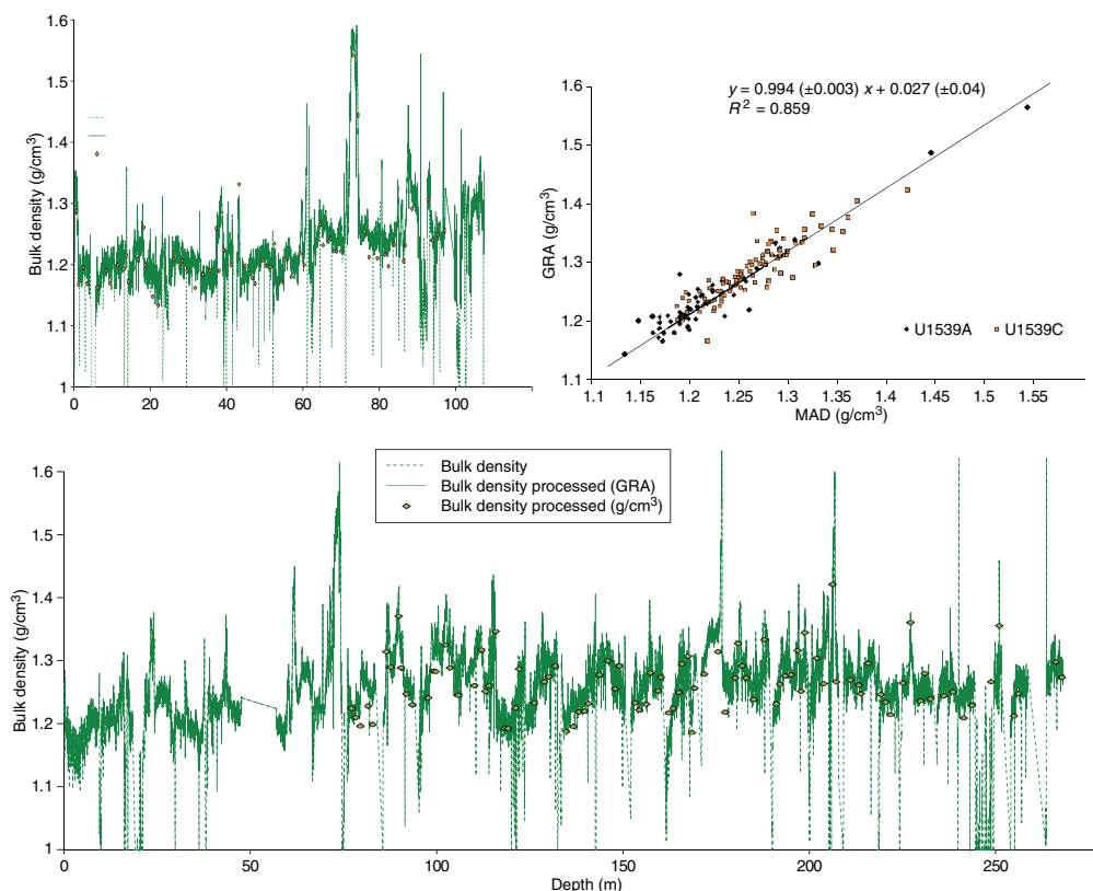
Figure F45. Bulk density data from WRMSL (green lines) and discrete moisture and density (MAD; dots), Holes U1539A (top) and U1539C (bottom). Top right: correlation between MAD- and gamma ray attenuation (GRA)-derived bulk density data from Holes U1539A (black diamonds) and U1539C (yellow squares). Linear best fit equation and correlation coefficient are shown.
