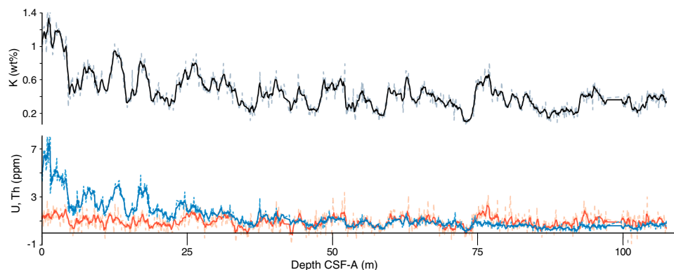
Figure F44. Calculation of K (black), U (blue), and Th (red) semiquantitatively derived from natural gamma radiation, Hole U1539A. Dashed lines = raw data, solid lines = smoothed data.
