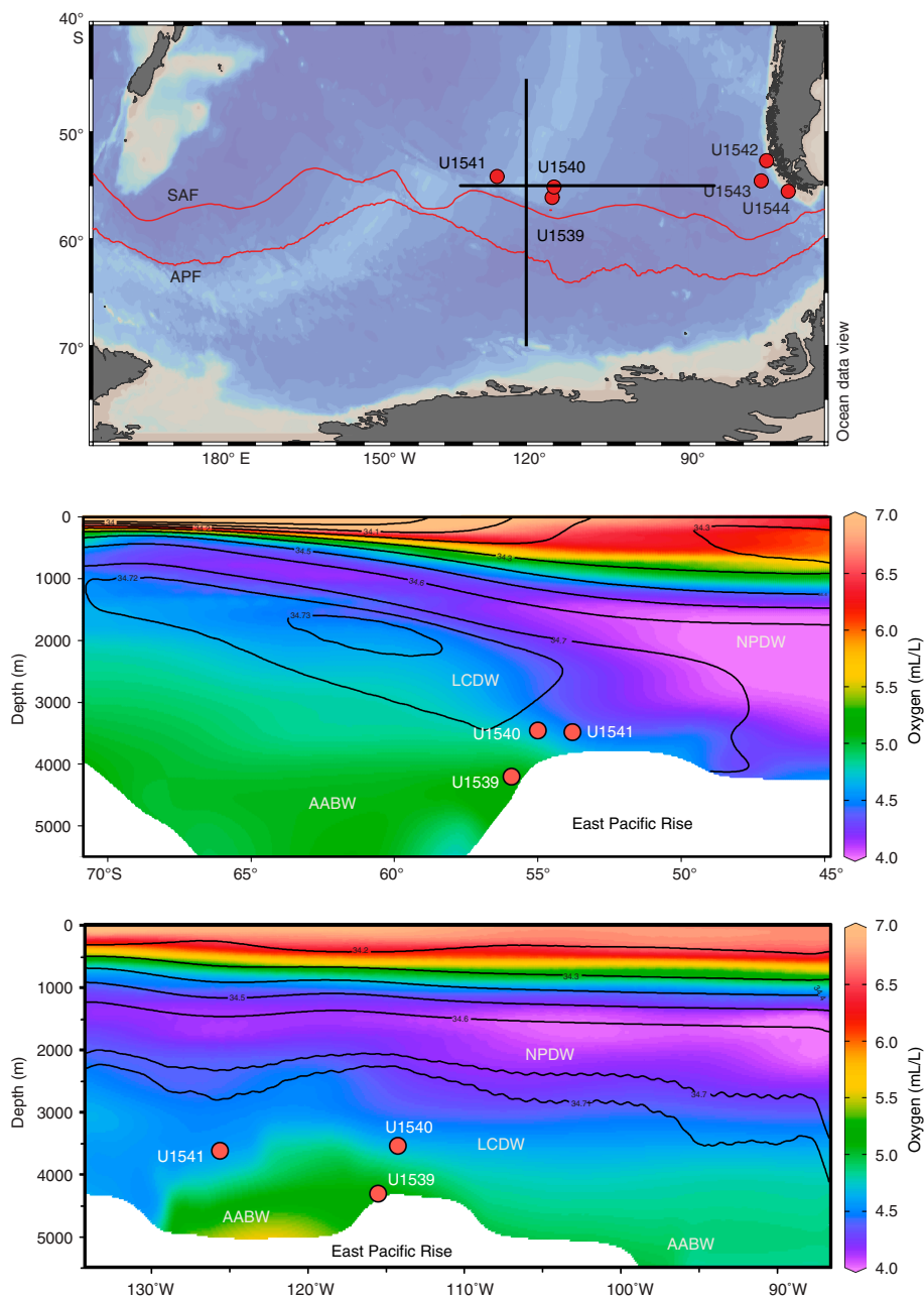
Figure F3. Modern salinity and oxygen distribution in the central South Pacific used to visualize major water masses. SAF = Subantarctic Front, APF = Antarctic Polar Front, NPDW = North Pacific Deep Water, LCDW = Lower Circumpolar Deep Water, AABW = Antarctic Bottom Water.
