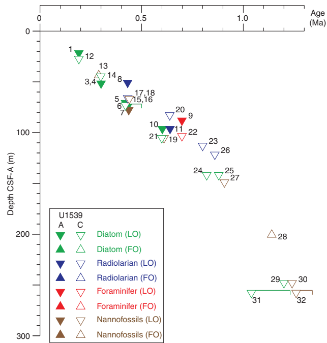
Figure F17. Age-depth plot, Holes U1539A and U1539C. FO = first occurrence, LO = last occurrence.
