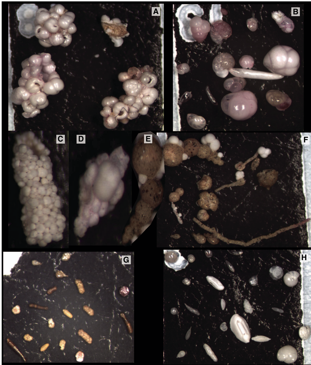
Figure F29. Benthic foraminifers in the mudline sample from Hole U1540B. A. Rhabdammina sp. that uses planktonic foraminifers of a single species ( Globocoinella inflata ) in its construction. B. Stained calcareous benthic foraminifers. C. Rhabdammina sp. that uses planktonic small benthic and planktonic foraminifers species in its construction. D. Rhabdammina sp. that uses multiple planktonic foraminifers species in its construction. E. Reophax sp. F, G. Stained and unstained agglutinated benthic foraminifers. H. Unstained calcareous benthic foraminifers.
