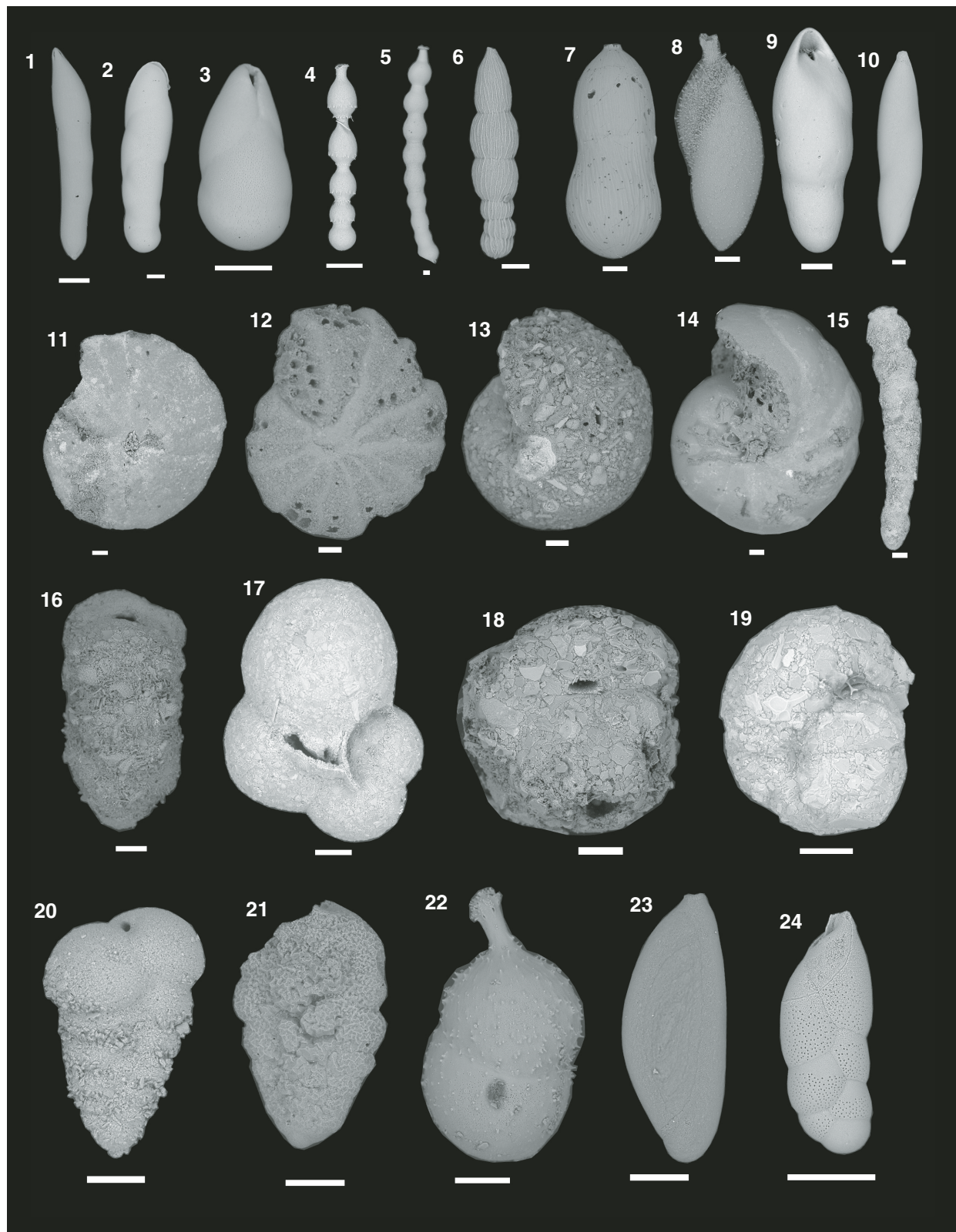
Figure F28. Benthic foraminifers, Holes U1540A, U1540B, and U1540D. Scale bars = 100 \mu m. (1) Dentalina sp. (383-U1540B-1H-CC). 2, 3. Fursenkoina texturata (383-U1540B-1H-CC). (4) Stilostomella lepidula (383-U1540B-1H-CC). 5. Stilostomella abyssorum (383-U1540D-17H-CC). 6, 7. Orthomorphina sp., (6) 383-U1540D-19H-CC, (7) 383-U1540D-16H-CC. 8. Francuscia extensa (383-U1540D-16H-CC). 9. Pleurostomella sp. (383-U1540D-17H-CC). 10. Pyrulina angusta (383-U1540B-1H-CC). 11–13. Cyclammina sp., (11) 383-U1540D-22H-CC, (12) 383-U1540D-19H-CC, (13) 383-U1540D-20H-CC. 14. Haplophragmium sp. (383-U1540D-22H-CC). 15. Reophax sp. (383-U1540D-22H-CC). 16. Karrerella sp. (383-U1540A-4H-CC). 17. Haplophragmoides sp. (383-U1540B-1H-CC). 18. Discammina sp. (383-U1540B-1H-CC). 19. Discammina compressa (383-U1540B-1H-CC). 20. Siphotextularia sp. (383-U1540A-15H-CC). 21. Bolivina decussata (383-U1540D-15H-CC). 22. Amphicoryna hirsuta (383-U1540B-1H-CC). 23. Spirosigmolite tenuis (383-U1540D-19H-CC). 24. Bolivina sp. (383-U1540A-4H-CC).
