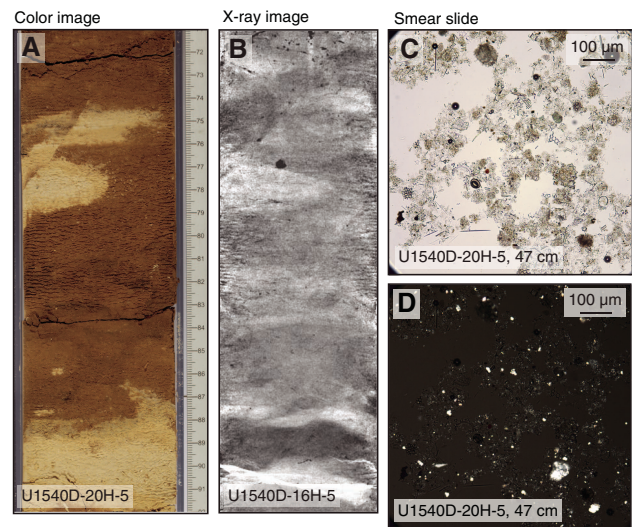
Figure F7. Representative (A) core and (B) X-ray and photomicrograph images of mineral properties of Lithofacies 7 (carbonate- and biosilica-bearing clay) in (C) PPL and (D) XPL, Hole U1540D.
