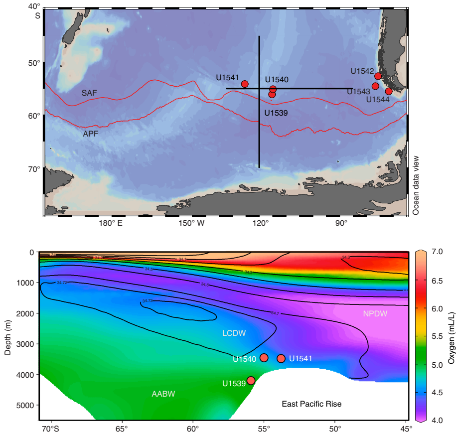
Figure F3. Modern salinity (contour lines) and oxygen distribution (colors) in the central South Pacific used to visualize major water masses. NPDW = North Pacific Deep Water, LCDW = Lower Circumpolar Deep Water, AABW = Antarctic Bottom Water. (Continued on next page.)
