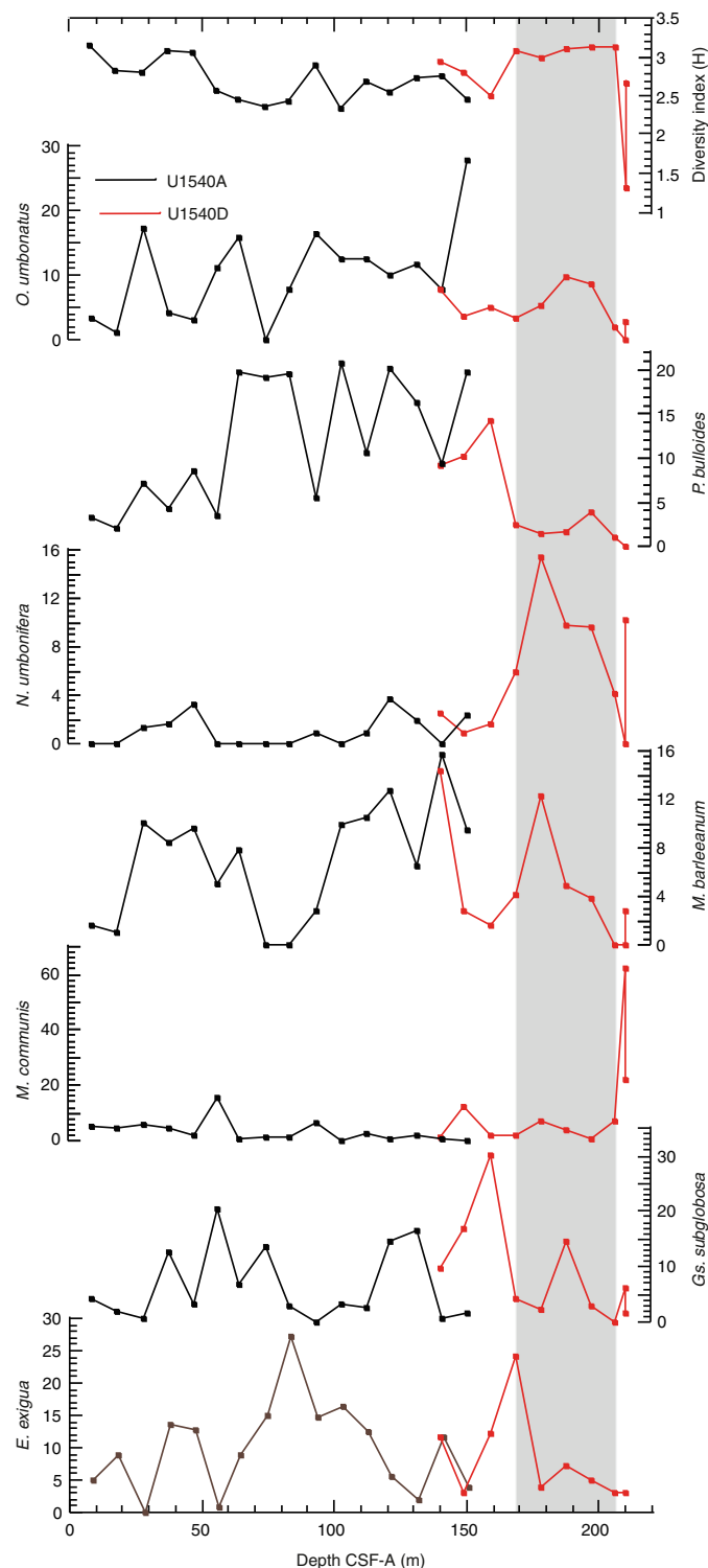
Figure F26. Species diversity index (H) and abundance of dominant species Epistominella exigua , Globocassidulina subglobosa , Martinotiella communis , Melonis barleeianum , Pullenia bulloides , and Oridorsalis umbonatus , Holes U1540A and U1540D. Gray field denotes an interval potentially influenced by warm corrosive bottom water.
