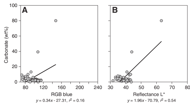
Figure F19. Relationships between bulk sedimentary carbonate content and (A) red-green-blue (RGB) blue and (B) color reflectance L^* , Unit I, Site U1542. Black solid line = linear regression of data.
