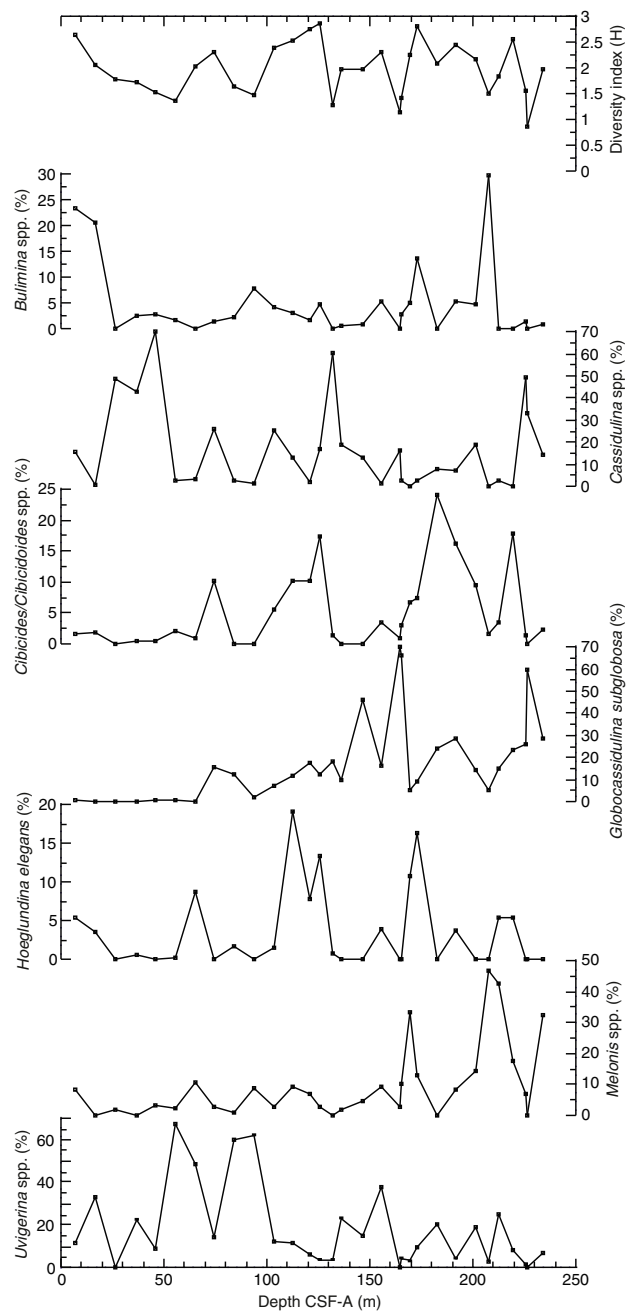
Figure F27. Species diversity index and abundance of dominant benthic foraminifer genus/species Uvigerina spp., Melonis spp., Hoeglundina elegans , Globocassidulina subglobosa , Cibicides/Cibicidoides spp., Cassidulina spp., and Bulimina spp., Site U1542.
