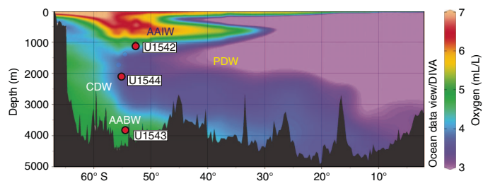
Figure F5. Modern oxygen distribution in the eastern South Pacific used to visualize major water masses. AAIW = Antarctic Intermediate Water, PDW = Pacific Deep Water, CDW = Circumpolar Deep Water, AABW = Antarctic Bottom Water. Red circles mark the eastern South Pacific and Chilean margin Sites U1542–U1544.
