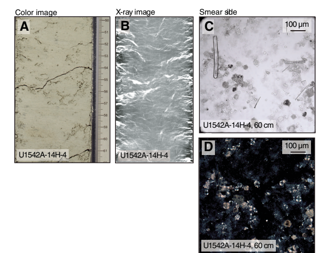
Figure F8. Representative (A) core and (B) X-ray images of Lithofacies 4 (nannofossil ooze). Smear slide photomicrographs of Lithofacies 4 mineral properties in (C) plane-polarized light (PPL) and (D) cross-polarized light (XPL), Hole U1542A. This is a foraminifer-rich variety of the nannofossil oozes described at previous Expedition 383 sites.
