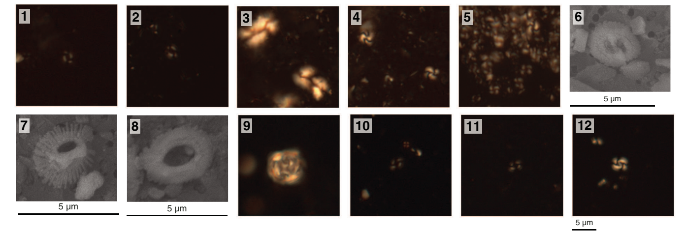
Figure F25. Calcareous nannofossils, Holes U1542A and U1542C. Light microscope and scanning electron microscope. 1, 2. Emiliania huxleyi (Hole U1542A mudline). 3, 4. 383-U1542A-11H-4, 75 cm. (3) Helicosphaera carteri . (4) Gephyrocapsa caribbeana . 5. G. caribbeana and small (<4 µm) Gephyrocapsa ooze (383-U1542A-14H-4, 40 cm). 6–8. 383-U1542A-13H-CC. (6) Small (<4 µm) Gephyrocapsa . (7) Gephyrocapsa protohuxleyi /dissolved small (<4 µm) Gephyrocapsa . (8) Small (<3 µm) Reticulofenestra . 9. Coccosphere of Gephyrocapsa (383-U1542A-14H-CC). 10, 11. Small (<3 µm) Reticulofenestra (383-U1542A-17H-CC). 12. Gephyrocapsa omega (383-U1542C-23H-CC).
