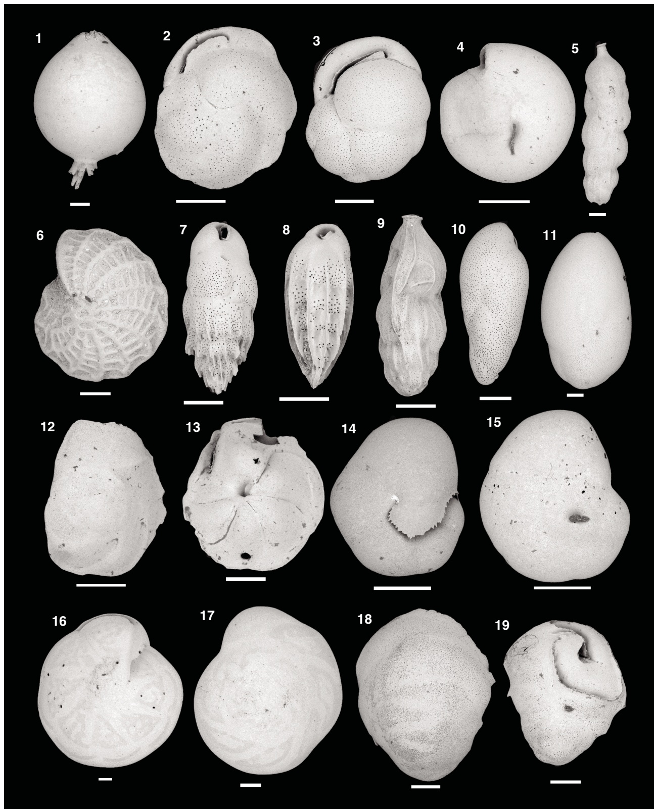
Figure F28. Benthic foraminifers, Holes U1542A–U1542C. Scale bars = 100 \mu\text{m} . 1, 5. 383-U1542A-2H-CC. (1) Oolina globulosa . 2. Cassidulina carinata (383-U1542A-1H-CC). 3, 7. 383-U1542A-4H-CC. (3) Cassidulina laevigata . 4. Biloculina sp. (383-U1542B-13H-CC). (5) Uvigerina peregrina . 6. Elphidium macellum (383-U1542C-22H-CC). (7) Bulimina mexicana . 8, 9, 16, 17. 383-U1542C-21H-CC. (8) Bulimina alazanensis . (9) Trifarina angulosa . 10, 12, 13. 383-U1542A-3H-CC. (10) Fursenkoina bradyi . 11, 14, 15, 18, 19. 383-U1542A-6H-CC. (11) Globobulimina pacifica . (12, 13) Osangularia culter . (14, 15) Rosalina sp. (16, 17) Hoeglundina elegans . (18, 19) Ehrenbergina sp.
