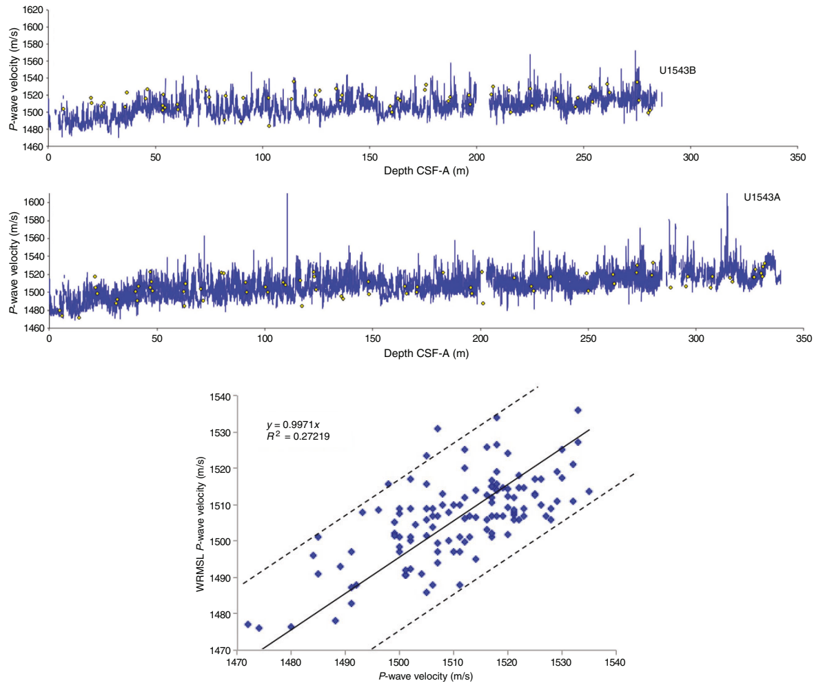
Figure F46. Top: P -wave data from Whole-Round Multisensor Logger (WRMSL; blue line) and discrete P -wave caliper (PWC) measurements (diamonds), Holes U1543A and U1543B. Bottom: correlation between PWC (x-axis) and WRMSL results for Holes U1543A and U1543B.
