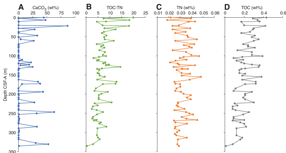
Figure F36. Solid phase geochemistry of (A) \text{CaCO}_3 , (B) total organic carbon:total nitrogen (TOC:TN), (C) TN, and (D) TOC, Site U1543.
