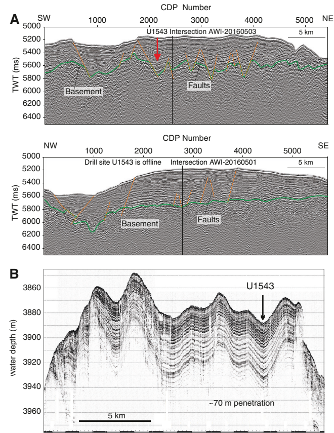
Figure F2. (A) Multichannel seismic (MCS) and (B) Parasound profiles across Site U1543. CDP = common depth point, TWT = two-way traveltime.
