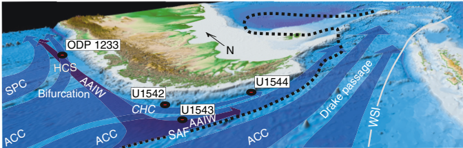
Figure F4. Schematic view of the southern Chilean margin and the Drake Passage region with major surface and intermediate water circulation and location of Expedition 383 sites and ODP Leg 202 Site 1233. HCS = Humboldt Current System, SPC = South Pacific Current, AAIW = Antarctic Intermediate Water, CHC = Cape Horn Current, ACC = Antarctic Circumpolar Current, SAF = Subantarctic Front, WSI = winter sea ice (approximate location).
