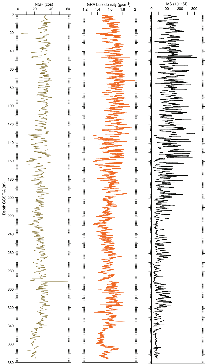
Figure F52. Complete spliced composite records of natural gamma radiation (NGR), cleaned gamma ray attenuation (GRA) bulk density, and Whole-Round Multisensor Logger magnetic susceptibility (MS), Site U1543.
