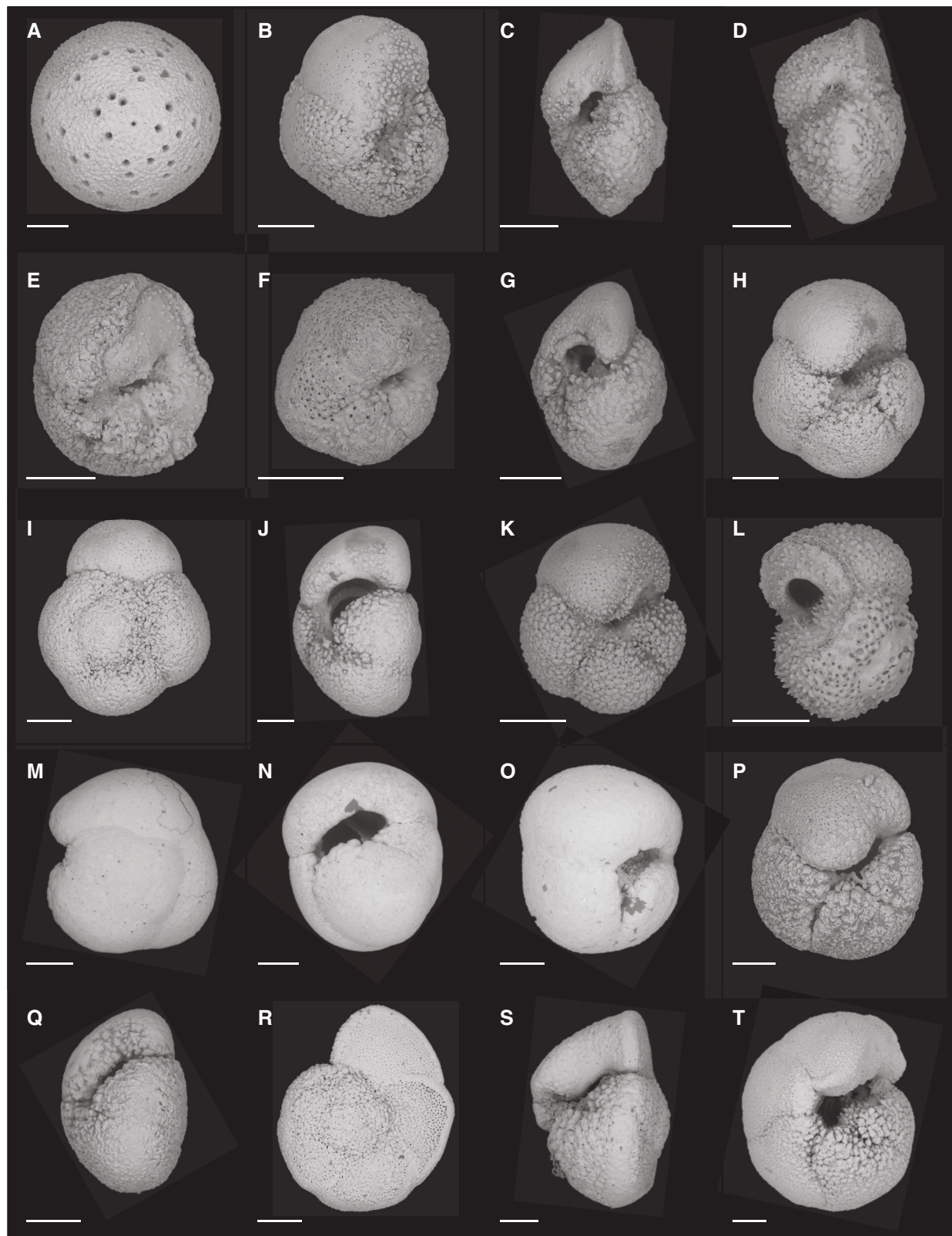
Figure F24. Planktonic foraminifers, Site U1543. Scale bars = 100 \mu\text{m} . A. Orbulina universa . B, C. Globoconella pliozea in (B) umbilical and (C) side view. D, E. Globoconella conomiozea in (D) side and (E) umbilical view. F, G. Globoconella sphericomiozea in (F) umbilical and (G) side view. H–J. Globoconella puncticulata puncticuloides in (H) umbilical, (I) spiral, and (J) side view. K, L. Globoconella puncticulata in (K) umbilical and (L) side view. M–O. Globoconella inflata in (M) spiral, (N) side, and (O) umbilical view. P, Q. Truncorotalia crassaformis in (P) umbilical and (Q) side view. R–T. Truncorotalia truncatulinoides in (R) spiral, (S) side, and (T) umbilical view.
