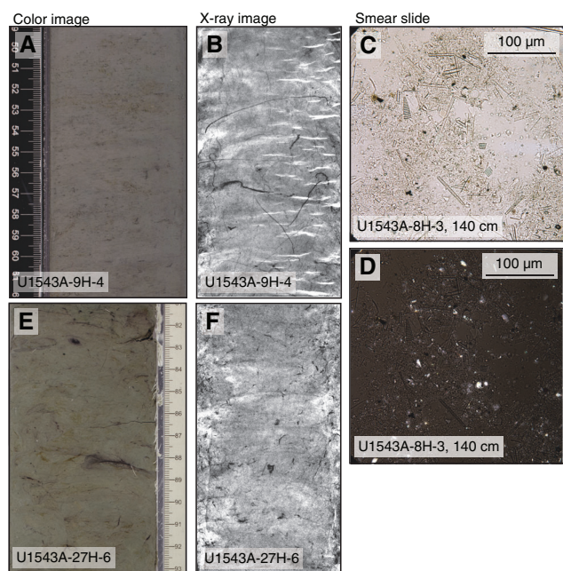
Figure F11. Representative (A) core and (B) X-ray and photomicrograph images of mineral properties of Lithofacies 7 (diatom-bearing to diatom-rich clay to silt) in (C) PPL and (D) XPL, Hole U1543A.
