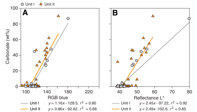
Figure F18. Relationships between bulk sedimentary carbonate content and (A) red-green-blue (RGB) blue and (B) color reflectance L*, Hole U1543A.
