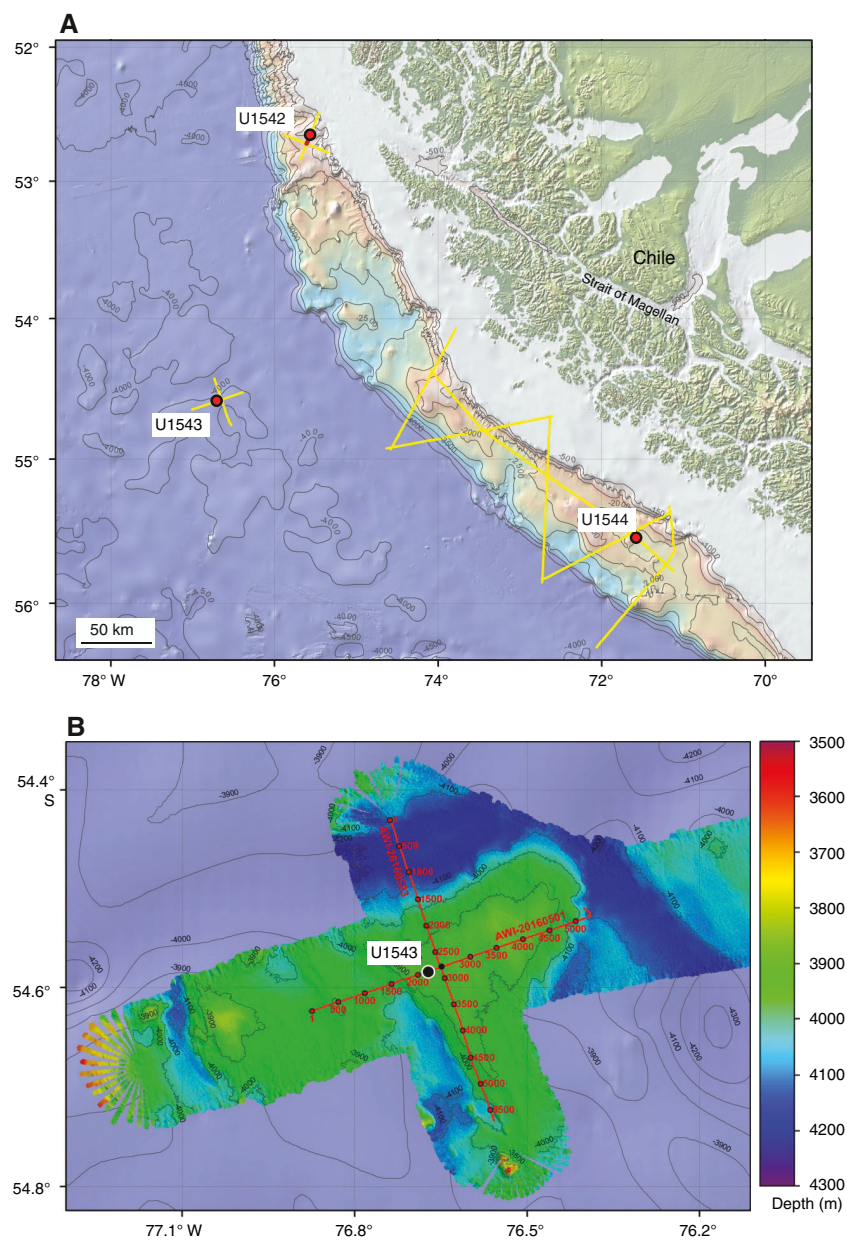
Figure F1. Oceanographic and bathymetric setting, Site U1543. A. Marine geological features. Yellow lines = seismic lines available in the region. B. Detailed bathymetry with seismic lines and shotpoints.
