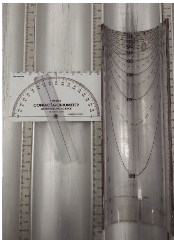
Figure F16. Goniometer and plastic protractor template used during Expedition 385 to measure dip and dip direction of structures.
