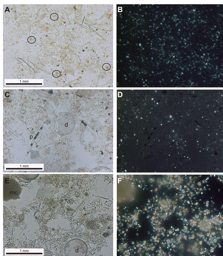
Figure F6. Subunit IA and IB characteristics, Hole U1547A. A, B. Higher organic matter and nannofossil content in a clay-rich diatom ooze from upper Subunit IA (2H-1, 109 cm). (A) Brown algal matter is circled (plane-polarized light [PPL]); (B) nannofossils are identified by their birefringence (brighter spots) under cross-polarized light (XPL). C, D. Decreasing organic matter, loss of nannofossils, and development of micrite in micrite-bearing diatom clay from Subunit IB (6H-5, 15 cm). (C) Diatoms (d) and black (opaque) pyrite framboids (p) (PPL); (D) sparse bright spots indicate presence of birefringent micrite (XPL). E, F. Micrite-rich diatom ooze that marks the Subunit IA/IB boundary (5H-5, 77 cm). (E) Diatom debris (d) and fine subhedral micrite (potentially dolomite) crystals are recognized by higher relief (PPL). Slightly large clump of material in the upper left corner may be a slightly more indurated microconcretion (mc). (F) Coarser micrite exhibits very high birefringence characteristic of carbonate (XPL).
