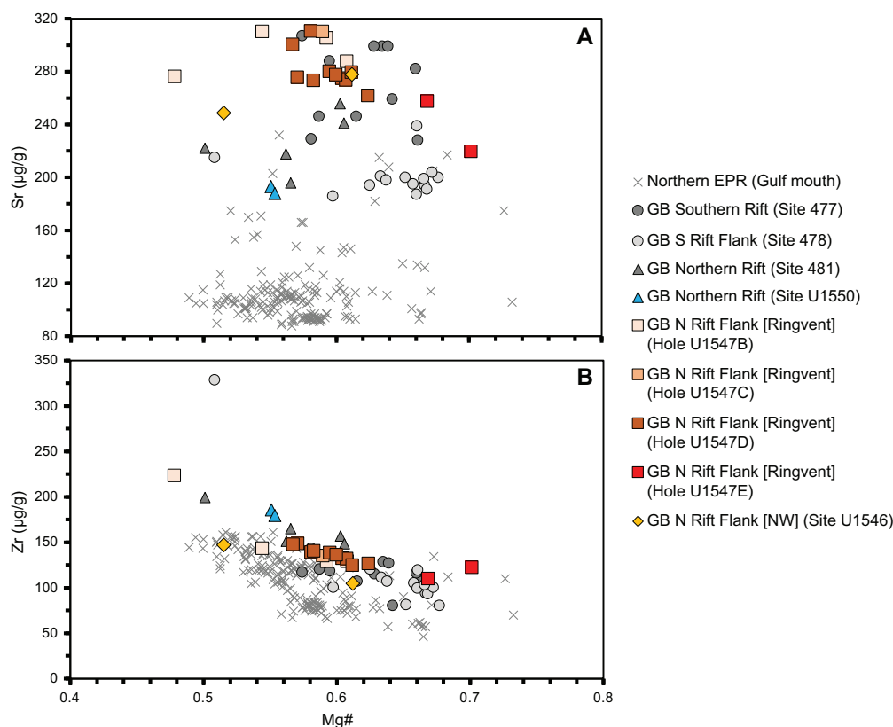
Figure F22. Mg\# versus (A) strontium (Sr) and (B) zirconium (Zr) content of mafic igneous rocks at drill sites from the Gulf of California. ppm = µg/g. Mg\# = 100 \times \text{molar } MgO / (MgO + FeO) , where all iron is treated as FeO. Guaymas Basin (GB) drill sites: DSDP Leg 64 (477, 478, 481) and Expedition 385 (U1546 [Hole C], U1547 [Holes B/C/D/E], and U1550 [Holes A/B]). On-axis: Sites 477 (southern rift) and 481/U1550 (northern rift). Off-axis: Sites 478 (southern rift flank), U1546 (northern rift flank in NW GB), and U1547 (northern rift flank at Ringvent). Gulf of California mouth drill sites lie at East Pacific Rise (EPR) off-axis locations on the Pacific plate (474, 483) and Rivera plate (482, 485). DSDP Leg 64 and 65 (Sites 482, 483, 485) data were compiled from the PetDB Database ( http://www.earthchem.org/petdb ) on 26 October 2020 using the following search criteria: longitude = -106 to -114, latitude = 20 to 28, and materials = igneous.
