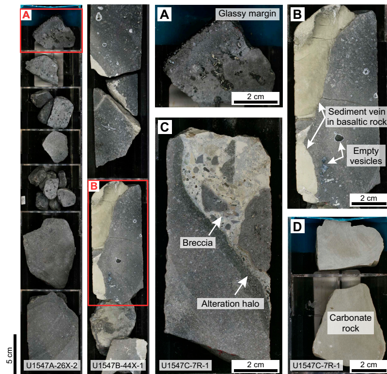
Figure F15. Igneous textures and sediment-magma interaction features, Site U1547. This phenomenon is abundant at Ringvent. A. Glassy margin and cryptocrystalline texture in basaltic rock. Elongate vesicles are seen just below the glassy margin. B. Injected sediment forming veins. C. Contact of basaltic breccia and coherent basaltic host rock. B and C are separated by an alteration halo. D. Pieces of carbonate forming the base of the sediment in Hole U1547C.
