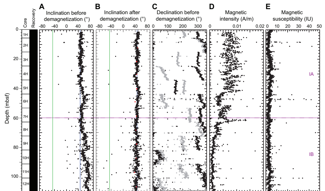
Figure F35. Inclination, declination, magnetic intensity, and magnetic susceptibility, Hole U1548E. Inclination data (A) before and (B) after AF demagnetization at 20 mT. Red squares = characteristic remanent magnetization inclination of discrete samples after principal component analysis. Expected geocentric axial dipole inclination ( \sim 46.2^\circ ) is indicated by green (reversed polarity) and blue (normal polarity) lines. C. Declination before demagnetization (in gray). Black = corrected using core orientation obtained from the Icefield MI-5 core orientation tool. D. Magnetic intensity (natural remanent magnetization). E. Section Half Multisensor Logger point magnetic susceptibility.
