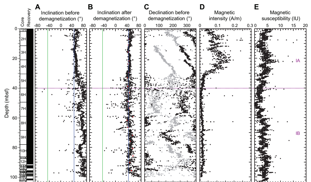
Figure F32. Inclination, declination, magnetic intensity, and magnetic susceptibility, Hole U1548A. Inclination data (A) before and (B) after AF demagnetization at 20 mT. Red squares = characteristic remanent magnetization inclination of discrete samples after principal component analysis. Expected geocentric axial dipole inclination (~46.2°) is indicated by green (reversed polarity) and blue (normal polarity) lines. C. Declination before demagnetization (in gray). Black = corrected using core orientation obtained from the Icefield MI-5 core orientation tool. D. Magnetic intensity (natural remanent magnetization). E. Section Half Multisensor Logger point magnetic susceptibility.
