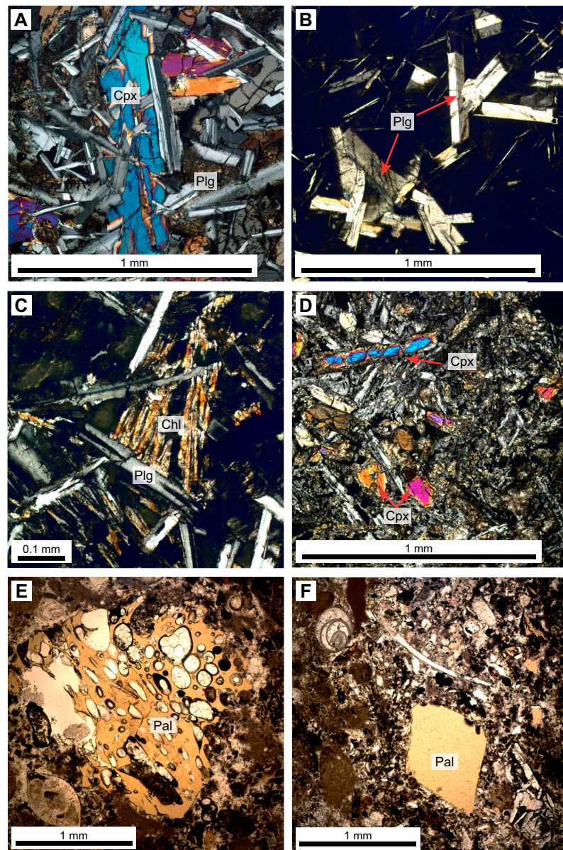
Figure F17. Representative basaltic rock sill material, Site U1547. A–D = XPL, E, F = PPL. A. Subophitic textures in aphyric basaltic rock (385-U1547D-8R-2; thin section [TS] 37). B. Glomeroporphyritic texture in plagioclase (Plg) phyric basaltic rock (385-U1547B-24F-1; TS 23). C. Complete alteration with chlorite (Chl) (385-U1547A-26X-2; TS 21). D. Partial alteration of clinopyroxene (Cpx) (385-U1547B-45X-1; TS 26). E, F. Representative peperite occurrence (385-U1547C-8R-1; TS 30). Pal = palagonite.
