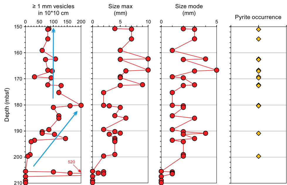
Figure F16. Vesicle abundance, maximum vesicle size, vesicle size mode, and qualitative record of pyrite occurrence for the deeper sill interval in Hole U1547B (385-U1547B-30X-1 through 50X-1).
