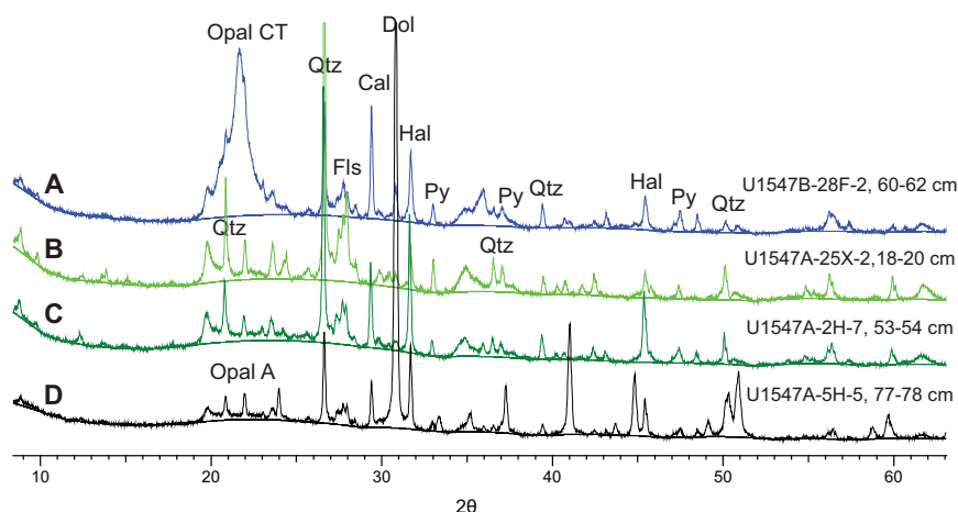
Figure F7. Representative XRD spectra, Site U1547. A. Siliceous claystone from Subunit ID. B, C. Clay-rich diatom ooze from (B) Subunit IB and (C) Subunit IA. D. Dolomite concretion. Qtz = quartz, Hal = halite, Cal = calcite, Fls = feldspar, Py = pyrite. Opal-CT is present in the sample from Subunit ID, whereas opal is still present in the other samples.
