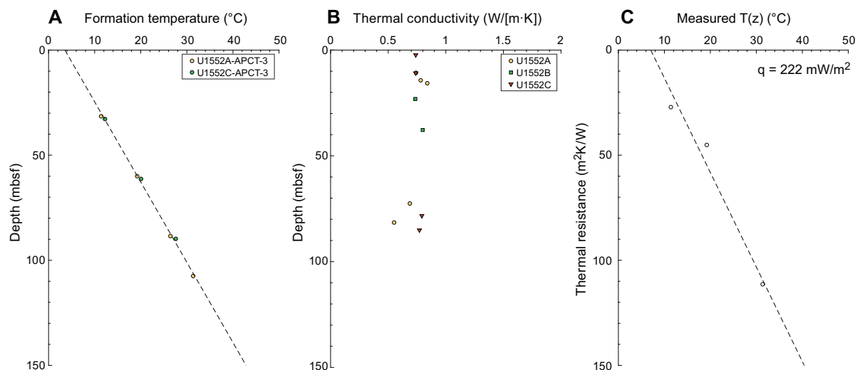
Figure F22. Heat flow calculations, Site U1552. A. Formation temperature measurements. APCT-3 = advanced piston corer temperature tool. B. Measured thermal conductivity. C. Heat flow, q [mW/m 2 ], shown as the slope of the line relating T(z) to cumulative thermal resistance.
