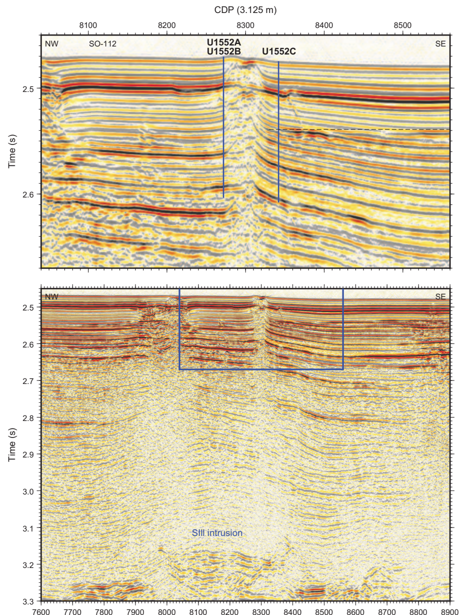
Figure F3. Bottom: Seismic Line SO-112 with an interpreted sill intrusion indicated at ~3.2 s two-way traveltime (TWT). Moderately blanked zones extend upward from the edges of this sill and have a substantial expression in the upper 0.15 s TWT (~110 m) of sediment. Blue box = expanded view shown in top panel. Top: enlarged view of the southeastern pipe structure with hole locations indicated. Near the pipe, between the locations of Holes U1552A–U1552C, strata in the upper 0.015 s TWT terminate against a structure that is interpreted to be a mostly buried mound. The black dashed line at ~2.54 s TWT southeast of the pipe indicates the interpreted base of a gas hydrate stability zone inferred from change in reflectivity crosscutting strata. This horizon is not apparent on the northwest side of the pipe. CDP = common depth point.
