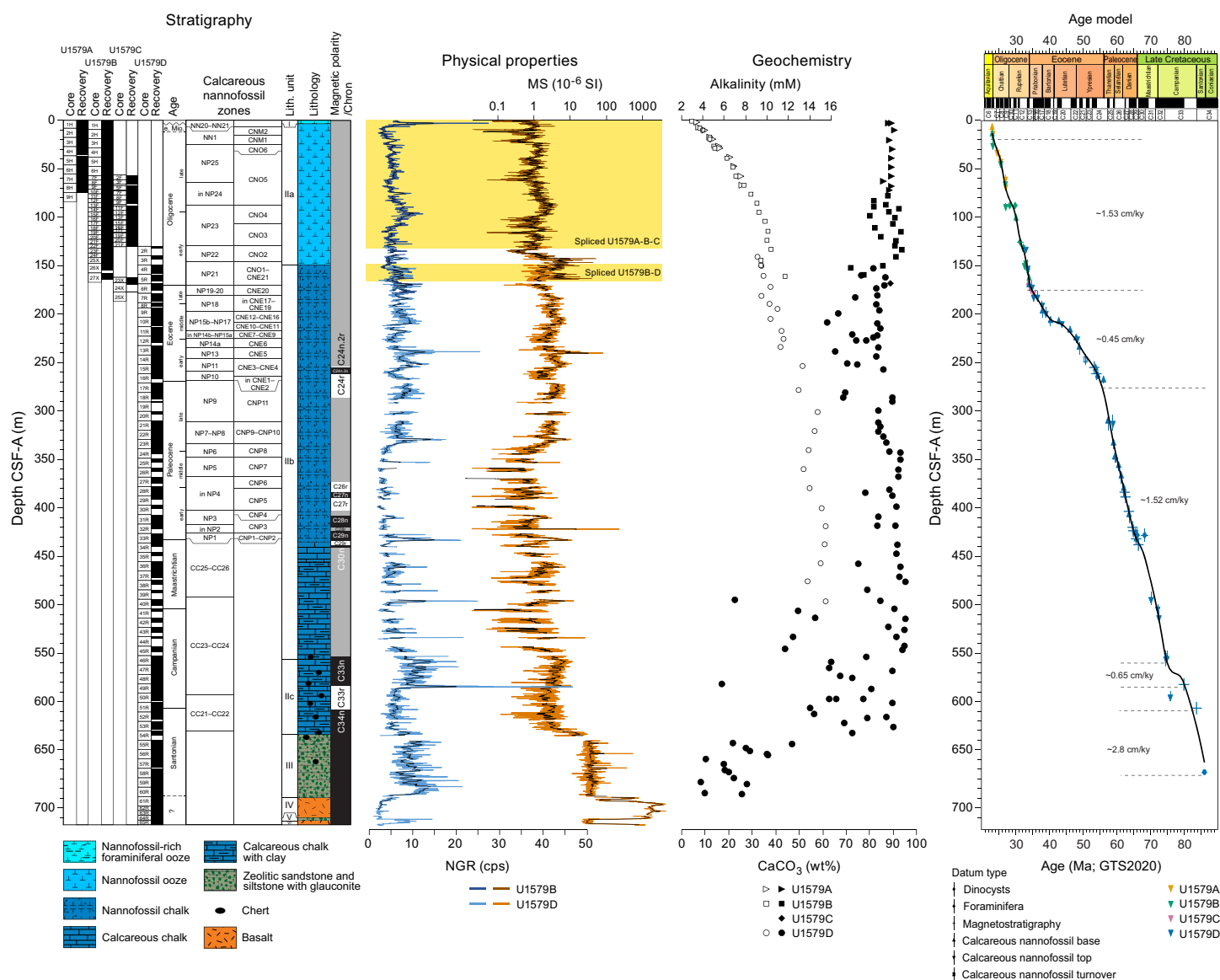
Figure F7. Stratigraphic summary, Site U1579. Calcareous nannofossil zones: NP following Martini (1971); CC following Sissingh (1977); CN following Agnini et al. (2014). Physical properties of NGR: dark blue = U1579B, light blue = U1579D, black = 15-point moving average, cps = counts per second. WRMSL MS: brown = U1579B, orange = U1579D, black = 25-point moving average. Alkalinity measurements (open symbols = Holes U1579A, U1579B, and U1579D) are from pore waters. Carbonate content (black closed symbols = all holes) is from bulk sediments. Age model is based on biostratigraphy and magnetostratigraphy, with estimated sedimentation rates. Yellow rectangles = stratigraphic intervals for which a splice is constructed.
