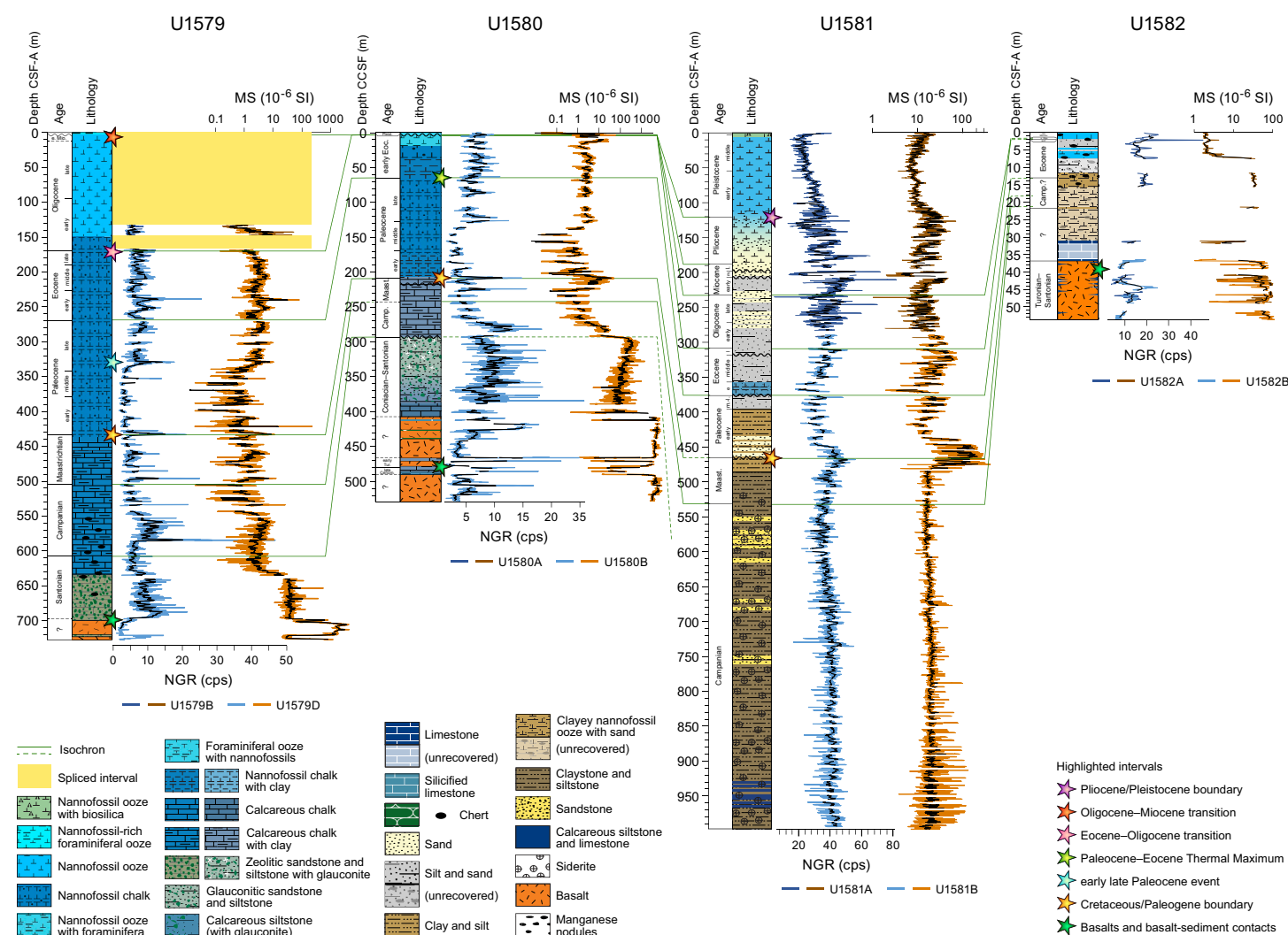
Figure F14. Lithologic summary with NGR and MS, Sites U1579–U1582. cps = counts per second.
