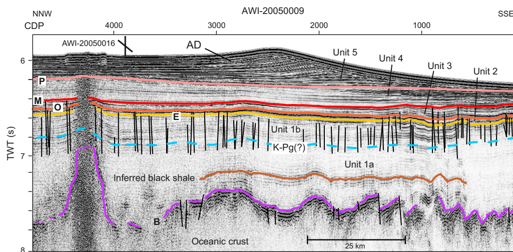
Figure F5. Pre-Expedition 392 seismostratigraphic model developed for the Transkei Basin (Schlüter and Uenzelmann-Neben, 2007). CDP = common depth point, TWT = two-way traveltime, B = top basement, K-Pg(?) = Cretaceous/Paleogene(?) boundary, E = late Eocene, O = Eocene/Oligocene boundary, M = middle Miocene, P = early Pliocene.
