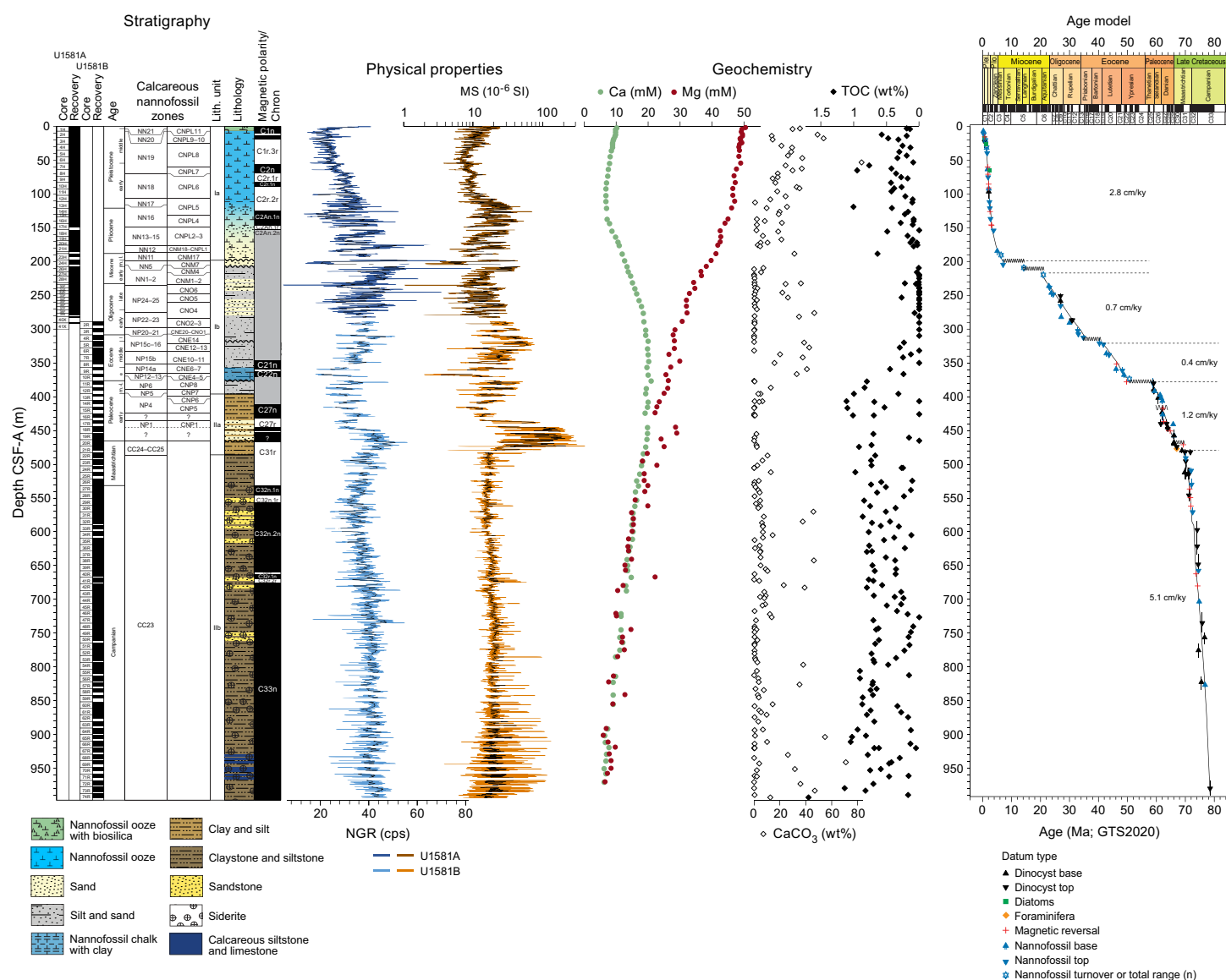
Figure F11. Stratigraphic summary, Site U1581. Calcareous nannofossil zones: NP following Martini (1971); CC following Sissingh (1977); CN following Agnini et al. (2014). Black NGR data = 15-point moving average, cps = counts per second, black WRMSL MS data = 25-point moving average. Ca (green circles) and Mg concentrations (red circles) are from pore waters. Carbonate (white diamonds) and TOC (black diamonds) contents are from bulk sediments (open circles). Age model is based on biostratigraphy and magnetostratigraphy, with reference to the GTS2020 (Gradstein et al., 2020) with estimated sedimentation rates.
