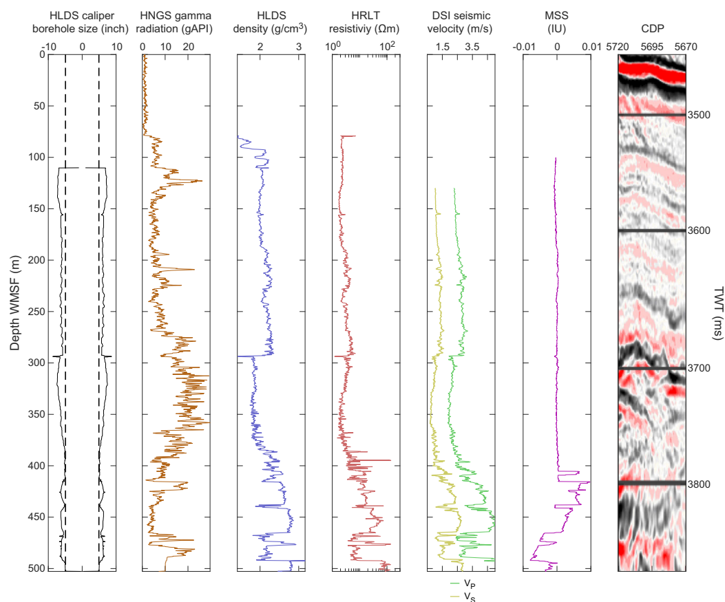
Figure F47. Downhole wireline logging results, Hole U1580A. Right column shows 50 traces of Seismic Line AWI-98015 in two-way traveltimes (TWT) around Site U1580, located at common depth point (CDP) 5695. HRLT = High-Resolution Laterolog Array.
