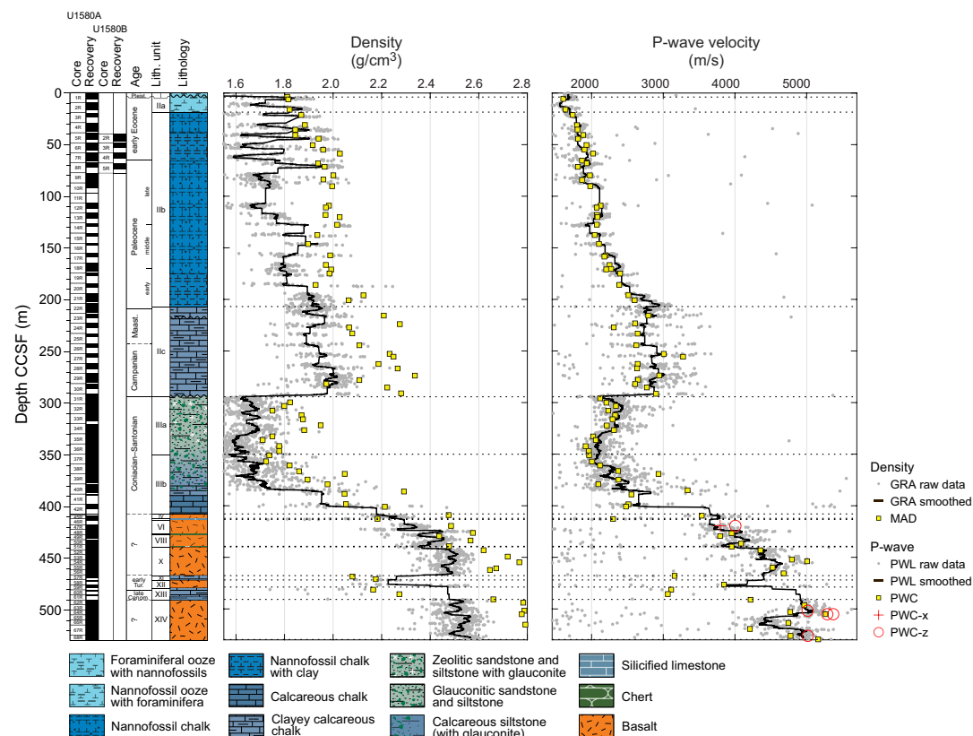
Figure F46. WRMSL density and P -wave velocity, Site U1580. All plotted data sets omit poor quality data points such as from section ends, cracks in the cores, or poor contact between the core and core liner.
