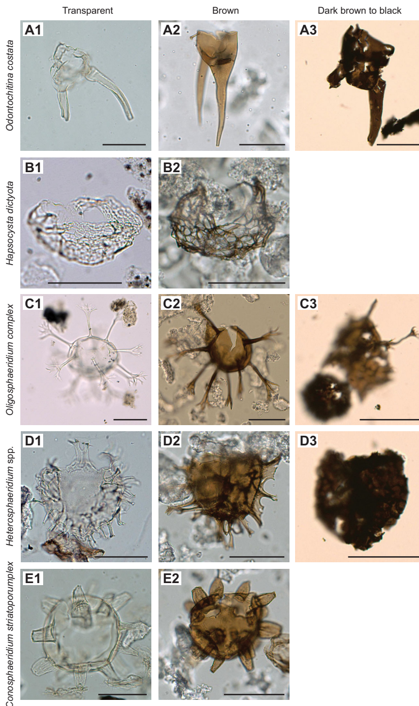
Figure F23. Color variation of specimens of Odontochitina costata , Hapsocysta dictyota , Oligosphaeridium complex, Heterosphaeridium spp., and Conosphaeridium striatoporum complex from Hole U1580A. Scale bar = 50 \mu m. Transparent (A1–E1), brown with rust colorations (A2–E2), and dark brown to black (A3, C3, D3). A (1) 34R-2, 133–134 cm (322.74 m CSF-A); (2) 35R-CC (339.38 m CSF-A); (3) 60R-1, 51–53 cm (481.11 m CSF-A). B (1) 38R-6, 66–67 cm (365.7 m CSF-A); (2) 40R-3, 21–24 cm (381.33 m CSF-A). C (1) 40R-3, 21–24 cm; (2) 35R-CC (339.38 m CSF-A); (3) 60R-1, 51–53 cm (481.11 m CSF-A). D (1) 4R-2, 133–134 cm (322.74 m CSF-A); (2) 35R-CC (339.38 m CSF-A); (3) 60R-1, 51–53 cm (481.11 m CSF-A). E (1) 34R-2, 133–134 cm (322.74 m CSF-A); (2) 35R-CC, 25–30 cm (339.38 m CSF-A).
