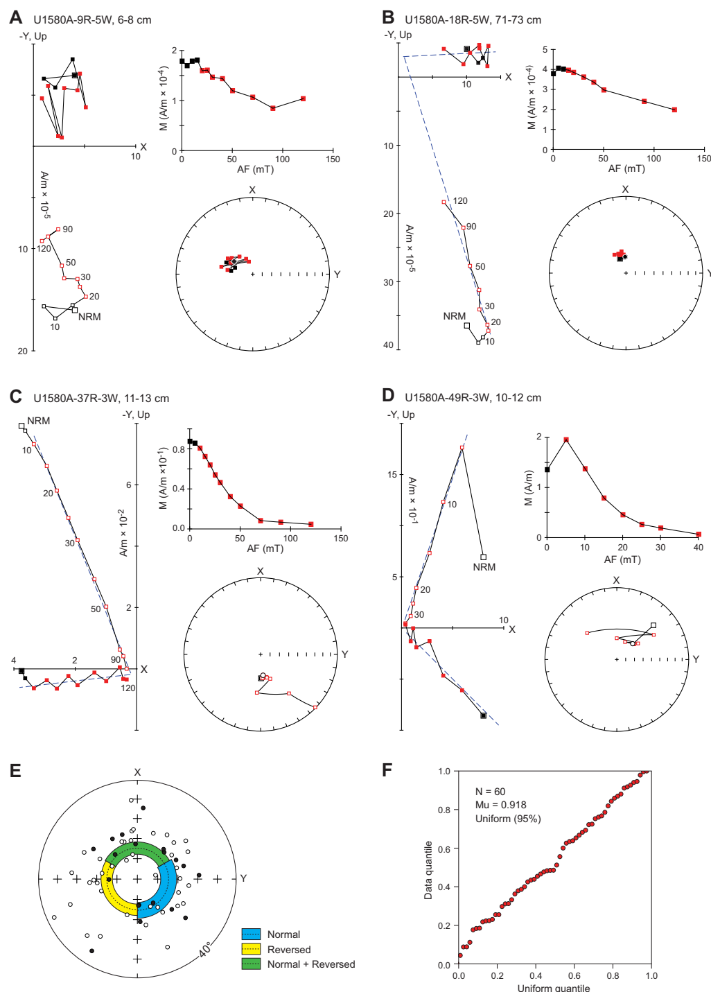
Figure F28. Discrete sample demagnetization analysis, Hole U1580A. A–C. Representative vector endpoint diagrams (left panels), equal area projections (round panels), and a graph showing natural magnetization (M) decay during demagnetization from Lithostratigraphic Units II–III (top right panels). D. Representative vector endpoint diagram (left panel), equal area projection (round panel), and a graph showing natural magnetization (M) decay during demagnetization from igneous rocks (Lithostratigraphic Unit VIII) (top right panel). Vector endpoint diagrams: white symbols = projections onto the vertical plane, black symbols = projections onto the horizontal plane, X and Y = axes of the working halves, and Up = vertical up-pointing (–Z)-axis of the core. Equal-area projections: open symbols = negative (up-pointing) directions, black symbols = positive (down-pointing) directions. All plots: red symbols = steps used to determine the characteristic remanent directions. E. Equal-area projection with all down-pointing (reversed; solid symbols) and up-pointing (normal; open symbols) paleomagnetic directions. Average inclination and 95% confidence boundaries are indicated in the inset (N + R = combined normal and reversed directions). F. Results from quantile-quantile analysis used to attest the uniformity of measured declinations; if \mu > 1.207 , the null hypothesis of a uniform distribution of declination can be excluded at a 95% certainty (Fisher et al., 1987; Tauxe, 2010); the uniformly distributed declination values support the lack of pervasive drilling-induced magnetic overprints.
