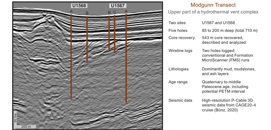
Figure F5. High-resolution 3-D seismic data showing the position of Site U1567 and U1568 holes along the Modgunn Transect across the upper part of a hydrothermal vent complex.
