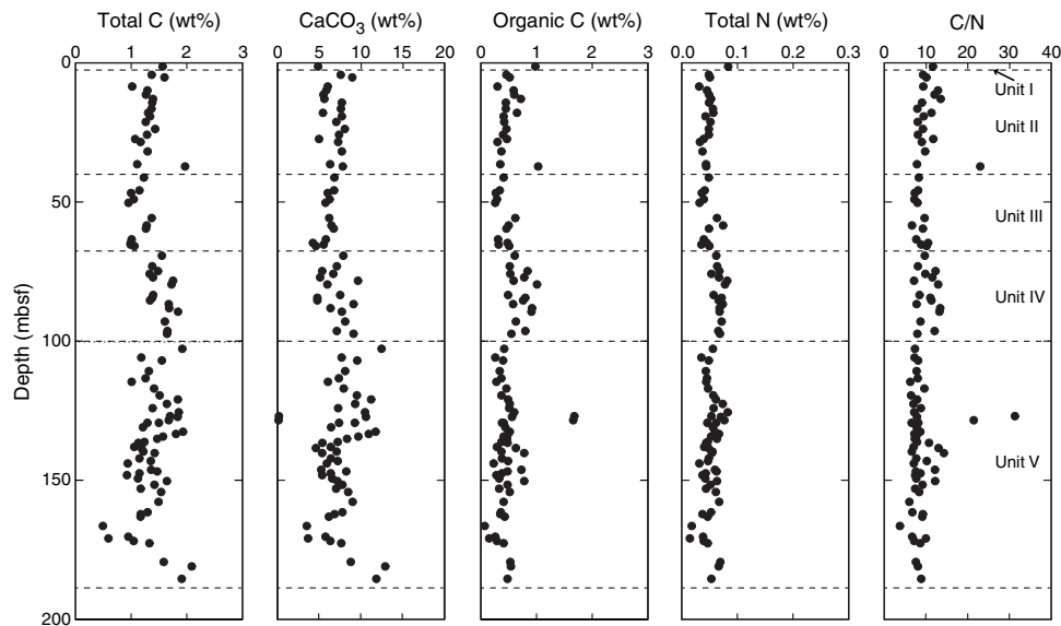
Figure F27. TC, CaCO 3 , total organic C, and TN downhole profiles and organic carbon to TN weight (C/N) ratio, Site U1517.
