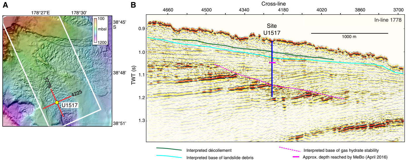
Figure F1. A. Bathymetry around Site U1517 with in-line and cross-line tracks from the 3-D seismic cube (white rectangle). B. IL1778 seismic section from the 3-D cube crossing Site U1517 with interpreted key horizons.
