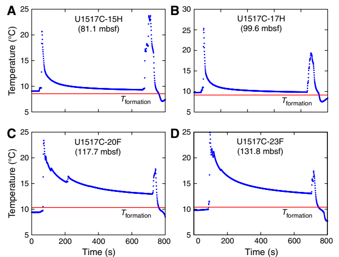
Figure F33. APCT-3 temperature-time data (blue dots) and estimated formation temperature ( T_{\text{formation}} ; red line), Hole U1517C. A. Data from 81.1 mbsf deployment with estimated formation temperature of 8.55°C. B. Data from 99.6 mbsf deployment with estimated formation temperature of 9.14°C. C. Data from 117.7 mbsf deployment with estimated formation temperature of 10.32°C. D. Data from 131.8 mbsf deployment with estimated formation temperature of 10.39°C.
