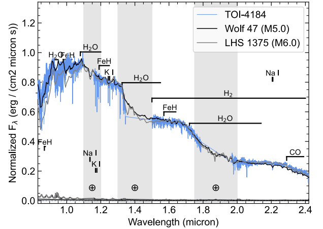
Fig. 5. Magellan/FIRE spectrum of TOI-4184. The SpeX Prism spectrum of the M5.0 standard Wolf 47 and M6.0 standard LHS 1375 (Kirkpatrick et al. 2010) are shown for comparison. Strong M dwarf spectral features are indicated, and high-telluric regions are shaded. Lines along the bottom of the plot give the uncertainties associated with the spectra.
