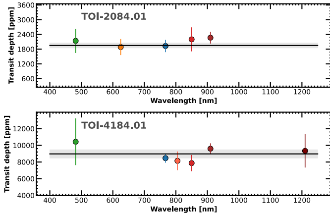
Fig. 11. Transit depths measured for multi-band photometric follow-up of TOI-2084.01 ( top panel ) and TOI-4184.01 ( bottom panel ). Solid horizontal lines correspond to the TESS measured transit depth.
