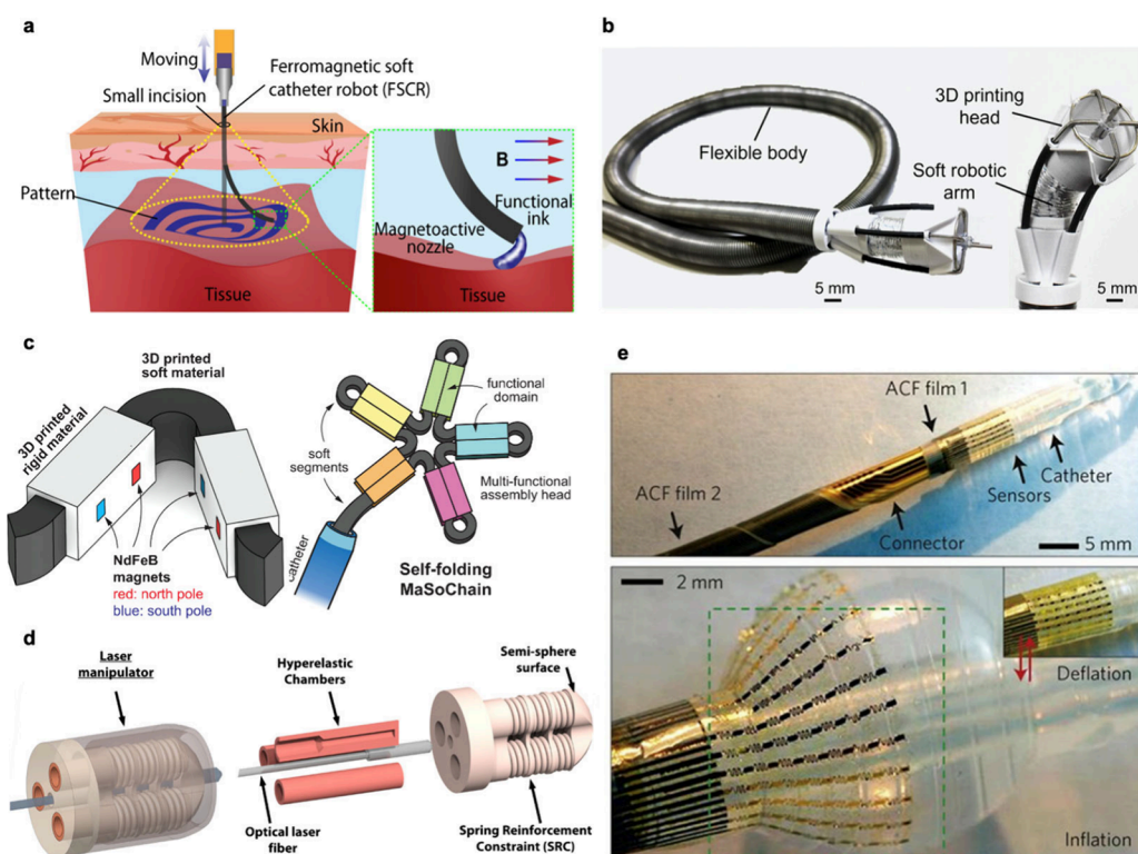
Figure 16. Functionalized catheters. (a) Ferromagnetic soft catheter robot for in vivo bioprinting through incisions through the skin. Reproduced with permission from ref 357 under CC BY 4.0. Copyright 2021 Springer Nature. (b) Flexible hydraulic arm for maneuvering 3D printhead with a tip that also has hydraulic XYZ control for precise positioning. Reproduced with permission from ref 358 under CC BY 4.0. Copyright 2023 Wiley. (c) Magnetic soft robotic chains for shape reconfiguration into multifunctional devices. Reproduced with permission from ref 359 under CC BY 4.0. Copyright 2023 Springer Nature. (d) Three channel hydraulically controlled laser manipulator for tumor ablation and microsurgery. Reproduced with permission from ref 360. Copyright 2021 The American Association for the Advancement of Science. (e) Multifunctional balloon catheter integrating sensors for temperature, pressure, flow, and electrophysiology monitoring. Reproduced with permission from ref 127. Copyright 2011 Springer Nature.
