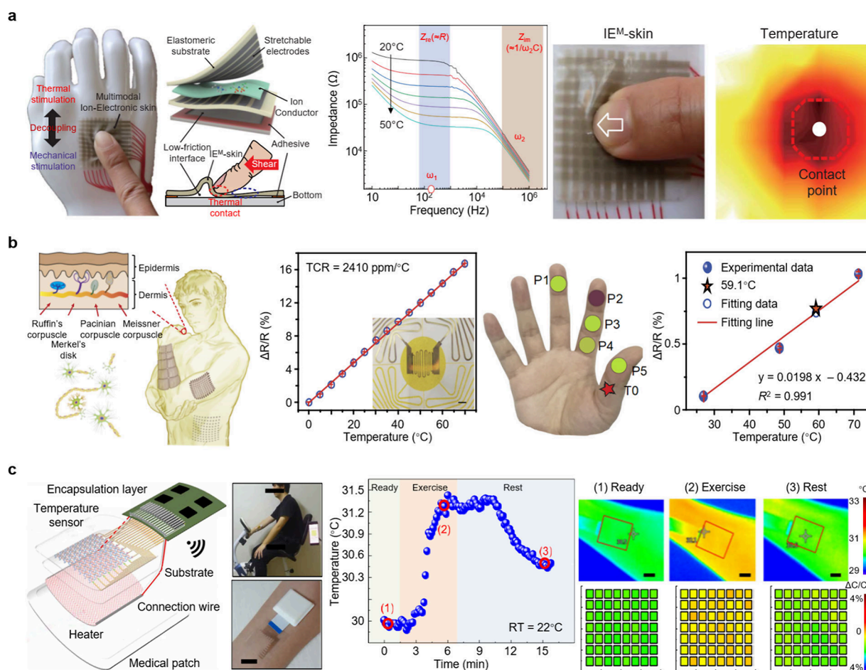
Figure 4. Temperature sensing for soft robotics. (a) Schematic of the multimodal ion-electronic skin and the responses under a unidirectional shear applied by the forefinger with the corresponding profiles of temperature. Reproduced with permission from ref 207. Copyright 2020 The American Association for the Advancement of Science. (b) Skin-inspired highly stretchable and conformable matrix networks with the linear changes along the temperature for the intelligent prosthetic hand configuration. Reproduced with permission from ref 208 under CC BY 4.0. Copyright 2018 Springer Nature. (c) Wireless skin-mounted graphene-based thermal patch for obtaining temperature distribution. Scale bar, 2 cm. Reproduced with permission from ref 209. Copyright 2022 The American Association for the Advancement of Science.
