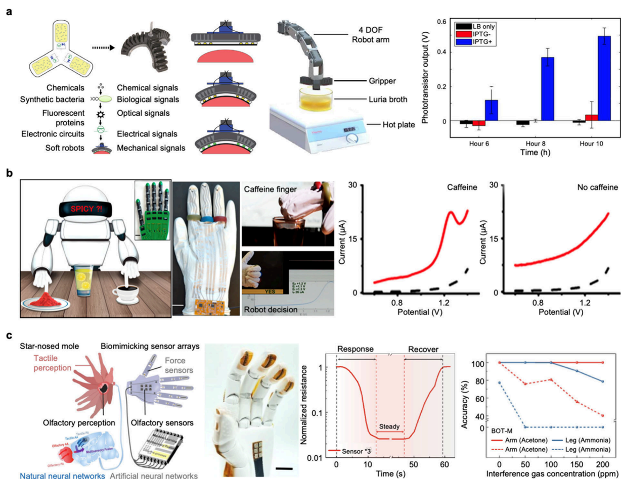
Figure 5. Biochemical sensing for soft robotics. (a) A biosensing soft robotic arm for autonomous parsing of chemical signals in an aqueous environment. Reproduced with permission from ref 212. Copyright 2019 The American Association for the Advancement of Science. (b) Chemical sensing at the robot fingertips for automated taste discrimination in food samples. Scale bar, 5 cm. Reproduced with permission from ref 213. Copyright 2018 American Chemical Society. (c) Bioinspired tactile-olfactory bionic sensing array for response during the gas flow with high recognition accuracy. Scale bar, 3 cm. Reproduced with permission from ref 214 under CC BY 4.0. Copyright 2022 Springer Nature.
