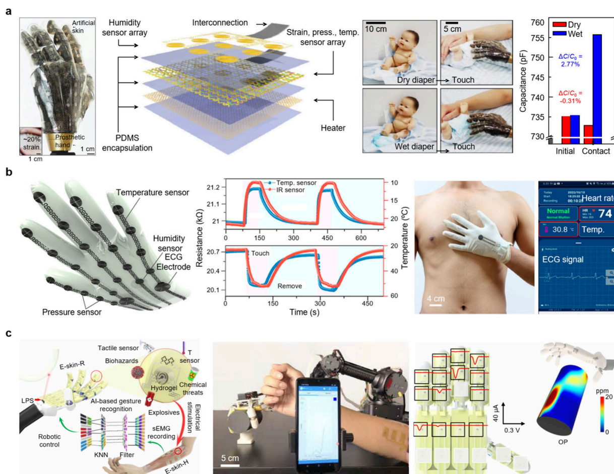
Figure 7. Multimodal sensing for soft robotics. (a) Smart artificial skin with stretchable sensors in various robotic-assisted situations. Reproduced with permission from ref 227. Copyright 2014 Springer Nature. (b) Stretchable electronic glove for simultaneous detection of multiple stimuli and demonstration of human–machine interfacing. Reproduced with permission from ref 228. Copyright 2023 American Chemical Society. (c) All-printed soft interface with robotic physiochemical sensing for gesture recognition with robotic control and mapping of hazardous distributions on the object. Reproduced with permission from ref 229. Copyright 2022 The American Association for the Advancement of Science.
