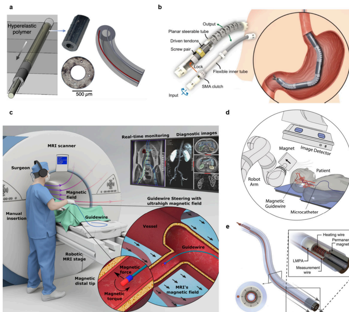
Figure 15. Steerable tethered robotic tools. (a) Hyperelastic microcatheter with four hydraulically actuated channels. Reproduced with permission from ref 347. Copyright 2021 The American Association for the Advancement of Science. (b) Hand-held robot with shape memory alloy clutch for bending modules. Reproduced with permission from ref 348 under CC BY 4.0. Copyright 2024 Springer Nature. (c) MRI-controlled magnetic guidewire that can operate under ultrahigh magnetic fields. Reproduced with permission from ref 349 under CC BY 4.0. Copyright 2023 The American Association for the Advancement of Science. (d) Telerobotic controlled robotic arm to manipulate a ferromagnetic soft continuum robot for neurovascular surgeries. Reproduced with permission from ref 350. Copyright 2022 The American Association for the Advancement of Science. (e) Variable stiffness catheter with a low-melting point alloy, heating coil, and permanent magnet tip. Reproduced with permission from ref 351 under CC BY 4.0. Copyright 2022 Wiley.
