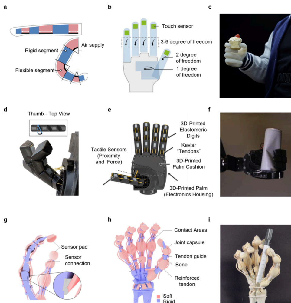
Figure 11. Soft prosthetics. (a) A soft pneumatic neuroprosthetic hand. Fiber-reinforced elastomeric tubular structure expands radially and contracts axially when inflated, enabling pneumatic actuation and control of soft fingers. (b) Schematic shows six active degrees of freedom for dexterous grasping and manipulation capabilities. (c) Photo of a transradial amputee wearing the soft neuroprosthetic hand, grasping a cupcake demonstrating its functionality. (a–c) Reproduced with permission from ref 283. Copyright 2023 Springer Nature. (d) A line-tendon driven robotic hand. Time-lapse image depicting thumb flexion achieved through line-driven tendon/cable actuation. (e) Schematic illustrating the line-tendon driven actuation mechanism for the prosthetic hand. (f) Utilizing elastomeric passive transmission technology, this robotic hand can balance speed and force output. (d–f) Reproduced with permission from ref 286. Copyright 2018 The American Association for the Advancement of Science. (g) 3D printed multimaterial bionic hand. Cross-sectional view of the index finger reveals the internal tendon structure, sensor cavity, and joint geometry. (h) Schematic with different colors representing the distinct materials used in the 3D printed construction. (i) Image shows various objects grasped by the bionic hand, enabled by a control algorithm for versatile grasping. (g–i) Reproduced with permission from ref 292 under CC BY 4.0. Copyright 2023 Springer Nature.
