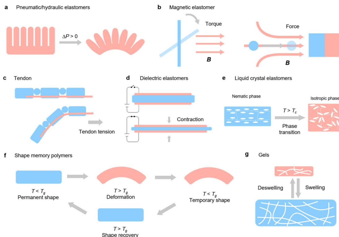
Figure 2. Actuation mechanisms for soft robotics categorized by material types. (a) Pneumatic/hydraulic elastomers: Fluidic pressure within the robot's internal cavities controls movement. (b) Magnetic elastomers: Soft elastomers embedded with magnetic particles offer precise control via torques or forces in response to an external magnetic field. (c) Tendon: Tension applied to tendons leads to deformation of the structure; elastic hinges store energy to return the actuated parts to their initial states. (d) Dielectric elastomers: Electrostatic forces between compliant electrodes compress a sandwiched dielectric material, resulting in deformation. (e) Liquid crystal elastomers: Stimuli induce phase changes in liquid crystal elastomers, affecting polymer chain orientation and length, thus altering the material's configuration. (f) Shape memory polymers: Actuation is triggered when the temperature surpasses a specific threshold, enabling shape-memory materials to revert to predefined shapes. (g) Gels: Environmental stimuli prompt volume changes in gels, dynamically influencing their shape and size.
