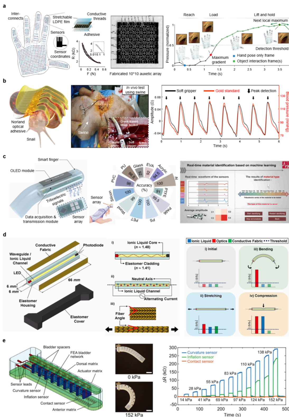
Figure 3. Exteroceptive and proprioceptive sensing for soft robotics. (a) Scalable tactile glove learning from the signatures of the grasp to decompose a tactile map. Reproduced with permission from ref 186. Copyright 2019 Springer Nature. (b) Miniaturized, nature-inspired, hand-shaped soft gripper for in vivo vital sign monitoring. Reproduced with permission from ref 187. Copyright 2021 The American Association for the Advancement of Science. (c) Triboelectric artificial tactile perception smart finger for material identification. Reproduced with permission from ref 189. Copyright 2022 The American Association for the Advancement of Science. (d) Multifunctional soft sensor for mechanoreception and proprioception of soft robots. Reproduced with permission from ref 190. Copyright 2020 The American Association for the Advancement of Science. (e) A soft robotic gripper combines multiple somatosensitive actuators with embedded sensors, providing proprioceptive and haptic feedback including deep and fine touch sensing. Reproduced with permission from ref 191. Copyright 2018 Wiley.
