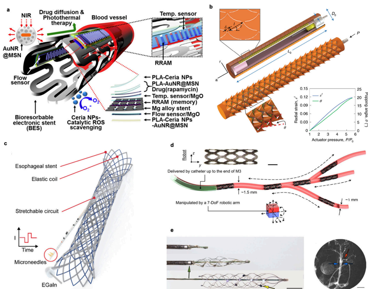
Figure 21. Soft robotic stents. (a) Bioresorbable bioelectronic stent with integrated sensors, wireless power and data transmission, and ceria nanoparticles for inflammation suppression. Reproduced with permission from ref 443. Copyright 2015 American Chemical Society. (b) Kirigami-inspired esophageal stent with drug-loaded polymers in microneedles for extended drug delivery. Reproduced with permission from ref 444. Copyright 2021 Springer Nature. (c) Nitinol stent with liquid metal antenna and stretchable circuits for electrical stimulation in the esophagus. Reproduced with permission from ref 445. Copyright 2023 The American Association for the Advancement of Science. (d) Shape memory polymer-based stent with magnetic particles for navigation in distal vasculature. Scale bar, 1 mm. Reproduced with permission from ref 446 under CC BY 4.0. Copyright 2022 Springer Nature. (e) Microelectrode array mounted onto a nitinol stent for a minimally invasive endovascular neural interface. Scale bar, 3 mm (left). Scale bar, 10 mm (right). Reproduced with permission from ref 447. Copyright 2016 Springer Nature.
