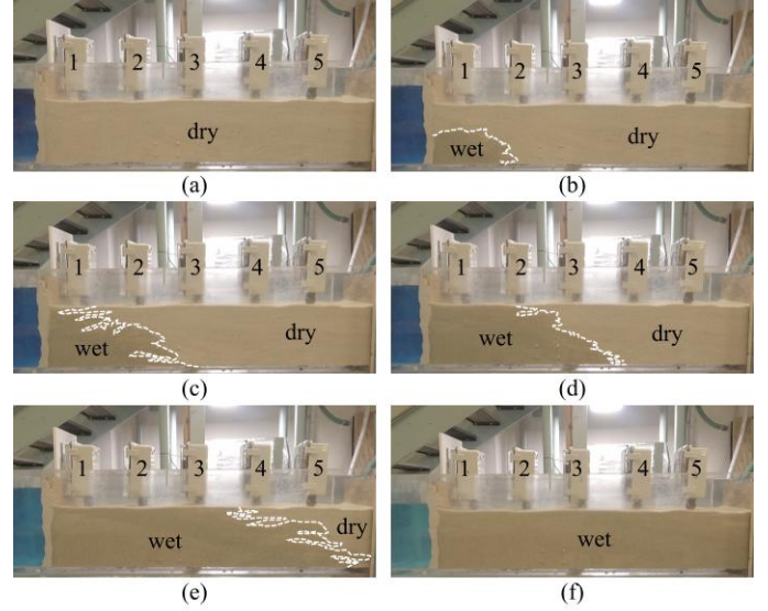
FIGURE 7. The experimental configuration illustrating the locations of five wireless sensing spike packages as moisture spreads, including (a) side view at TS 1; (b) side view at TS 2; (c) side view at TS 3; (d) side view at TS 4; (e) side view at TS 5; and (f) side view at TS 6.
