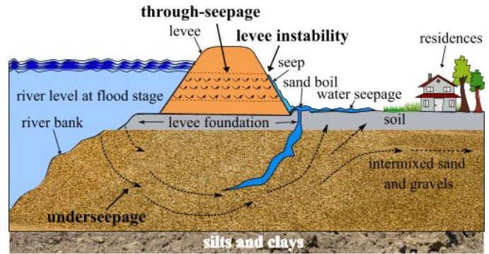
FIGURE 1. Diagram of an earthen levee depicted in cross-section, featuring labeled layers and potential areas of structural weakness.
