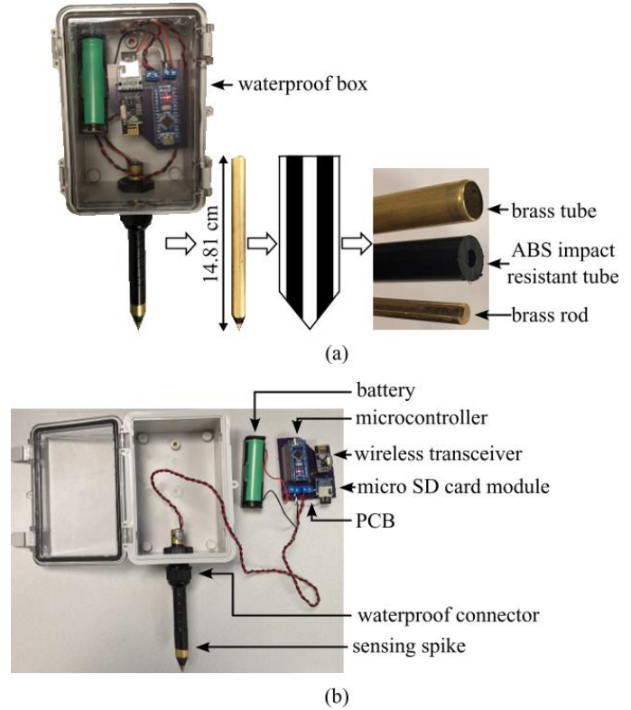
FIGURE 2. Detailed layout of a wireless sensing spike package with key components, showing: (a) outside view of the package; and (b) inside view of the package.
