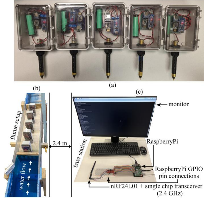
FIGURE 4. Overall wireless communication of a network of sensing spike packages, displaying: (a) network of five wireless sensing spike packages, (b) layout of the flume setup, and (c) detailed layout of the base station.
