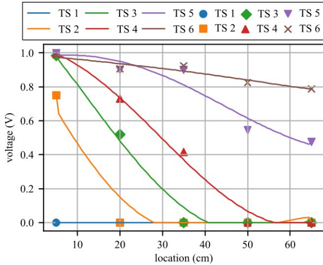
FIGURE 8. 1D kriging outcomes from the moisture test for six-TS.
