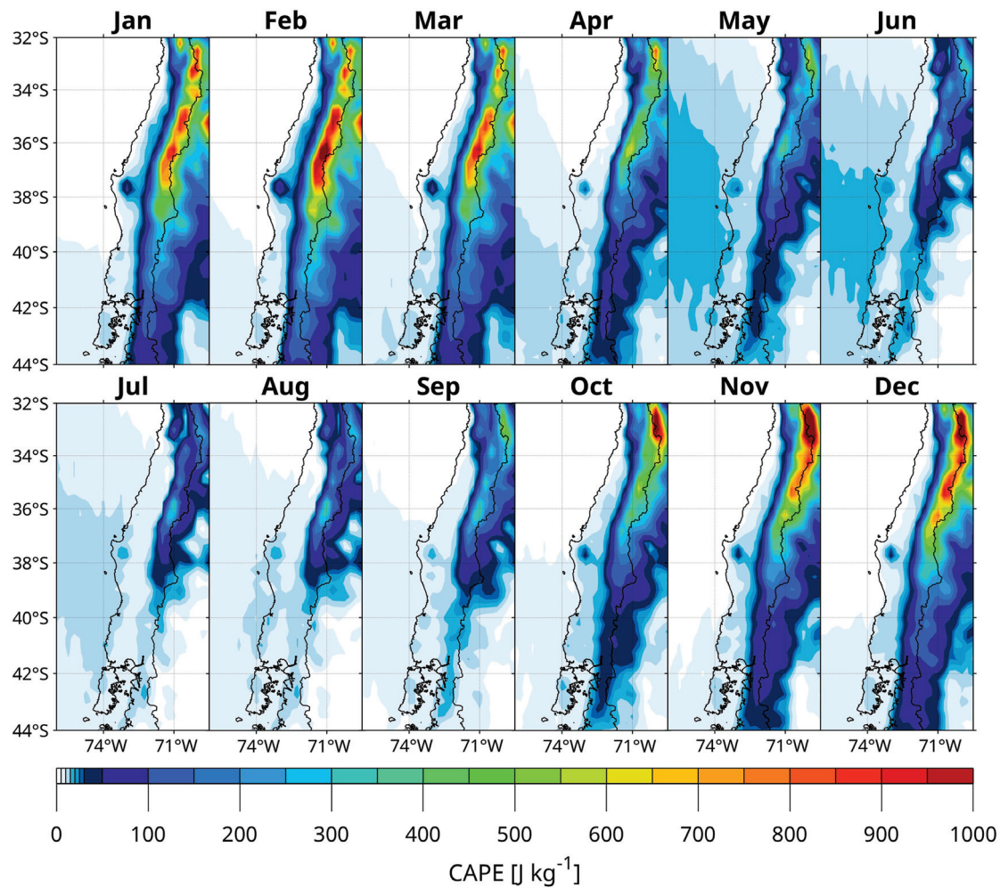
FIG. 5. Monthly distribution of mean MLCAPE (1959–2021).
