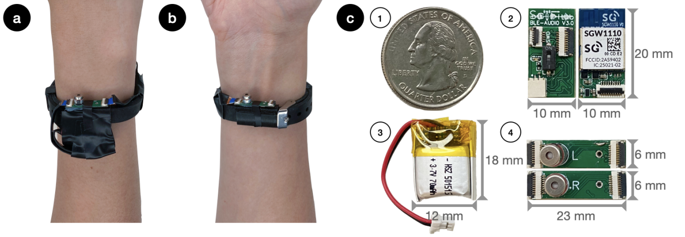
Figure 4: Hardware of EchoWrist. (a) (b) Wearing EchoWrist at the wrist. All components are mounted on a silicone wristband. (c) Customized PCBs for the microcontroller module and the sensing module. (1) US Quarter Dollar coin. (2) Customized PCB with SGW1110 module (front and back views). (3) 3.7 V 70 mAh LiPo battery. (4) Sensor module with speaker and microphone.
