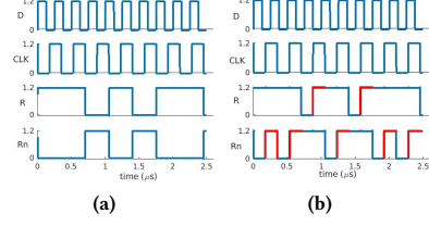
Figure 7: Simulation of polymorphic Register behavior: (a) at 0^\circ\text{C} , D is latched to R and the inverse to \bar{R} ( R_n ) when CLK is high; (b) at -40^\circ\text{C} , R and \bar{R} ( R_n ) both enter logical high state at CLK transition. This is invalid data and shows the register entering a forbidden state (red).
