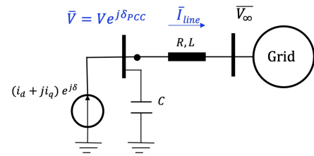
Fig. 3: The testbed for dynamic simulation.
