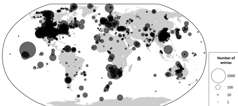
Figure 5. Bubble chart of the modern geographical distribution and sample quantities in the database.
