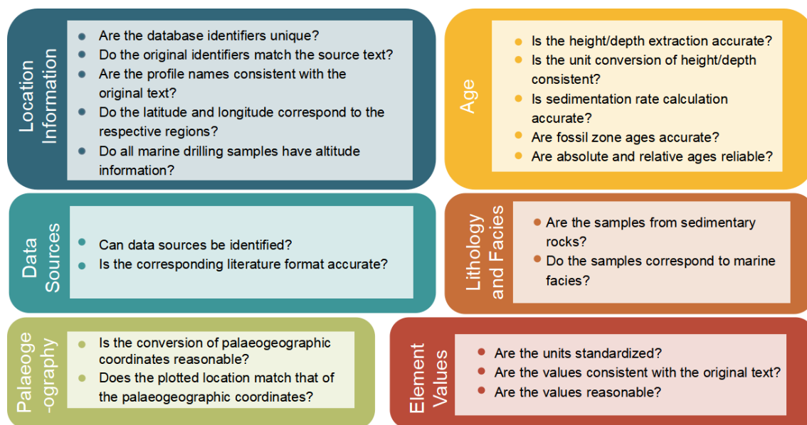
Figure 2. The data filtering and processing criteria for the DM-SED.
