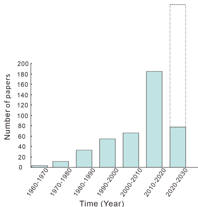
Figure 1. The distribution of the publication years for the newly compiled literature (the dashed line denotes the predicted literature from 2023 to 2030).
