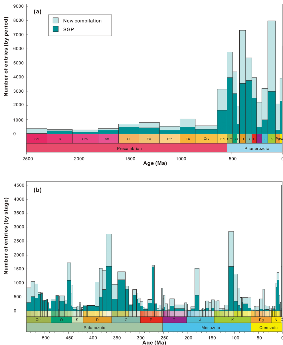
Figure 4. The age distribution of samples in the database. (a) Age distribution of samples (excluding a small number of samples with ages > 2500 Ma from the figure, for a total of 1258 samples). (b) Age distribution of Phanerozoic samples at the stage level. Sd: Siderian; R: Rhyacian; Ors: Orosirian; Stt: Statherian; Cl: Calymnian; Ec: Ectasian; Stn: Stenian; Tn: Tonian; Cry: Cryogenian; Ed: Ediacaran; Cm: Cambrian; O: Ordovician; S: Silurian; D: Devonian; C: Carboniferous; P: Permian; T: Triassic; J: Jurassic; K: Cretaceous; Pg: Paleogene; N: Neogene; Q: Quaternary.
