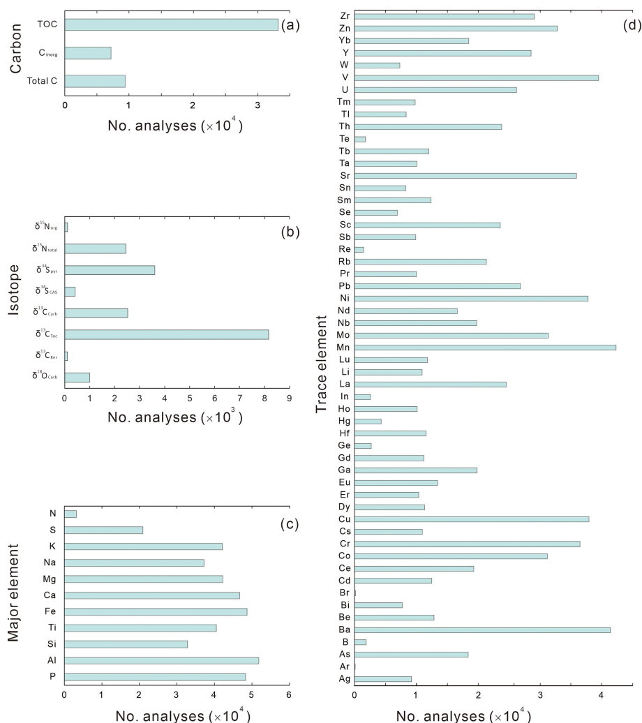
Figure 3. Histogram distribution of the different subsets. (a) Carbon elements. (b) Isotopes. (c) Major elements. (d) Trace elements.
