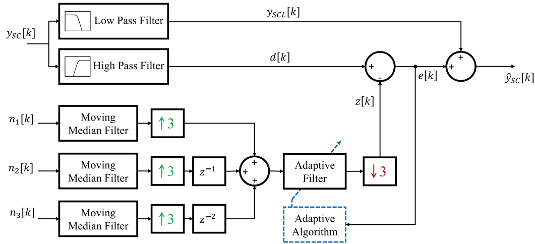
FIGURE 2. An Overview of Motion Artifact Reduction Algorithm: The above block diagram depicts multirate adaptive filtering architecture for motion artifact reduction from SC recording with three channel accelerometer recordings as the noise source reference. Figure shows how multi-channel noise reference stream is combined to a single stream via upsampling and delaying before feeding into adaptive filter. On the other hand SC is decomposed into d[k] and y_{scl}[k] high pass and low pass filters respectively. The error between high frequency components d[k] and adaptive filter artifact estimation z[k] is denoted as e[k] and is being fed back to the adaptive algorithm to update the adaptive filter coefficients.
