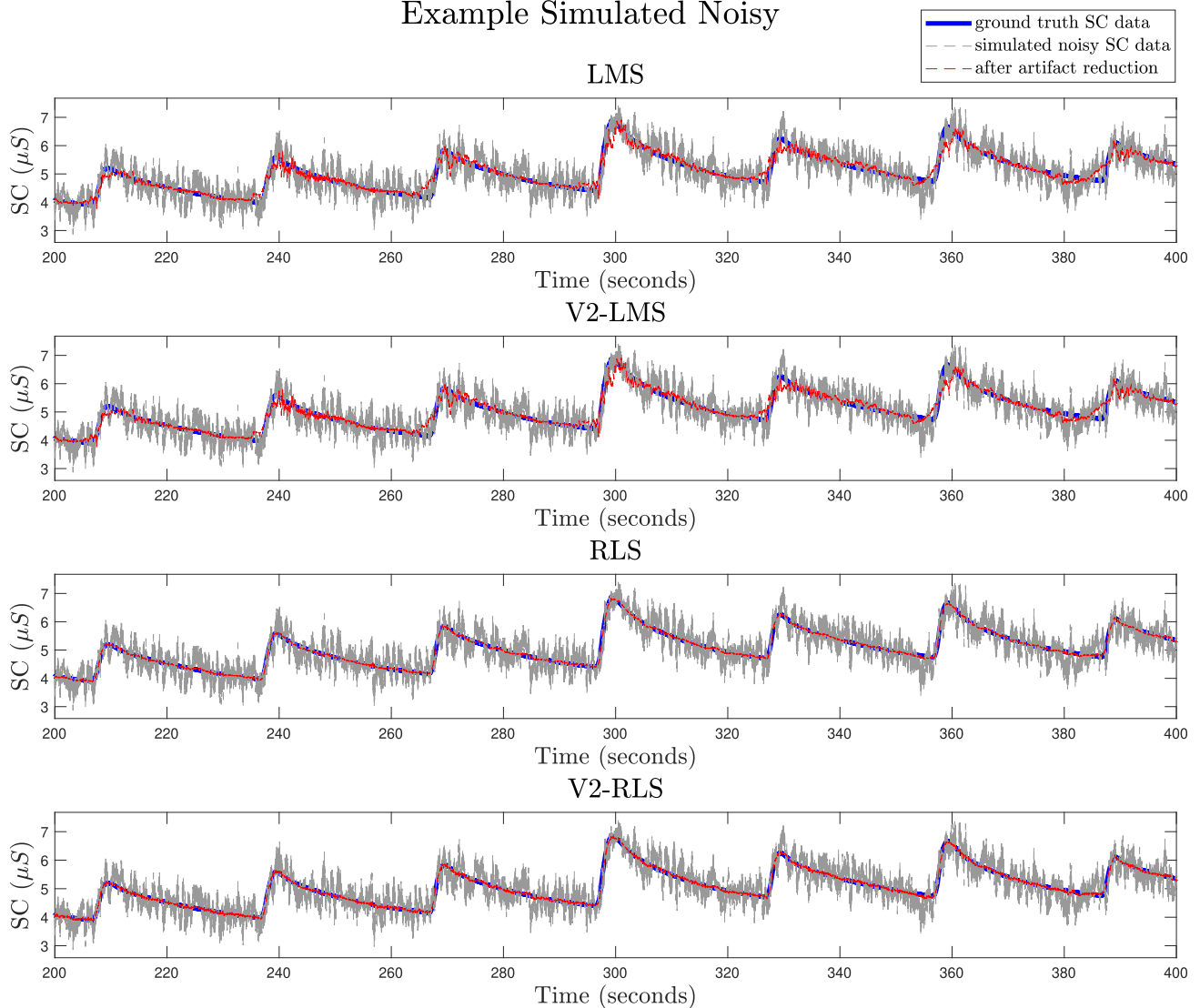
FIGURE 3. Non-linear Artifact Reduction Result Example with Simulated Noise Source. Subplots from top to bottom show the artifact removal performance with LMS filter, V2-LMS, RLS, V2-RLS filter with a single noise reference.
