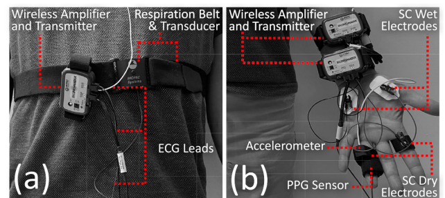
FIGURE 1. An Overview of the Experimental Setup. (a) A participant wearing respiration belt and the ECG leads; (b) and placements of SC sensor, accelerometer and PPG sensor on participants non-dominant hand.
