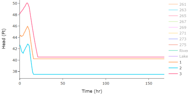
Fig. 8: Head Levels at Water Reserve Tanks over 1 Week (Pump Controller Sabotage)
