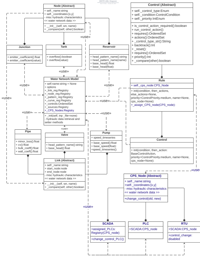
Fig. 1: WNTR Water Network Core Components (Black) + CPS Module Additions (Blue): Model, Nodes, Links, Controls, CPS_Nodes
