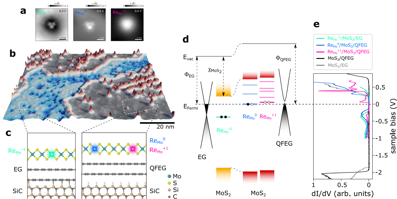
Fig. 2 | Charge state tristability of Re dopants in \text{MoS}_2 on EG and QFEG on SiC. a STM topographies ( I = 100 pA) of single Re dopants in the three different charge states ( \text{Re}_{\text{Mo}}^{-1} , \text{Re}_{\text{Mo}}^0 , and \text{Re}_{\text{Mo}}^{+1} ). b 3D representation of a large-scale STM image of Re-doped monolayer \text{MoS}_2 on domains of epitaxial graphene (EG) (center blue region) or domains of QFEG substrate (outer gray region). At positive bias (here 0.6 V), Re dopants are imaged as a dark blue pits on EG whereas they appear as red hills on \text{MoS}_2 grown on QFEG, depending on their charge states. c Atomic model of the \text{MoS}_2/\text{EG} and \text{MoS}_2/\text{QFEG} interface. On EG only \text{Re}_{\text{Mo}}^{-1} are observed, whereas on
